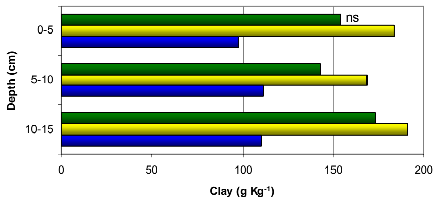
Figure 3. Management zones, tillage system and depths effects on clay content. Letters denote means separation between management zones at the same depth by LSD (0.10) . ns = differences were not significant.
