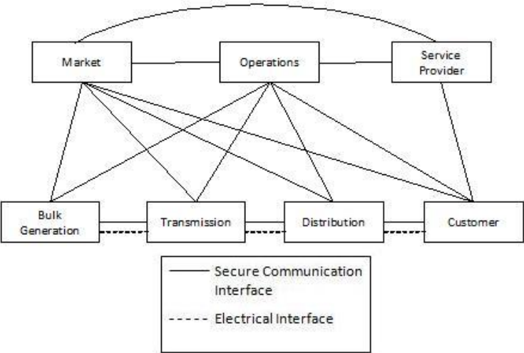
Figure 2.3: Smart Grid Technology
