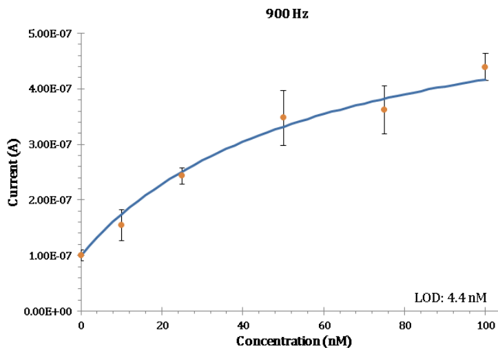
Figure 4.4: The dynamic range of Signal-ON current at 900 Hz covers target concentrations from 4.4 to 100 nM.
