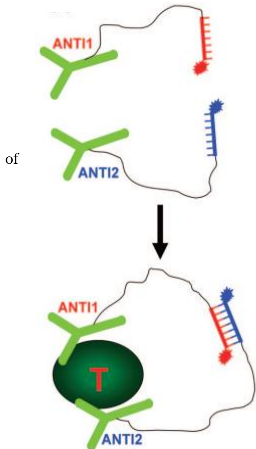
Figure 1.9: Molecular pincer assay. molecular beacons for detecting proteins based on ANTI1 and ANTI2 depict antibodies labeled with signaling oligonucleotides. T corresponds to the target protein.
