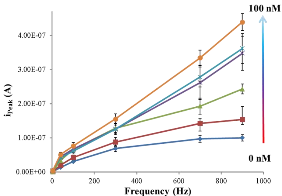
Figure 4.6: Sensors' response to various target-bound concentrations (0 nM, 10 nM, 25 nM, 50 nM, 75 nM, 100 nM). Error bars represent the standard deviations of measurements taken from 3 independent electrodes.
