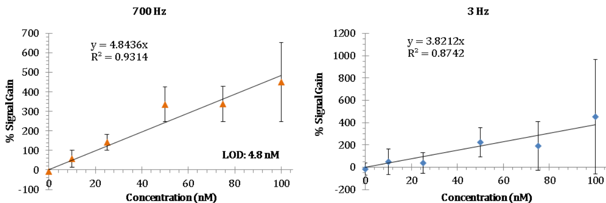
Figure 4.8: The signal gain of the bistable sensor is relatively large. Shown above are the sensor responses using SWV at various concentrations of fully complementary target-DNA at 3 Hz and 700 Hz. Electrode-to-electrode variability is enhanced at low SW frequencies (<10 Hz).
