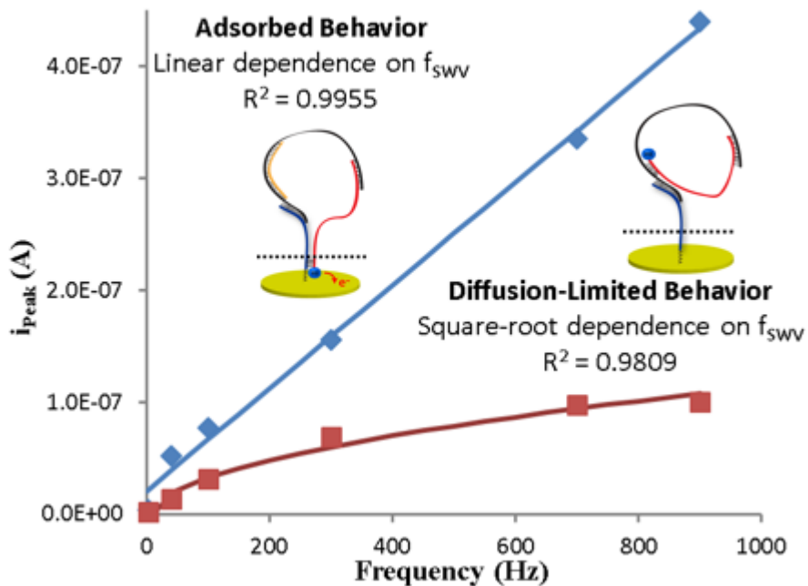
Figure 4.7: The sensor response changes from a square-root dependence on f_{\text{swv}} at low concentrations of target to a more linear dependence on f_{\text{swv}} at high concentrations of target
