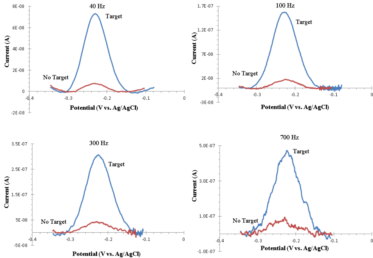
Figure 4.5: Peak current response curves for target-free and target-bound states for 100 nM EC-DNA sensor obtained using SWV at various frequencies.
