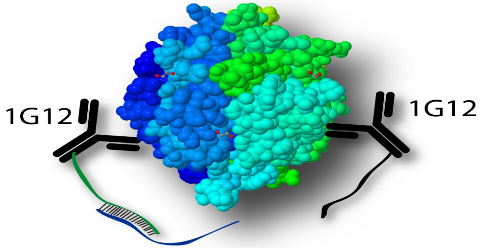
Figure 2.7: Theoretical schematic of the target protein molecule in a larger dimer formation in solution therefore DNA elongation may be required.
