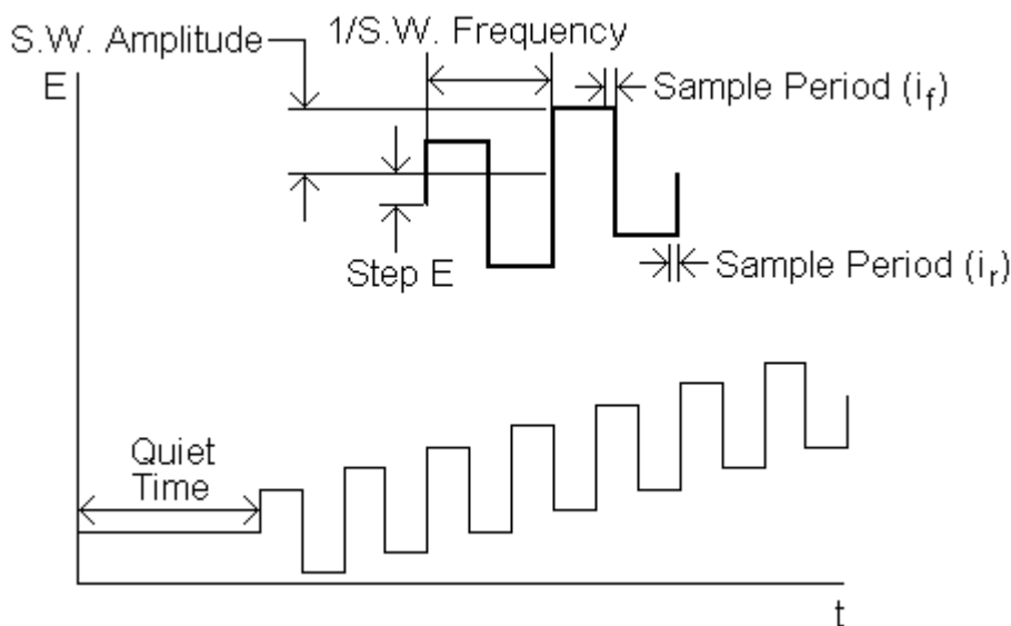
Figure 1.11: Potential wave form for square wave voltammetry.
