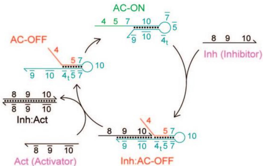
Figure 4.1: Zhang and Winfree design of an allosteric catalyst state that changed via the addition of inhibitor (Inh) and activator (Act). Inh binds to AC-ON to form the Inh:AC-OFF complex. Act binds to Inh:AC-OFF to remove the AC-OFF duplex and the waste product of Inh:Act. AC-OFF then spontaneously converts to AC-ON.
