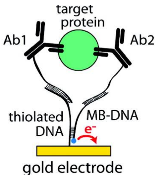
Figure 1.14: Electrochemical Proximity Assay (ECPA) combines the proximity effect and SWV detection of a redox-tagged molecule to bring it near the gold surface, which increases the current relative to the target protein 78 .
