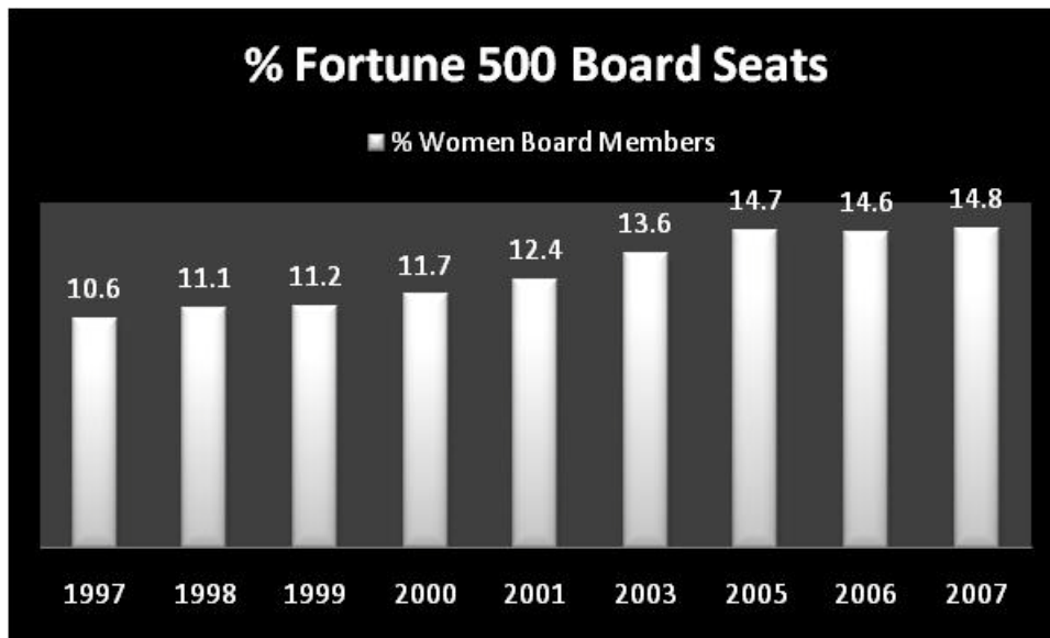
FIGURE 2C Catalyst, 2008 http://www.catalyst.org/publication/206/women-in-us-management
