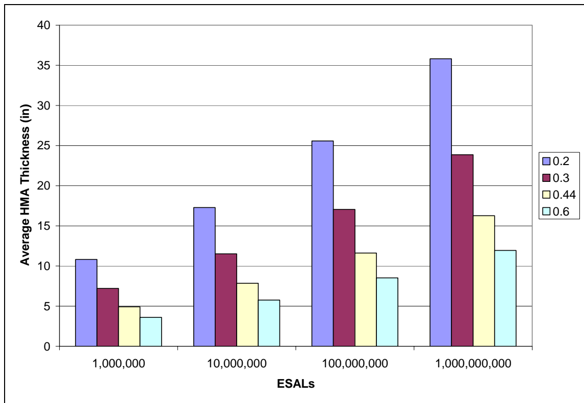
Figure 3. 7 Resulting HMA Thickness from Changing Layer Coefficient ( a_1 ).
