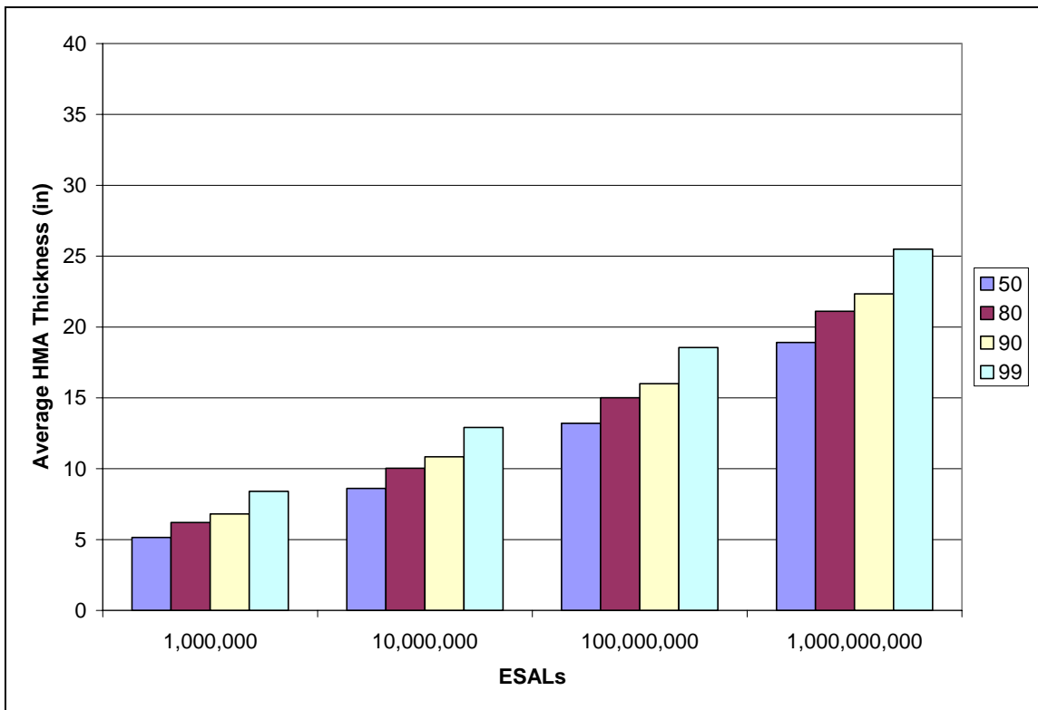
Figure 3. 9 Resulting HMA Thickness from Changing Reliability ( R ).
