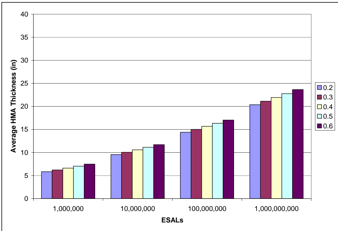
Figure 3. 11 Resulting HMA Thickness from Changing Variability ( S_0 ).
