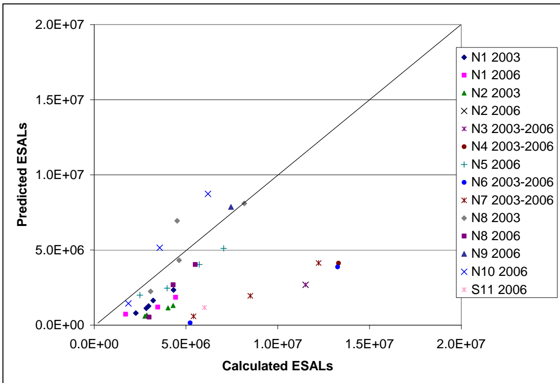
Figure 4.16 Calculated vs. Predicted ESALs Using a_1 = 0.44 .
