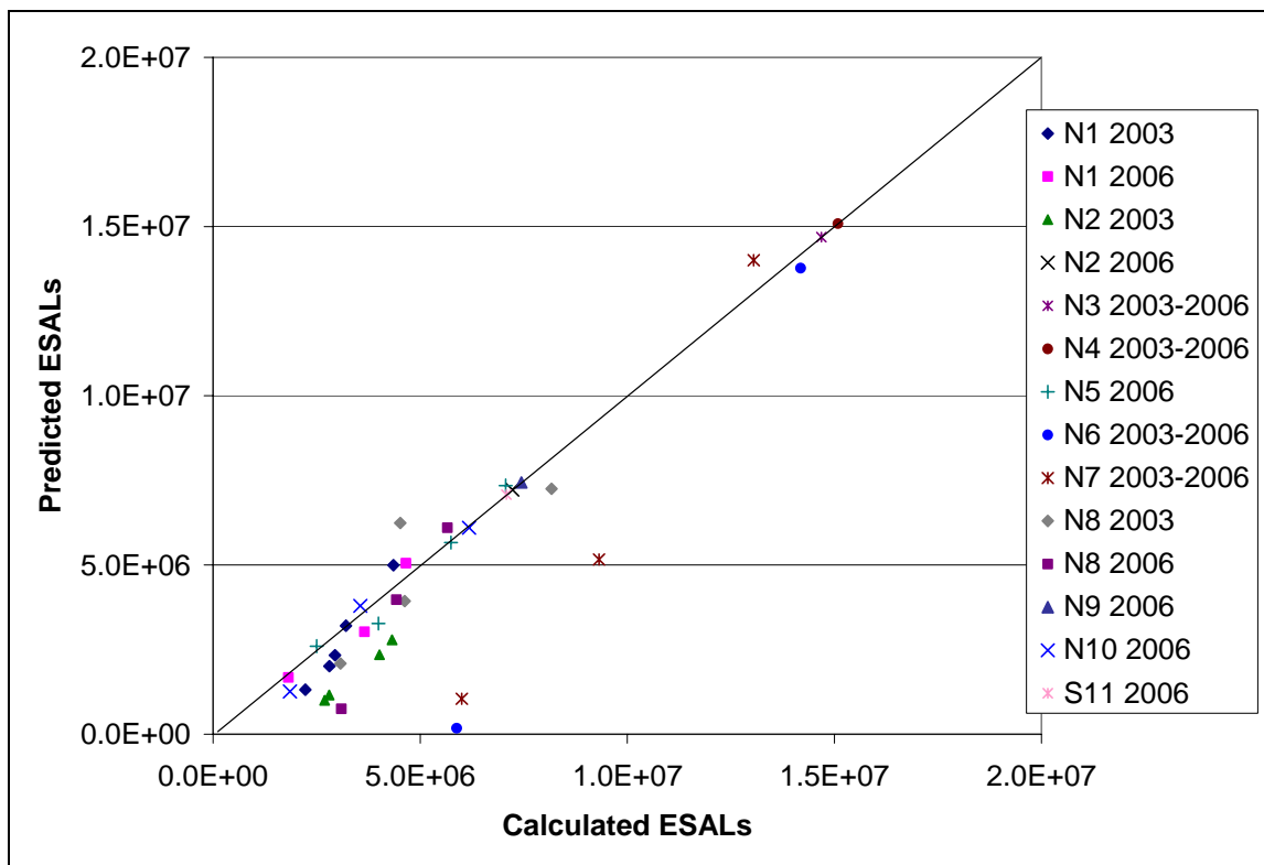
Figure 4. 11 Calculated vs. Predicted ESALs.
