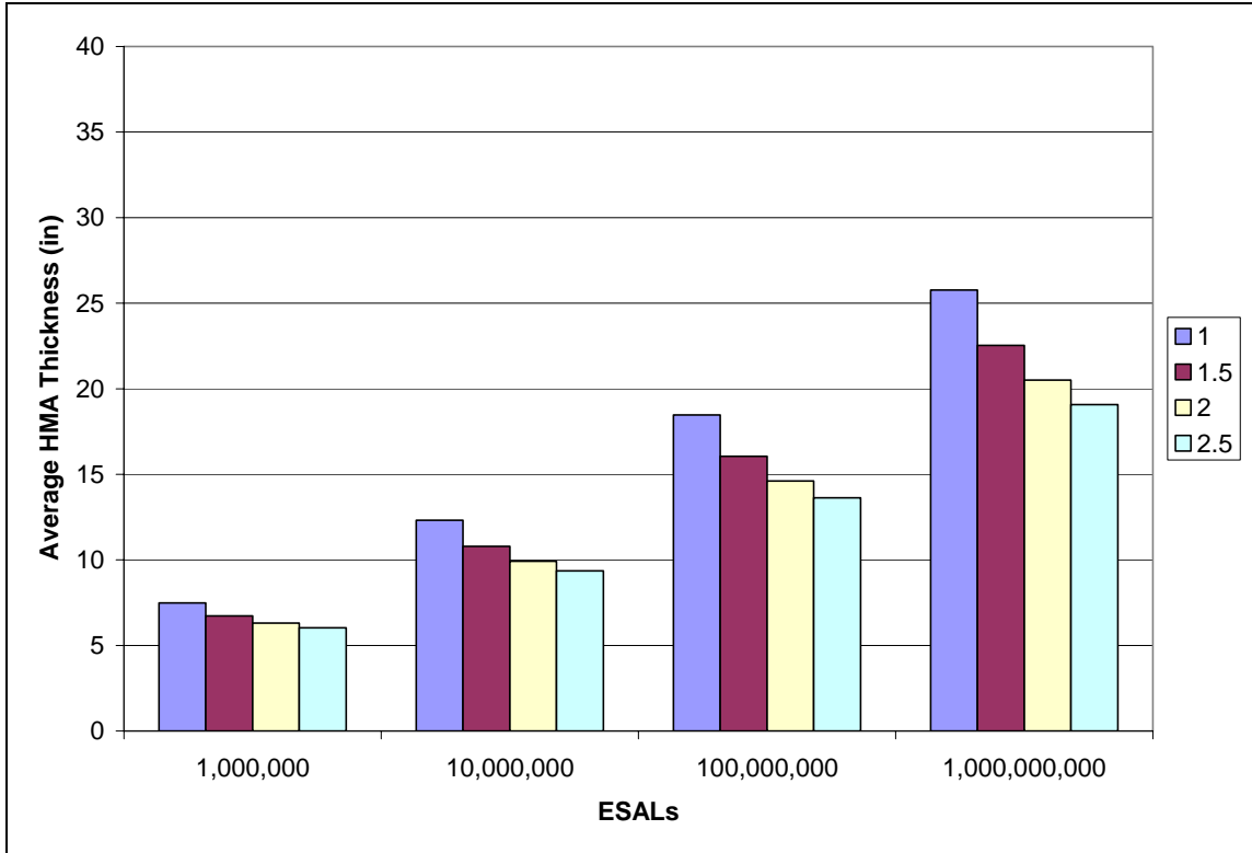
Figure 3. 10 Resulting HMA Thickness from Changing Serviceability ( \Delta PSI).
