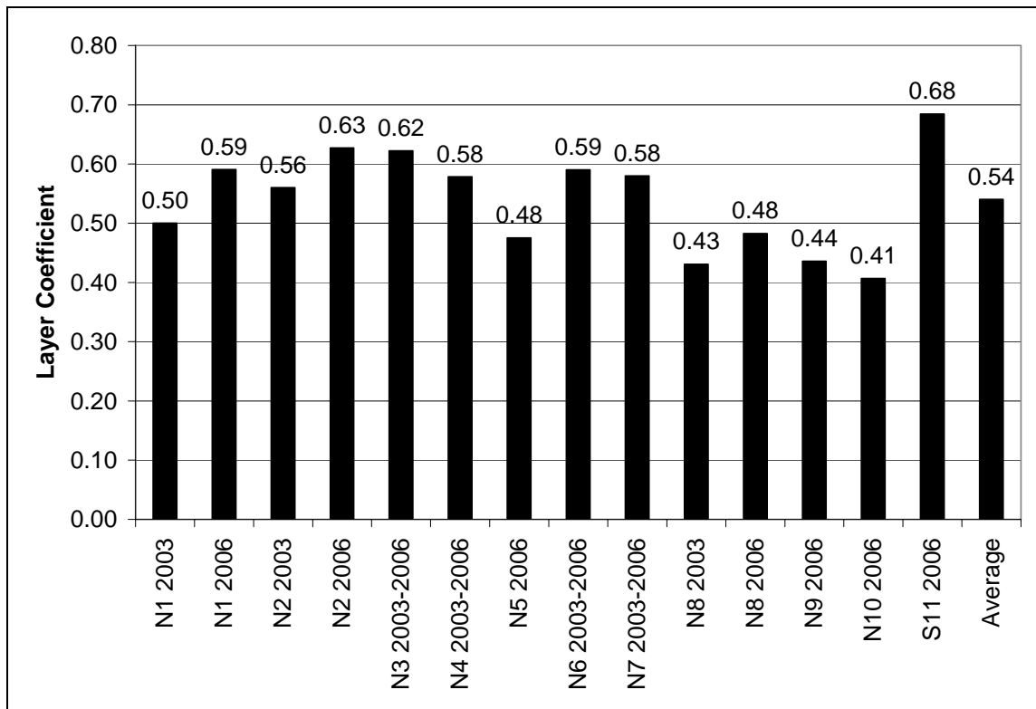
Figure 4. 12 Regressed Layer Coefficients.
