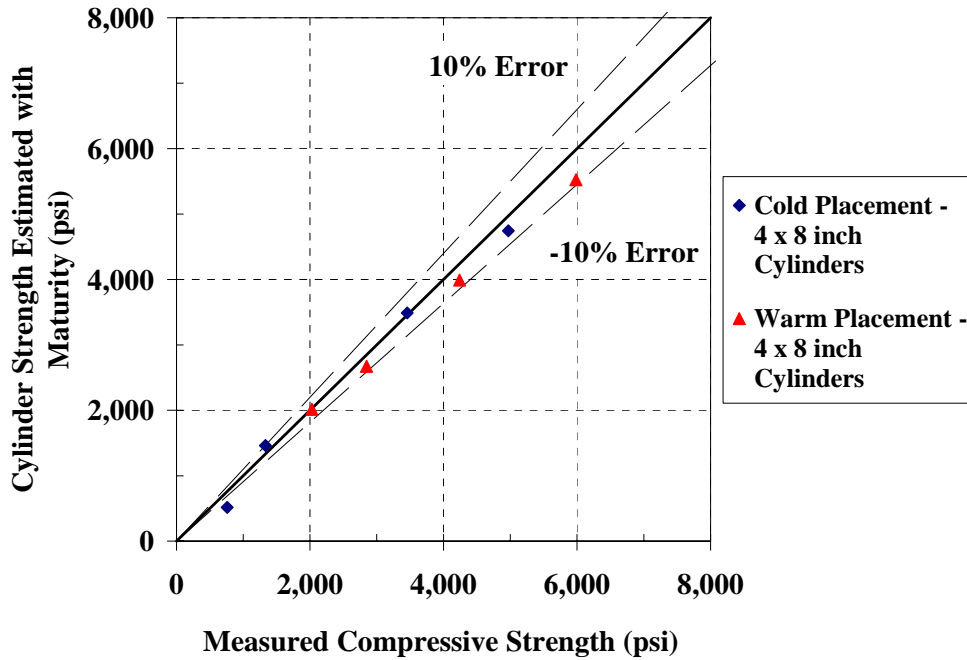
Figure C-77: 45°-line graph for estimating the strength of water-tank-cured 4 x 8 inch cylinder from the mock bridge deck water-tank S-M relationships using the Arrhenius maturity function ( E = 40 \text{ kJ/mol} )
