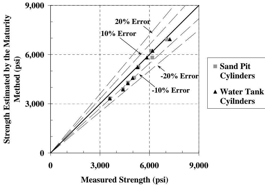
Figure 4-44: 45°-line graph for estimated cylinder strengths from the laboratory S-M relationship using the Nurse-Saul maturity function ( T_o = 0\text{ }^\circ\text{C} )
