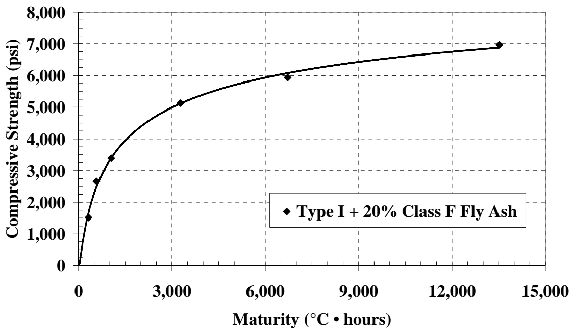
Figure 2-18: Example of a strength-maturity relationship using Nurse-Saul maturity function with T_0 = 0 °C
