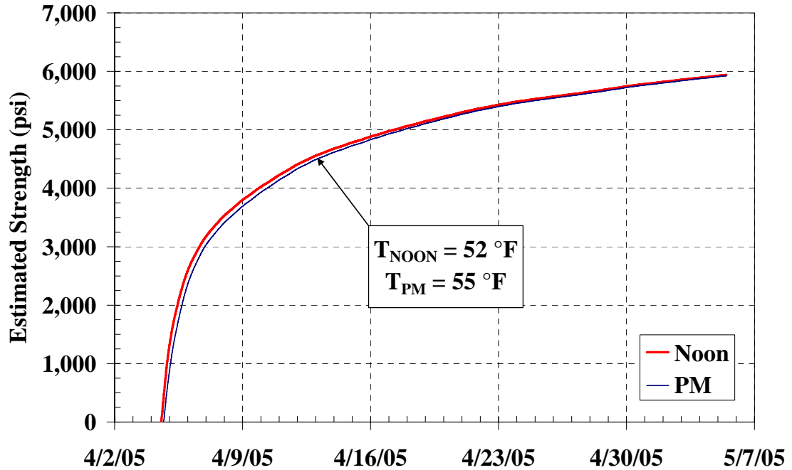
Figure 5-92: Creek Bridge deck strength development using Nurse-Saul maturity function with T_o = -10\text{ }^{\circ}\text{C}
