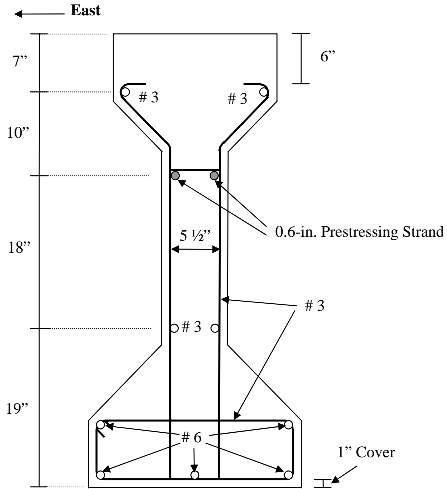
Figure 4-3: Cross-sectional reinforcement configuration for mock girder
