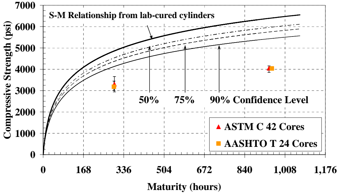
Figure C-48: Cores with laboratory S-M relationship and confidence levels for the warm-weather placement of the mock bridge deck ( E = 40 \text{ kJ/mol} )
