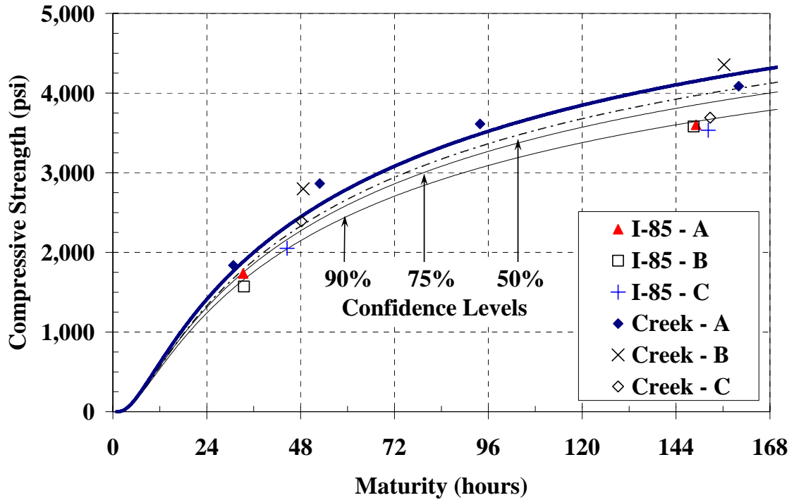
Figure 5-87: I-85 Bridge S-M relationship with confidence levels and verification test results ( E = 40 \text{ kJ/mol} )
