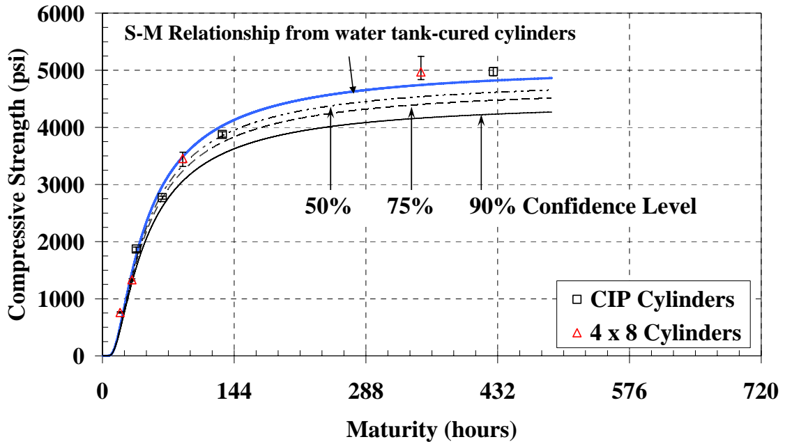
Figure C-21: Cast-in-place cylinders and 4 x 8 inch cylinders with water-tank S-M relationship and confidence levels for the cold-weather placement of mock bridge deck ( E = 40 \text{ kJ/mol} )
