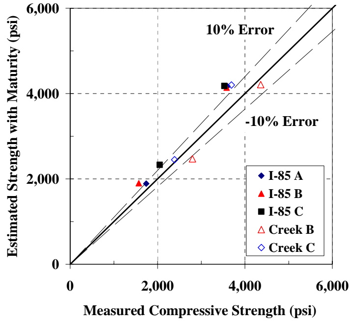
Figure C-93: 45°-line graph for estimating the strength of the verification cylinders using I-85 Bridge S-M relationship with Arrhenius maturity function ( E = 40 kJ/mol)
