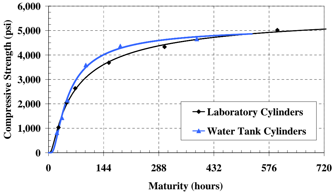
Figure 5-28: S-M relationships using the Arrhenius maturity function for mock bridge deck cold-weather placement ( E = 33.5\text{ kJ/mol} )
