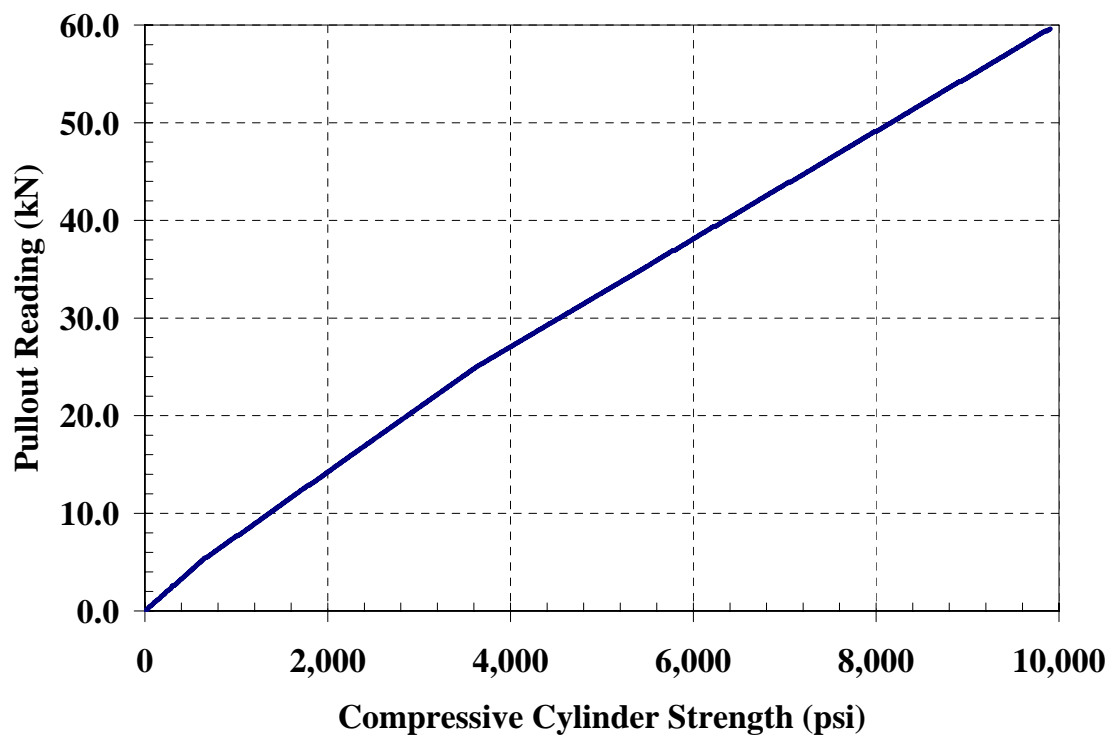
Figure A-1: Pullout reading versus compressive strength of cylinders
