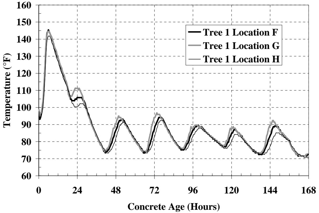
Figure B-6: Girder temperatures Tree 1 Location F, G, and H
