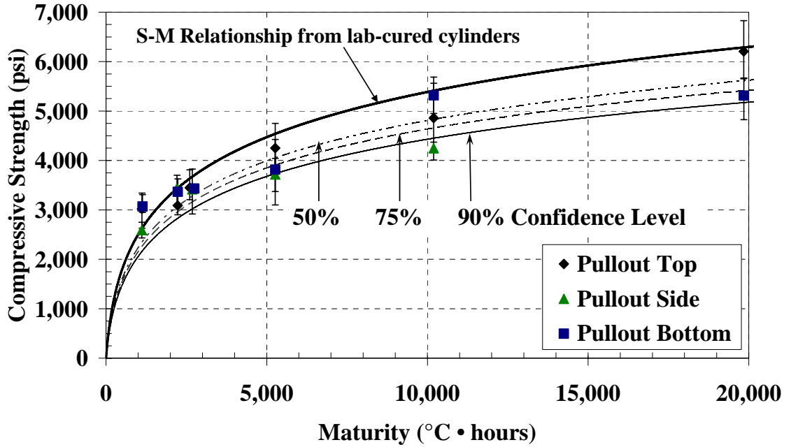
Figure 5-59: Pullout test with laboratory S-M relationship and confidence levels for the warm-weather placement of the mock bridge deck ( T_0 = 0^{\circ}\text{C} )
