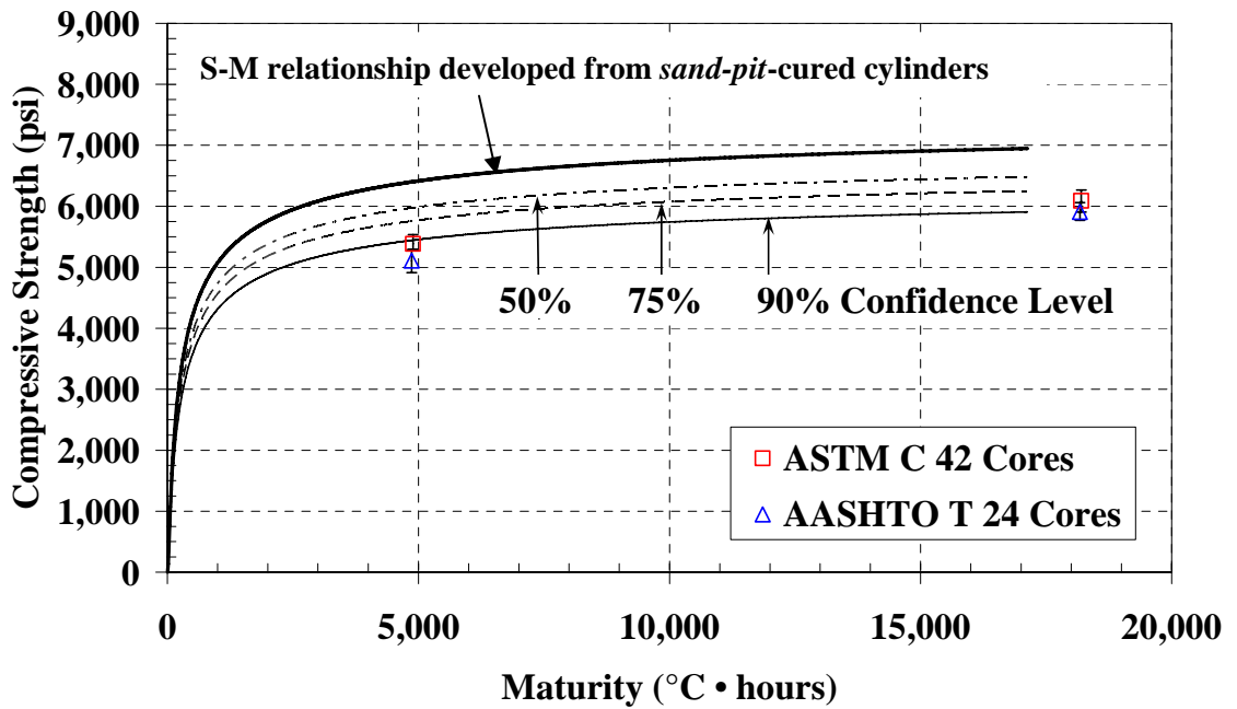
Figure B-41: Cores with sand-pit S-M relationship and confidence levels ( T_0 = 0^\circ\text{C} ).
