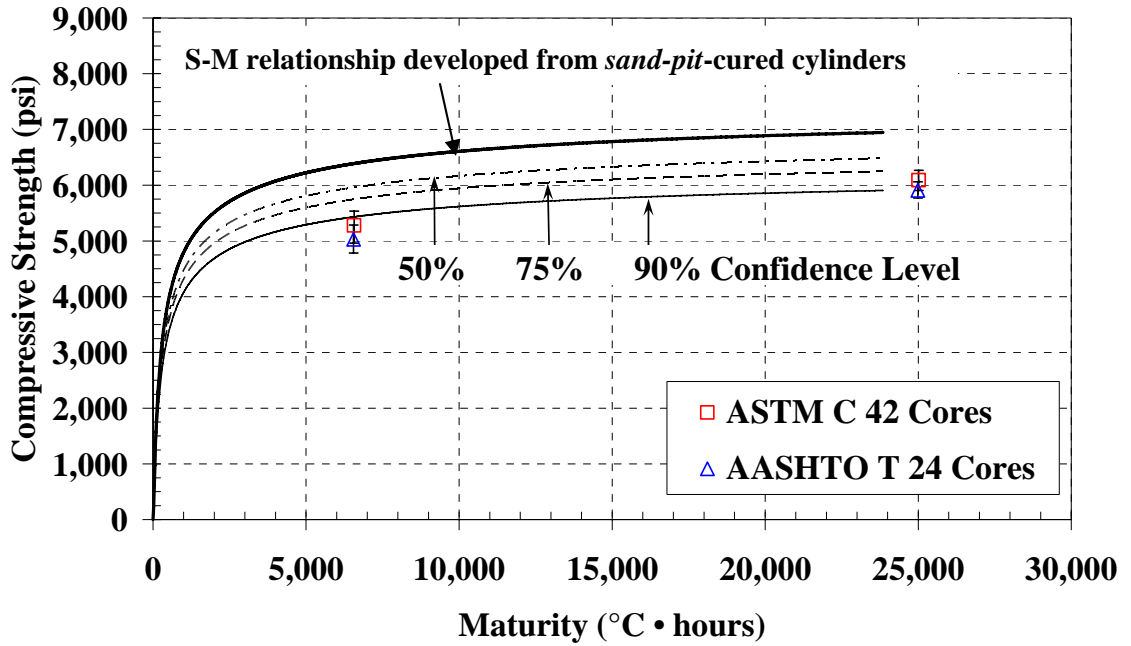
Figure B-40: Cores with sand pit S-M relationship and confidence levels ( T_0 = -10^\circ\text{C} )
