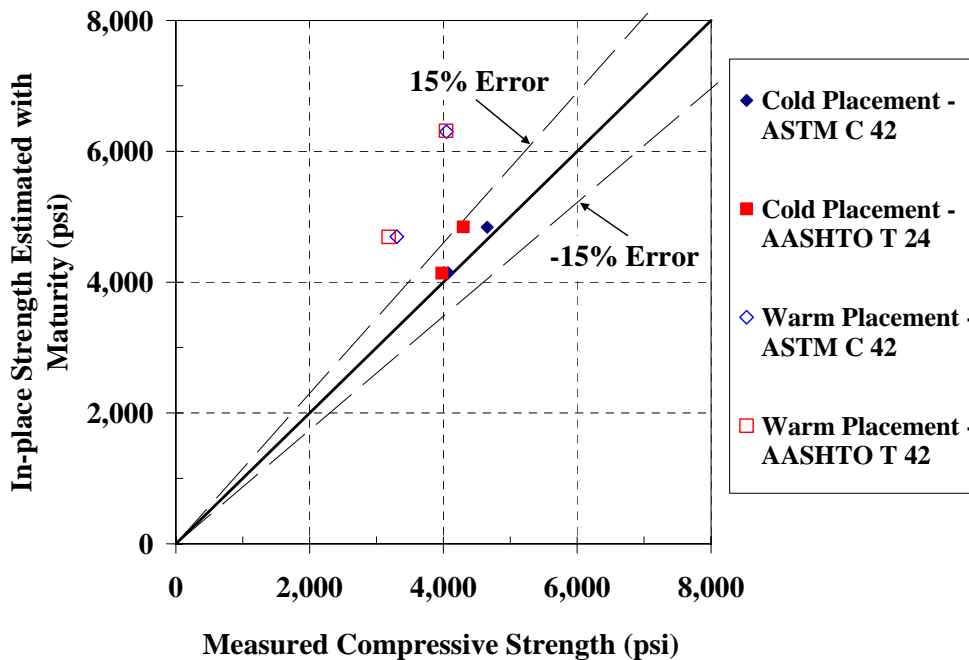
Figure 5-114: 45°-line graph for estimating the strength of cores for the mock bridge deck using laboratory S-M relationship with Nurse-Saul maturity function ( T_0 = 0\text{ }^\circ\text{C} )
