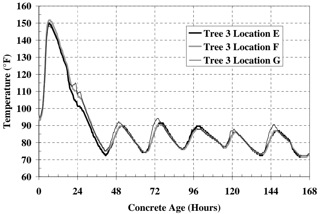
Figure B-11: Girder temperatures Tree 3 Location E, F, and G
