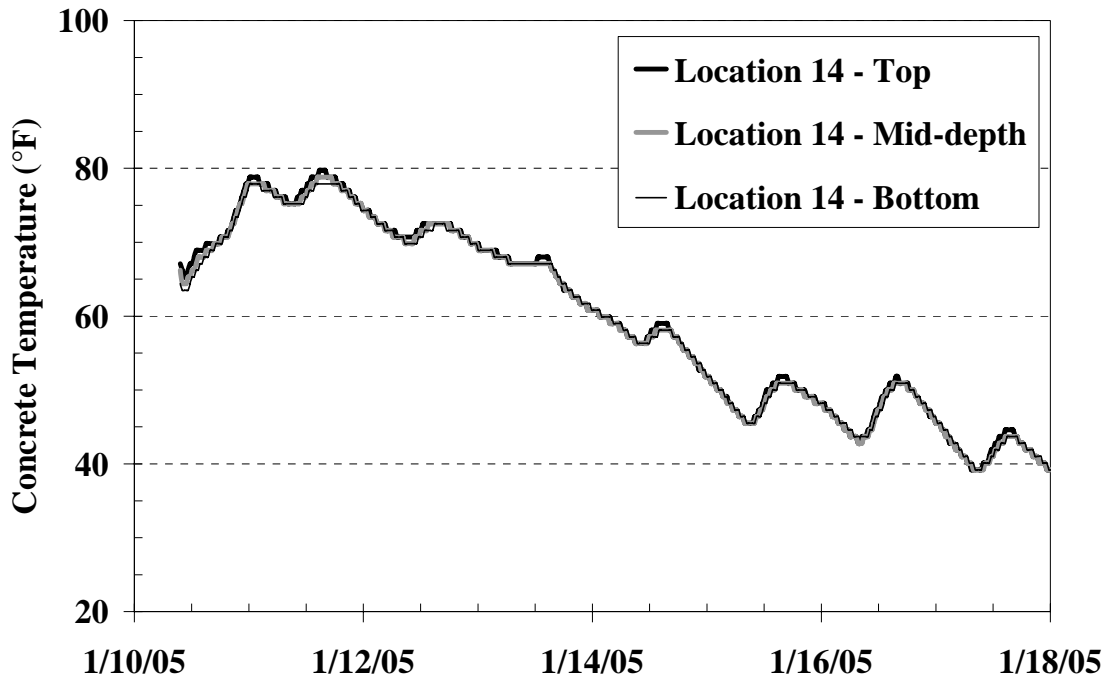
Figure C-66: Temperature history of Location 14 from the I-85 Bridge
