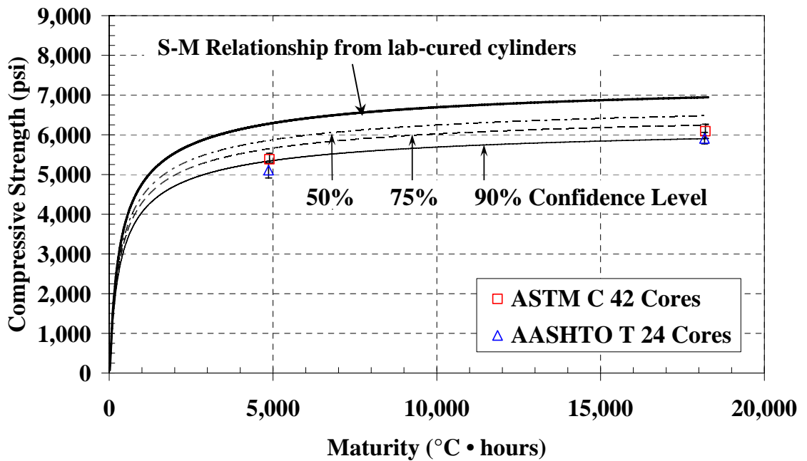
Figure 4-40: Cores with laboratory S-M relationship and confidence levels ( T_o = 0 \text{ }^{\circ}\text{C} )
