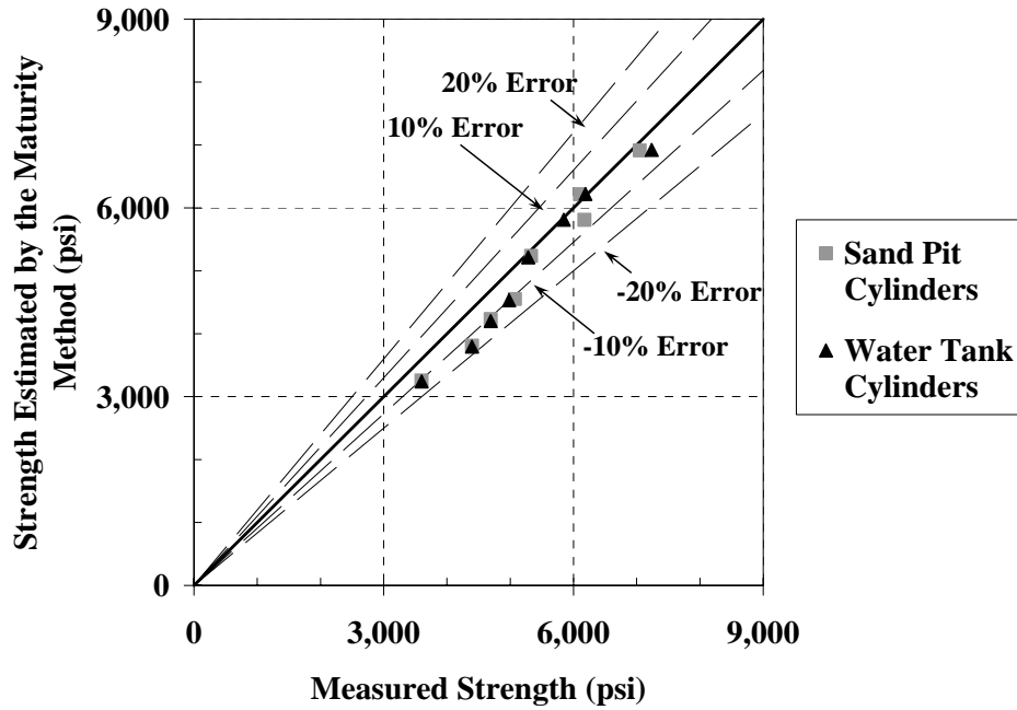
Figure 4-43: 45°-line graph for estimated cylinder strengths from the laboratory S-M relationship using the Nurse-Saul maturity function ( T_o = -10\text{ }^\circ\text{C} )
