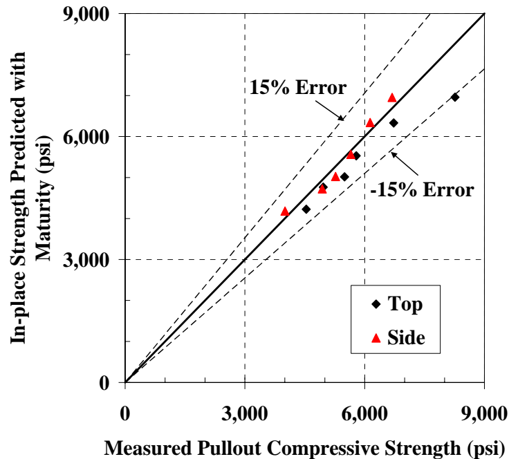
Figure 4-49: 45°-line graph for estimating the strength of pullout test on the mock girder using laboratory S-M relationship with Nurse-Saul maturity function (T o = 0 °C)
