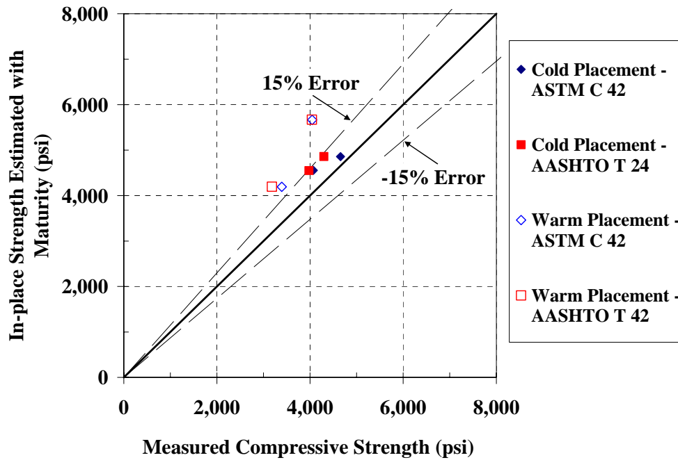
Figure 5-116: 45°-line graph for estimating the strength of cores for the mock bridge deck using water-tank S-M relationship with Nurse-Saul maturity function ( T_0 = 0\text{ }^{\circ}\text{C} )
