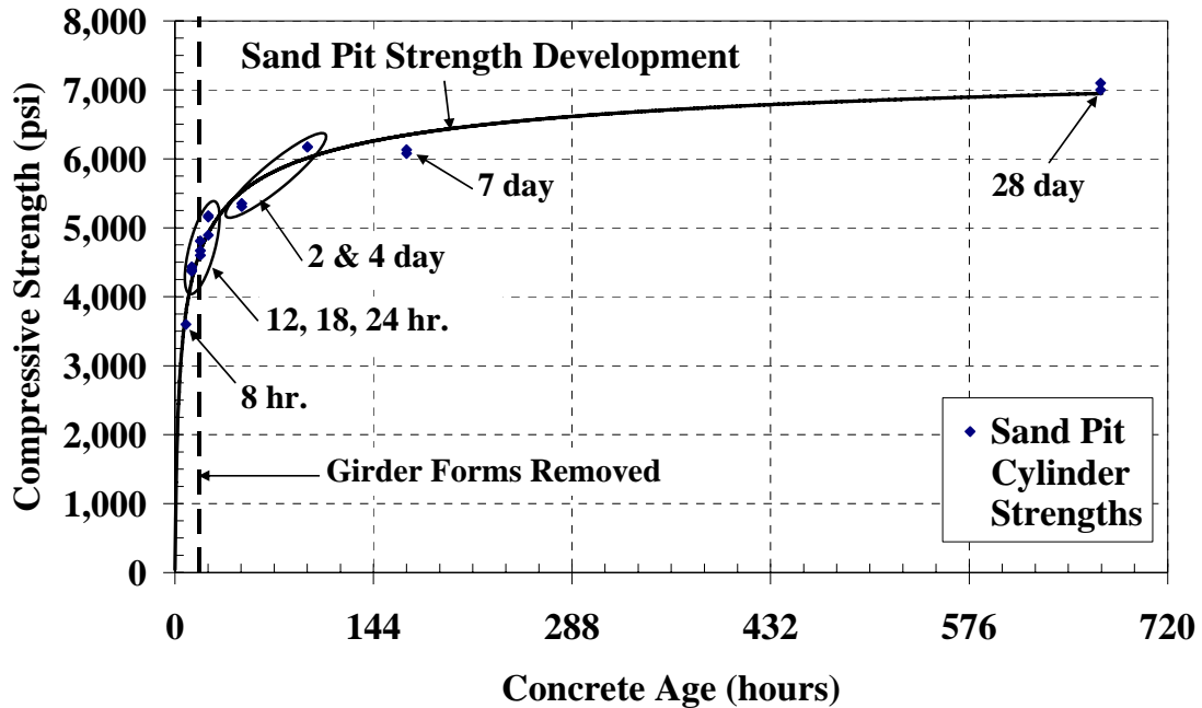
Figure 4-62: Evaluation of the testing ages for the prestressed girder project
