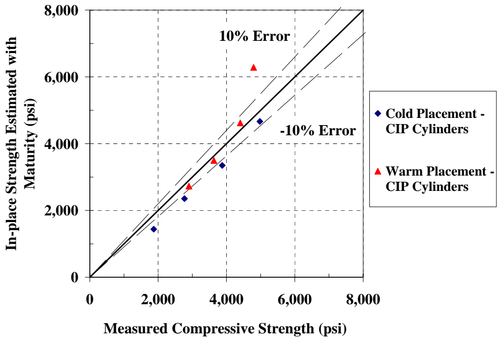
Figure 5-110: 45°-line graph for estimating the strength of CIP cylinders on the mock bridge deck using Laboratory S-M relationship with Nurse-Saul maturity function ( T_0 = 0\text{ }^\circ\text{C} )
