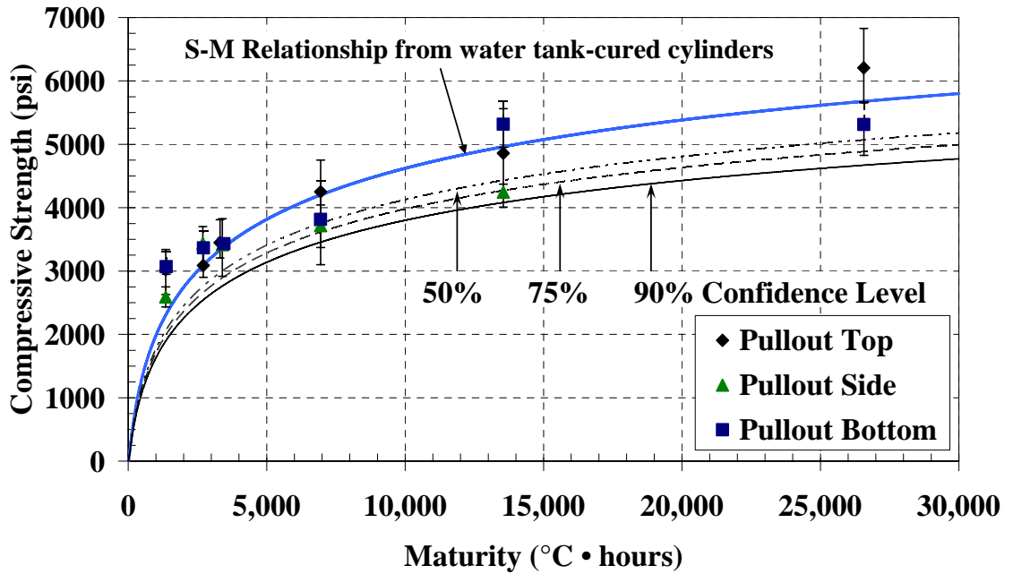
Figure C-41: Pullout test with water-tank S-M relationship and confidence levels for the warm-weather placement of mock bridge deck ( T_o = -10^\circ\text{C} )
