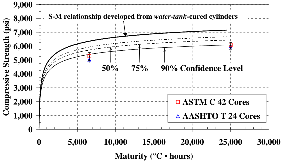
Figure B-36: Cores with water-tank S-M relationship and confidence levels ( T_0 = -10^\circ\text{C} )
