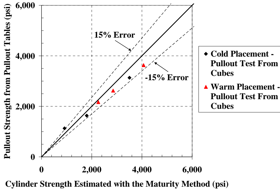
Figure 5-104: 45°-line graph to evaluate the pullout table using estimated strength from water-tank S-M relationship using the Nurse-Saul maturity function ( T_0 = 0\text{ }^{\circ}\text{C} )
