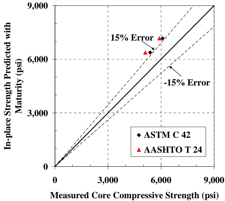
Figure 4-57: 45°-line graph for estimating the strength of cores for the mock girder using water-tank S-M relationship with Nurse-Saul maturity function ( T_o = 0\text{ }^\circ\text{C} )
