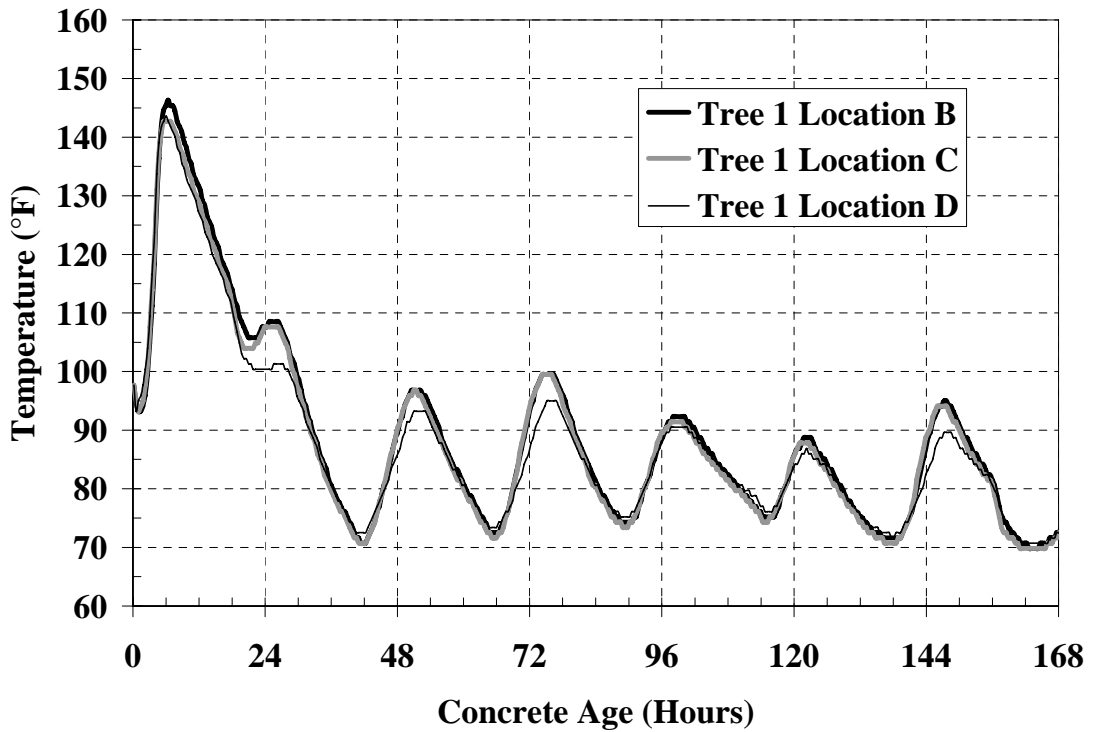
Figure B-5: Girder temperatures Tree 1 Location B, C, and D
