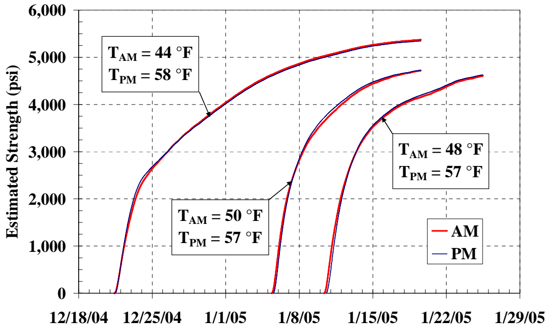
Figure 5-88: I-85 Bridge deck strength development using Nurse-Saul maturity function with T_o = -10\text{ }^\circ\text{C}
