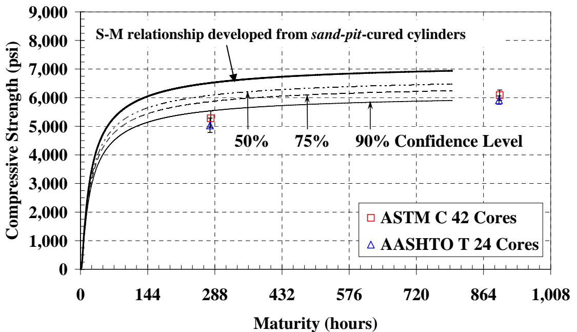
Figure B-43: Cores with sand-pit S-M relationship and confidence levels ( E = 40 kJ/mol)
