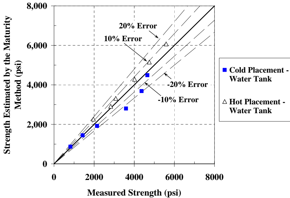
Figure 5-96: 45°-line graph for estimated cylinder strengths from the laboratory S-M relationship using the Nurse-Saul maturity function ( T_0 = -10\text{ }^\circ\text{C} )
