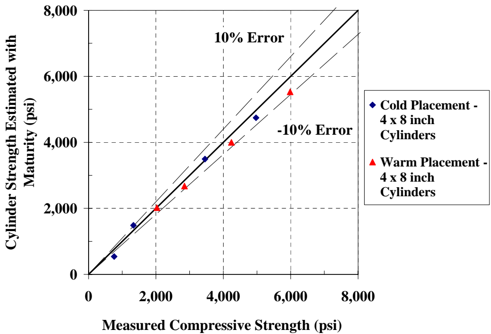
Figure 5-102: 45°-line graph for estimating the strength of water-tank-cured 4 x 8 inch cylinder from the mock bridge deck water-tank S-M relationships using the Nurse-Saul maturity function ( T_0 = 0\text{ }^{\circ}\text{C} )
