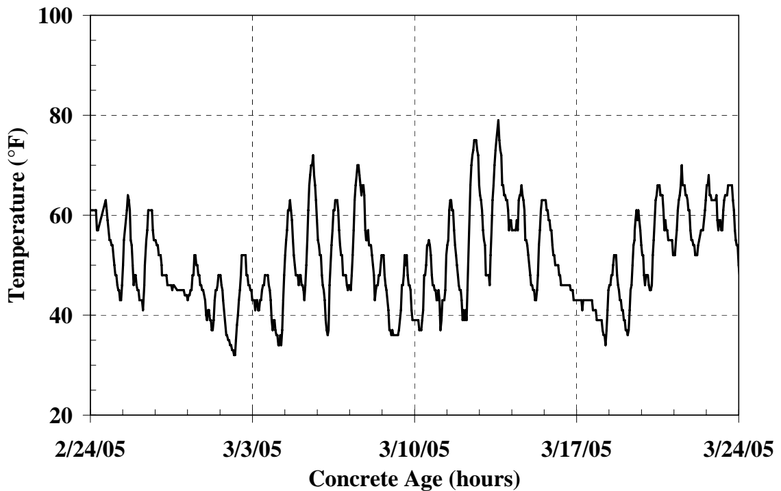
Figure C-2: Ambient temperatures of the cold-weather placement of mock bridge deck
