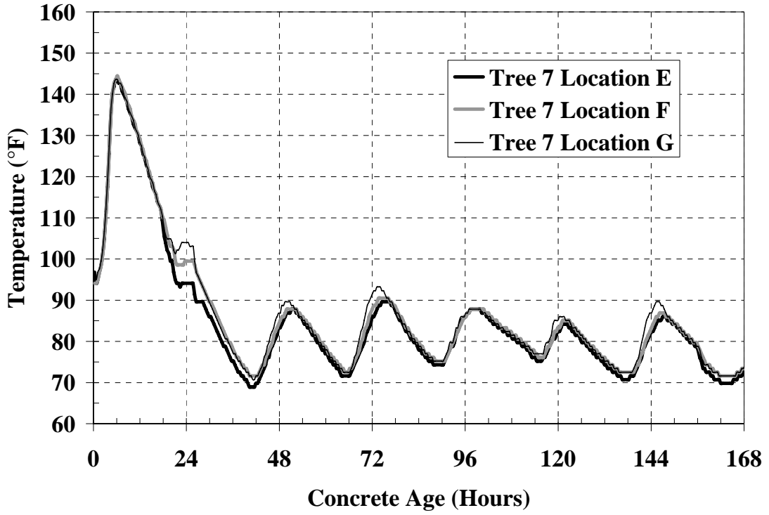
Figure B-18: Girder temperatures Tree 7 Location E, F, and G
