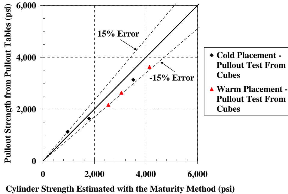
Figure C-79: 45°-line graph to evaluate the pullout table using estimated strength from water-tank S-M relationship using the Arrhenius maturity function ( E = 40 \text{ kJ/mol} )
