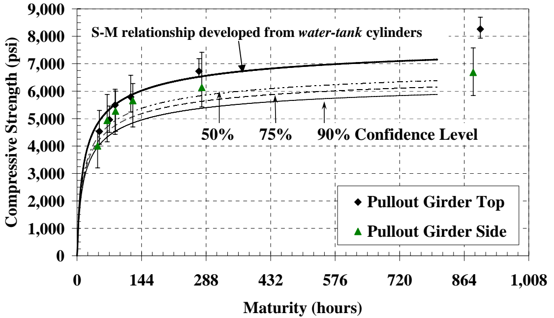
Figure B-30: Pullout test with water-tank S-M relationship and confidence levels (E = 33.5 kJ/mol)
