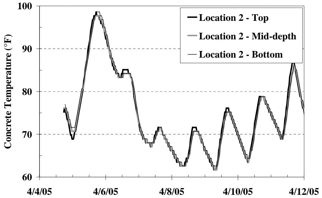
Figure C-70: Temperature history of Location 2 from the Creek Bridge
