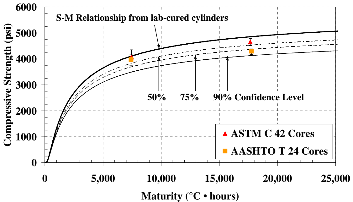
Figure C-22: Cores with laboratory S-M relationship and confidence levels for the cold-weather placement of the mock bridge deck ( T_0 = -10 \text{ }^{\circ}\text{C} )
