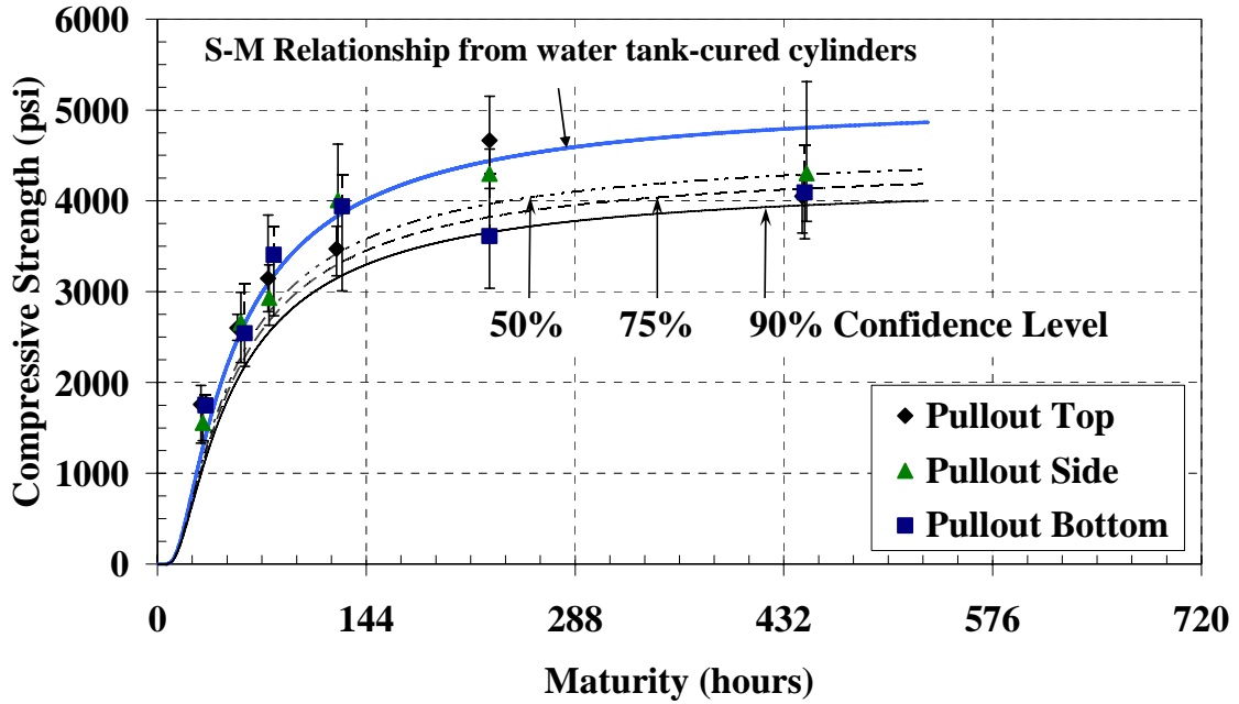
Figure 5-37: Pullout test with water-tank S-M relationship and confidence levels for the cold-weather placement of mock bridge deck ( E = 33.5 kJ/mol)
