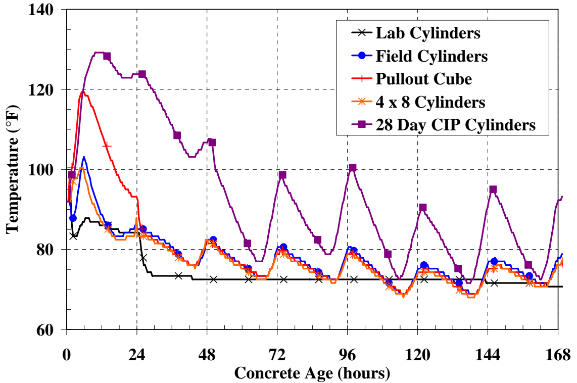
Figure C-28: Molded cylinder temperature history for warm-weather placement of mock bridge deck
