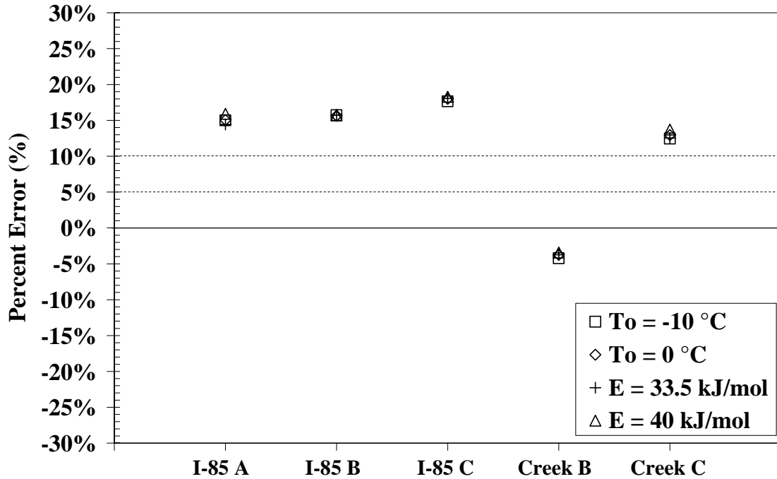
Figure 5-127: 7-day verification test percent errors for the best-fit I-85 Bridge S-M relationship
