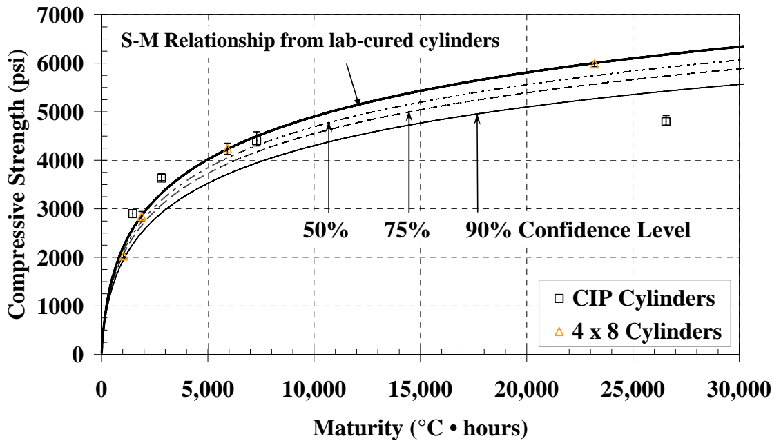
Figure C-43: Cast-in-place cylinders and 4x 8 inch cylinders with laboratory S-M relationship and confidence levels for the warm-weather placement of the mock bridge deck ( T_0 = -10 \text{ }^{\circ}\text{C} )
