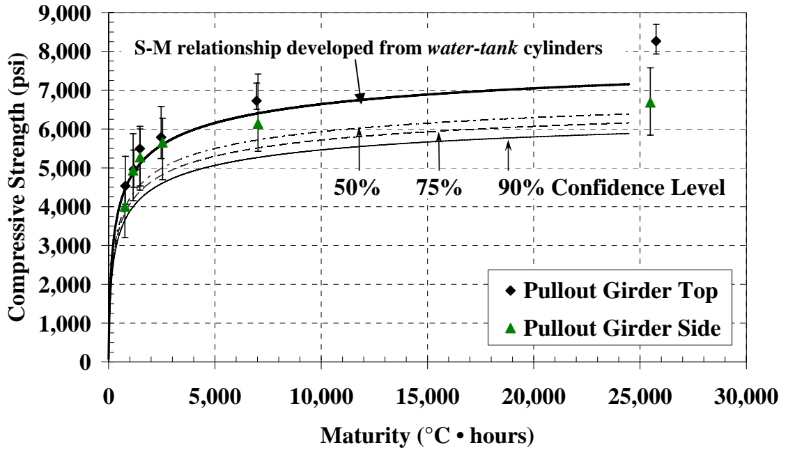
Figure B-28: Pullout test with water-tank S-M relationship and confidence levels ( T_o = -10^{\circ}\text{C} )
