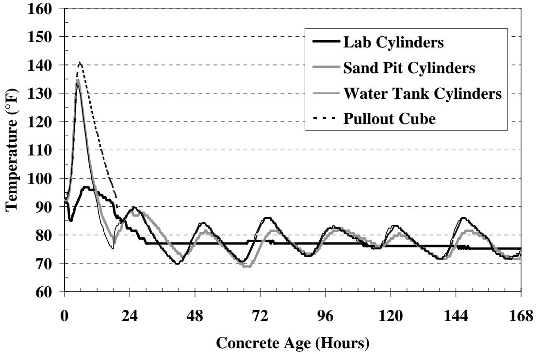
Figure B-4: Molded cylinder temperature history
