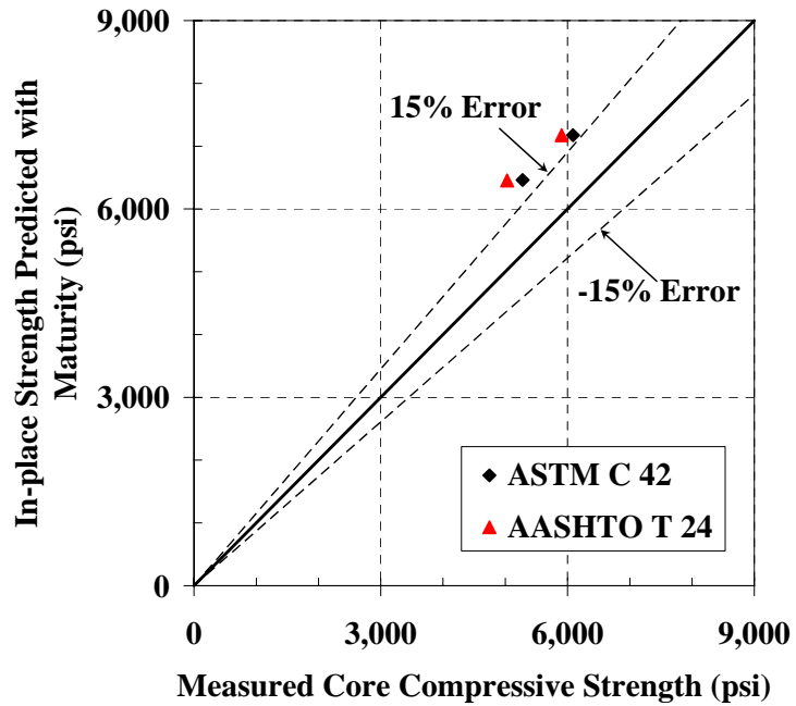
Figure B-55: 45°-line graph for estimating the strength of cores for the mock girder using water-tank S-M relationship with Arrhenius maturity function ( E = 33.5\text{ kJ/mol} )
