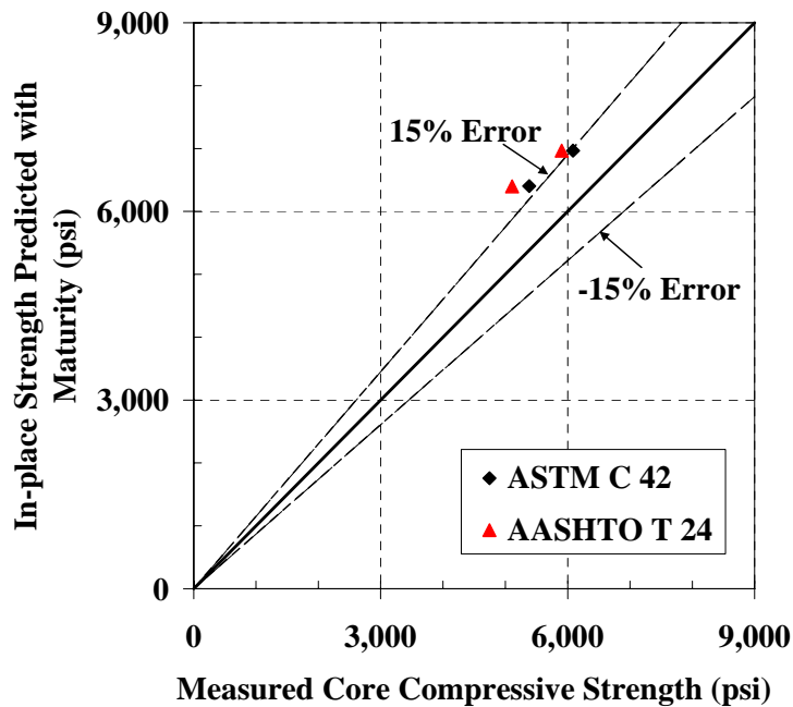
Figure 4-59: 45°-line graph for estimating the strength of cores for the mock girder using sand-pit S-M relationship with Nurse-Saul maturity function ( T_0 = 0 °C)
