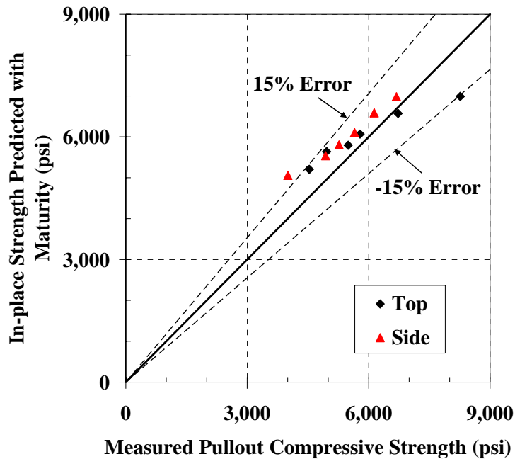
Figure 4-54: 45°-line graph for estimating the strength of pullout test on the mock girder using sand-pit S-M relationship with Arrhenius maturity function ( E = 40 kJ/mol)
