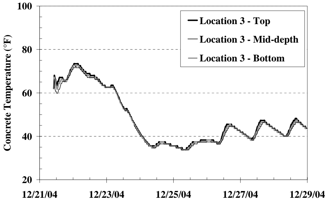
Figure C-54: Temperature history of Location 3 from the I-85 Bridge
