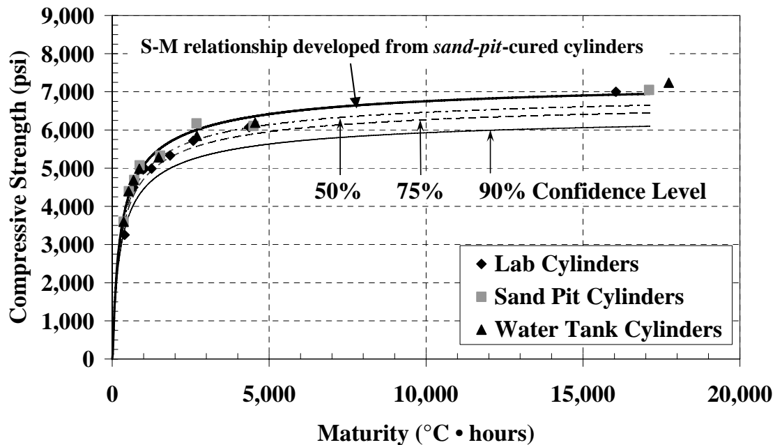
Figure B-25: Sand-pit S-M relationship with confidence levels ( T_0 = 0\text{ }^\circ\text{C} )
