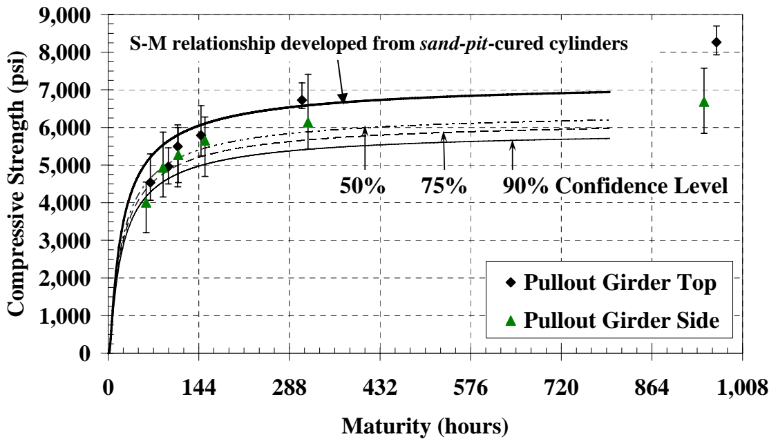
Figure B-35: Pullout test with sand-pit S-M relationship and confidence levels (E = 40 kJ/mol)
