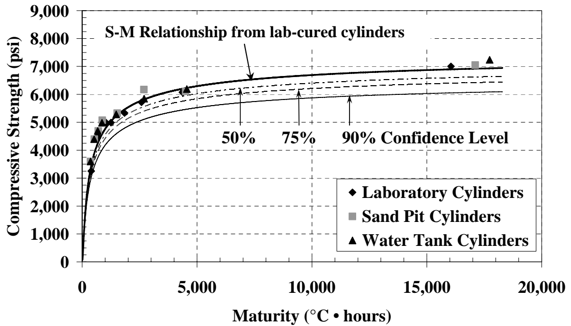
Figure 4-32: Laboratory S-M relationship with confidence levels ( T_0 = 0\text{ }^\circ\text{C} )
