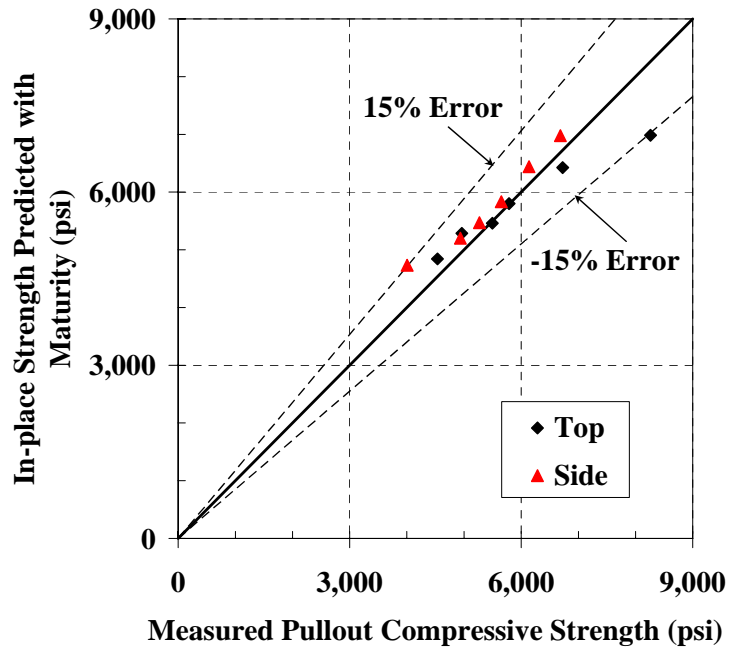
Figure B-47: 45°-line graph for estimating the strength of pullout test on the mock girder using laboratory S-M relationship with Arrhenius maturity function ( E = 33.5\text{ kJ/mol} )
