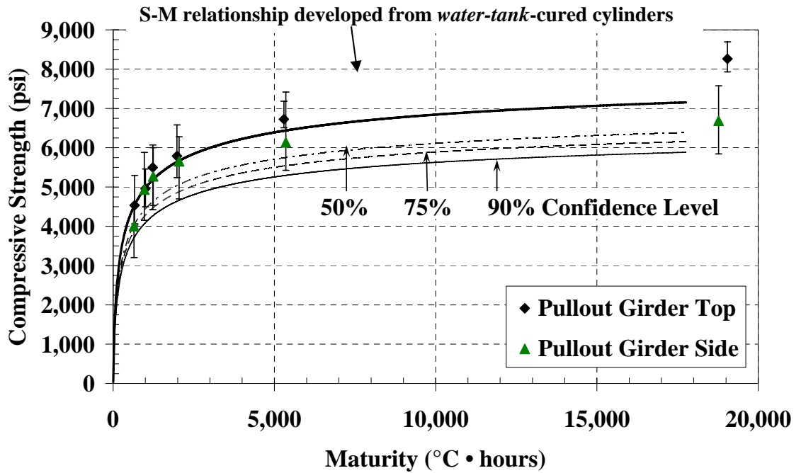
Figure B-29: Pullout test with water-tank S-M relationship and confidence levels ( T_o = 0^{\circ}\text{C} )
