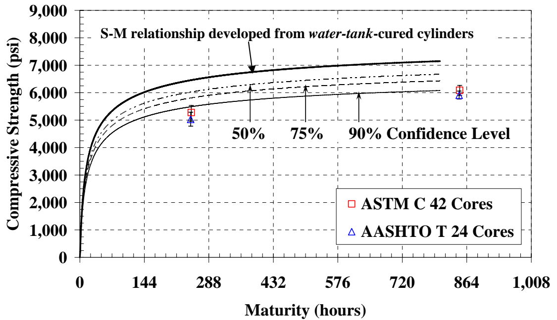
Figure B-38: Cores with water-tank S-M relationship and confidence levels ( E = 33.5 kJ/mol)
