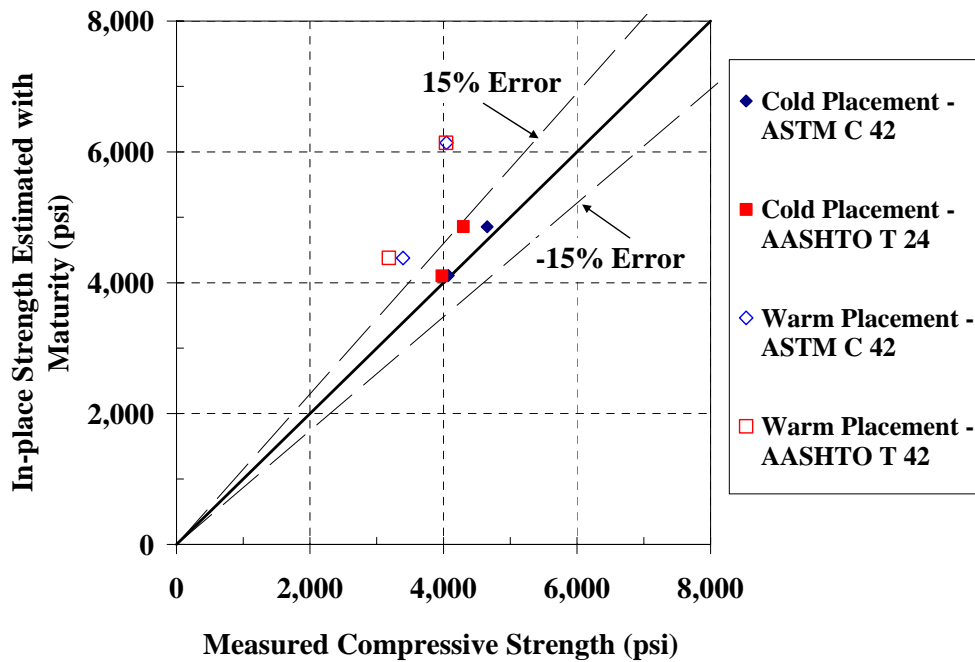
Figure C-88: 45°-line graph for estimating the strength of cores for the mock bridge deck using laboratory S-M relationship with Nurse-Saul maturity function ( T_0 = -10 \text{ }^\circ\text{C} )
