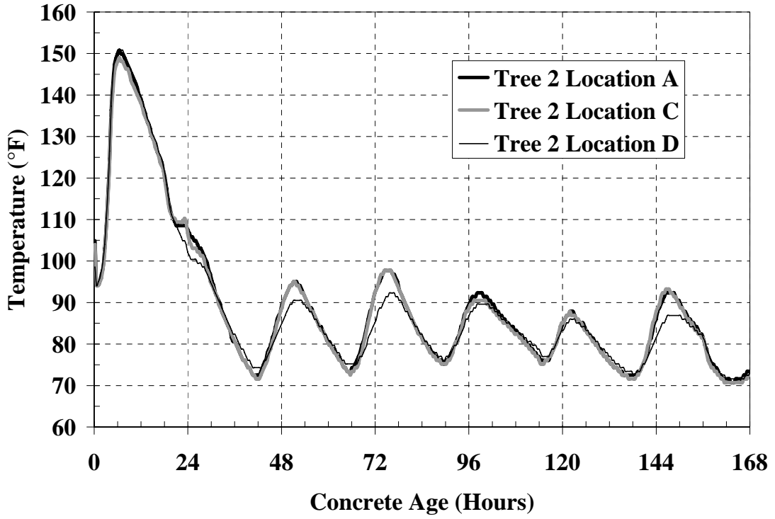
Figure B-8: Girder temperatures Tree 2 Location A, C, and D
