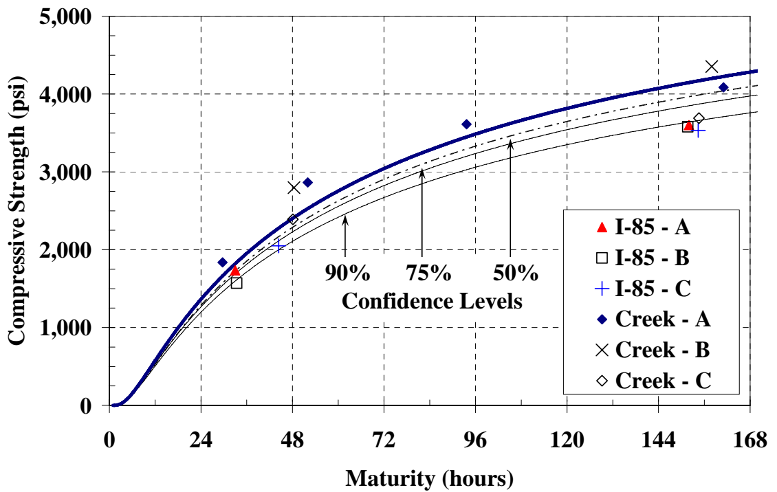
Figure 5-86: I-85 Bridge S-M relationship with confidence levels and verification test results ( E = 33.5 \text{ kJ/mol} )
