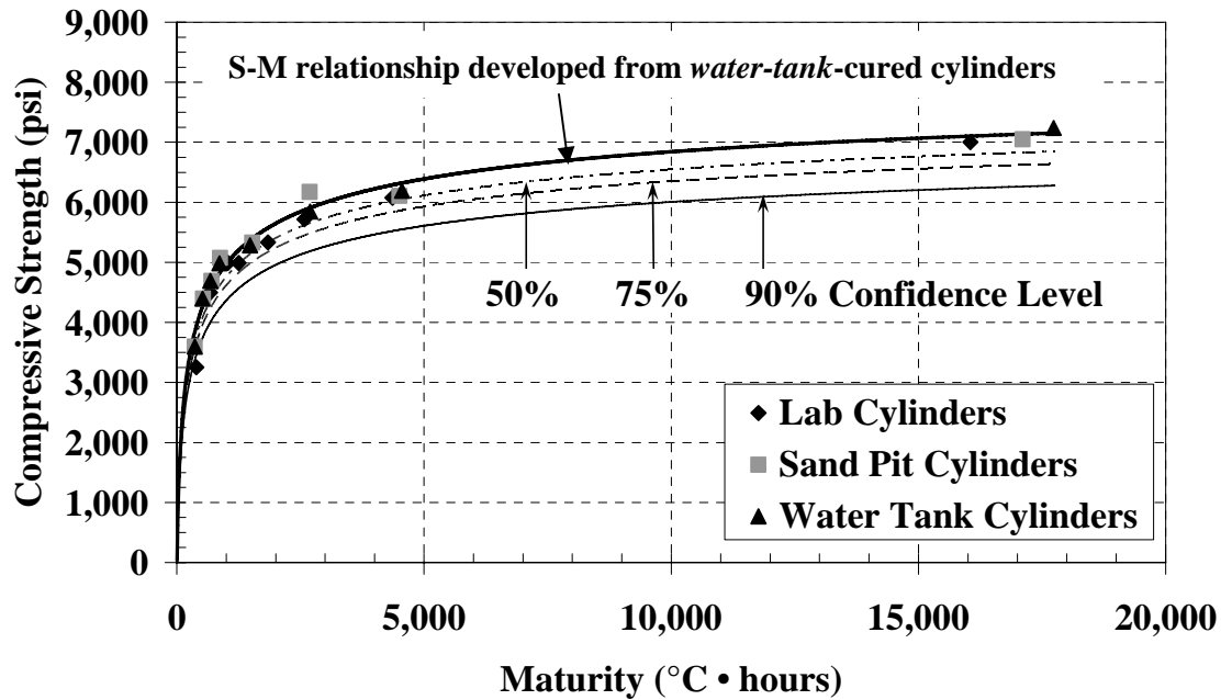
Figure B-21: Water-tank S-M relationship with confidence levels ( T_0 = 0\text{ }^\circ\text{C} )
