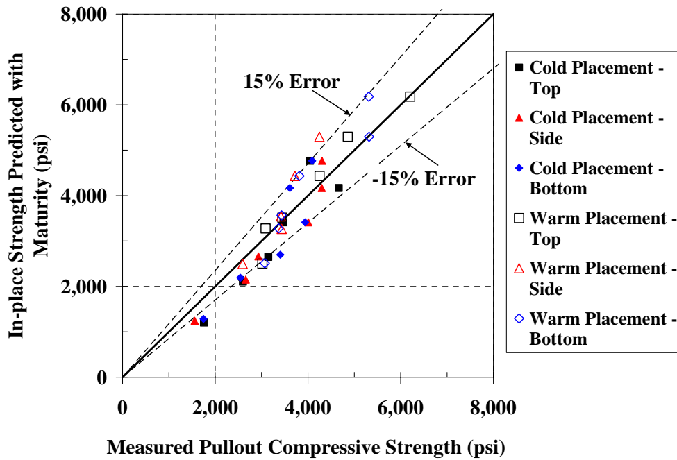
Figure C-80: 45°-line graph for estimating the strength of pullout test on the mock bridge deck using laboratory S-M relationship with Nurse-Saul maturity function ( T_0 = -10 \text{ }^\circ\text{C} )
