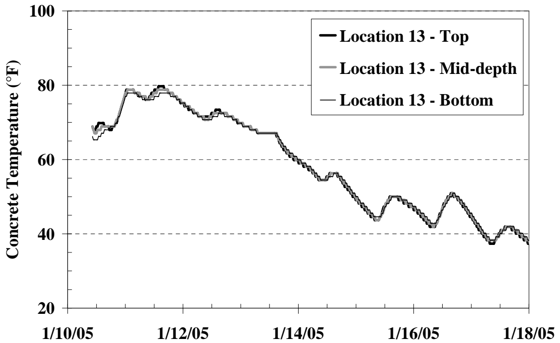
Figure C-65: Temperature history of Location 13 from the I-85 Bridge
