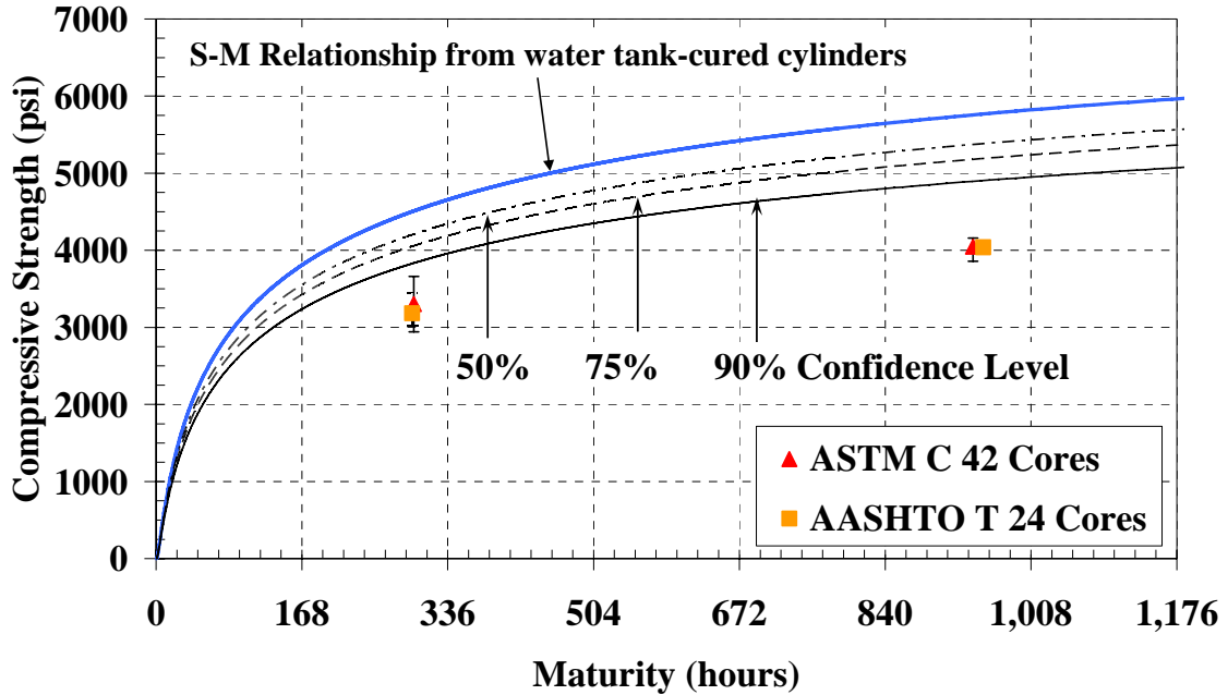
Figure C-50: Cores with water-tank S-M relationship and confidence levels for the warm-weather placement of mock bridge deck ( E = 40 kJ/mol)
