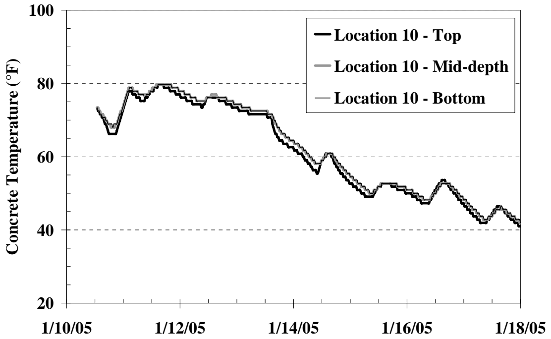
Figure C-62: Temperature history of Location 10 from the I-85 Bridge
