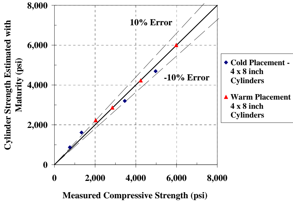
Figure C-74: 45°-line graph for estimating the strength of water-tank-cured 4 x 8 inch cylinder from the mock bridge deck laboratory S-M relationships using the Nurse-Saul maturity function ( T_o = -10\text{ }^\circ\text{C} )
