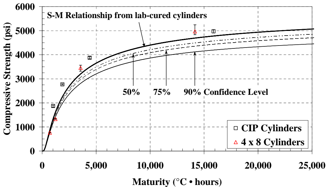
Figure C-18: Cast-in-place cylinders and 4x 8 inch cylinders with laboratory S-M relationship and confidence levels for the cold-weather placement of the mock bridge deck ( T_0 = -10 \text{ }^{\circ}\text{C} )
