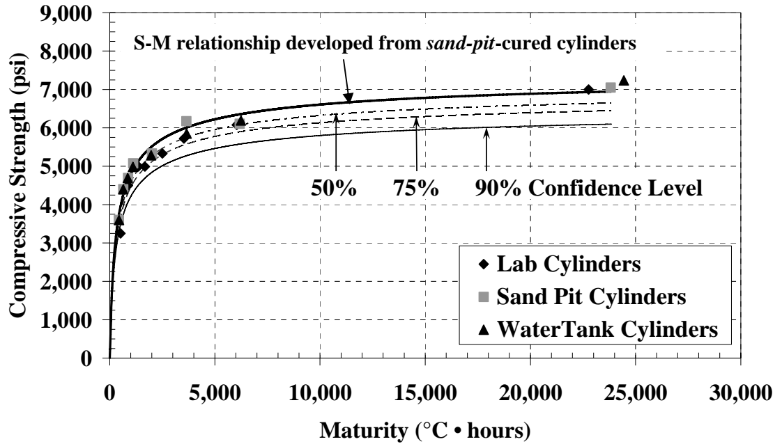
Figure B-24: Sand-pit S-M relationship with confidence levels ( T_0 = -10\text{ }^\circ\text{C} )
