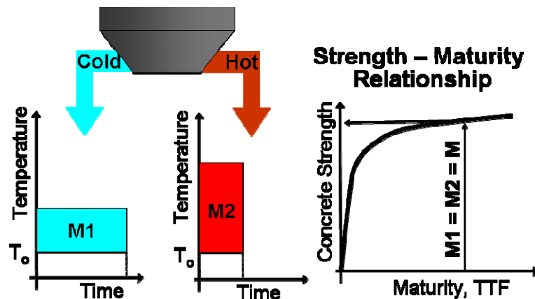
Figure 2-1: Diagram showing the effect of temperature histories on maturity calculation
