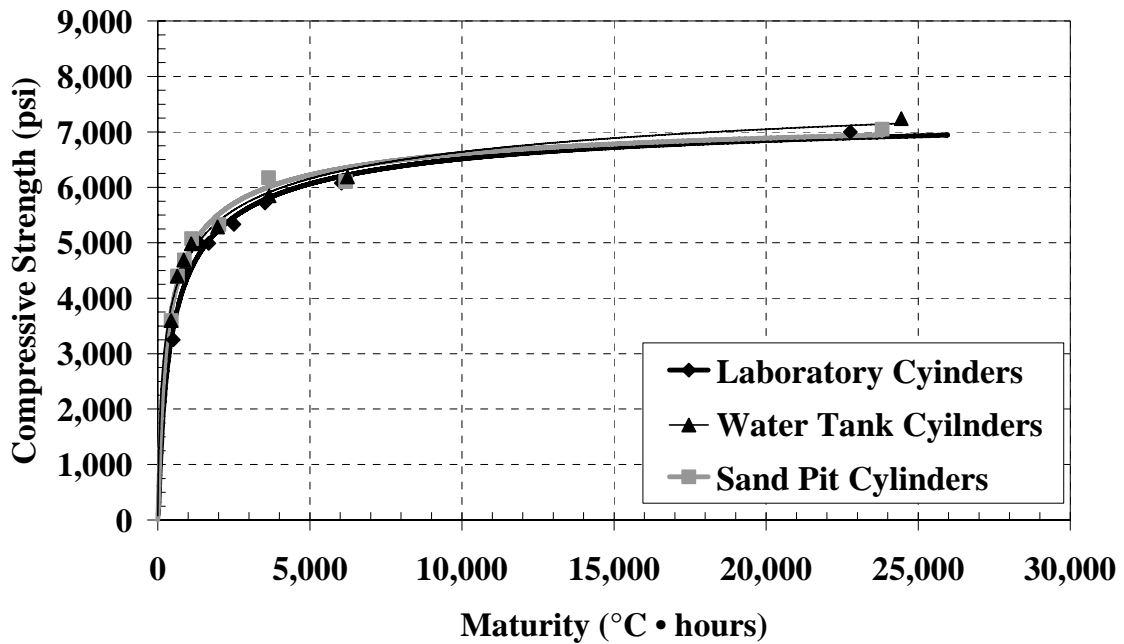
Figure 4-27: S-M relationships using the Nurse-Saul maturity function with T_o = -10\text{ }^\circ\text{C}
