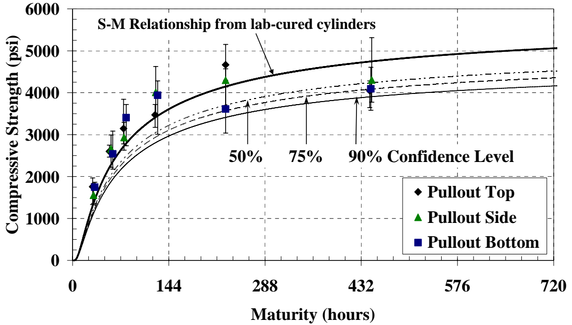
Figure 5-35: Pullout test with laboratory S-M relationship and confidence levels for the cold-weather placement of the mock bridge deck ( E = 33.5 kJ/mol)
