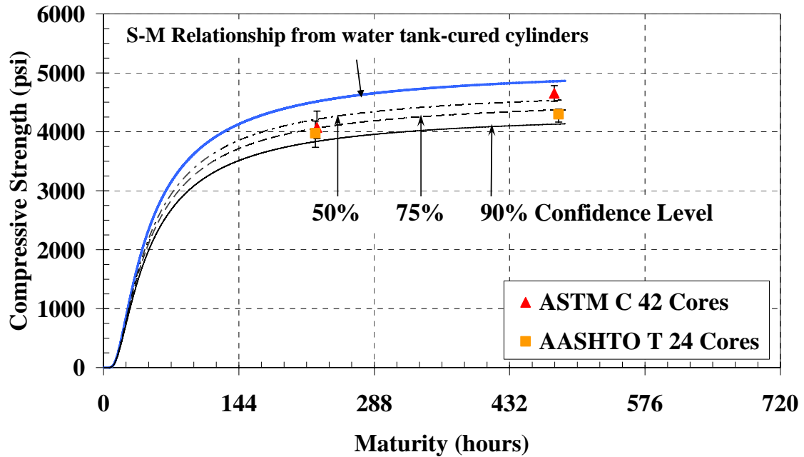
Figure C-25: Cores with water-tank S-M relationship and confidence levels for the cold-weather placement of mock bridge deck ( E = 40 kJ/mol)
