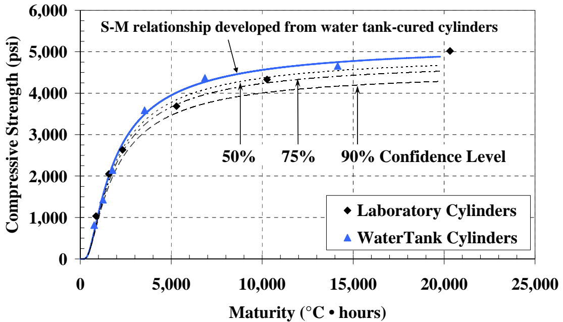
Figure C-10: Water-tank S-M relationship with confidence levels for the cold-weather placement of mock bridge deck (T o = -10 °C)
