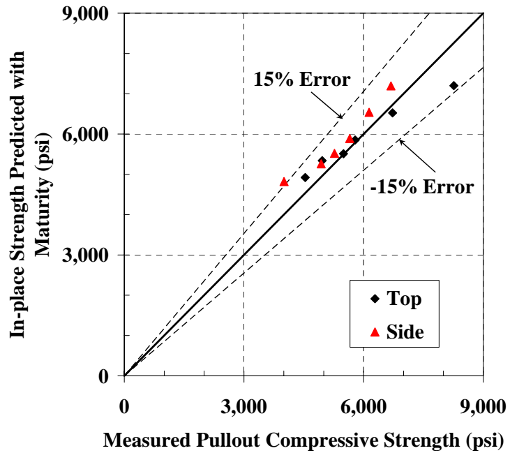
Figure B-49: 45°-line graph for estimating the strength of pullout test on the mock girder using water-tank S-M relationship with Arrhenius maturity function ( E = 33.5\text{ kJ/mol} )
