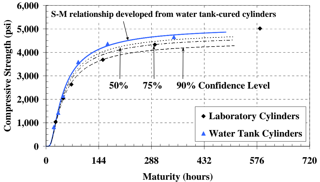
Figure C-13: Water-tank S-M relationship with confidence levels for the cold-weather placement of mock bridge deck ( E = 40 \text{ kJ/mol} )
