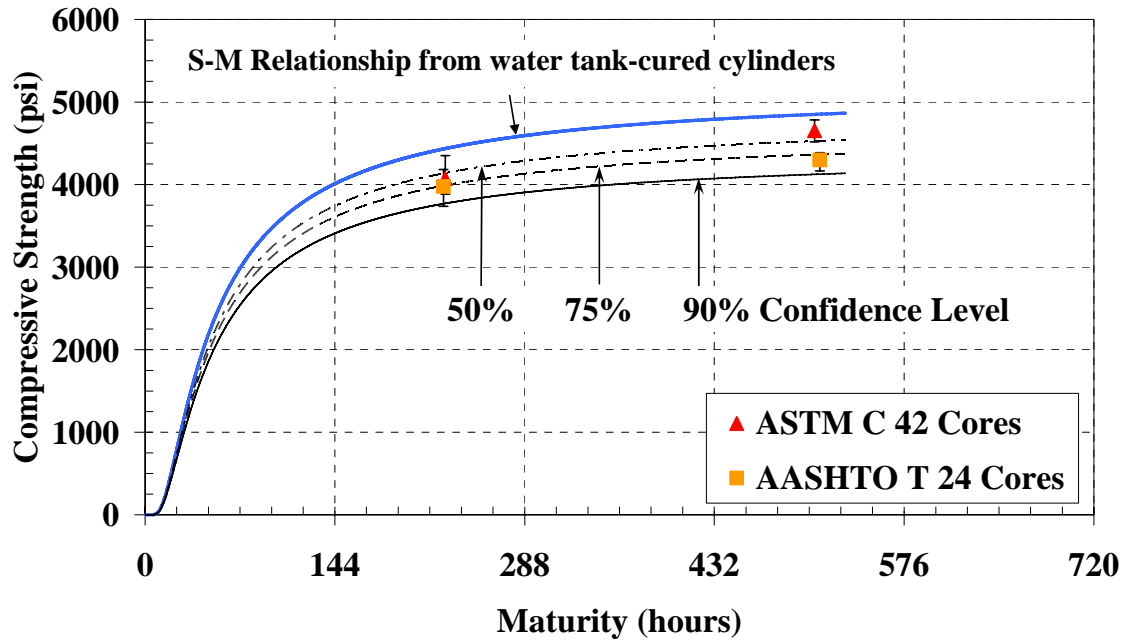
Figure 5-45: Cores with water-tank S-M relationship and confidence levels for the cold-weather placement of mock bridge deck ( E = 33.5 kJ/mol)
