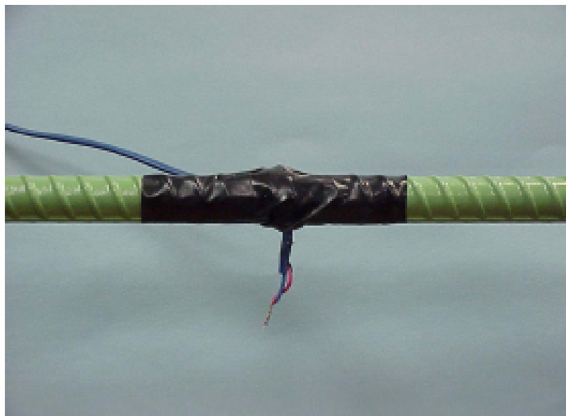
Figure 2. Typical attachment of thermocouple to reinforcing steel
