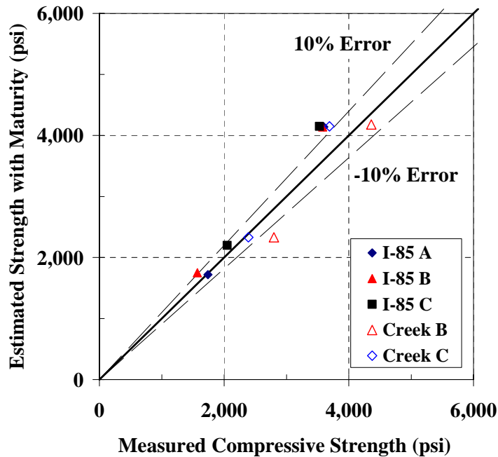
Figure C-92: 45°-line graph for estimating the strength of the verification cylinders using I-85 Bridge S-M relationship with Nurse-Saul maturity function ( T_o = -10 \text{ }^\circ\text{C} )
