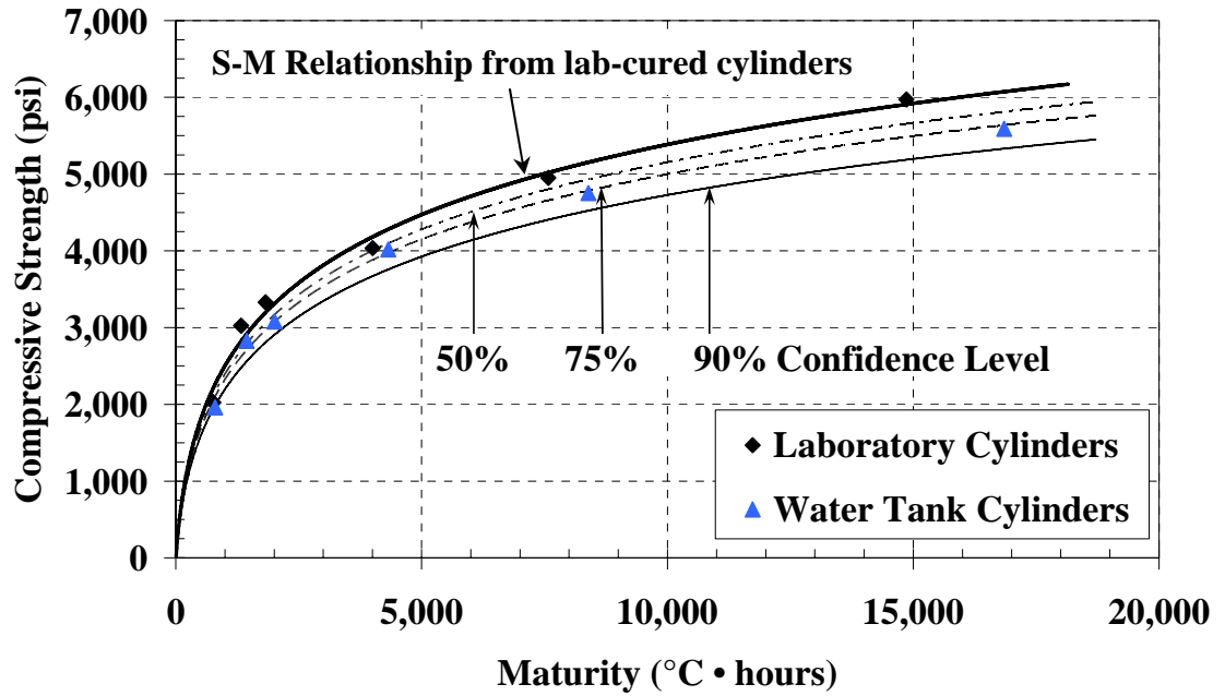
Figure 5-56: S-M relationship for the Laboratory cured cylinders with confidence levels for the warm-weather placement of the mock bridge deck ( T_0 = 0^{\circ}\text{C} )
