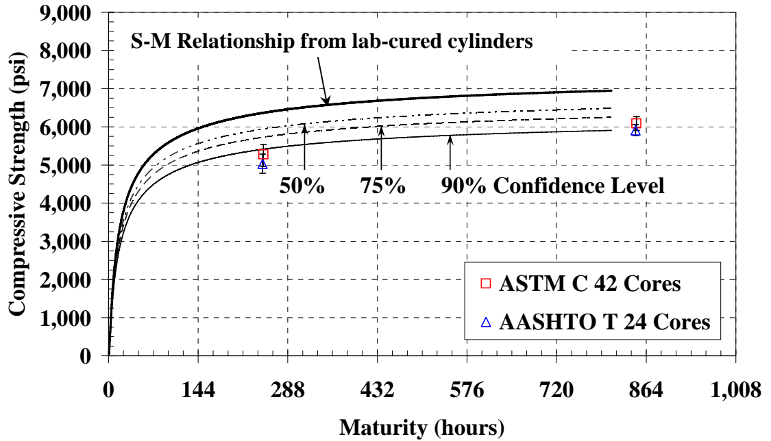
Figure 4-41: Cores with laboratory S-M relationship and confidence levels (E = 33.5 kJ/mol)
