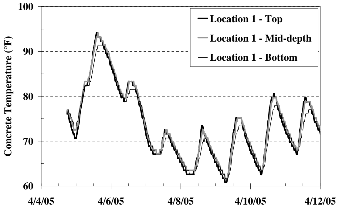
Figure C-69: Temperature history of Location 1 from the Creek Bridge
