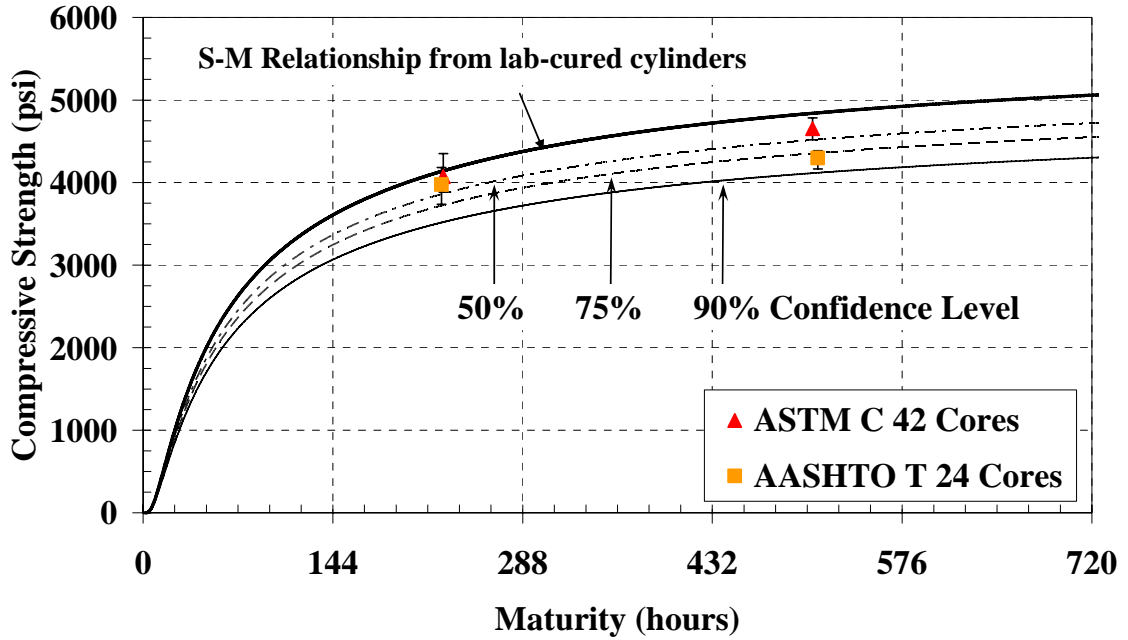
Figure 5-43: Cores with laboratory S-M relationship and confidence levels for the cold-weather placement of the mock bridge deck ( E = 33.5 kJ/mol)
