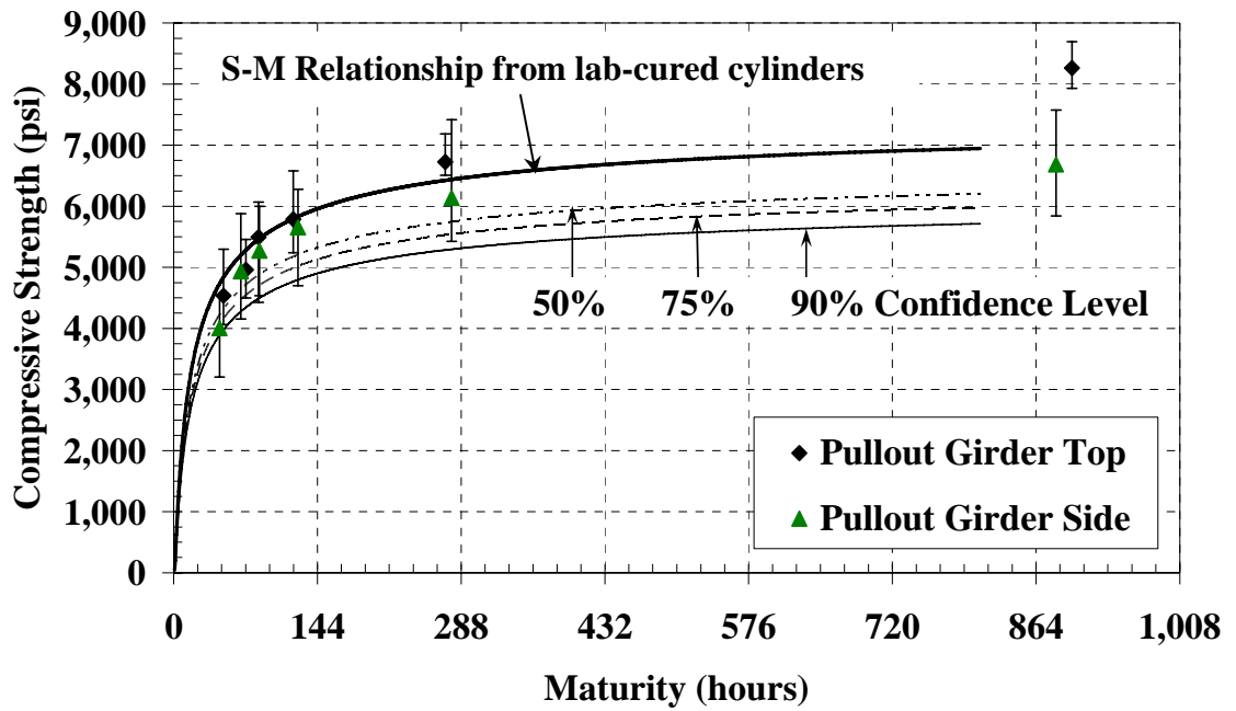
Figure 4-37: Pullout test with laboratory S-M relationship and confidence levels (E = 33.5 kJ/mol)
