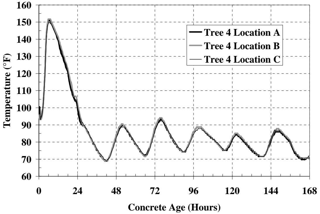
Figure B-12: Girder temperatures Tree 4 Location A, B, and C
