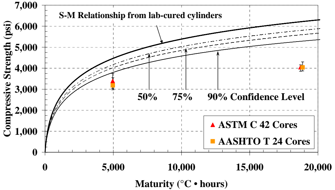
Figure 5-67: Cores with laboratory S-M relationship and confidence levels for the warm-weather placement of the mock bridge deck ( T_0 = 0^{\circ}\text{C} )
