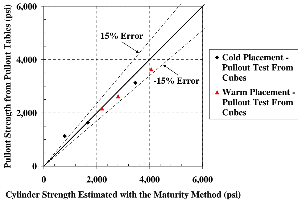
Figure C-78: 45°-line graph to evaluate the pullout table using estimated strength from water-tank S-M relationship using the Nurse-Saul maturity function ( T_0 = -10 \text{ }^\circ\text{C} )
