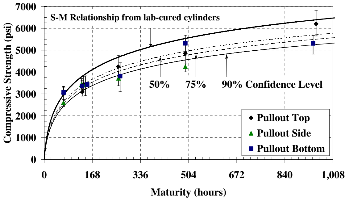
Figure 5-60: Pullout test with laboratory S-M relationship and confidence levels for the warm-weather placement of the mock bridge deck ( E = 33.5 \text{ kJ/mol} )
