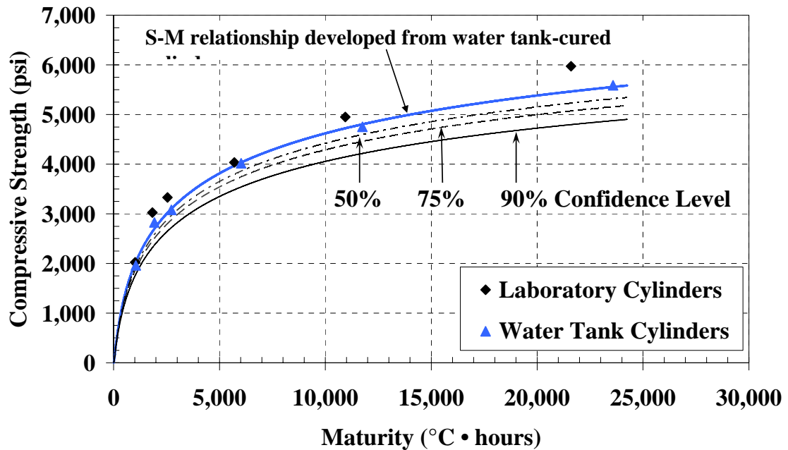
Figure C-35: Water-tank cylinders S-M relationship with confidence levels for the warm-weather placement of mock bridge deck ( T_o = -10\text{ }^\circ\text{C} )
