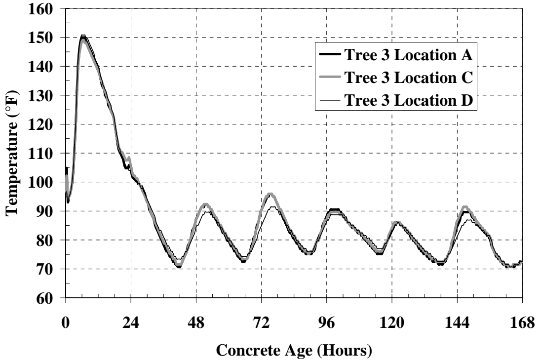
Figure B-10: Girder temperatures Tree 3 Location A, C, and D
