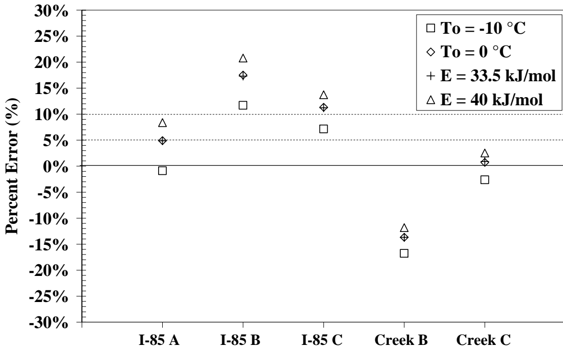
Figure 5-126: 2,400-psi verification test percent errors for best-fit I-85 Bridge S-M relationship
