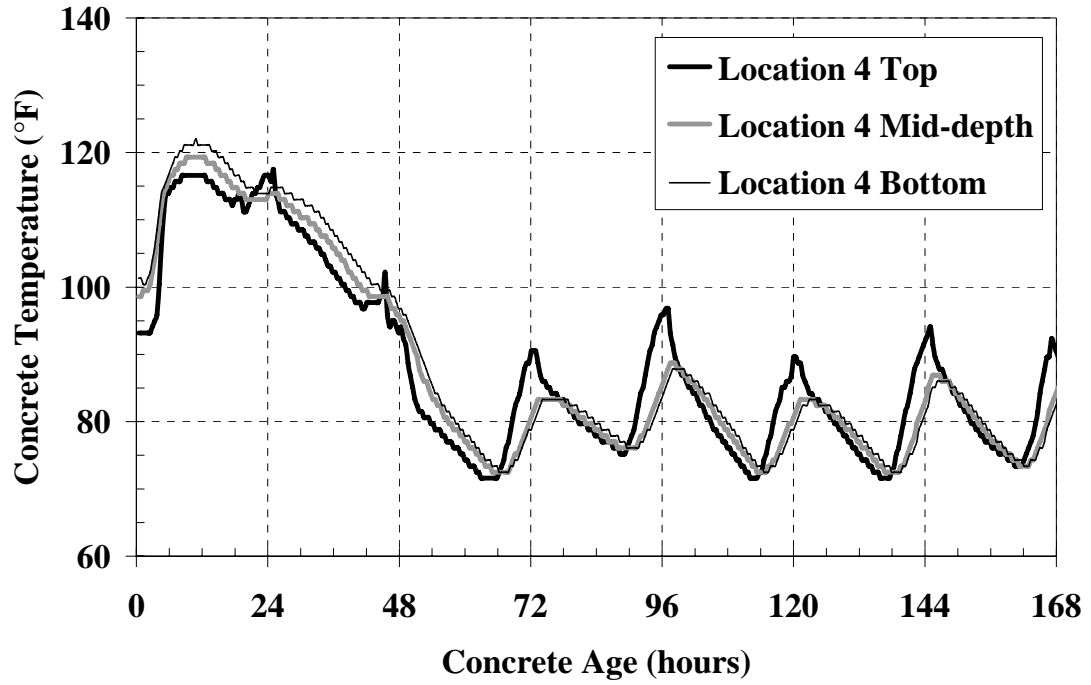
Figure C-32: Mock bridge deck temperatures Location 4 for warm-weather placement
