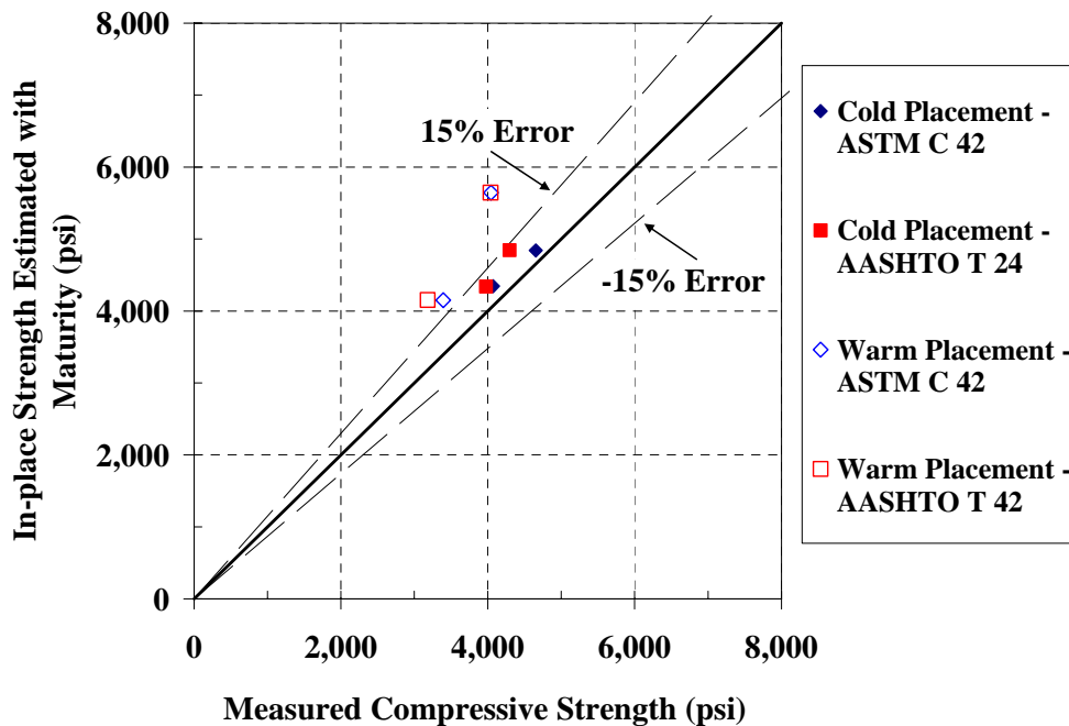
Figure C-90: 45°-line graph for estimating the strength of cores for the mock bridge deck using water-tank S-M relationship with Nurse-Saul maturity function ( T_0 = -10 \text{ }^\circ\text{C} )
