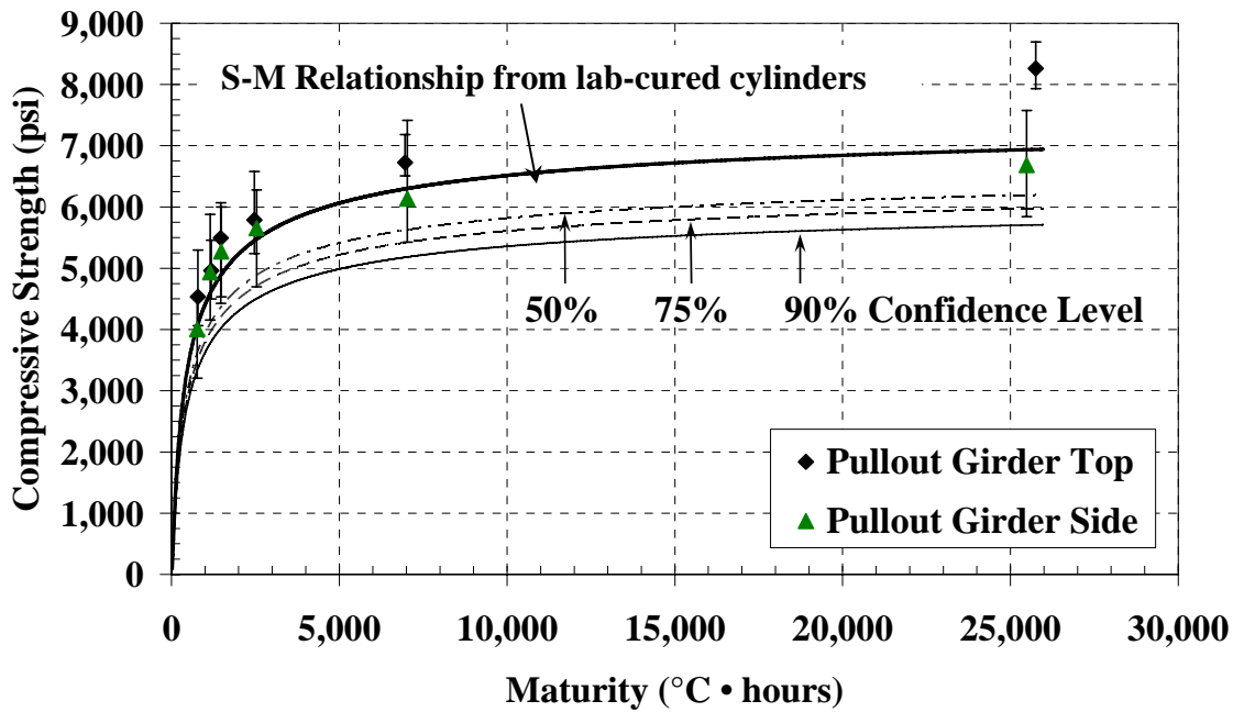
Figure 4-35: Pullout test with laboratory S-M relationship and confidence levels ( T_0 = -10\text{ }^\circ\text{C} )
