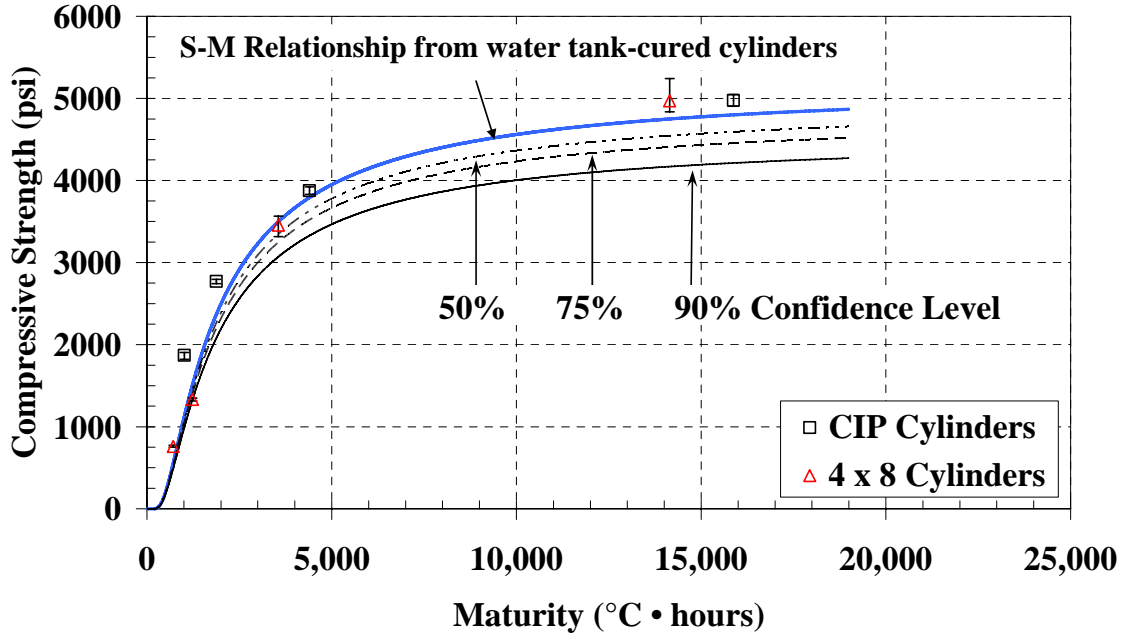
Figure C-20: Cast-in-place cylinders and 4 x 8 inch cylinders with water-tank S-M relationship and confidence levels for the cold-weather placement of mock bridge deck ( T_o = -10^{\circ}\text{C} )
