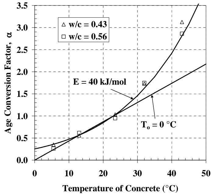
Figure 2-7: Comparing Arrhenius maturity function with E = 40 \text{ kJ/mol} to Nurse-Saul maturity function with T_0 = 0 \text{ }^{\circ}\text{C} ( 32 \text{ }^{\circ}\text{F} ) (Carino 1984)
