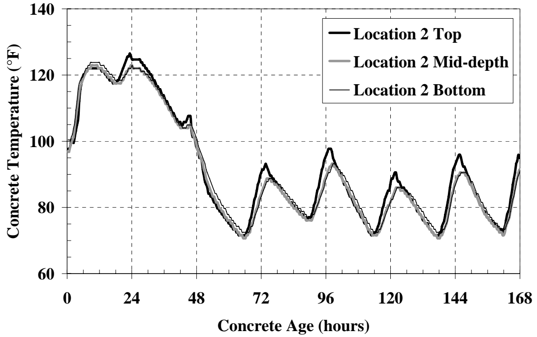
Figure C-30: Mock bridge deck temperatures Location 2 for warm-weather placement
