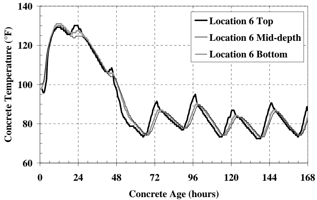
Figure C-34: Mock bridge deck temperatures Location 6 for warm-weather placement
