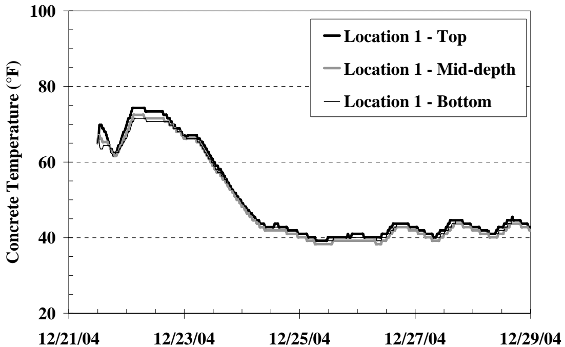
Figure C-51: Temperature history of Location 1 from the I-85 Bridge
