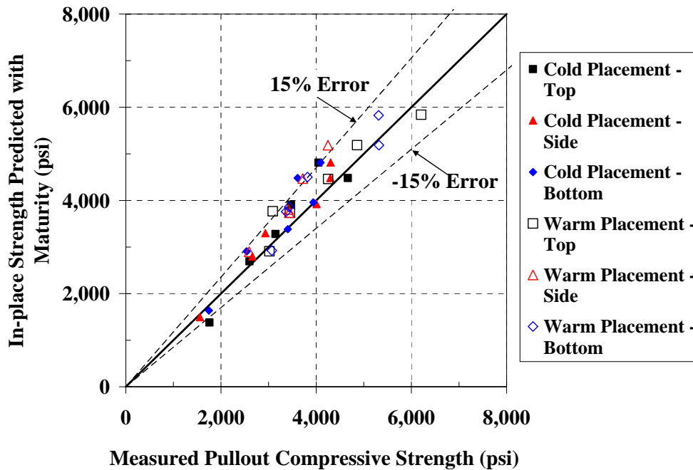
Figure C-83: 45°-line graph for estimating the strength of pullout test on the mock bridge deck using water-tank S-M relationship with Arrhenius maturity function ( E = 40 \text{ kJ/mol} )
