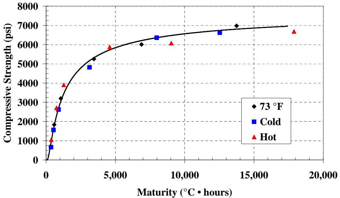
Figure 2-4: Strength-maturity relationship using the NSM function for Figure 2-3 ( T_0 = 0\text{ }^\circ\text{C} )
