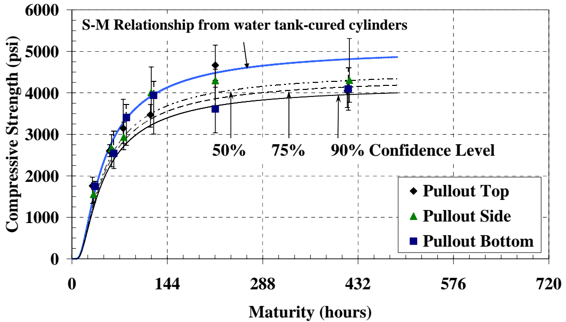
Figure C-17: Pullout test with water-tank S-M relationship and confidence levels for the cold-weather placement of mock bridge deck ( E = 40 \text{ kJ/mol} )
