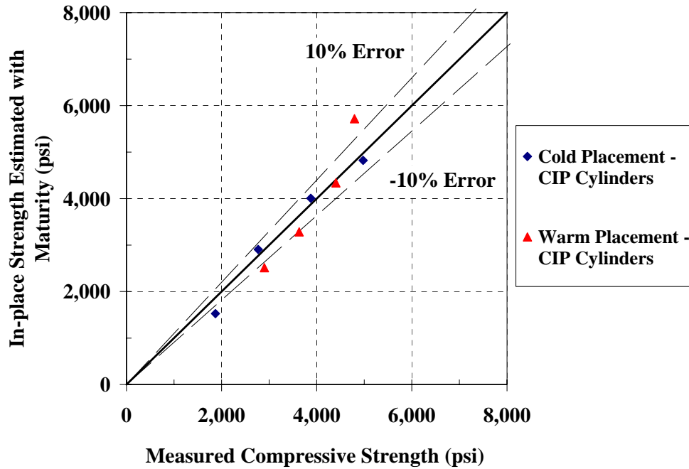
Figure 5-112: 45°-line graph for estimating the strength of CIP cylinders on the mock bridge deck using water-tank S-M relationship with Nurse-Saul maturity function ( T_o = 0\text{ }^\circ\text{C} )
