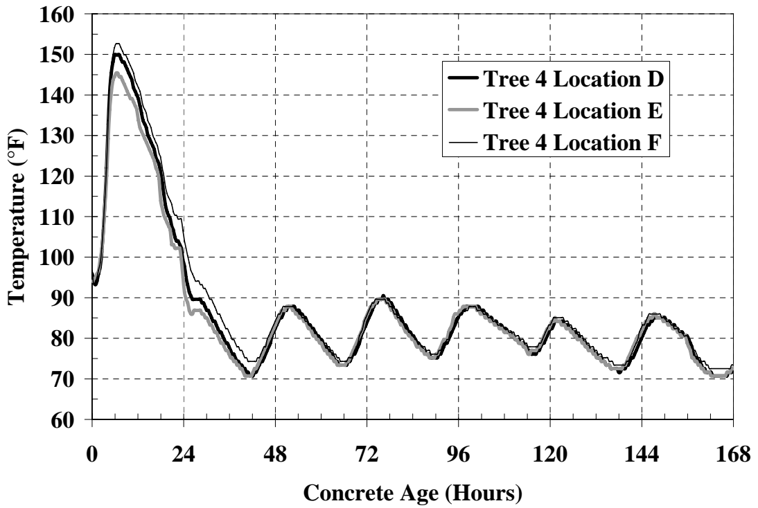
Figure B-13: Girder temperatures Tree 4 Location D, E, and F
