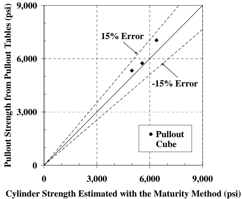
Figure B-45: 45°-line graph to evaluate the pullout table using estimated strength from water-tank S-M relationship using the Arrhenius maturity ( E = 33.5\text{ kJ/mol} )
