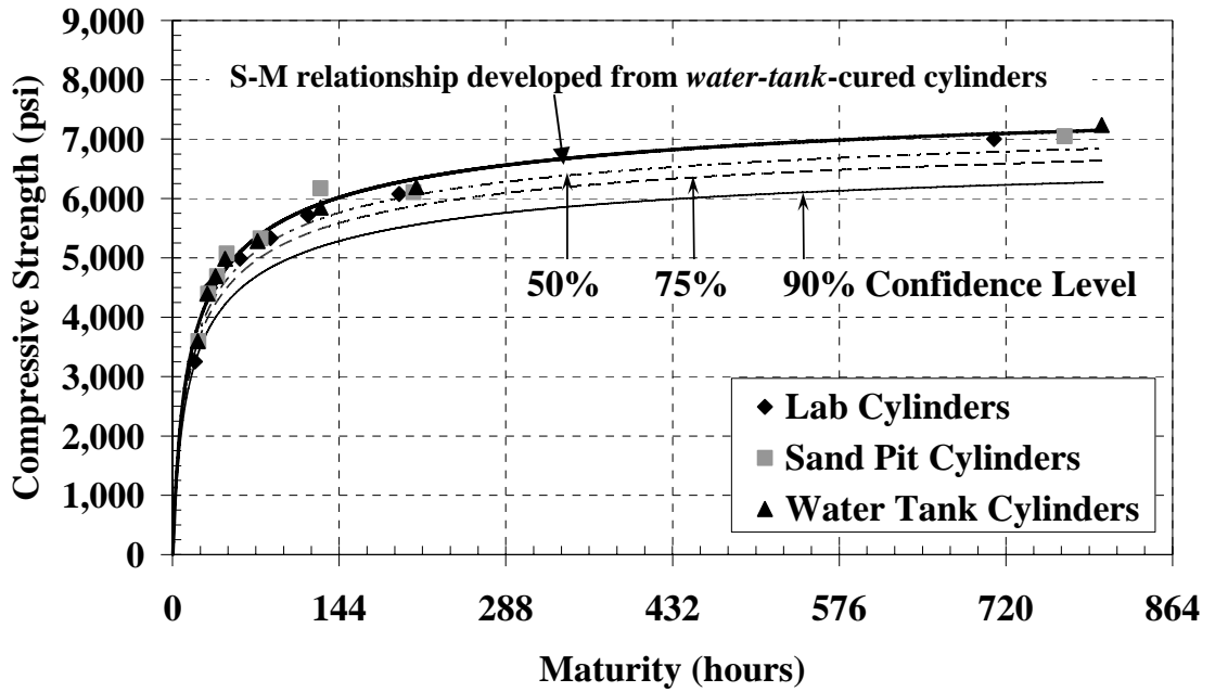
Figure B-22: Water-tank S-M relationship with confidence levels ( E = 33.5 kJ/mol)
