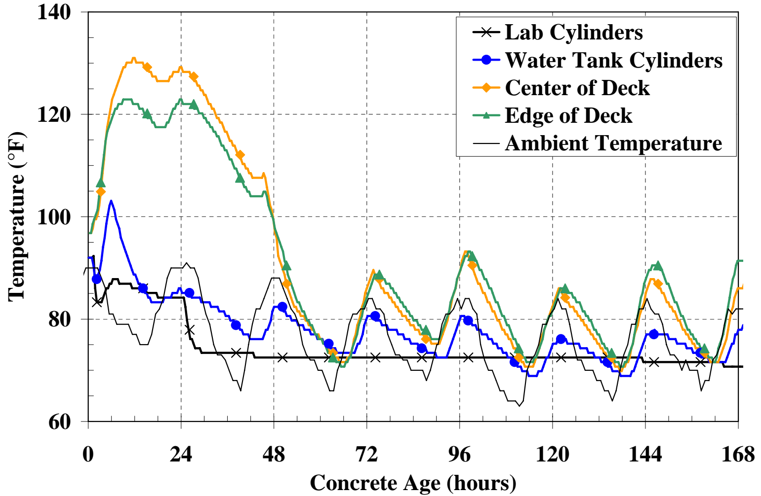
Figure 5-46: Temperature history of 6 x 12 inch cylinders and the mock bridge deck for the warm-weather placement
