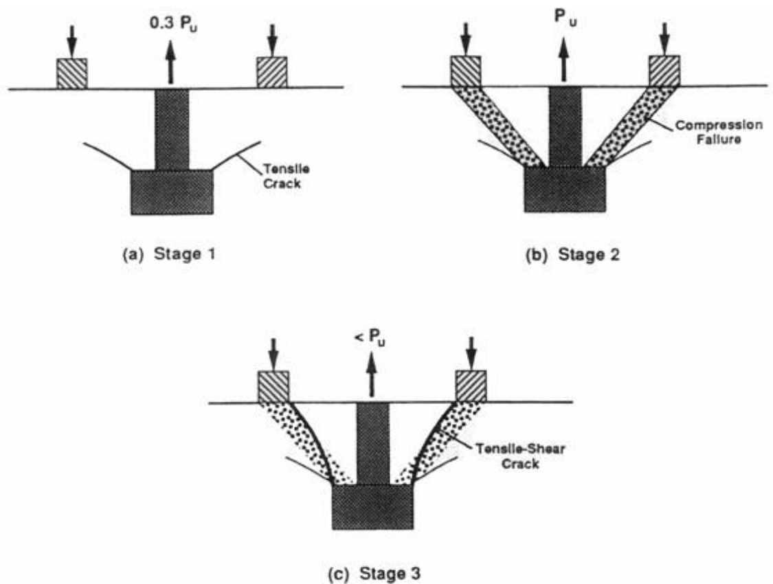
Figure 2-27: Failure mechanism of pullout test according to Krenchel and Bickley (Carino 1991)
