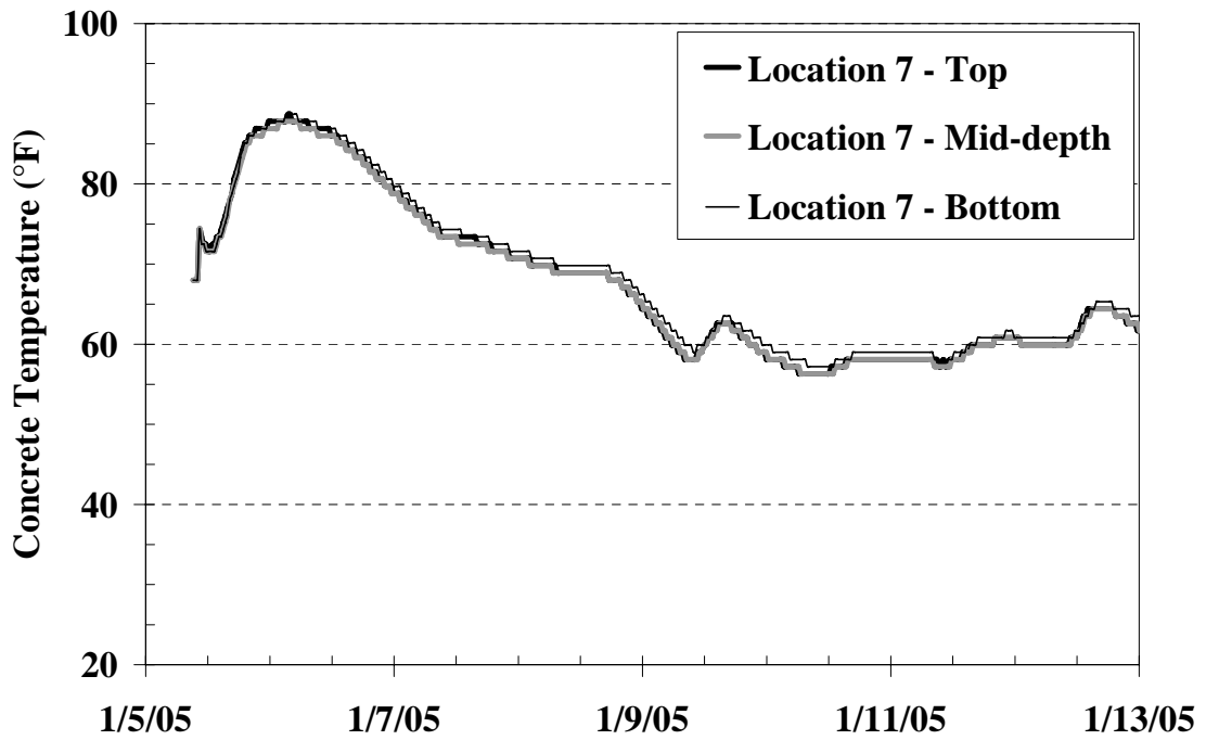
Figure C-59: Temperature history of Location 7 from the I-85 Bridge
