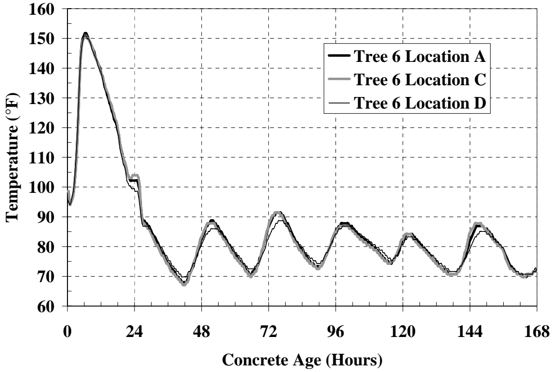
Figure B-16: Girder temperatures Tree 6 Location A, C, and D
