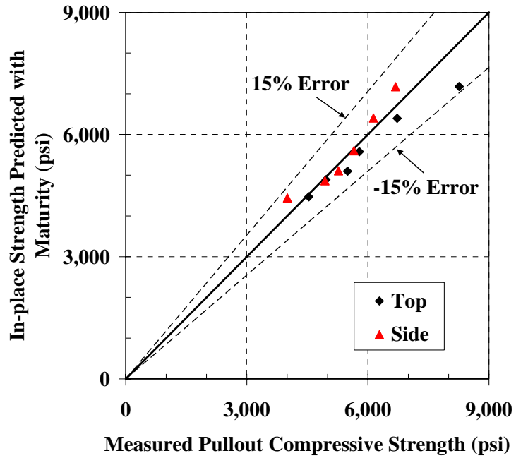
Figure B-48: 45°-line graph for estimating the strength of pullout test on the mock girder using water-tank S-M relationship with Nurse-Saul maturity function ( T_o = -10\text{ }^\circ\text{C} )
