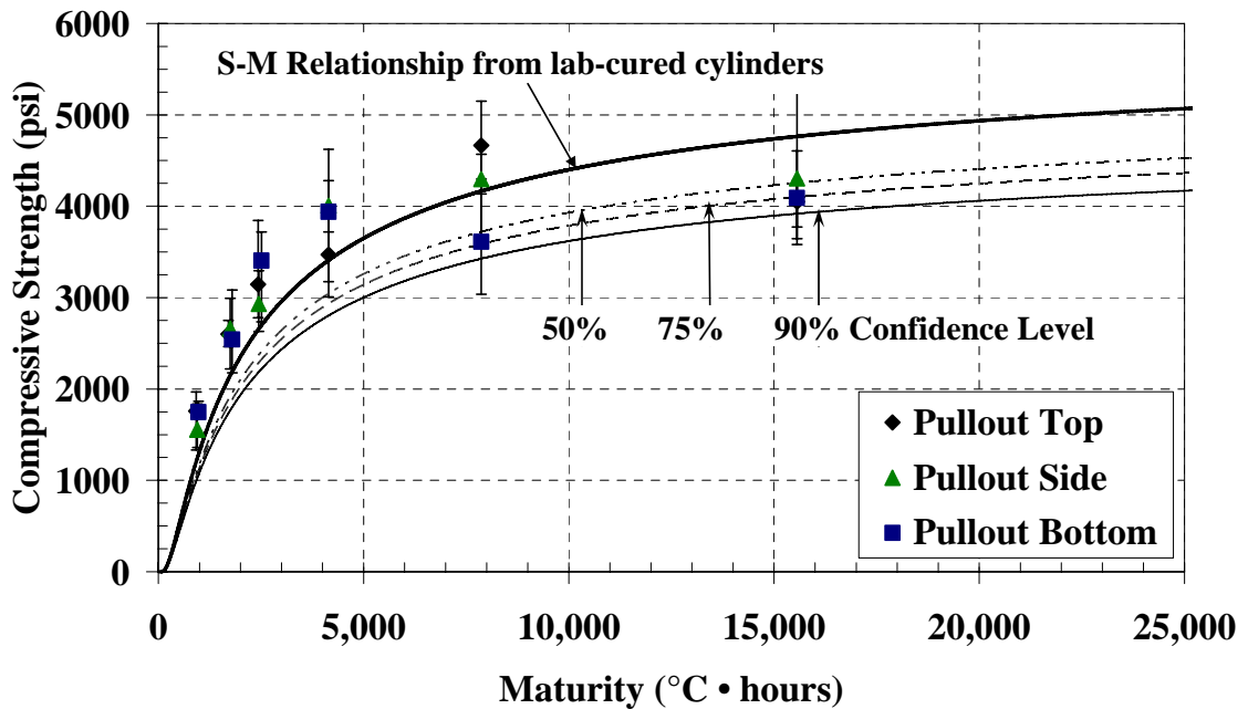
Figure C-14: Pullout test with laboratory S-M relationship and confidence levels for the cold-weather placement of the mock bridge deck ( T_0 = -10 \text{ }^{\circ}\text{C} )
