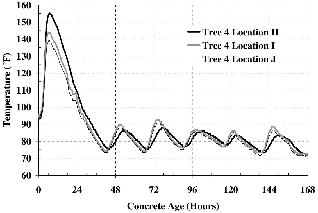
Figure B-14: Girder temperatures Tree 4 Location H, I, and J
