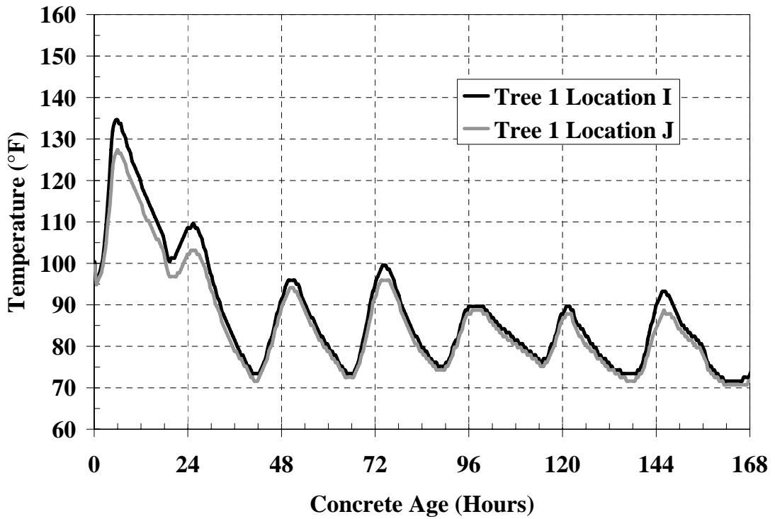
Figure B-7: Girder temperatures Tree 1 Location I and J
