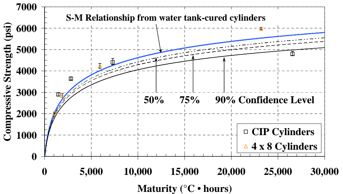
Figure C-45: Cast-in-place cylinders and 4 x 8 inch cylinders with water-tank S-M relationship and confidence levels for the warm-weather placement of mock bridge deck ( T_0 = -10^\circ\text{C} )
