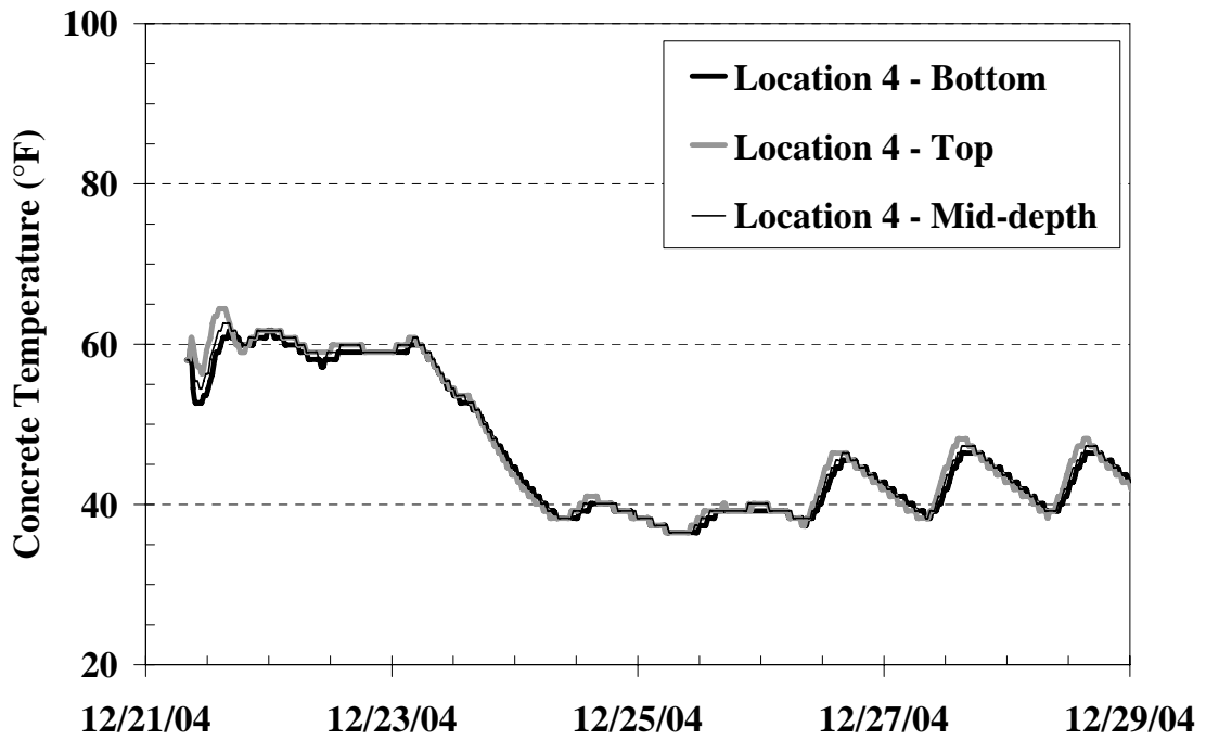
Figure C-55: Temperature history of Location 4 from the I-85 Bridge
