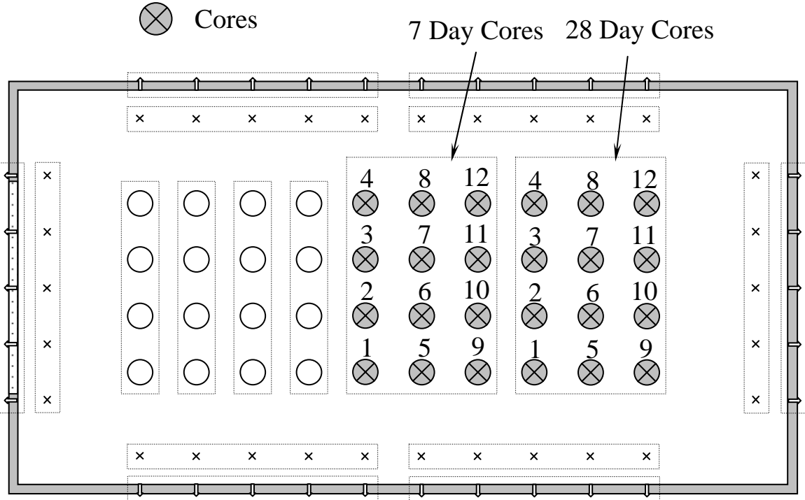
Figure C-1: Top of mock bridge deck core numbering
