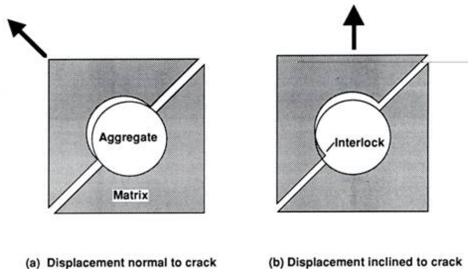
Figure 2-26: Model to illustrate aggregate interlock mechanism during pullout test (Carino 1991)
