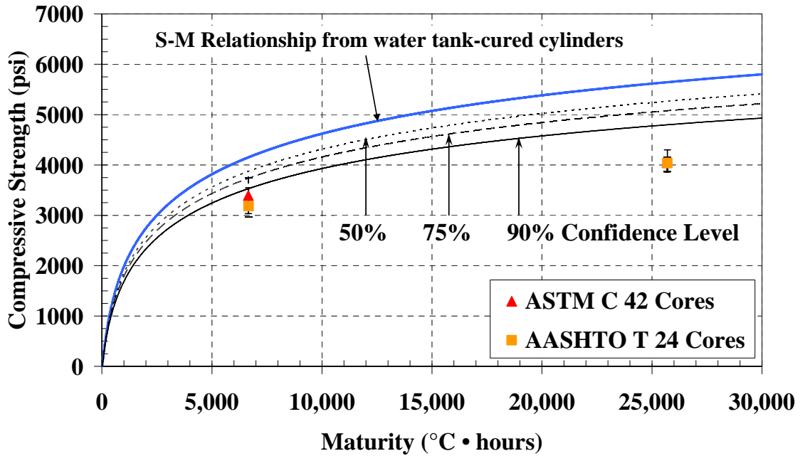
Figure C-49: Cores with water-tank S-M relationship and confidence levels for the warm-weather placement of mock bridge deck ( T_o = -10^{\circ}\text{C} )
