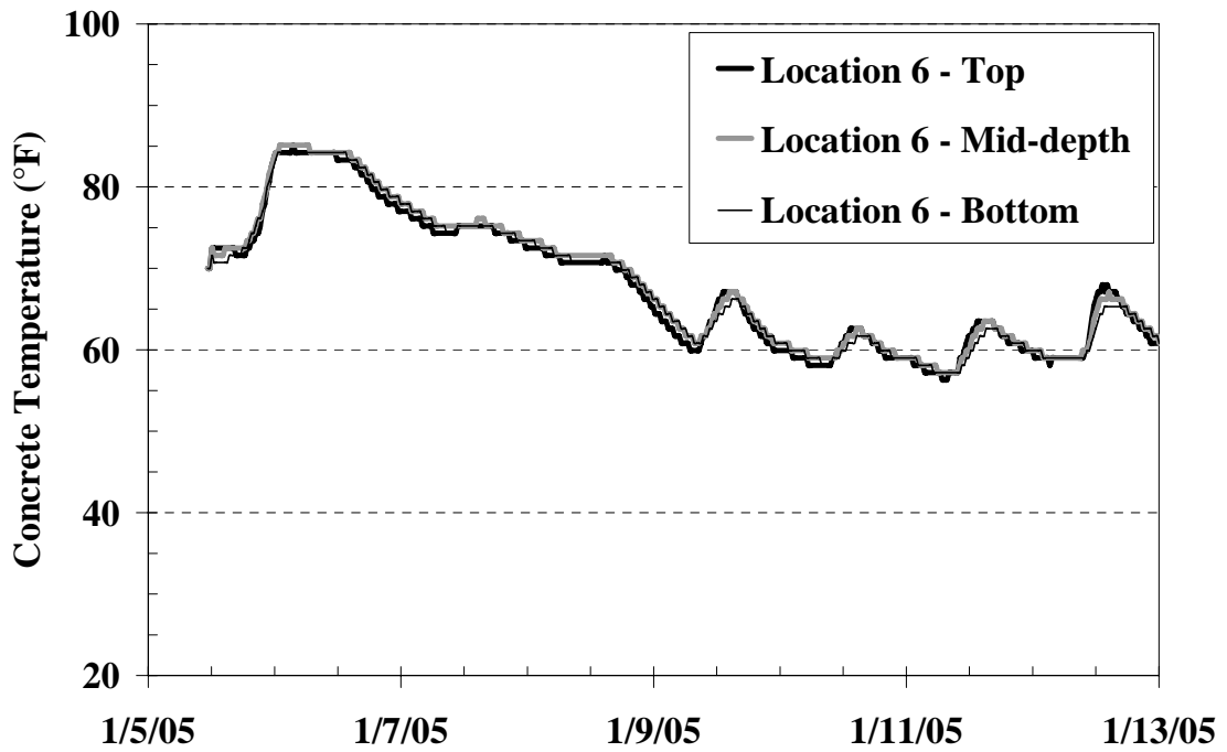
Figure C-57: Temperature history of Location 6 from the I-85 Bridge
