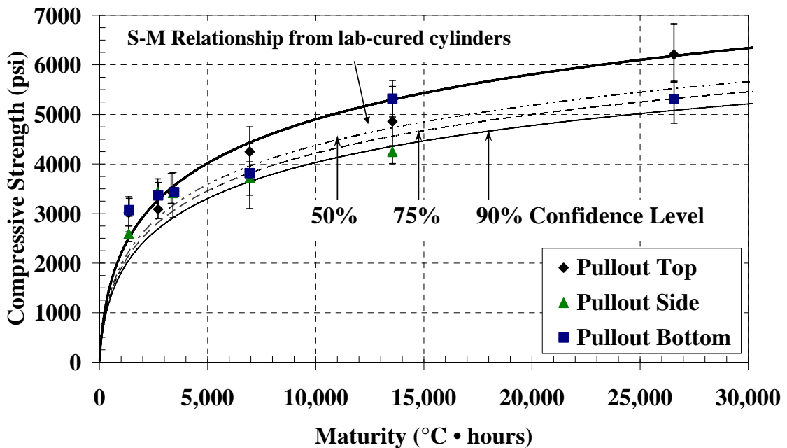
Figure C-39: Pullout test with laboratory S-M relationship and confidence levels for the warm-weather placement of the mock bridge deck ( T_o = -10 \text{ }^{\circ}\text{C} )
