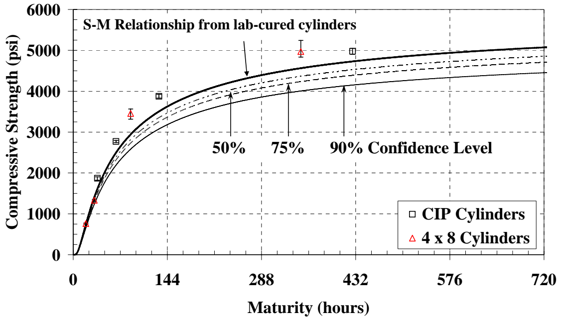
Figure C-19: Cast-in-place cylinders and 4 x 8 inch cylinders with laboratory S-M relationship and confidence levels for the cold-weather placement of the mock bridge deck ( E = 40 \text{ kJ/mol} )
