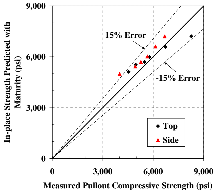
Figure 4-52: 45°-line graph for estimating the strength of pullout test on the mock girder using water-tank S-M relationship with Arrhenius maturity function ( E = 40 kJ/mol)
