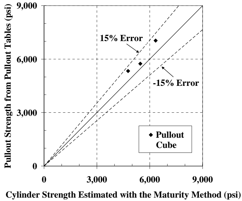
Figure B-44: 45°-line graph to evaluate the pullout table using estimated strength from water-tank S-M relationship using the Nurse-Saul maturity function ( T_0 = -10\text{ }^\circ\text{C} )
