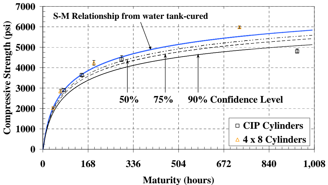
Figure 5-66: Cast-in-place cylinders and 4 x 8 inch cylinders with water-tank S-M relationship and confidence levels for the warm-weather placement of mock bridge deck ( E = 33.5 \text{ kJ/mol} )
