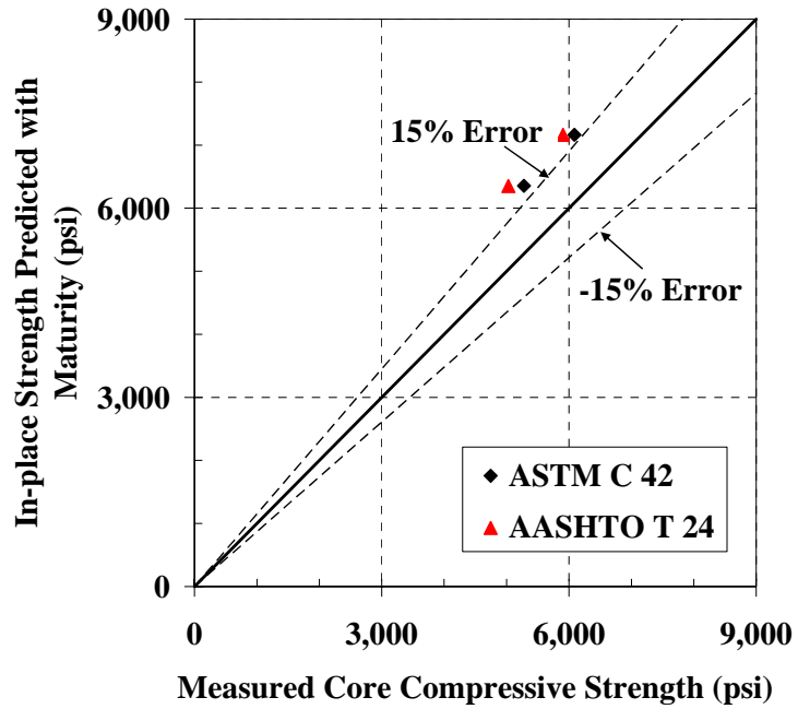
Figure B-54: 45°-line graph for estimating the strength of cores for the mock girder using water-tank S-M relationship with Nurse-Saul maturity function ( T_0 = -10\text{ }^\circ\text{C} )
