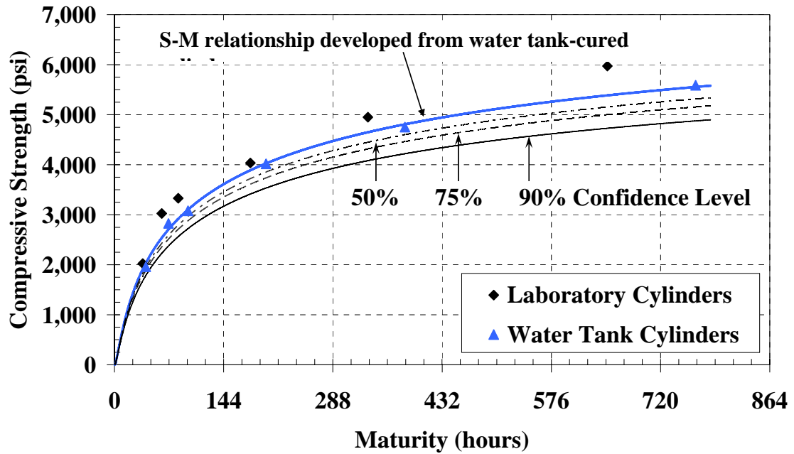
Figure C-38: Water-tank cylinders S-M relationship with confidence levels for the warm-weather placement of mock bridge deck ( E = 40 \text{ kJ/mol} )
