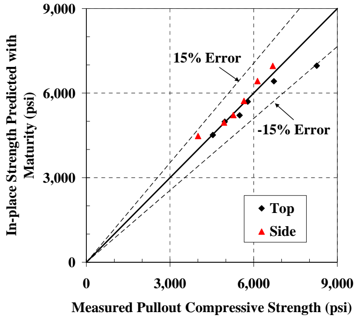
Figure B-50: 45°-line graph for estimating the strength of pullout test on the mock girder using sand-pit S-M relationship with Nurse-Saul maturity function ( T_o = -10\text{ }^\circ\text{C} )
