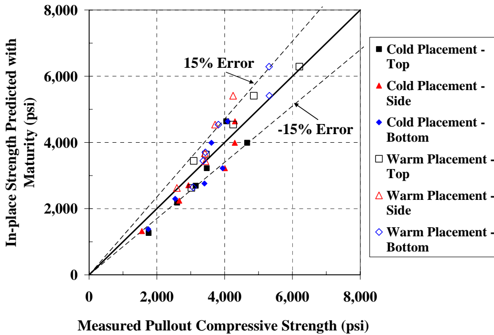
Figure 5-106: 45°-line graph for estimating the strength of pullout test on the mock bridge deck using laboratory S-M relationship with Nurse-Saul maturity function ( T_o = 0\text{ }^{\circ}\text{C} )
