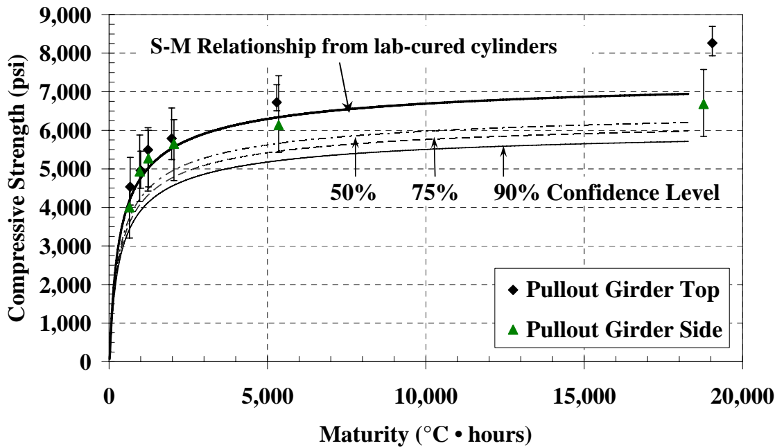
Figure 4-36: Pullout test with laboratory S-M relationship and confidence levels ( T_0 = 0\text{ }^\circ\text{C} )
