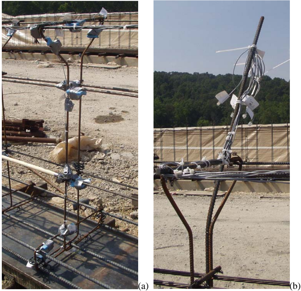
Figure 4-18: (a) iButton Tree 4 installed on a stirrup and (b) Lead wires with phone jacks
