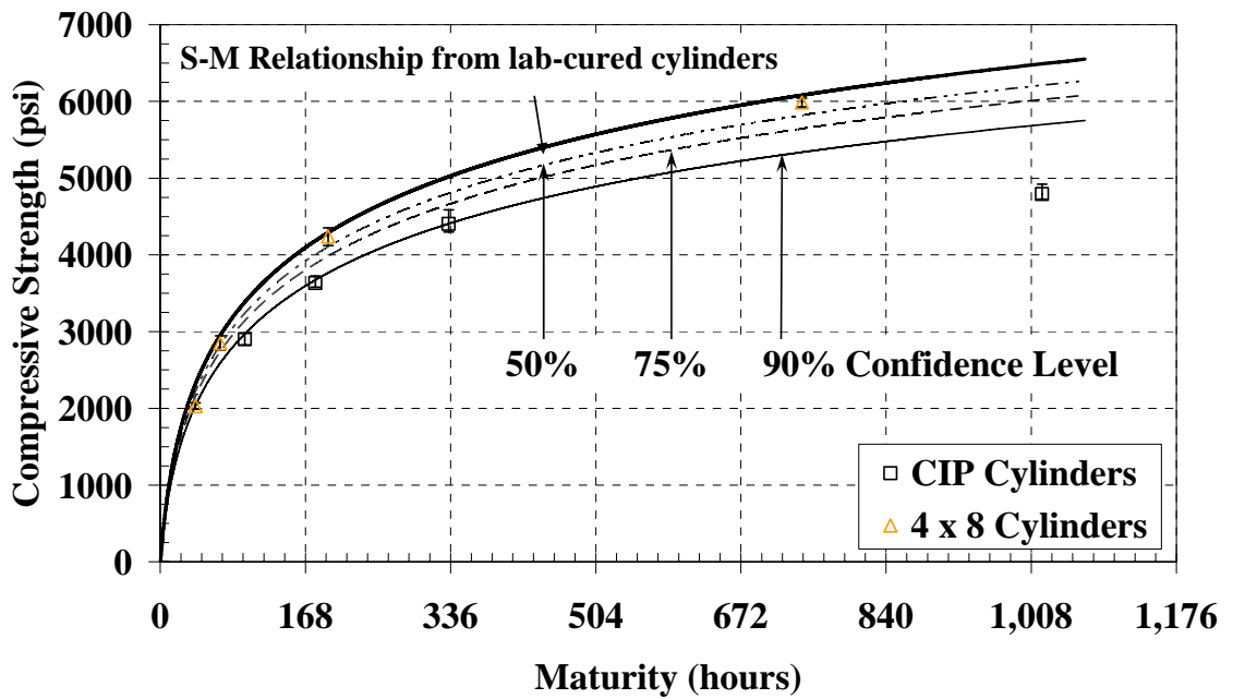
Figure C-44: Cast-in-place cylinders and 4x 8 inch cylinders with laboratory S-M relationship and confidence levels for the warm-weather placement of the mock bridge deck ( E = 40 \text{ kJ/mol} )
