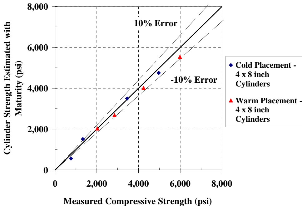
Figure C-76: 45°-line graph for estimating the strength of water-tank-cured 4 x 8 inch cylinder from the mock bridge deck water-tank S-M relationships using the Nurse-Saul maturity function ( T_0 = -10 \text{ }^\circ\text{C} )
