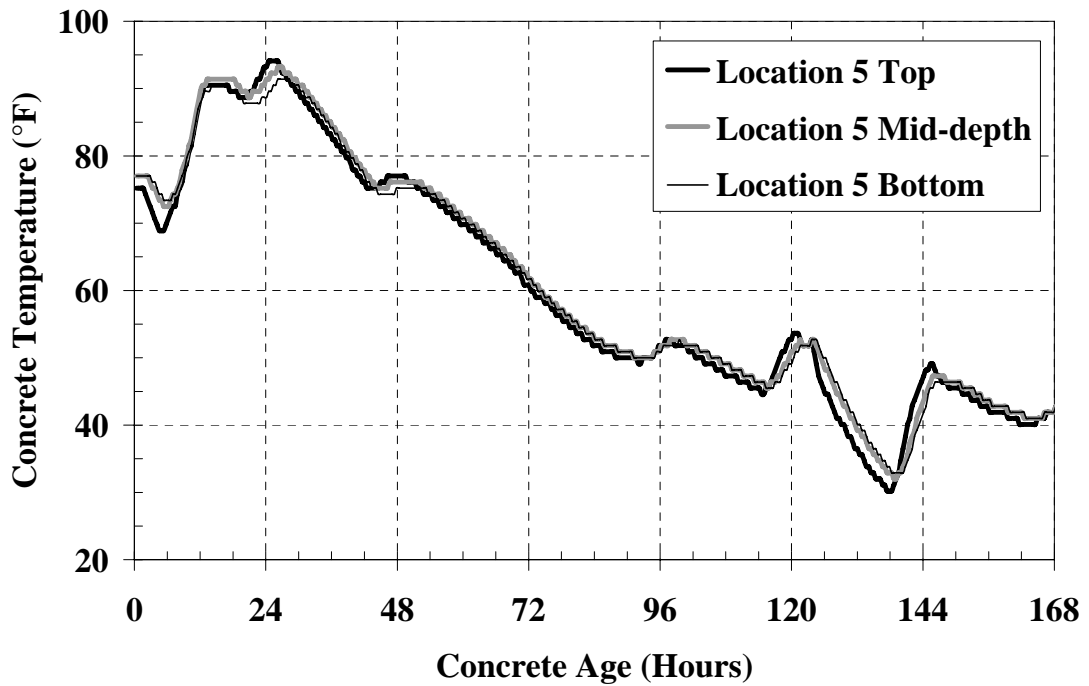
Figure C-8: Mock bridge deck temperatures Location 5 for cold-weather placement
