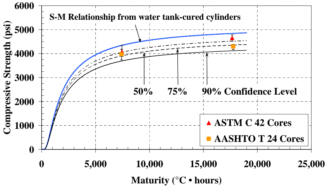
Figure C-24: Cores with water-tank S-M relationship and confidence levels for the cold-weather placement of mock bridge deck ( T_o = -10^{\circ}\text{C} )
