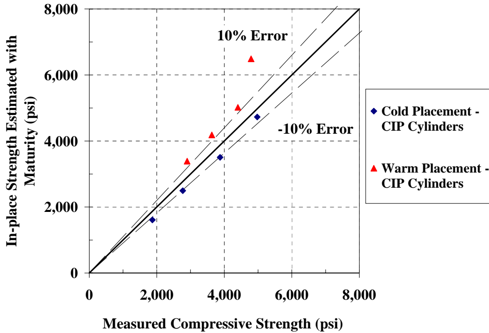
Figure C-85: 45°-line graph for estimating the strength of CIP cylinders on the mock bridge deck using Laboratory S-M relationship with Arrhenius maturity function ( E = 40 \text{ kJ/mol} )
