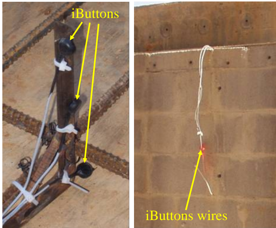
Figure 5-10: iButtons installed in the mock bridge deck
