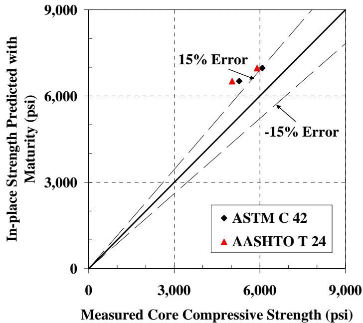
Figure 4-60: 45°-line graph for estimating the strength of cores for the mock girder using sand-pit S-M relationship with Arrhenius maturity function ( E = 40 kJ/mol)
