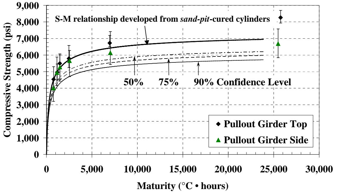
Figure B-32: Pullout test with sand-pit S-M relationship and confidence levels ( T_0 = -10^{\circ}\text{C} )
