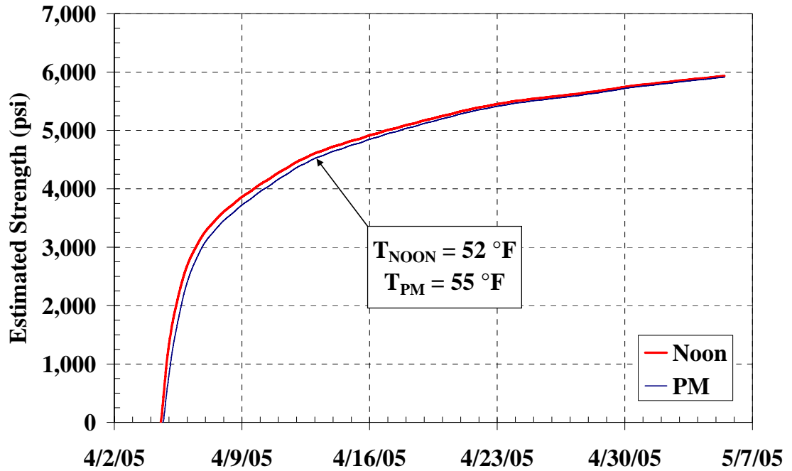
Figure 5-93: Creek Bridge deck strength development using Nurse-Saul maturity function with T_o = 0 \text{ }^\circ\text{C}
