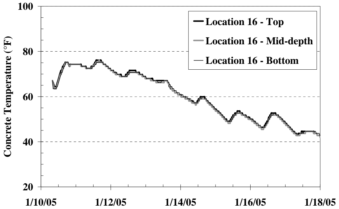
Figure C-68: Temperature history of Location 16 from the I-85 Bridge
