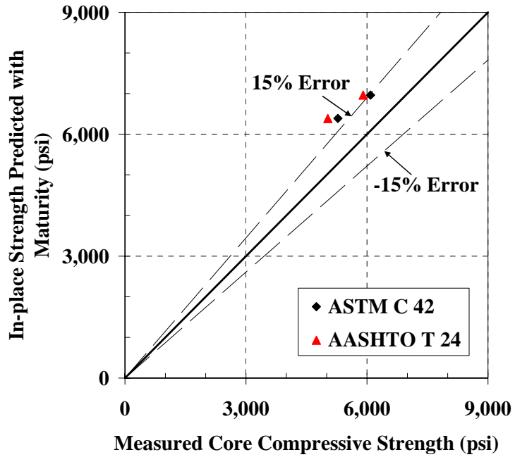
Figure B-56: 45°-line graph for estimating the strength of cores for the mock girder using sand-pit S-M relationship with Nurse-Saul maturity function ( T_0 = -10\text{ }^\circ\text{C} )
