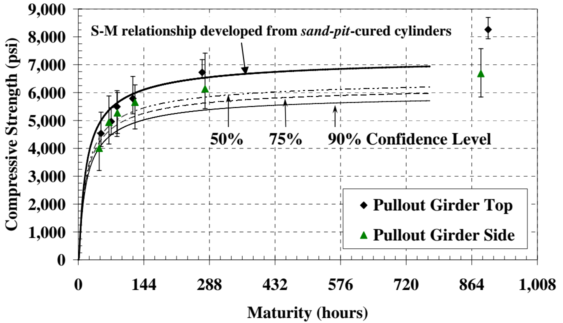
Figure B-34: Pullout test with sand-pit S-M relationship and confidence levels (E = 33.5 kJ/mol)
