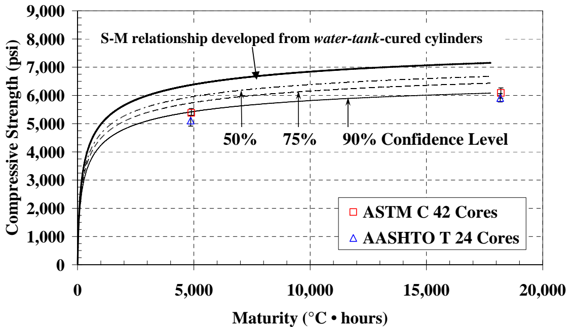
Figure B-37: Cores with water-tank S-M relationship and confidence levels ( T_0 = 0^\circ\text{C} )
