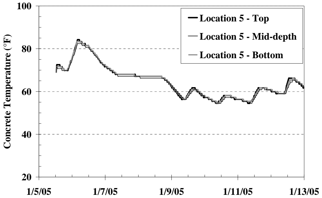
Figure C-56: Temperature history of Location 5 from the I-85 Bridge
