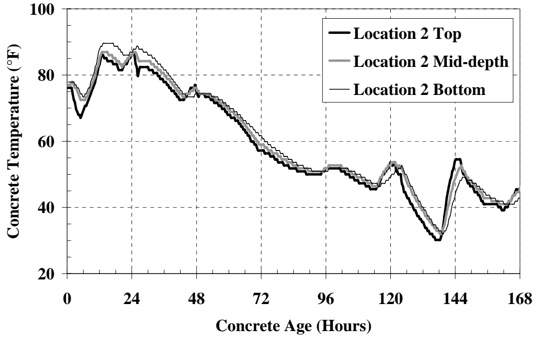
Figure C-5: Mock bridge deck temperatures Location 2 for cold-weather placement
