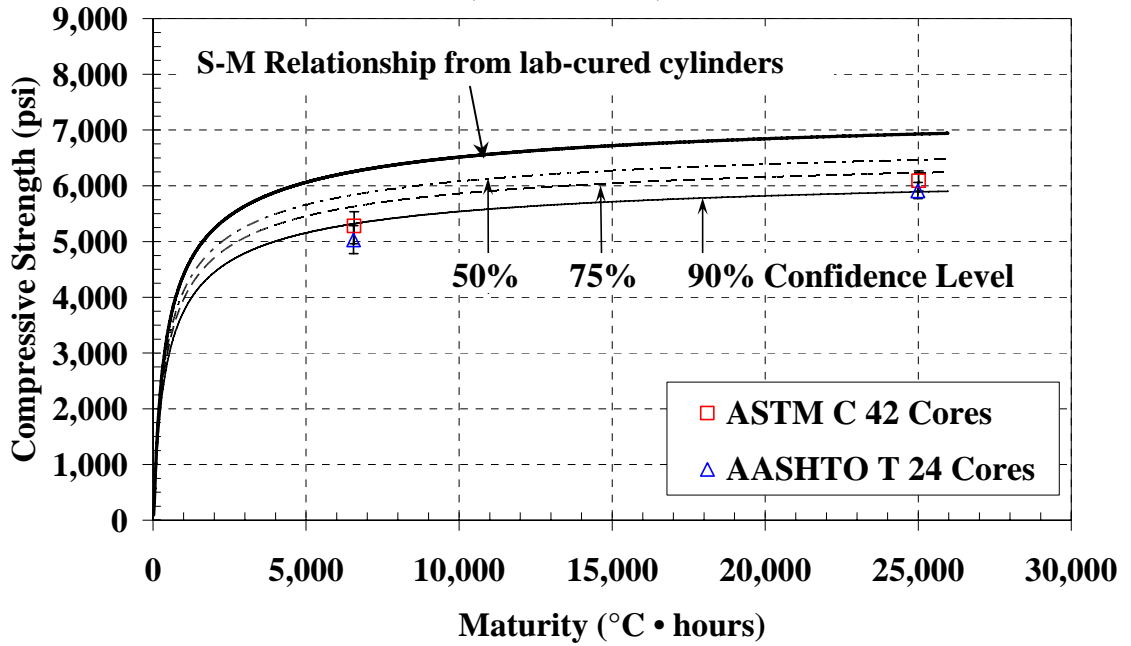
Figure 4-38: Pullout test with laboratory S-M relationship and confidence levels ( E = 40 \text{ kJ/mol} )
