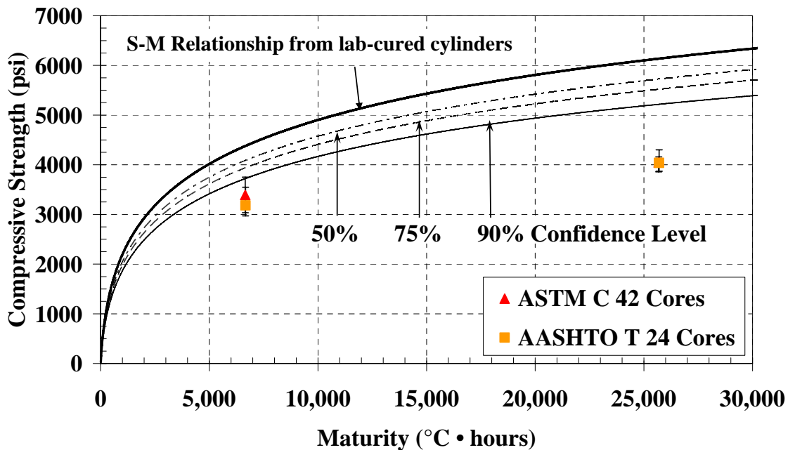
Figure C-47: Cores with laboratory S-M relationship and confidence levels for the warm-weather placement of the mock bridge deck ( T_o = -10 \text{ }^{\circ}\text{C} )
