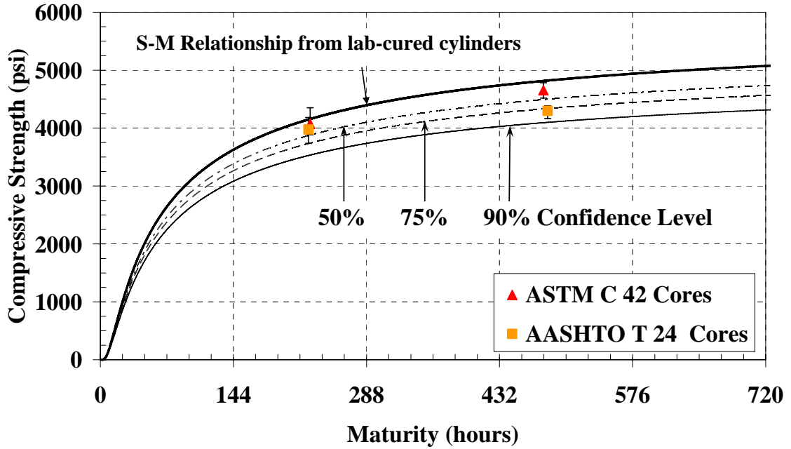
Figure C-23: Cores with laboratory S-M relationship and confidence levels for the cold-weather placement of the mock bridge deck ( E = 40 \text{ kJ/mol} )
