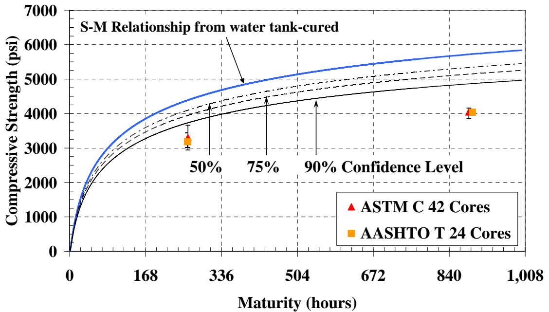
Figure 5-70: Cores with water-tank S-M relationship and confidence levels for the warm-weather placement of mock bridge deck ( E = 33.5 \text{ kJ/mol} )
