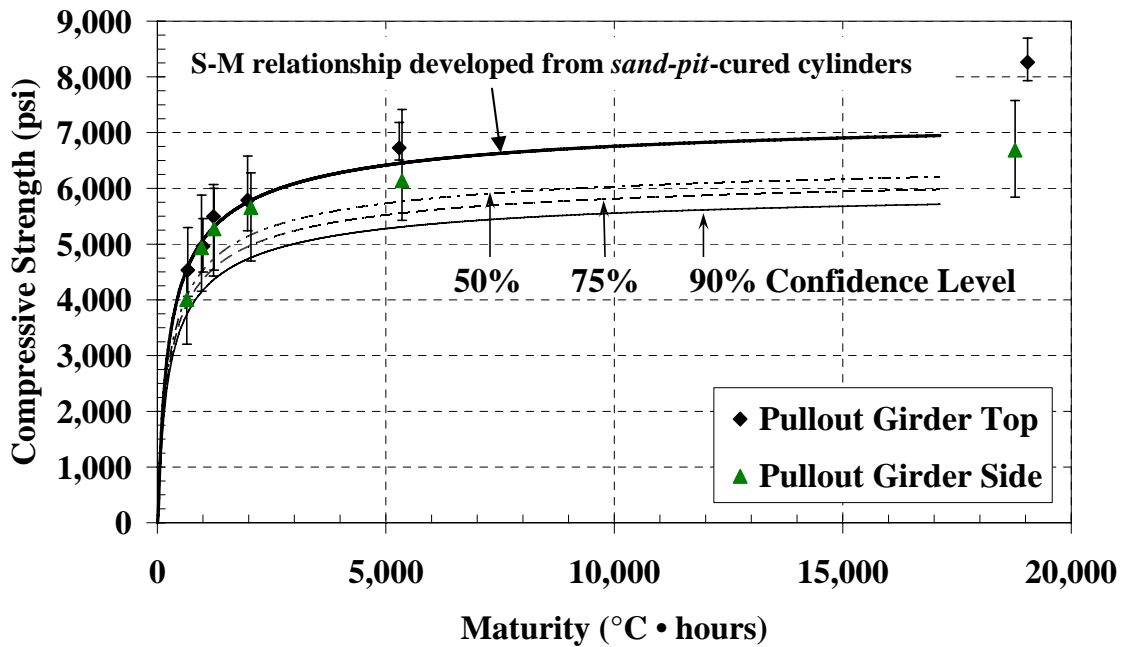
Figure B-33: Pullout test with sand-pit S-M relationship and confidence levels ( T_0 = 0^{\circ}\text{C} )
