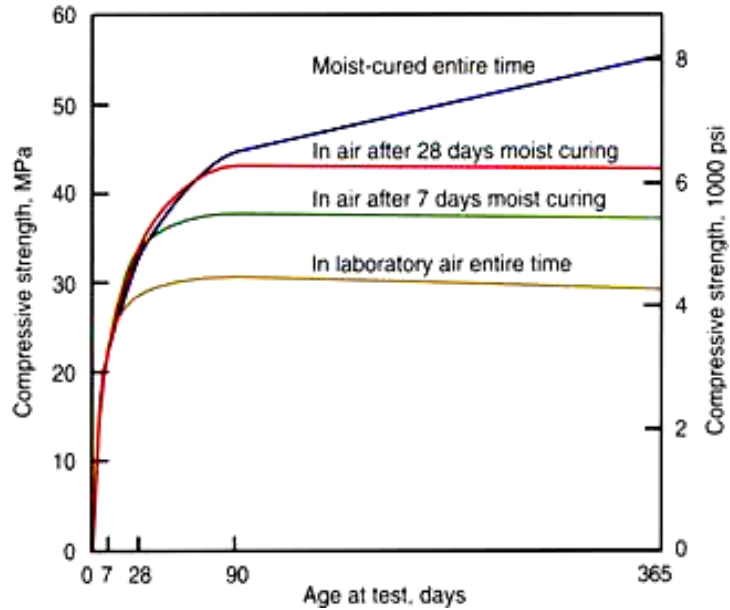
Figure 2-13: Effect of moist-curing time on strength gain of concrete (Gonnerman and Shuman 1928)
