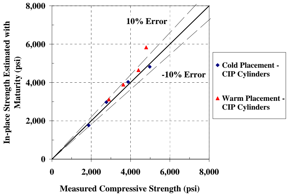
Figure C-87: 45°-line graph for estimating the strength of CIP cylinders on the mock bridge deck using water-tank S-M relationship with Arrhenius maturity function ( E = 40 \text{ kJ/mol} )
