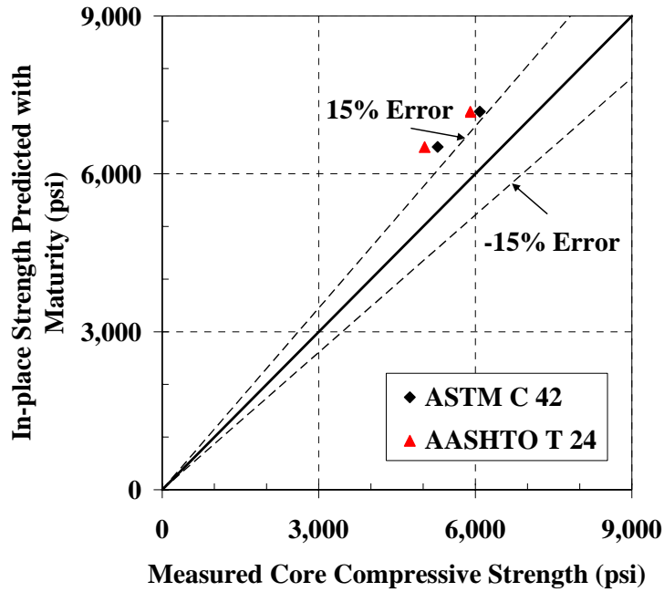
Figure 4-58: 45°-line graph for estimating the strength of cores for the mock girder using water-tank S-M relationship with Arrhenius maturity function ( E = 40 kJ/mol)
