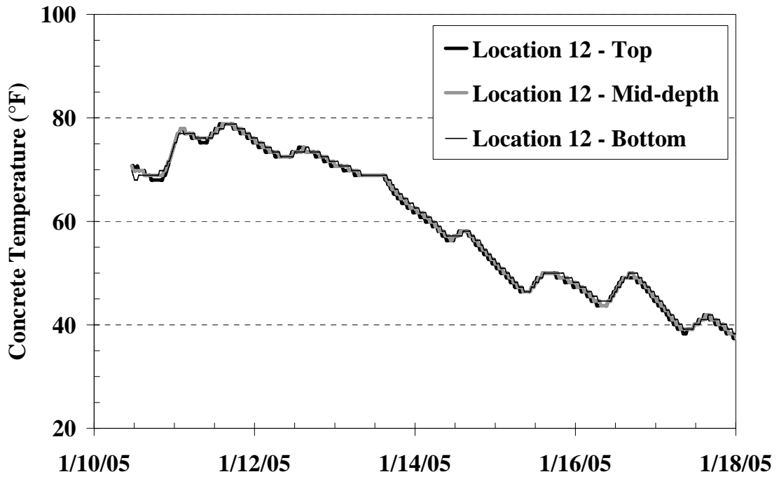
Figure C-64: Temperature history of Location 12 from the I-85 Bridge
