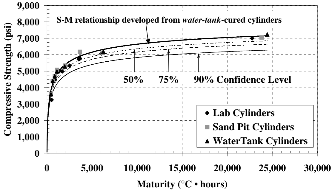
Figure B-20: Water-tank S-M relationship with confidence levels ( T_0 = -10\text{ }^\circ\text{C} )
