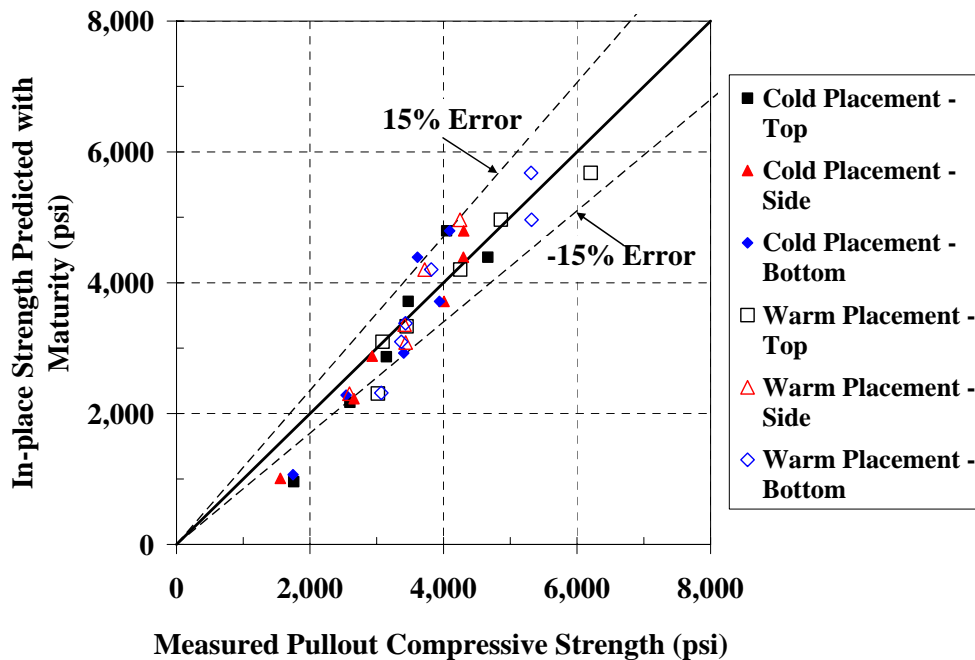
Figure C-82: 45°-line graph for estimating the strength of pullout test on the mock bridge deck using water-tank S-M relationship with Nurse-Saul maturity function ( T_0 = -10 \text{ }^\circ\text{C} )
