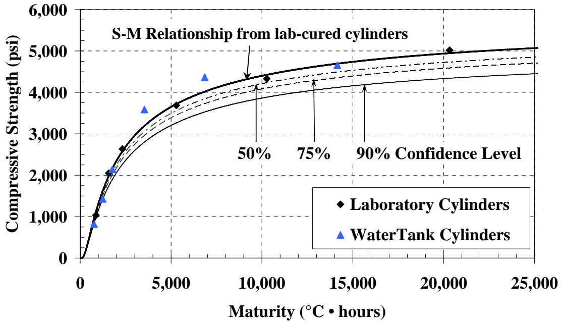
Figure 5-30: S-M relationship for the laboratory cured cylinders with confidence levels for the cold-weather placement of the mock bridge deck ( T_0 = -10^{\circ}\text{C} )
