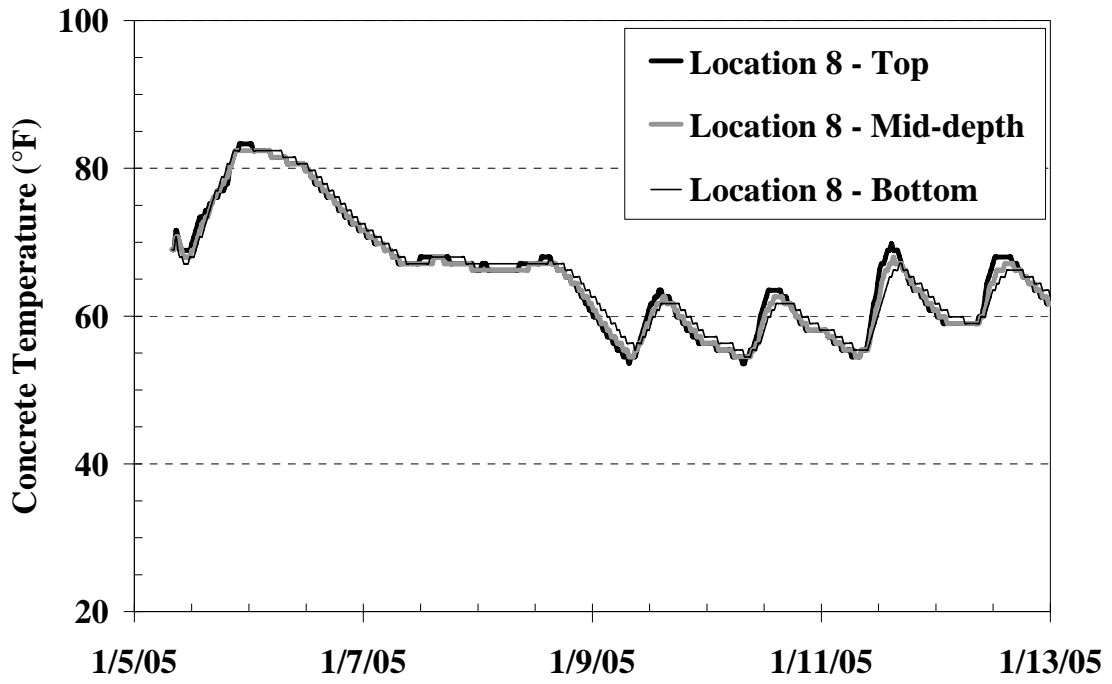
Figure C-60: Temperature history of Location 8 from the I-85 Bridge
