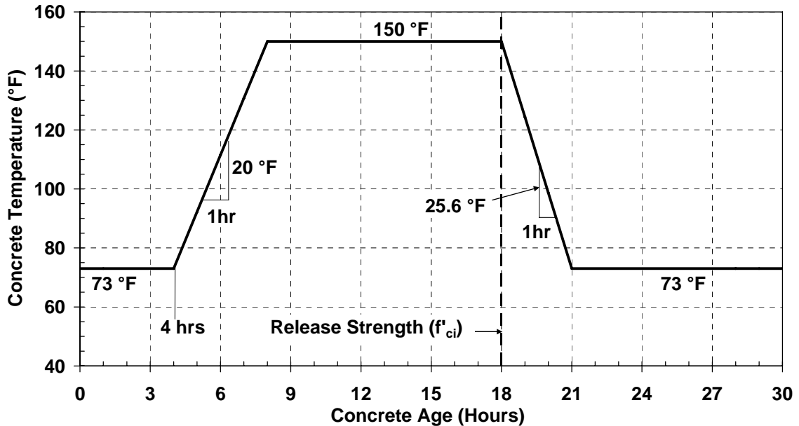
Figure 4-2: Assumed temperature profile for prestressed girder
