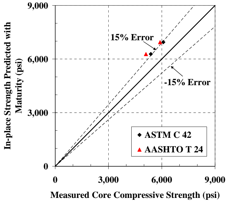
Figure 4-55: 45°-line graph for estimating the strength of cores for the mock girder using laboratory S-M relationship with Nurse-Saul maturity function ( T_0 = 0\text{ }^{\circ}\text{C} )
