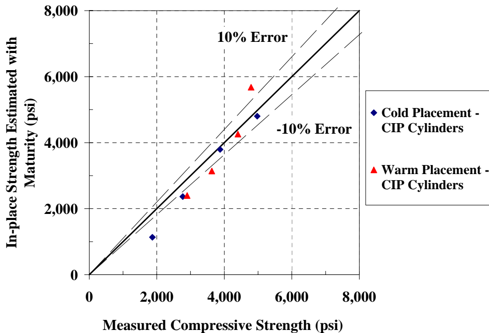
Figure C-86: 45°-line graph for estimating the strength of CIP cylinders on the mock bridge deck using water-tank S-M relationship with Nurse-Saul maturity function ( T_0 = -10 \text{ }^\circ\text{C} )
