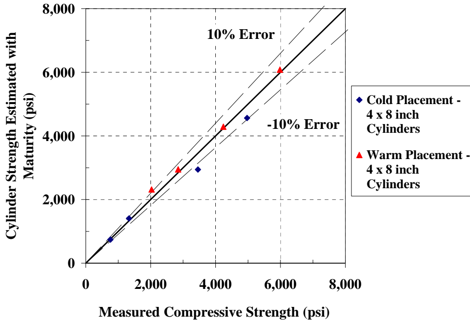
Figure C-75: 45°-line graph for estimating the strength of water-tank-cured 4 x 8 inch cylinder from the mock bridge deck laboratory S-M relationships using the Arrhenius maturity function ( E = 40 \text{ kJ/mol} )
