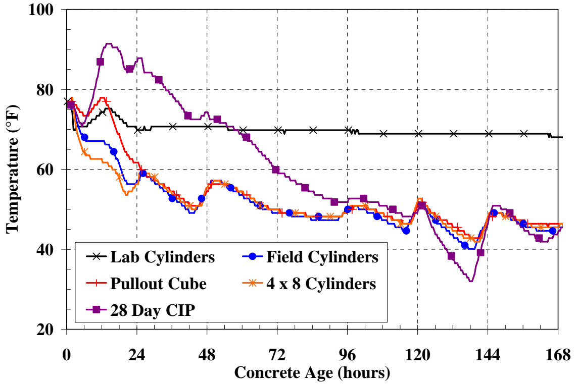
Figure C-3: Molded cylinder temperature history for cold-weather placement of mock bridge deck
