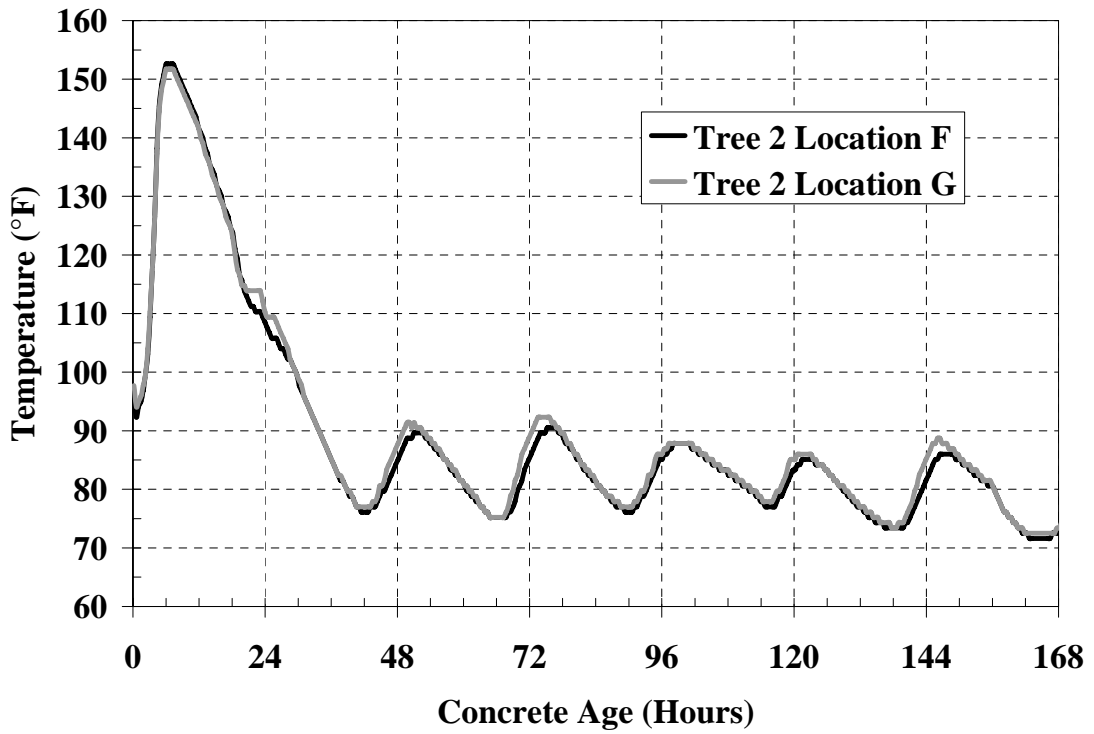
Figure B-9: Girder temperatures Tree 2 Location F and G
