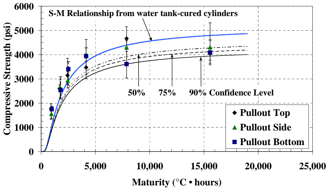
Figure C-16: Pullout test with water-tank S-M relationship and confidence levels for the cold-weather placement of mock bridge deck ( T_o = -10^{\circ}\text{C} )
