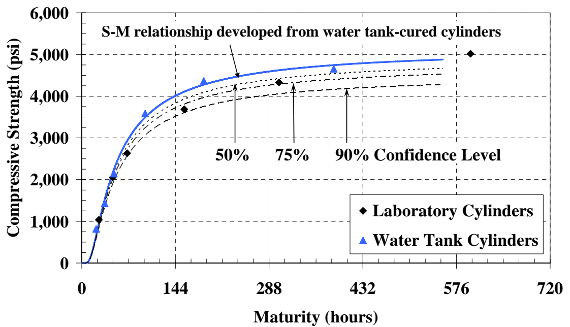
Figure C-12: Water-tank S-M relationship with confidence levels for the cold-weather placement of mock bridge deck ( E = 33.5\text{ kJ/mol} )
