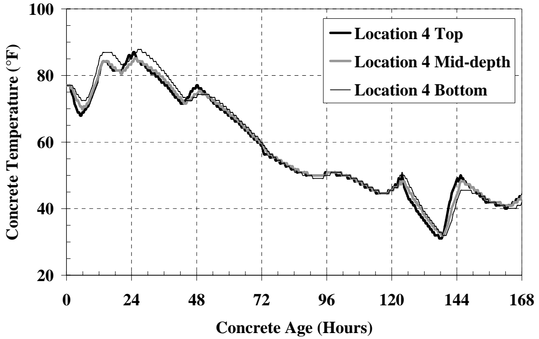
Figure C-7: Mock bridge deck temperatures Location 4 for cold-weather placement
