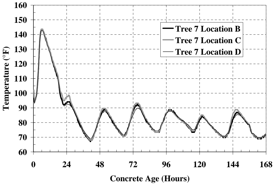
Figure B-17: Girder temperatures Tree 7 Location B, C, and D
