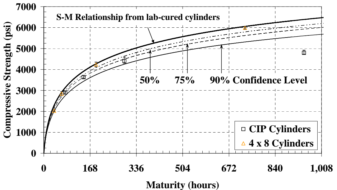
Figure 5-64: Cast-in-place cylinders and 4 x 8 inch cylinders with laboratory S-M relationship and confidence levels for the warm-weather placement of the mock bridge deck ( E = 33.5 \text{ kJ/mol} )
