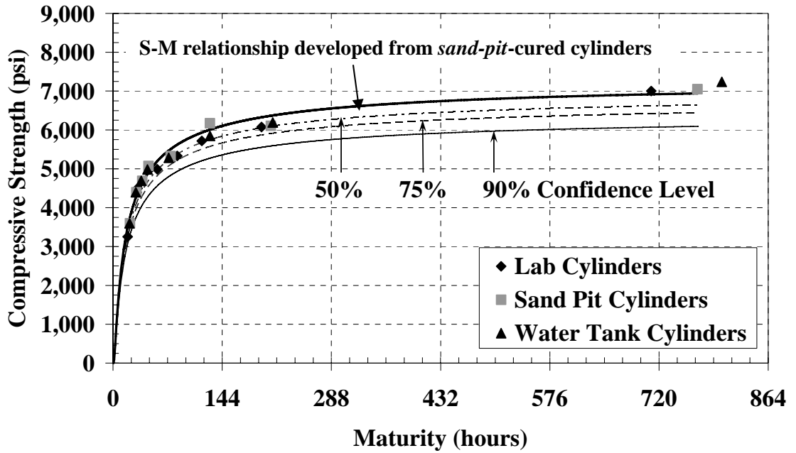
Figure B-26: Sand-pit S-M relationship with confidence levels (E = 33.5 kJ/mol)
