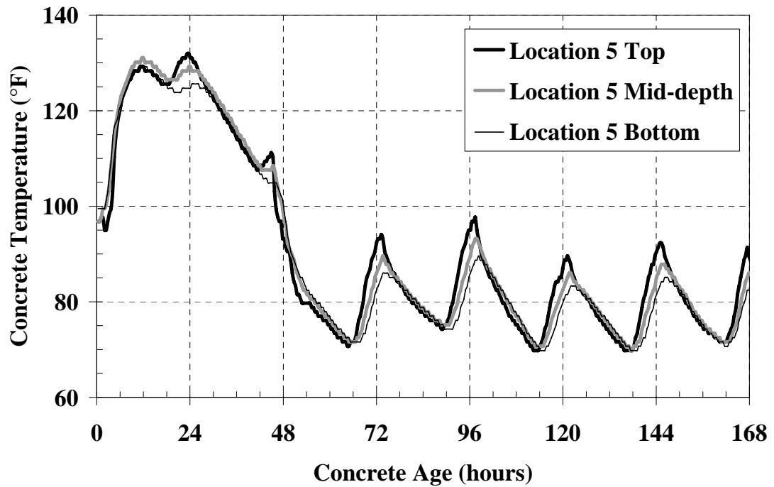
Figure C-33: Mock bridge deck temperatures Location 5 for warm-weather placement
