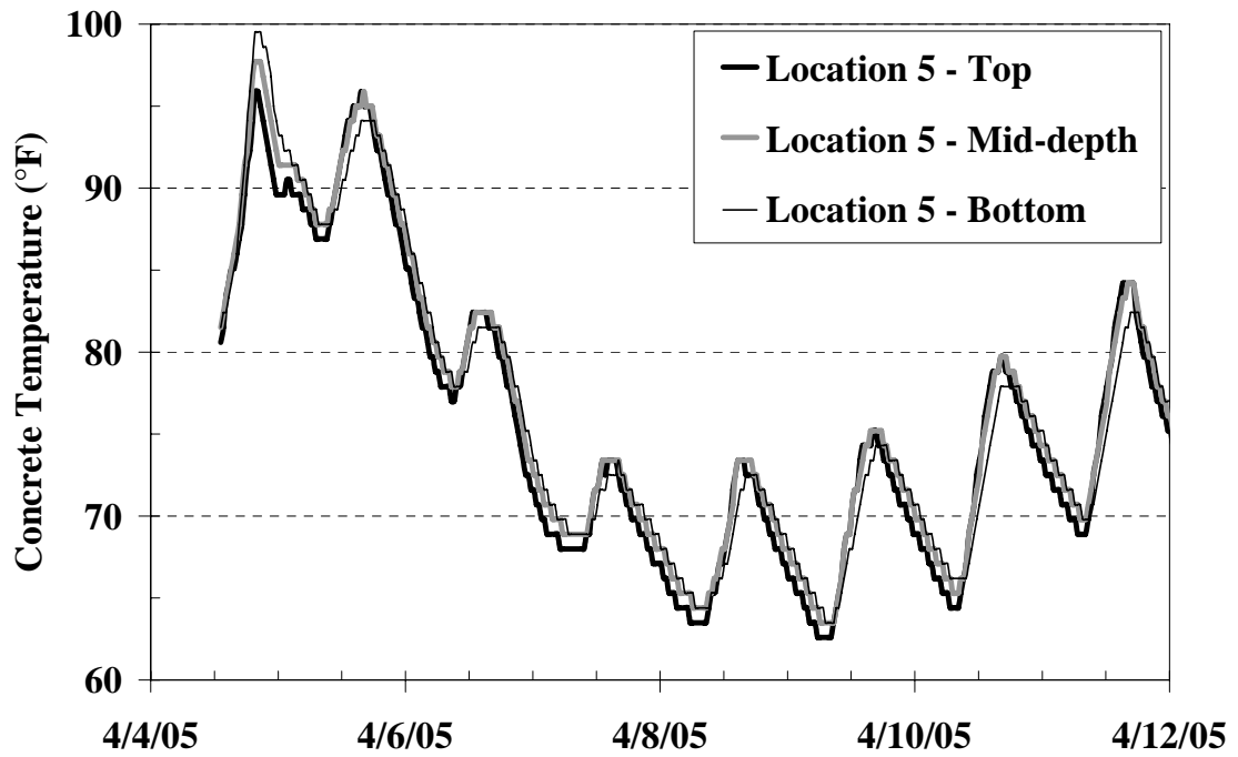
Figure C-73: Temperature history of Location 5 from the Creek Bridge
