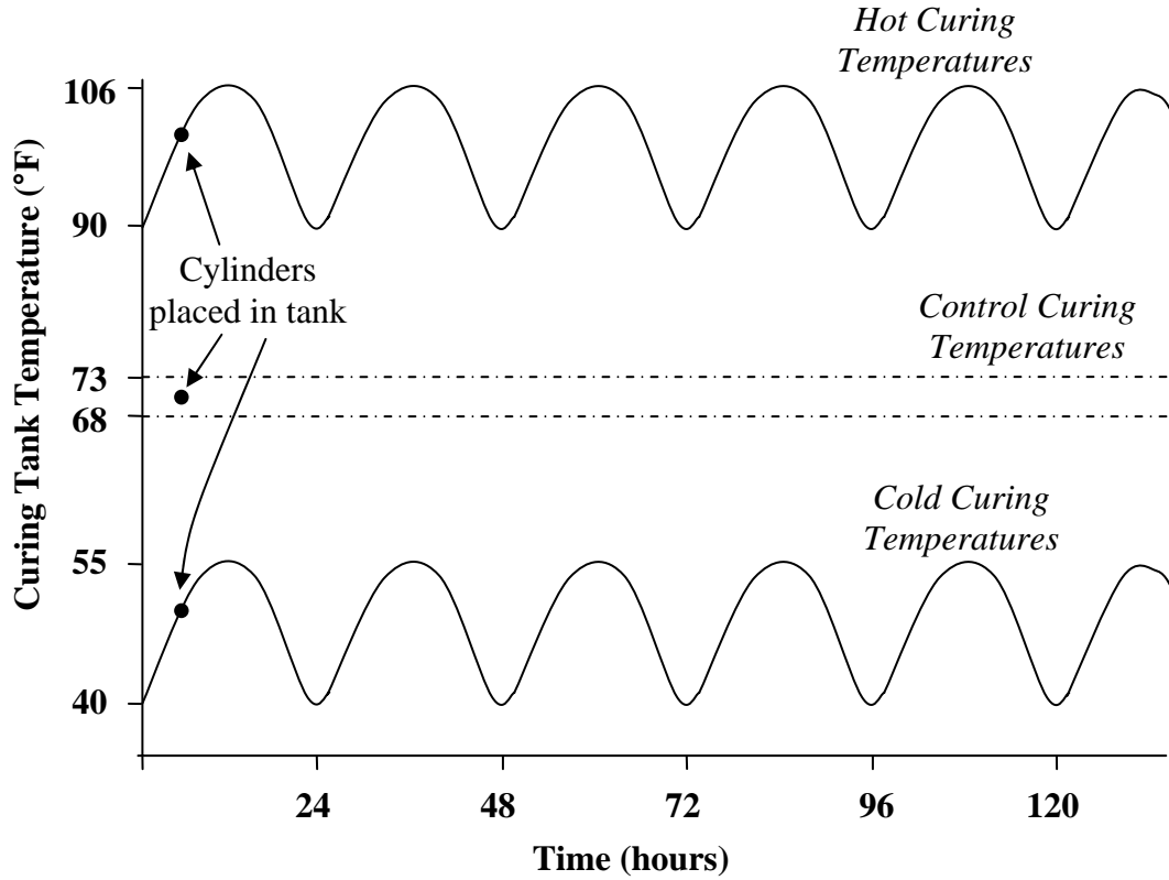
Figure 3-1: Temperature cycles of the three curing methods (Wade 2005)
