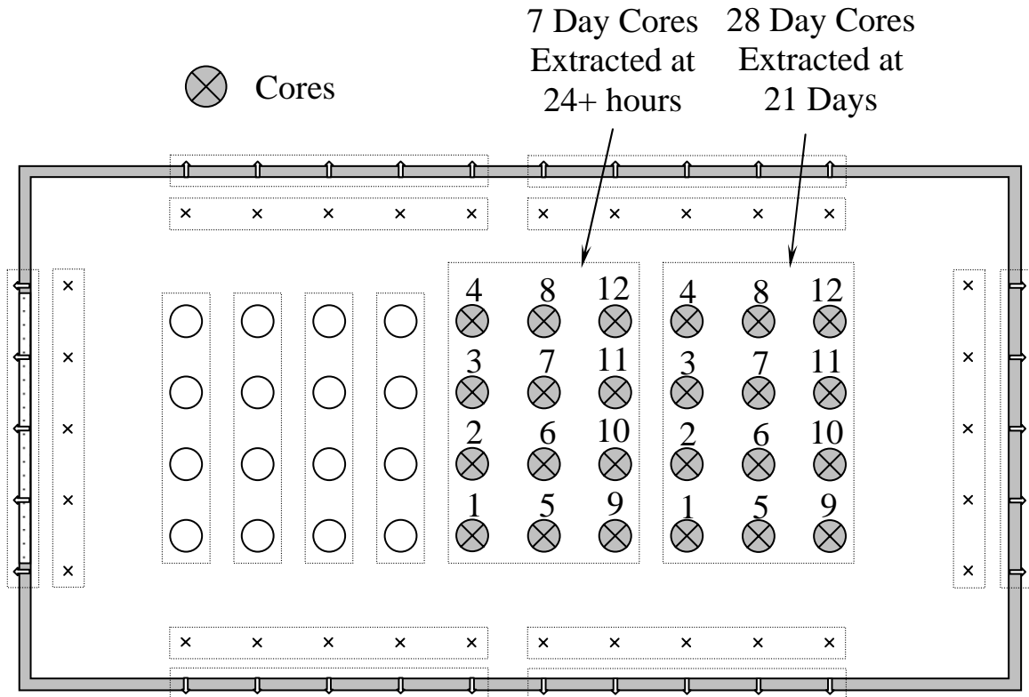
Figure C-26: Top of mock bridge deck core numbering
