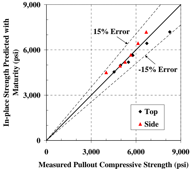
Figure 4-51: 45°-line graph for estimating the strength of pullout test on the mock girder using water-tank S-M relationship with Nurse-Saul maturity function (T o = 0 °C)
