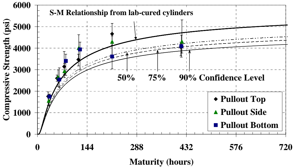
Figure C-15: Pullout test with laboratory S-M relationship and confidence levels for the cold-weather placement of the mock bridge deck ( E = 40 \text{ kJ/mol} )
