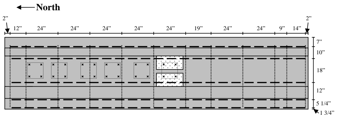
Figure 4-4: Side view of formwork, steel reinforcement, and access panels
