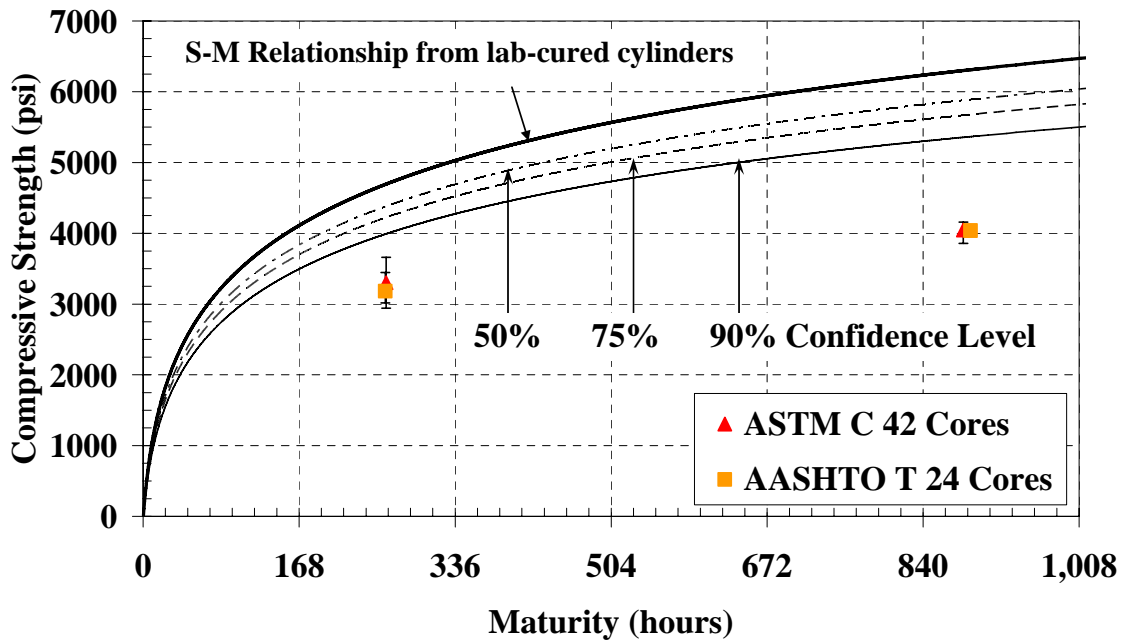
Figure 5-68: Cores with laboratory S-M relationship and confidence levels for the warm-weather placement of the mock bridge deck ( E = 33.5 \text{ kJ/mol} )
