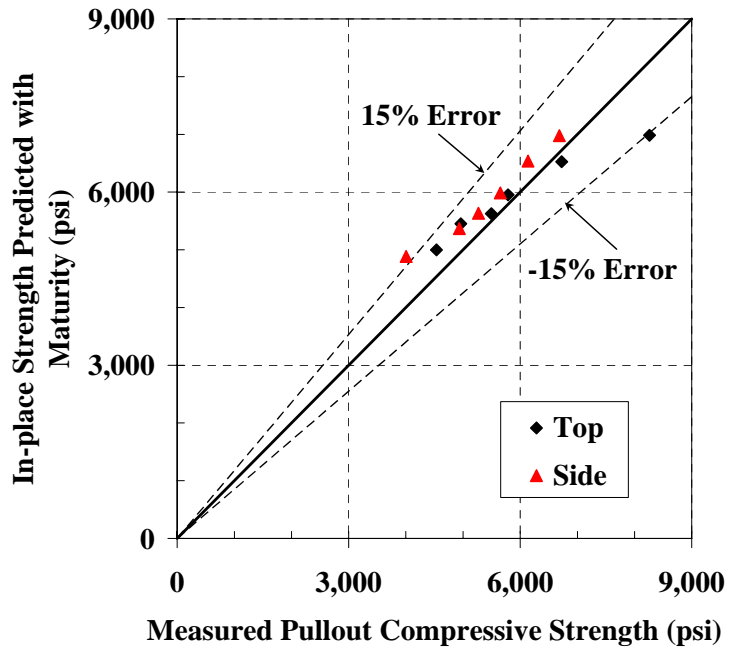
Figure B-51: 45°-line graph for estimating the strength of pullout test on the mock girder using sand-pit S-M relationship with Arrhenius maturity function ( E = 33.5\text{ kJ/mol} )
