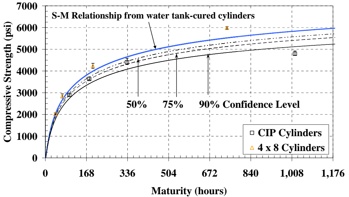
Figure C-46: Cast-in-place cylinders and 4 x 8 inch cylinders with water-tank S-M relationship and confidence levels for the warm-weather placement of mock bridge deck ( E = 40 \text{ kJ/mol} )
