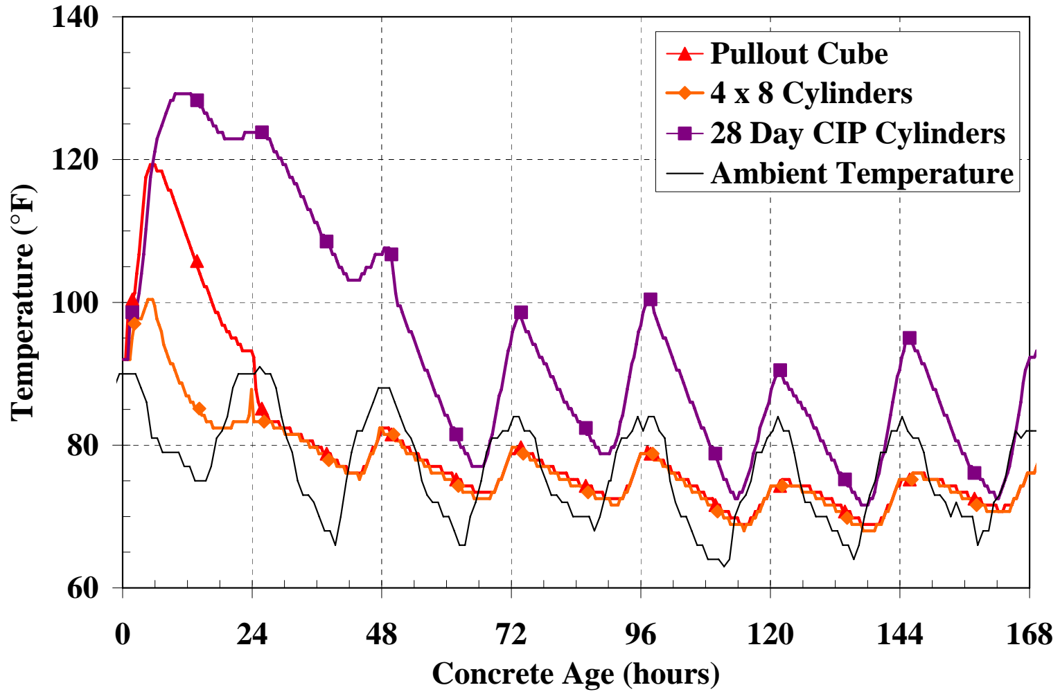
Figure 5-47: Temperature history of pullout cubes, 4 x 8 inch water-tank cylinders, and 28-day CIP cylinders for the warm-weather placement
