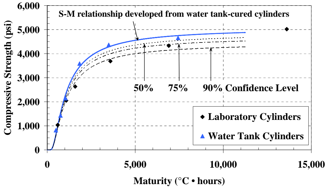
Figure C-11: Water-tank S-M relationship with confidence levels for the cold-weather placement of mock bridge deck ( T_o = 0\text{ }^\circ\text{C} )
