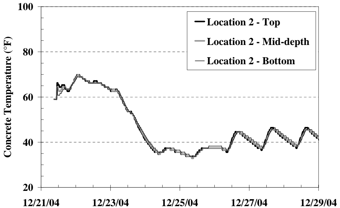
Figure C-53: Temperature history of Location 2 from the I-85 Bridge
