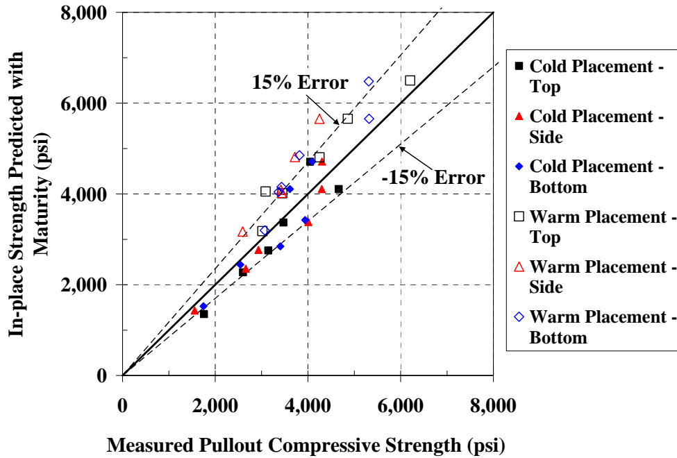
Figure C-81: 45°-line graph for estimating the strength of pullout test on the mock bridge deck using laboratory S-M relationship with Arrhenius maturity function ( E = 40 \text{ kJ/mol} )
