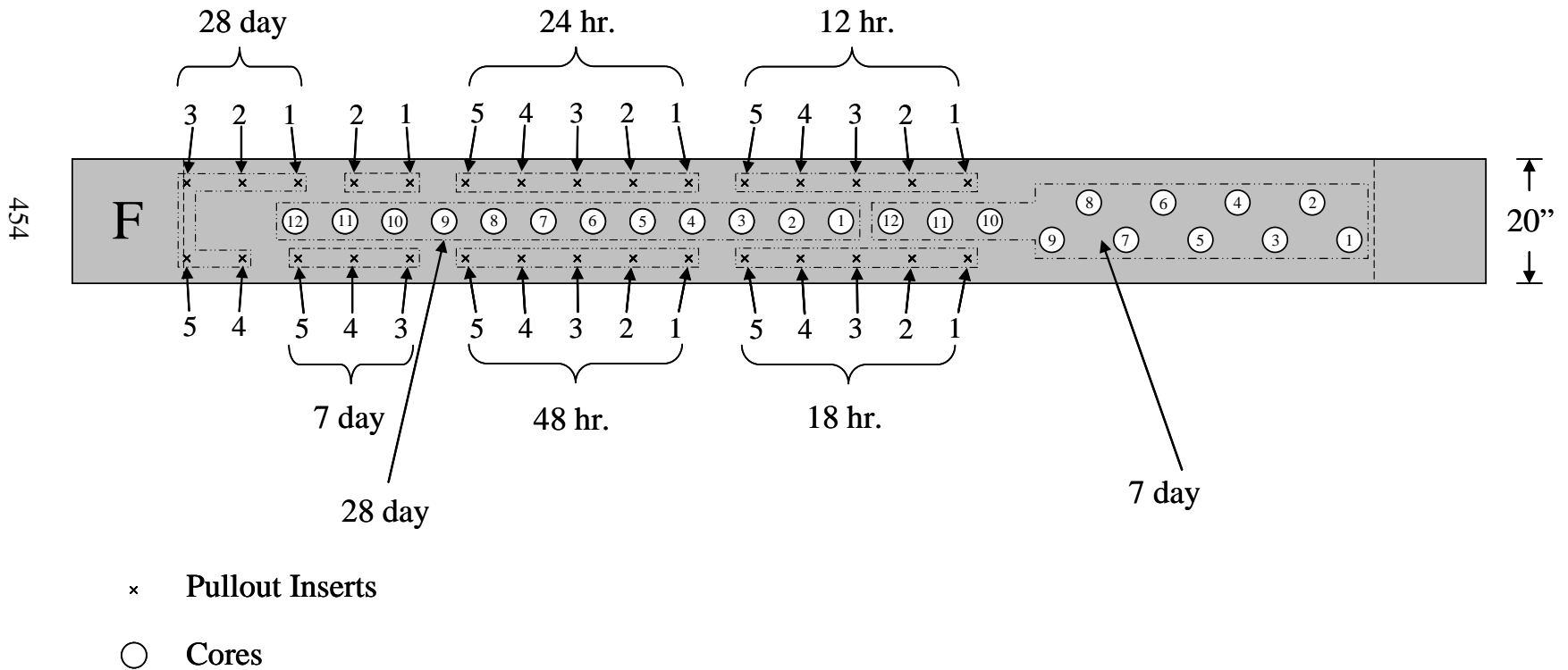
Figure B-2: Top of mock girder cores and pullout inserts layout and numbering
