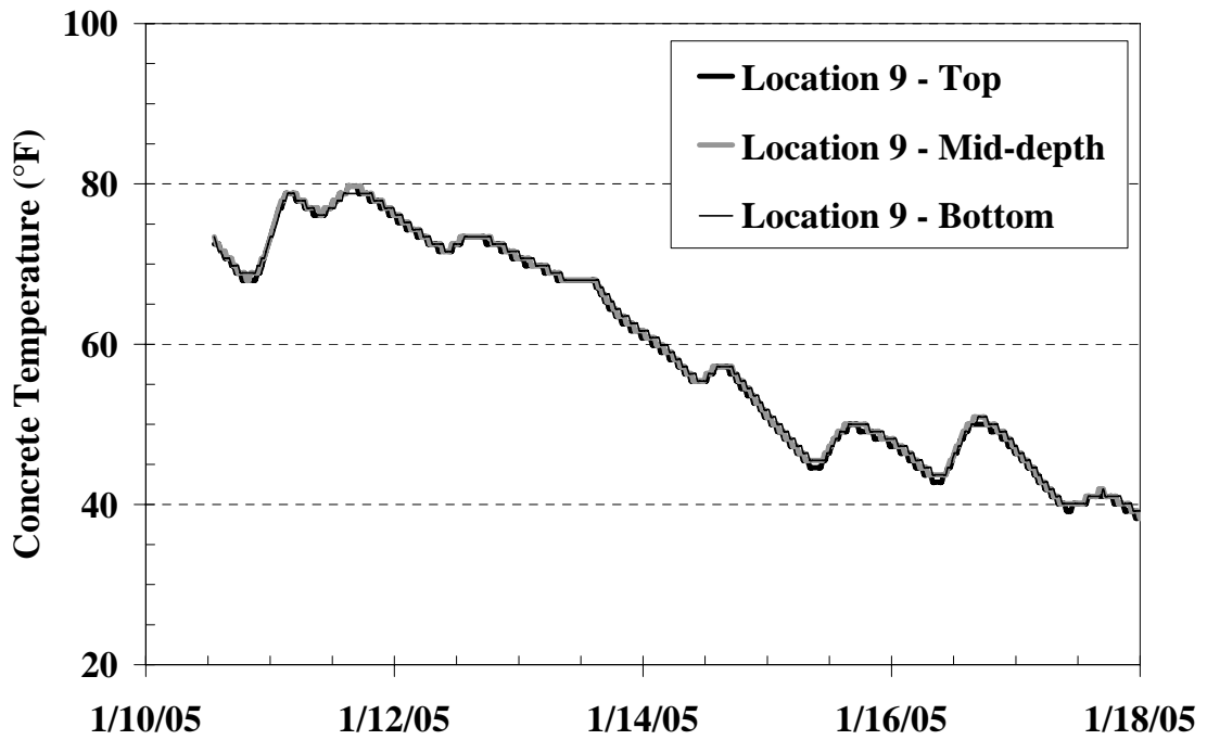
Figure C-61: Temperature history of Location 9 from the I-85 Bridge
