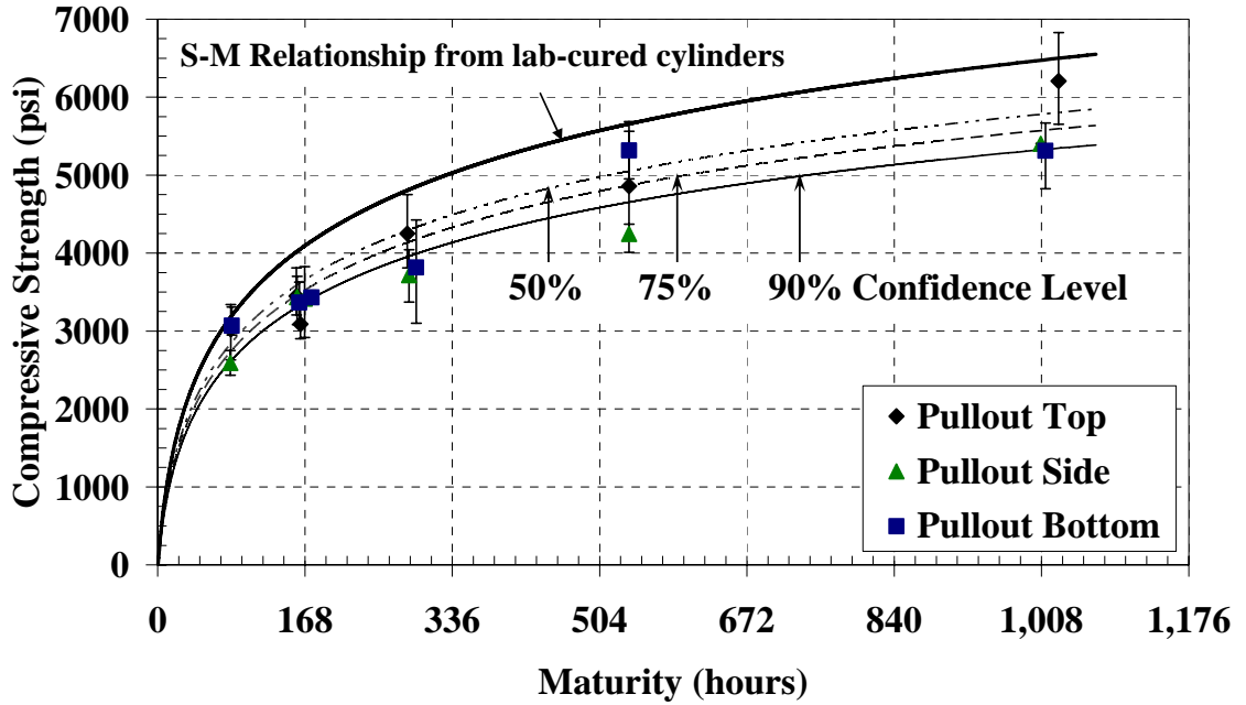
Figure C-40: Pullout test with laboratory S-M relationship and confidence levels for the warm-weather placement of the mock bridge deck ( E = 40 \text{ kJ/mol} )
