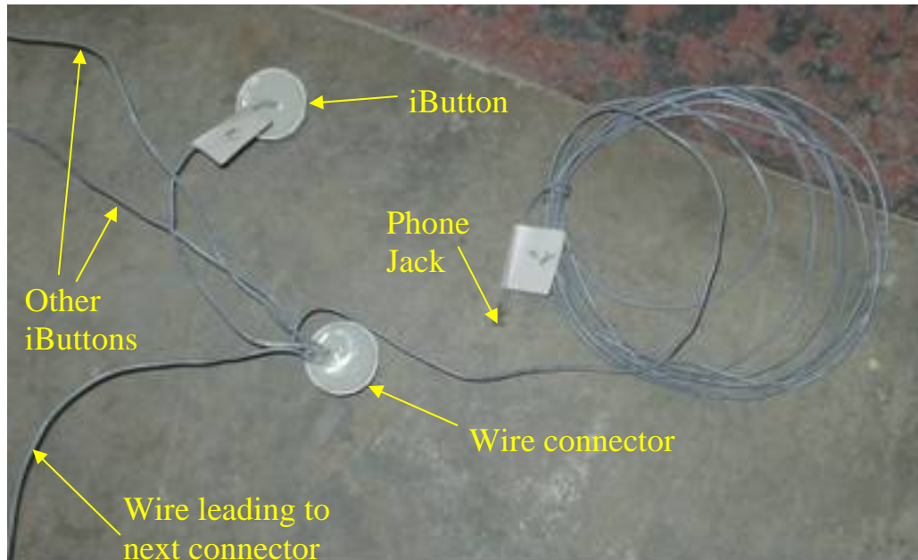
Figure 4-16: iButton tree
