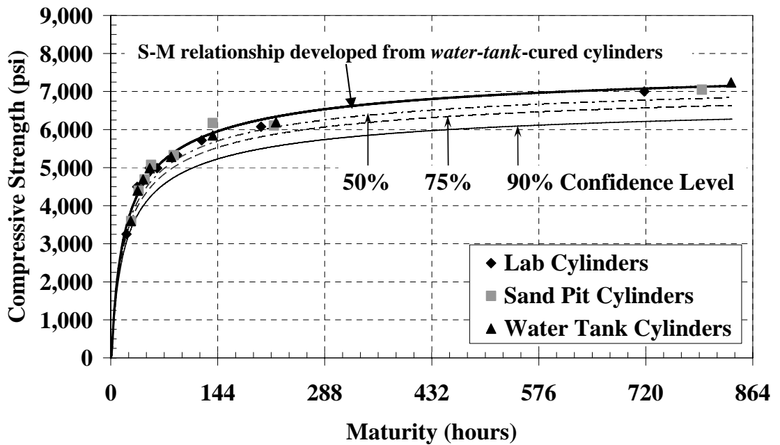
Figure B-23: Water-tank S-M relationship with confidence levels ( E = 40 kJ/mol)
