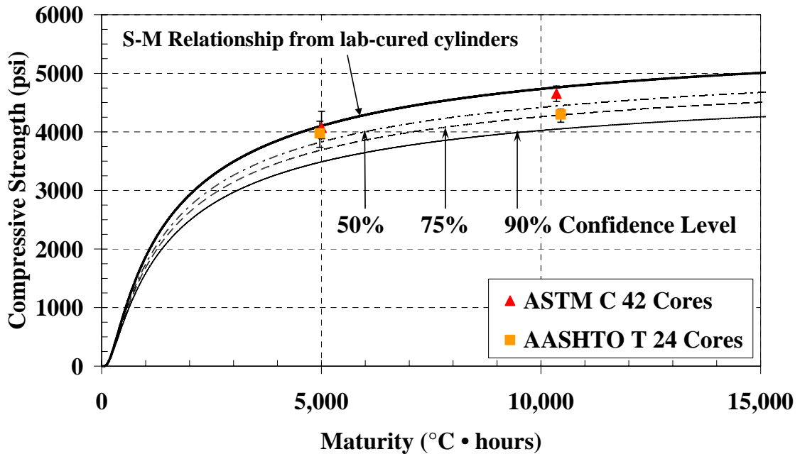
Figure 5-42: Cores with laboratory S-M relationship and confidence levels for the cold-weather placement of the mock bridge deck ( T_o = 0 \text{ }^{\circ}\text{C} )
