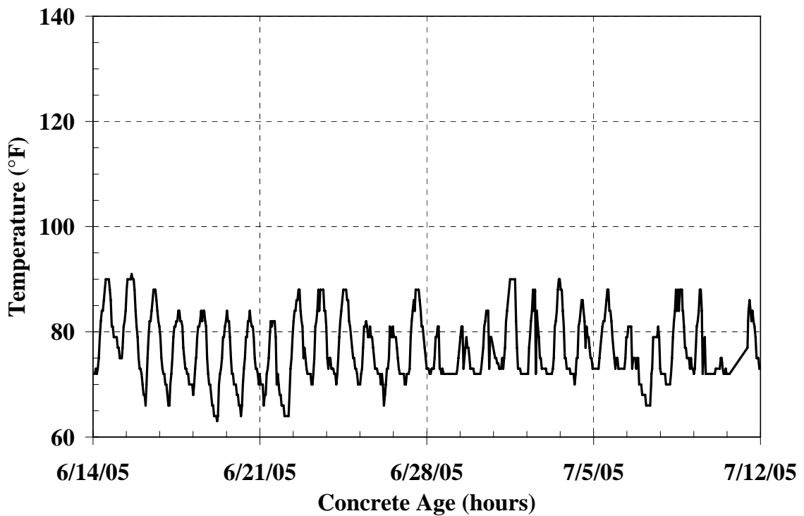
Figure C-27: Ambient air temperatures of the warm-weather placement of mock bridge deck
