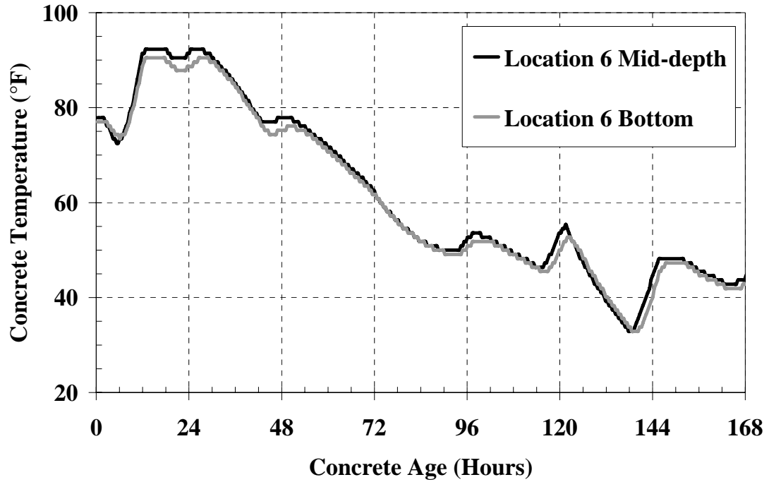
Figure C-9: Mock bridge deck temperatures Location 6 for cold-weather placement
