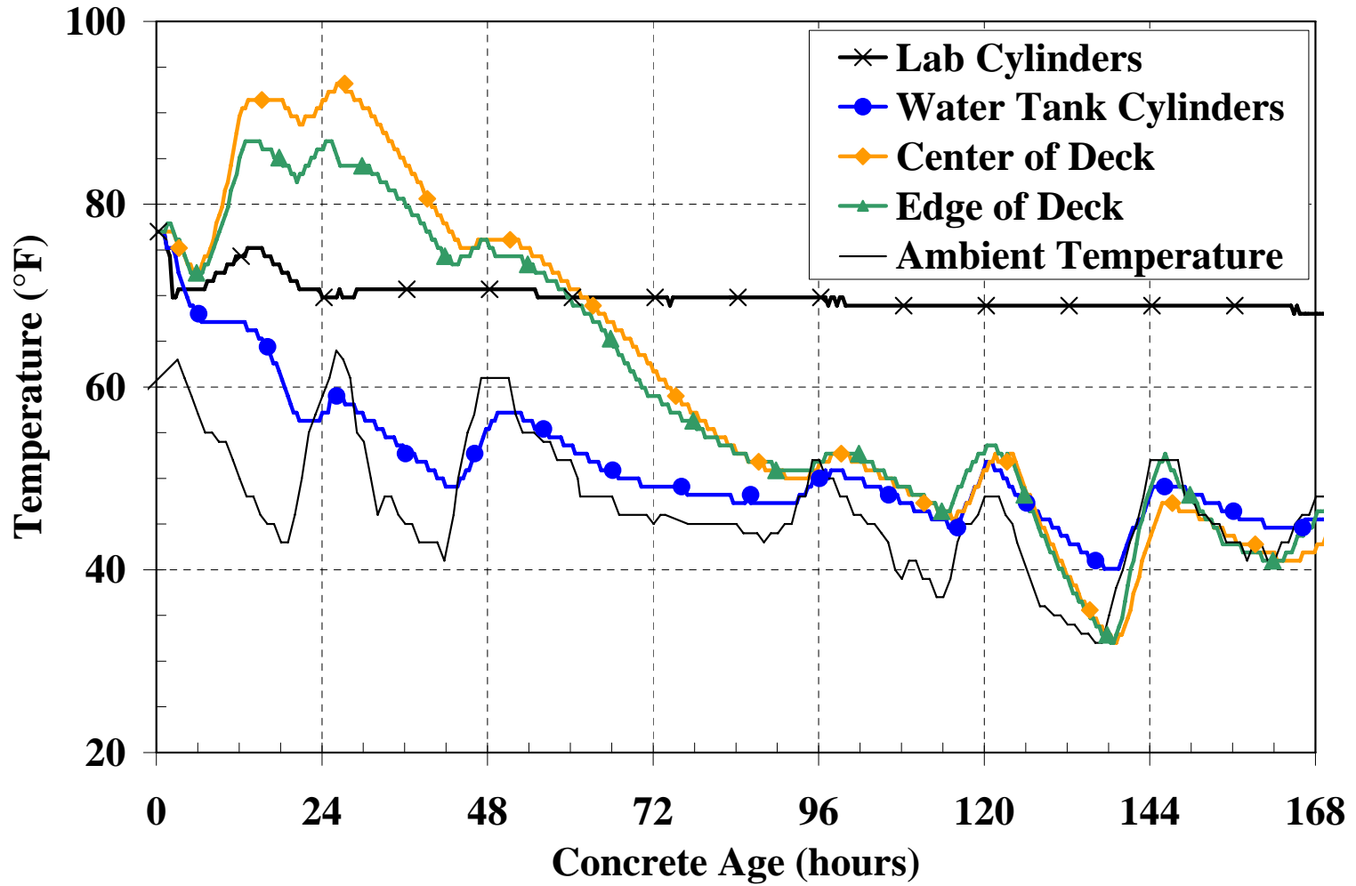
Figure 5-21: Temperature history of 6 x 12 inch cylinders and the mock bridge deck for the cold-weather placement
