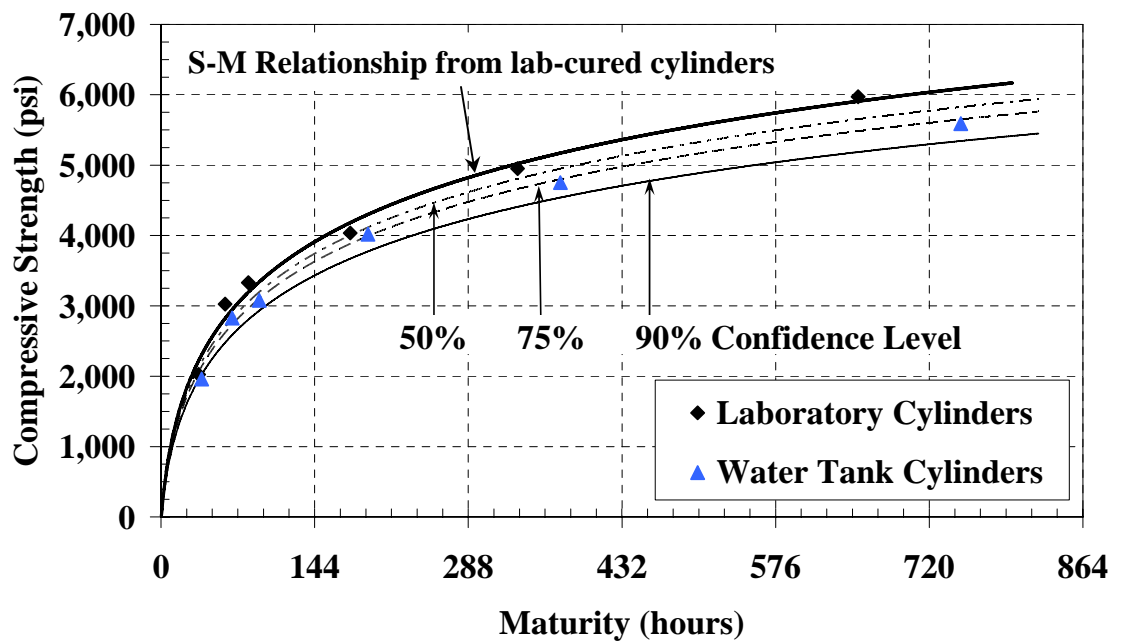
Figure 5-57: S-M relationship for the Laboratory cured cylinders with confidence levels for the warm-weather placement of the mock bridge deck ( E = 33.5 \text{ kJ/mol} )
