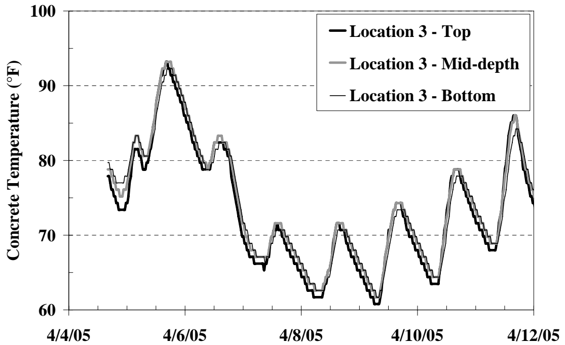
Figure C-71: Temperature history of Location 3 from the Creek Bridge
