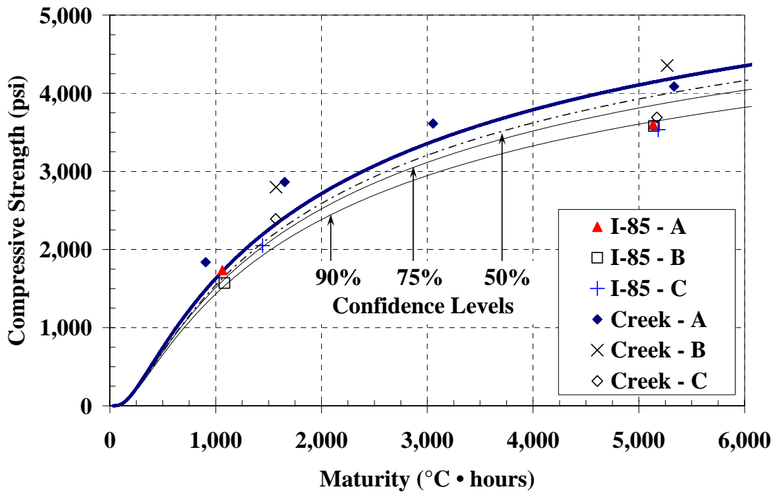
Figure 5-84: I-85 Bridge S-M relationship with confidence levels and verification test results ( T_o = -10\text{ }^\circ\text{C} )
