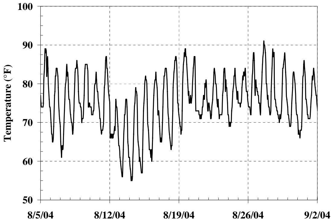
Figure B-3: Ambient air temperatures of the prestressed plant project
