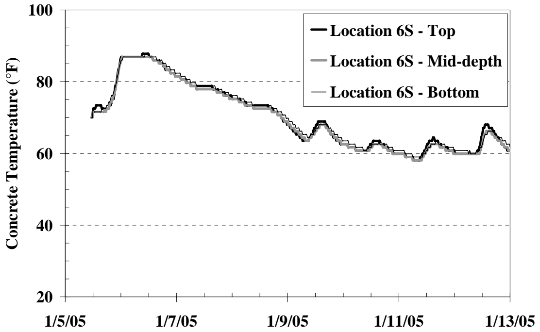
Figure C-58: Temperature history of Location 6S from the I-85 Bridge
