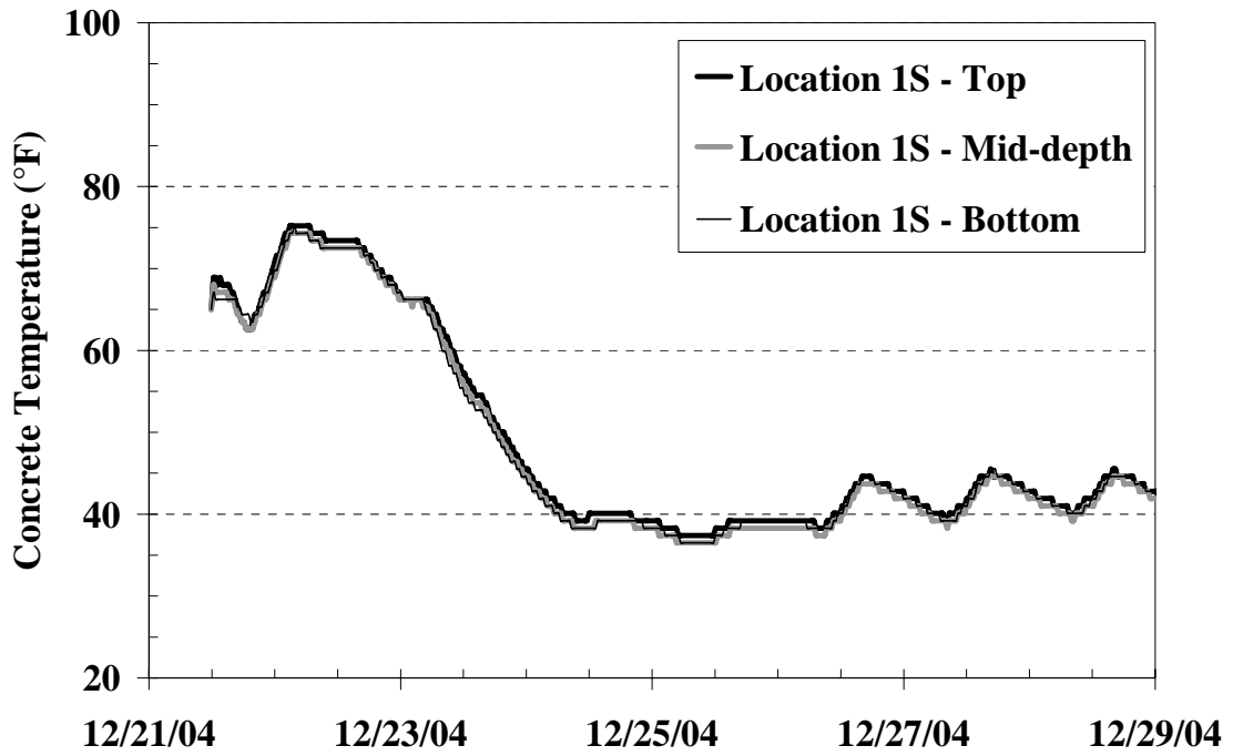
Figure C-52: Temperature history of Location 1S from the I-85 Bridge
