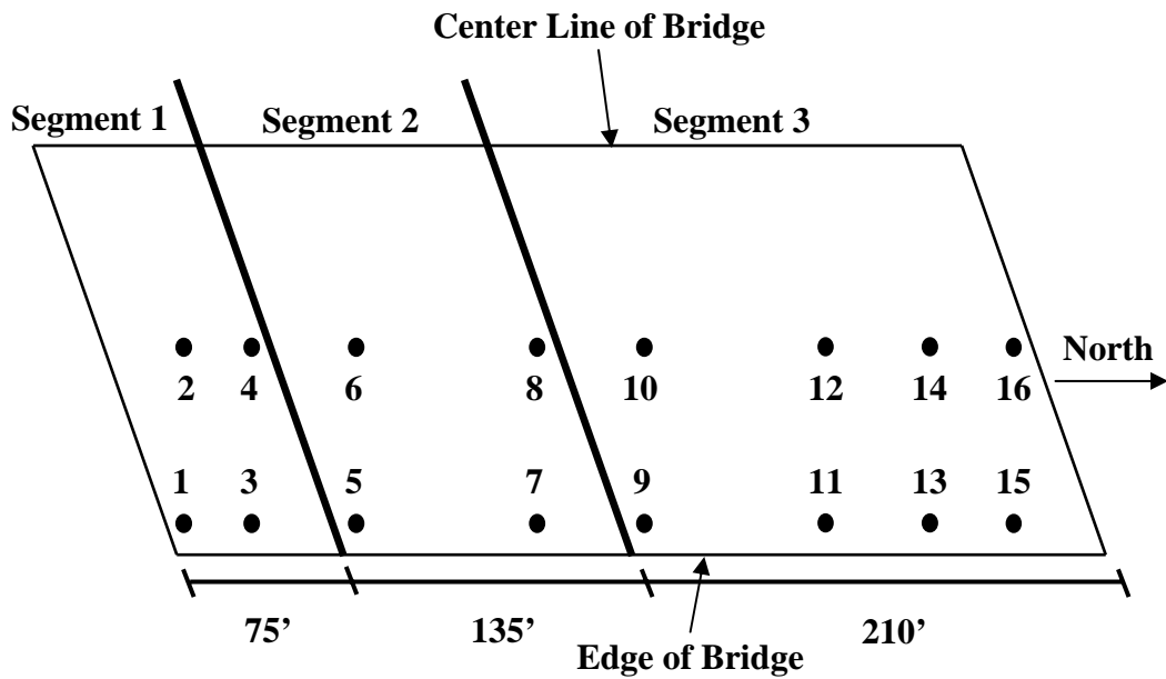
Figure 5-7: Temperature sensor layout for the I-85 Bridge
