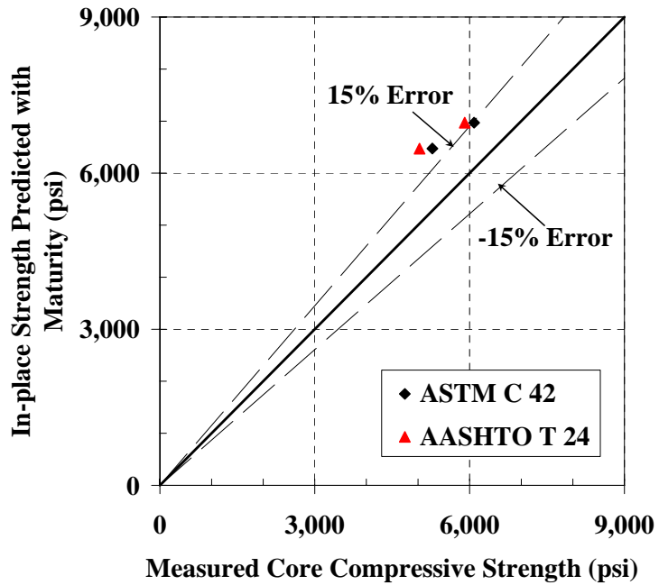
Figure B-57: 45°-line graph for estimating the strength of cores for the mock girder using sand-pit S-M relationship with Arrhenius maturity function ( E = 33.5\text{ kJ/mol} )
