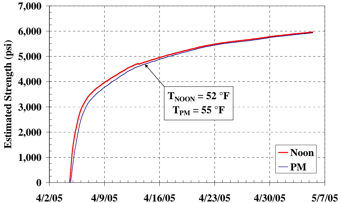
Figure 5-95: Creek Bridge deck strength development using Arrhenius maturity function with E = 40 \text{ kJ/mol}
