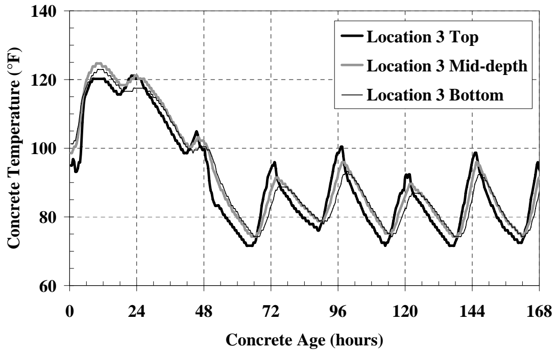
Figure C-31: Mock bridge deck temperatures Location 3 for warm-weather placement
