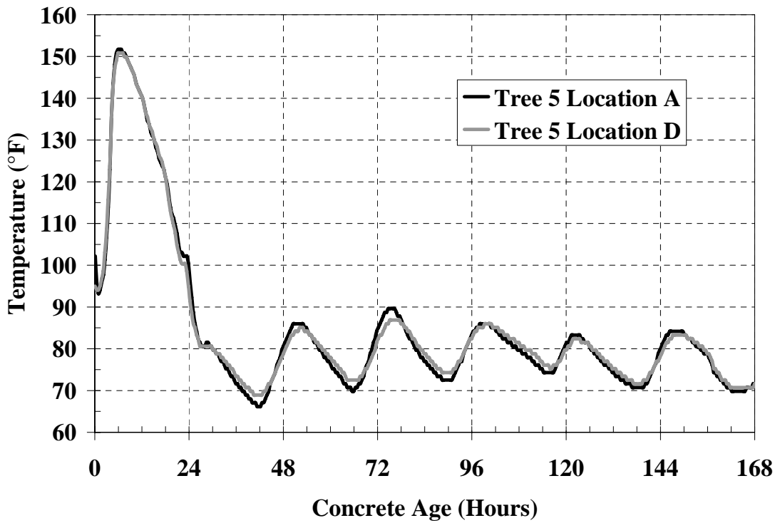
Figure B-15: Girder temperatures Tree 5 Location A and D
