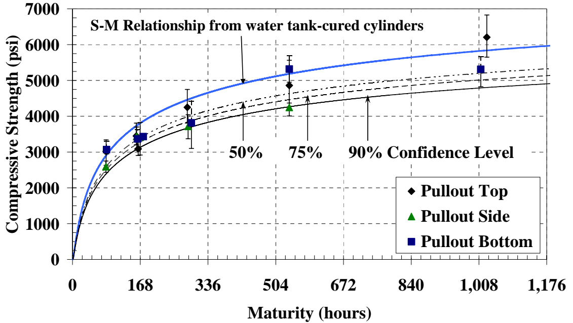
Figure C-42: Pullout test with water-tank S-M relationship and confidence levels for the warm-weather placement of mock bridge deck ( E = 40 \text{ kJ/mol} )
