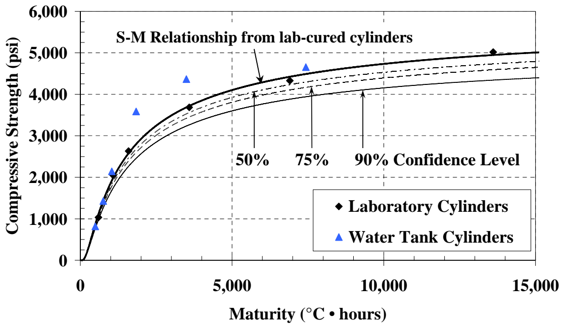
Figure 5-31: S-M relationship for the laboratory cured cylinders with confidence levels for the cold-weather placement of the mock bridge deck ( T_0 = 0^{\circ}\text{C} )
