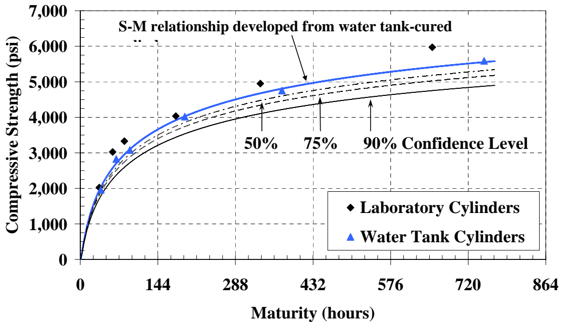
Figure C-37: Water-tank cylinders S-M relationship with confidence levels for the warm-weather placement of mock bridge deck ( E = 33.5 \text{ kJ/mol} )
