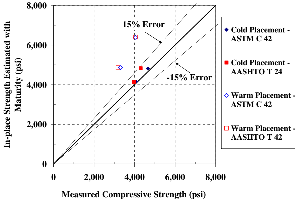
Figure C-89: 45°-line graph for estimating the strength of cores for the mock bridge deck using laboratory S-M relationship with Arrhenius maturity function ( E = 40 \text{ kJ/mol} )
