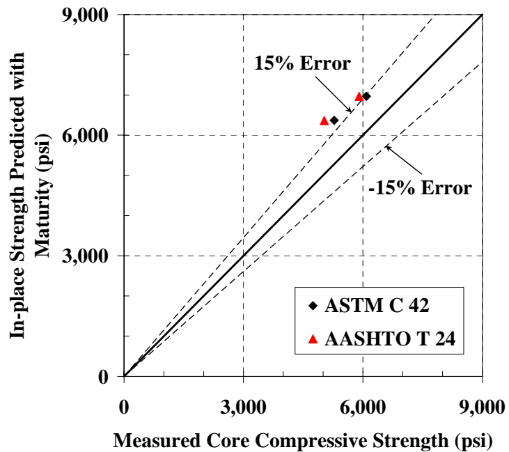
Figure B-53: 45°-line graph for estimating the strength of cores for the mock girder using laboratory S-M relationship with Arrhenius maturity function ( E = 33.5\text{ kJ/mol} )
