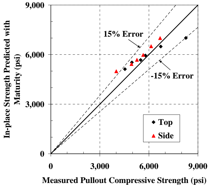
Figure 4-50: 45°-line graph for estimating the strength of pullout test on the mock girder using laboratory S-M relationship with Arrhenius maturity function ( E = 40 kJ/mol)
