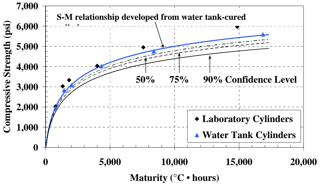
Figure C-36: Water-tank cylinders S-M relationship with confidence levels for the warm-weather placement of mock bridge deck ( T_o = 0^{\circ}\text{C} )
