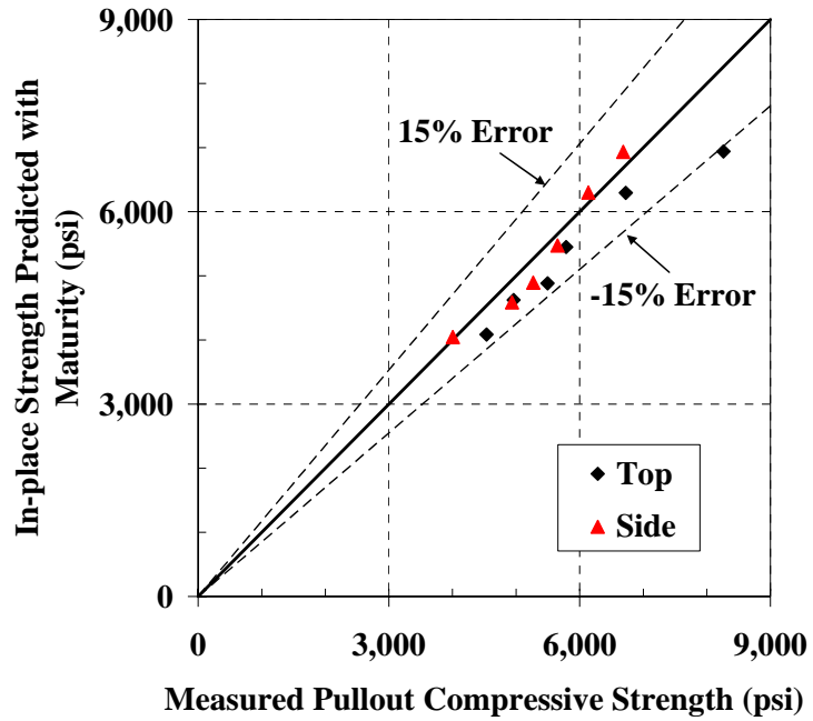
Figure B-46: 45°-line graph for estimating the strength of pullout test on the mock girder using laboratory S-M relationship with Nurse-Saul maturity function ( T_0 = -10\text{ }^\circ\text{C} )
