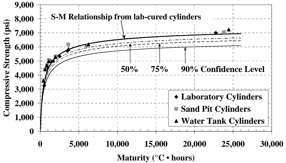
Figure 4-31: Laboratory S-M relationship with confidence levels ( T_0 = -10\text{ }^\circ\text{C} )
