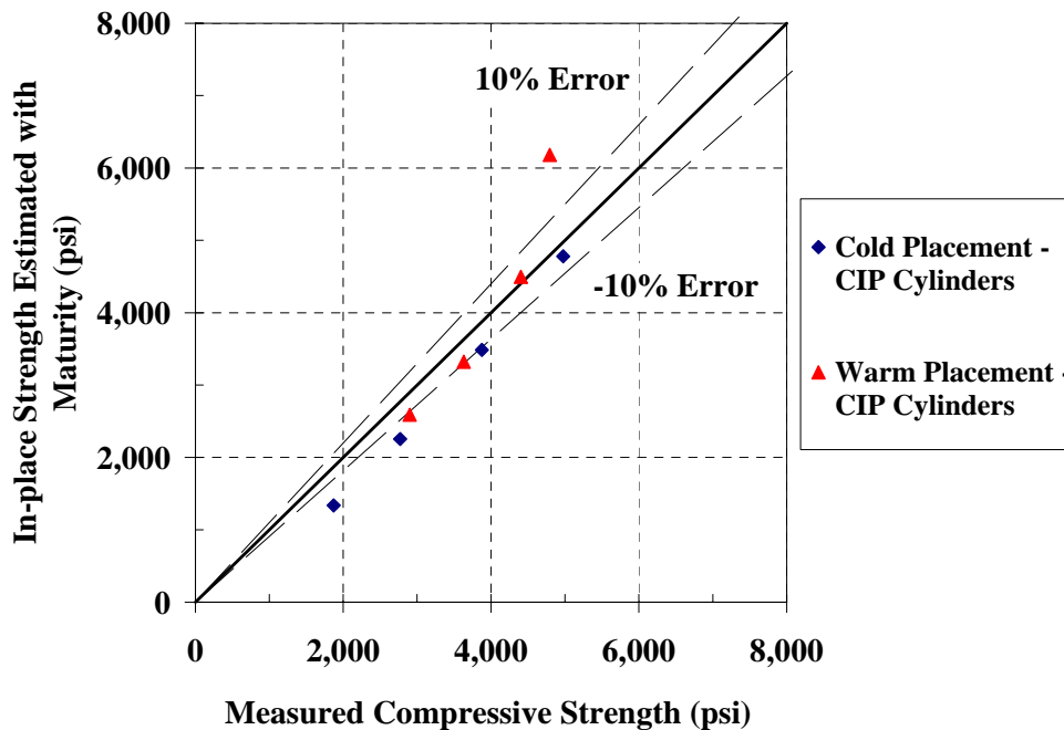
Figure C-84: 45°-line graph for estimating the strength of CIP cylinders on the mock bridge deck using Laboratory S-M relationship with Nurse-Saul maturity function ( T_0 = -10 \text{ }^\circ\text{C} )
