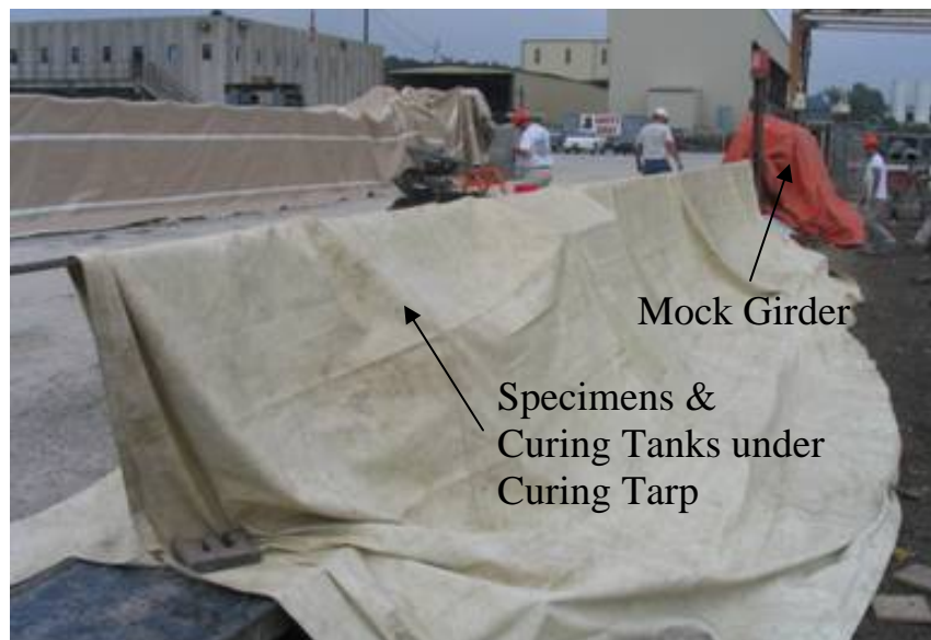
Figure 4-10: Curing tarp over the specimens and mock girder
