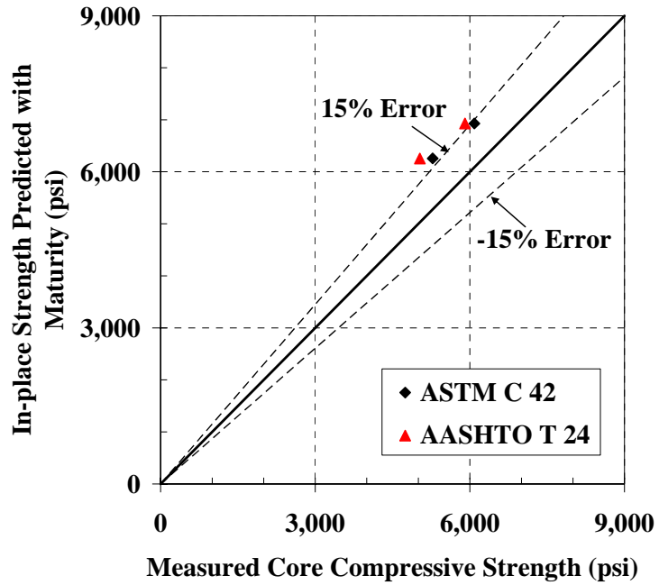
Figure B-52: 45°-line graph for estimating the strength of cores for the mock girder using laboratory S-M relationship with Nurse-Saul maturity function test ( T_0 = -10\text{ }^\circ\text{C} )
