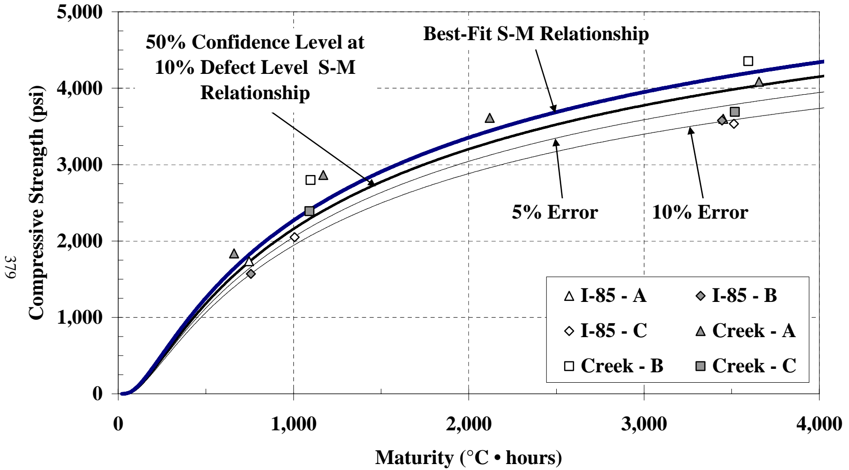
Figure 5-132: Applying a confidence level and acceptance criteria to the verification test results
