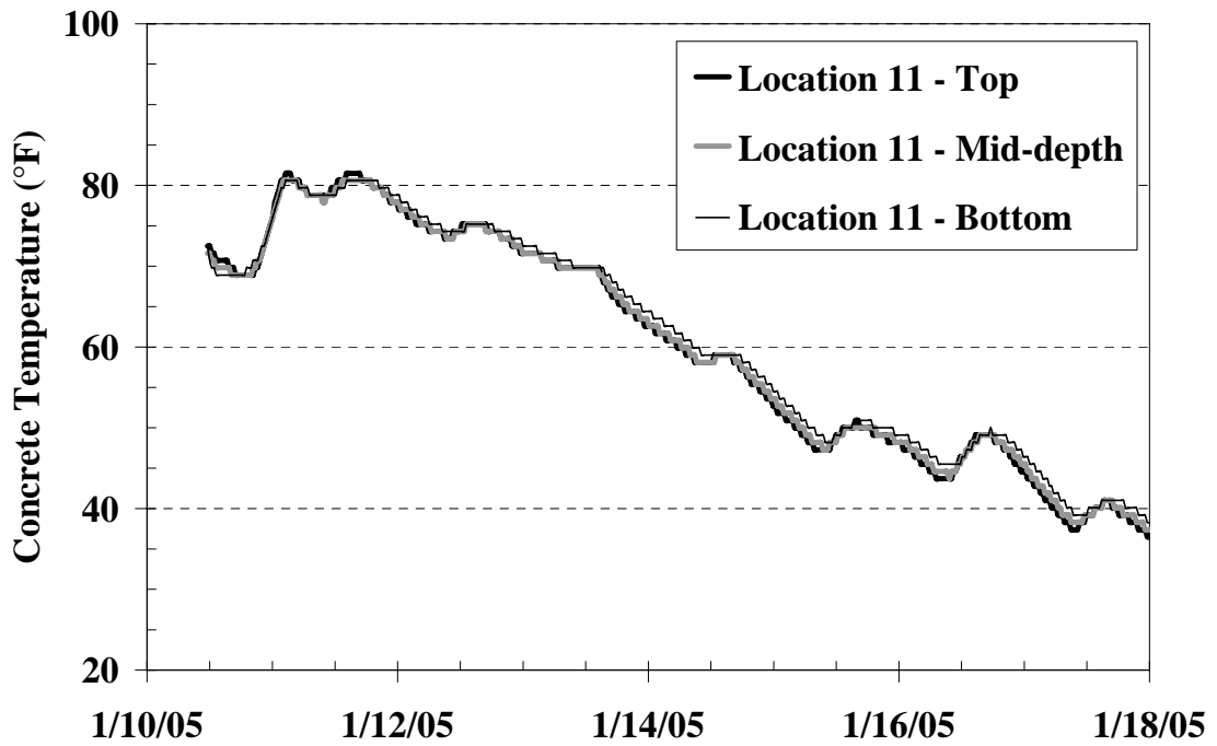
Figure C-63: Temperature history of Location 11 from the I-85 Bridge
