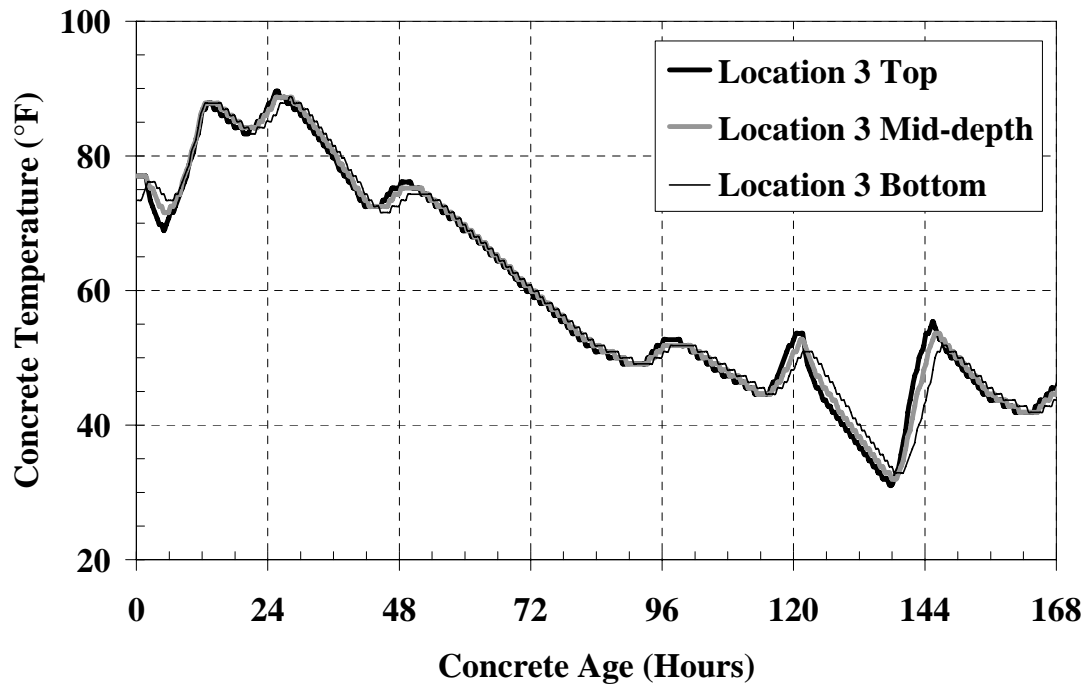
Figure C-6: Mock bridge deck temperatures Location 3 for cold-weather placement
