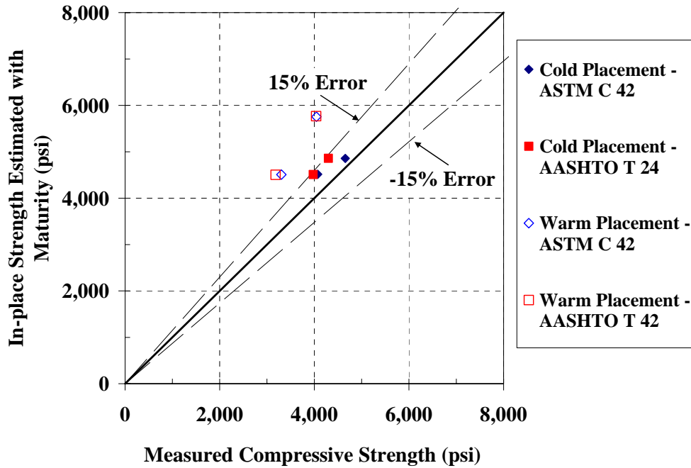
Figure C-91: 45°-line graph for estimating the strength of cores for the mock bridge deck using water-tank S-M relationship with Arrhenius maturity function ( E = 40 \text{ kJ/mol} )
