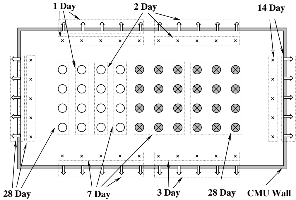
Top Layout
