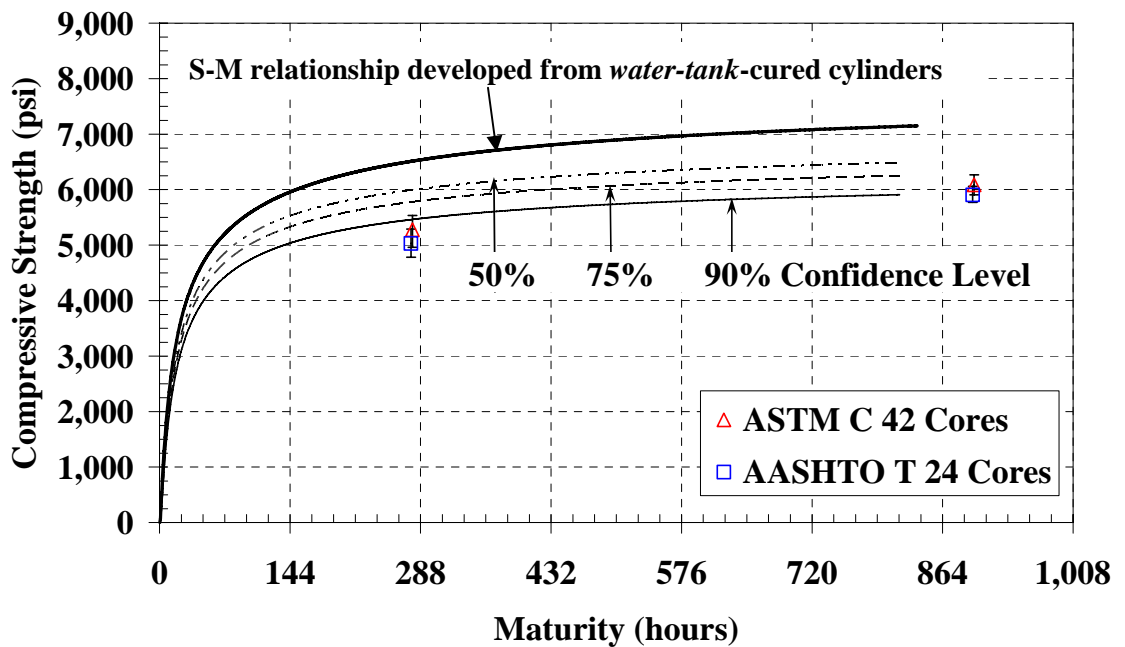
Figure B-39: Cores with water-tank S-M relationship and confidence levels ( E = 40 kJ/mol)
