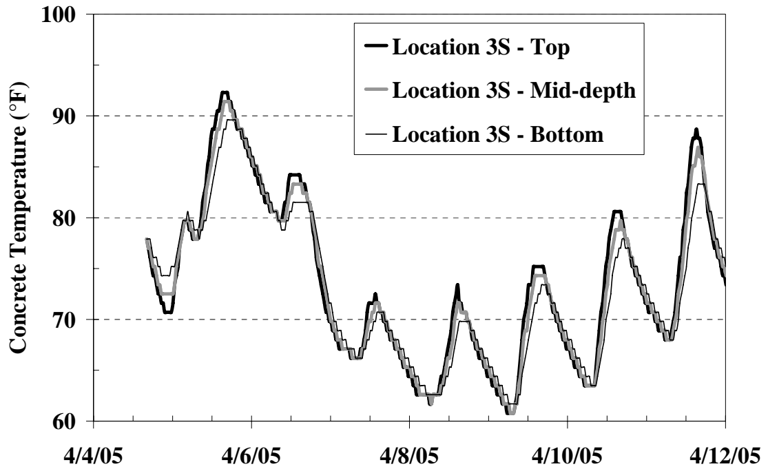
Figure C-72: Temperature history of Location 3S from the Creek Bridge
