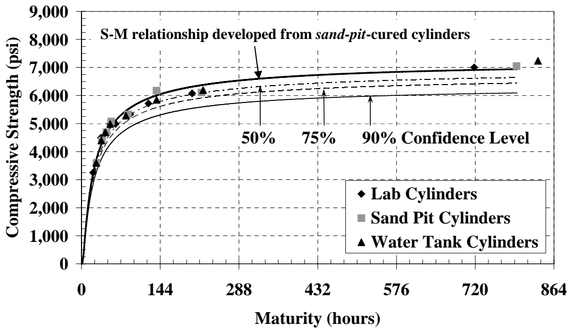
Figure B-27: Sand pit S-M relationship with confidence levels (E = 40 kJ/mol)
