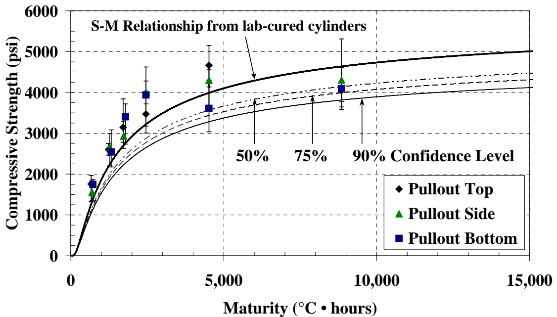
Figure 5-34: Pullout test with laboratory S-M relationship and confidence levels for the cold-weather placement of the mock bridge deck ( T_o = 0\text{ }^\circ\text{C} )
