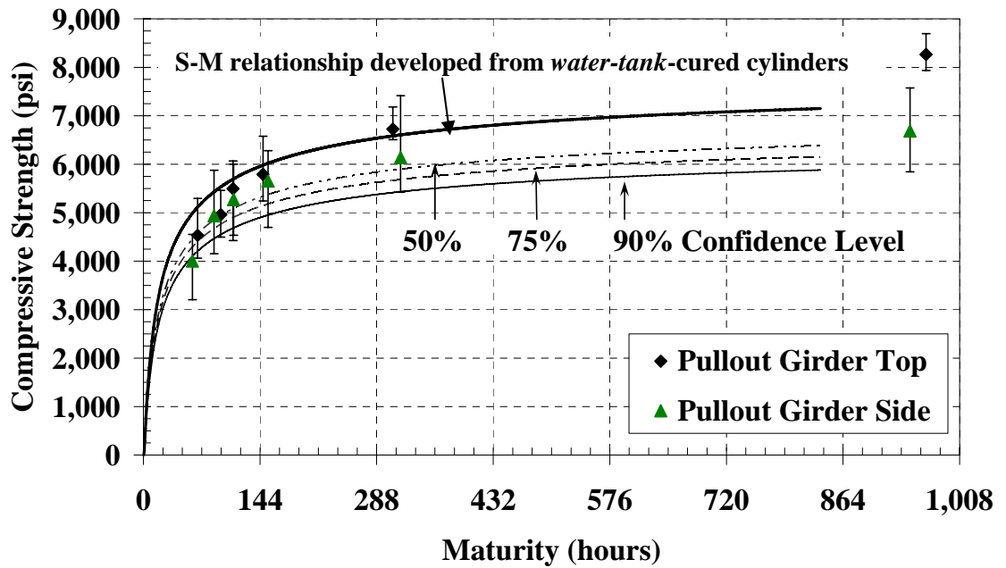
Figure B-31: Pullout test with water-tank S-M relationship and confidence levels (E = 40 kJ/mol)
