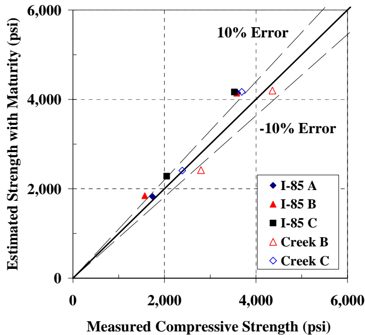
Figure 5-124: 45°-line graph for estimating the strength of the verification cylinders using I-85 Bridge S-M relationship with Nurse-Saul maturity function ( T_o = 0\text{ }^\circ\text{C} )
