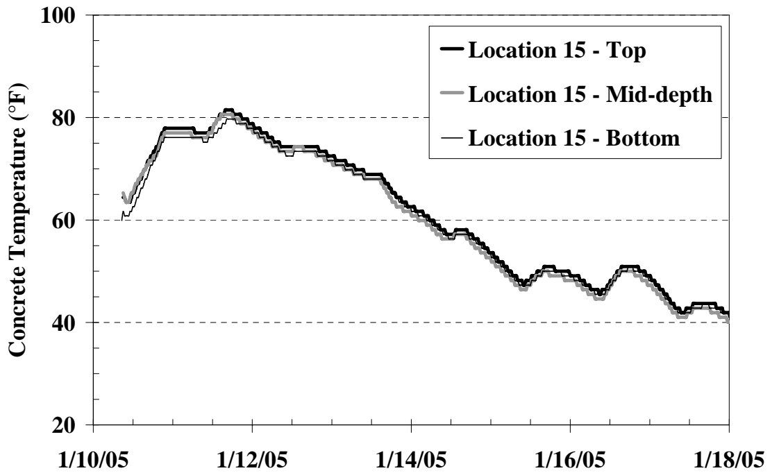
Figure C-67: Temperature history of Location 15 from the I-85 Bridge
