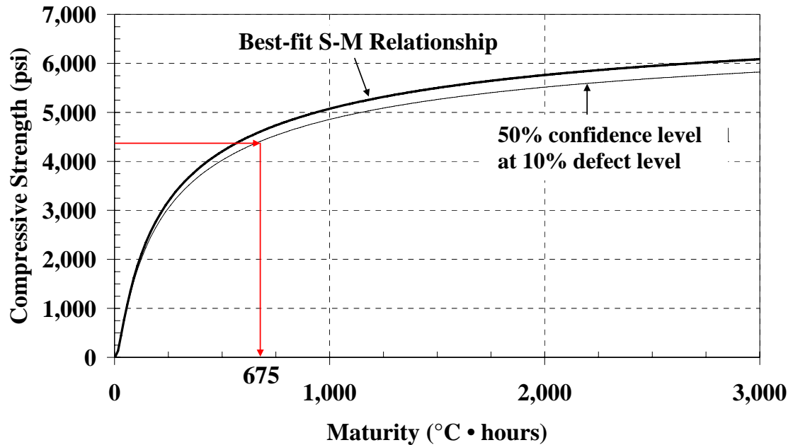
Figure 4-63: 50% confidence level S-M relationship for the prestressed girder project
