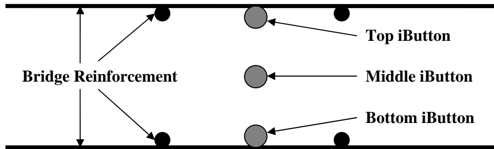
Figure 5-6: Diagram of the iButtons at each location
