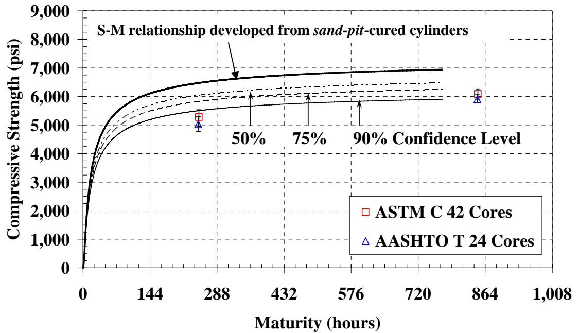
Figure B-42: Cores with sand-pit S-M relationship and confidence levels ( E = 33.5 kJ/mol)
