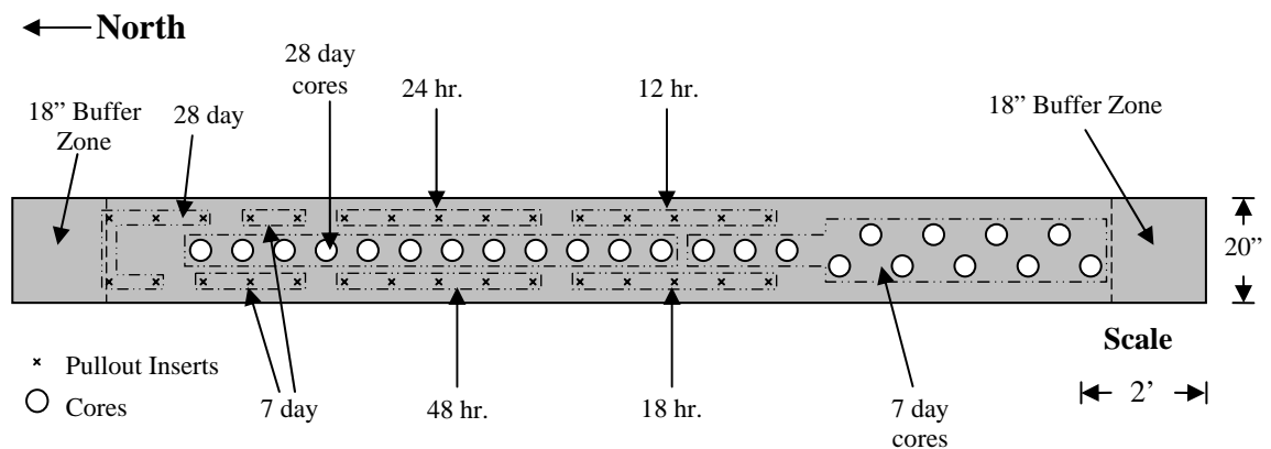
Figure 4-5: Plan view of mock girder
