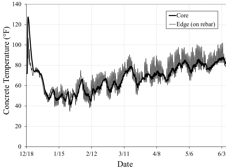
Figure 5-33: Elba bent cap long-term temperature data
