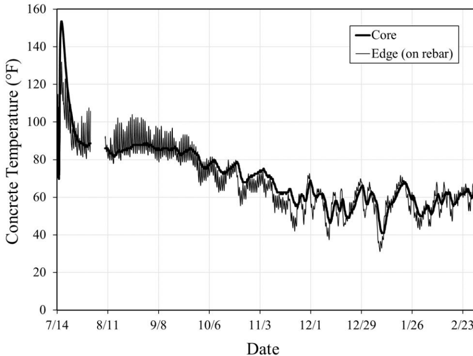
Figure 5-43: Brewton bent cap long-term temperature data
