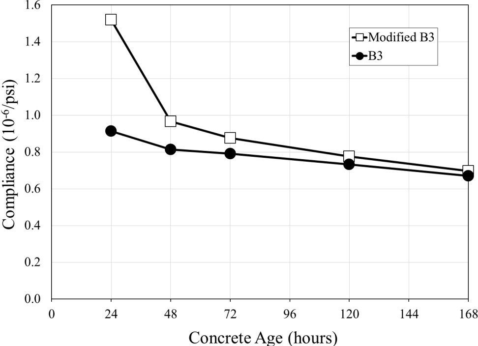
Figure 7-2: Compliance values: B3 versus Modified B3 (Eiland 2015)
