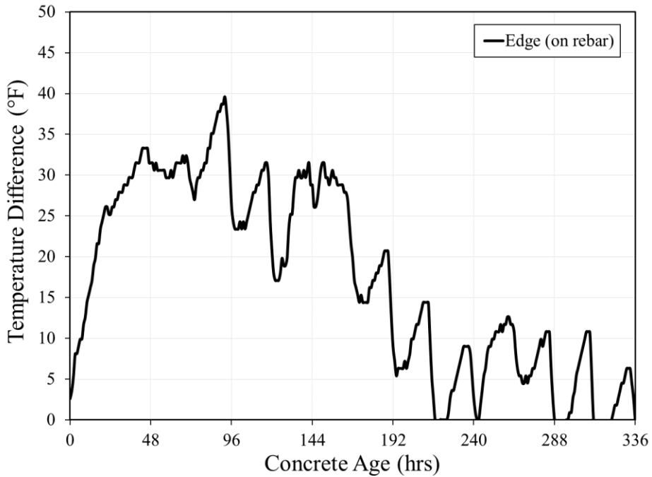
Figure 5-4: Albertville bent cap 14-day temperature difference data
