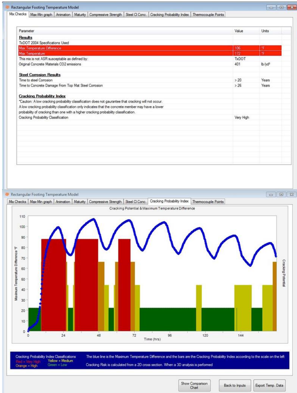
Figure 2-17: Example ConcreteWorks output summary (top) and \Delta T /cracking risk profile (bottom) (Eiland 2015)
