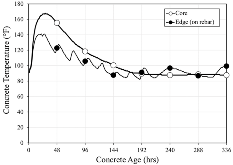
Figure 5-8: Harpersville crashwall 14-day temperature data
