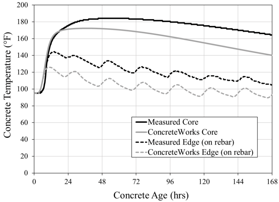
Figure 6-5: Scottsboro pedestal measured temperature data versus ConcreteWorks predictions (Eiland 2015)
