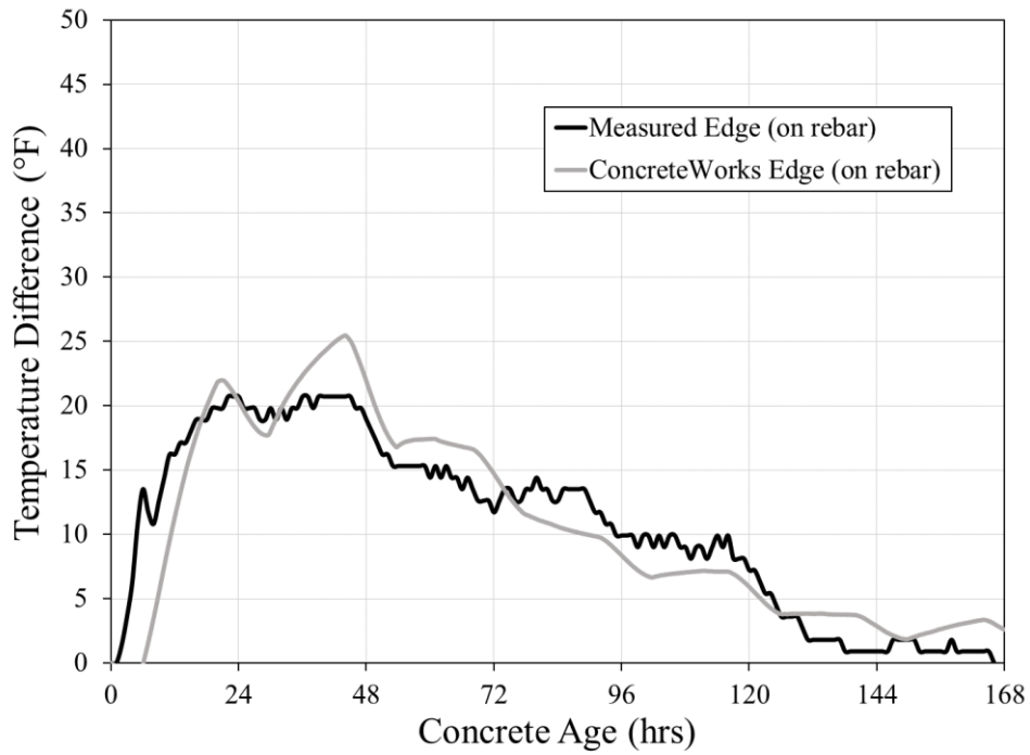
Figure 6-10: Elba bent cap measured temperature difference data versus ConcreteWorks predictions (Eiland 2015)
