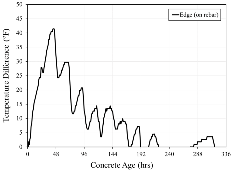
Figure 5-9: Harpersville crashwall 14-day temperature difference data
