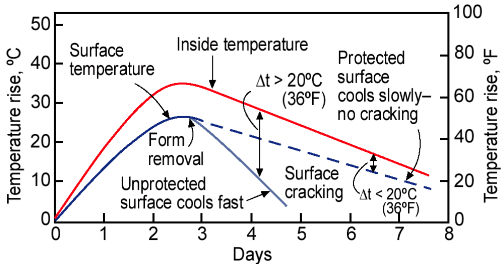
Figure 2-14: The effects of early formwork removal time (Gajda and Alsamsam 2006) ( ^{\circ}\text{F} = 1.8 \times ^{\circ}\text{C} + 32 )
