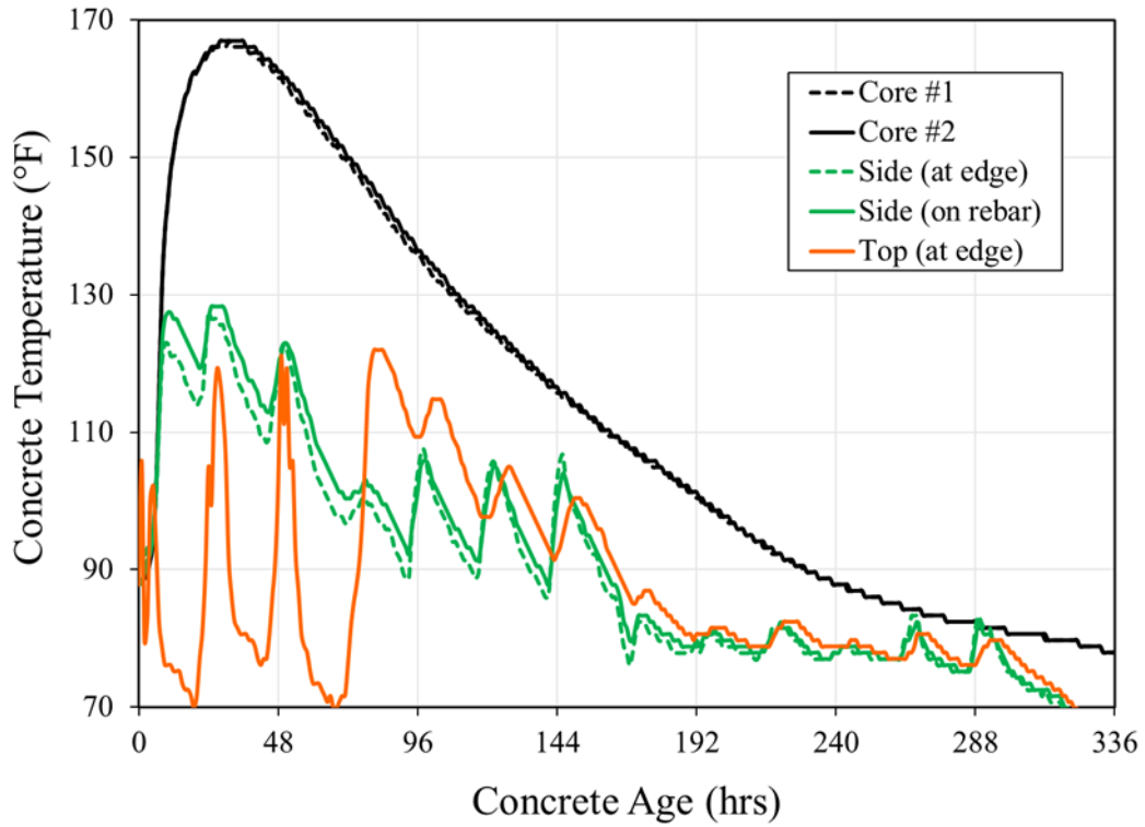
Appendix Figure E-1: Cross-section #1 temperature data – Scottsboro bent cap
