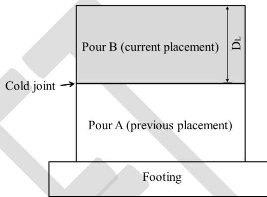
Figure 4: Least dimension of multiple placements (DL)
