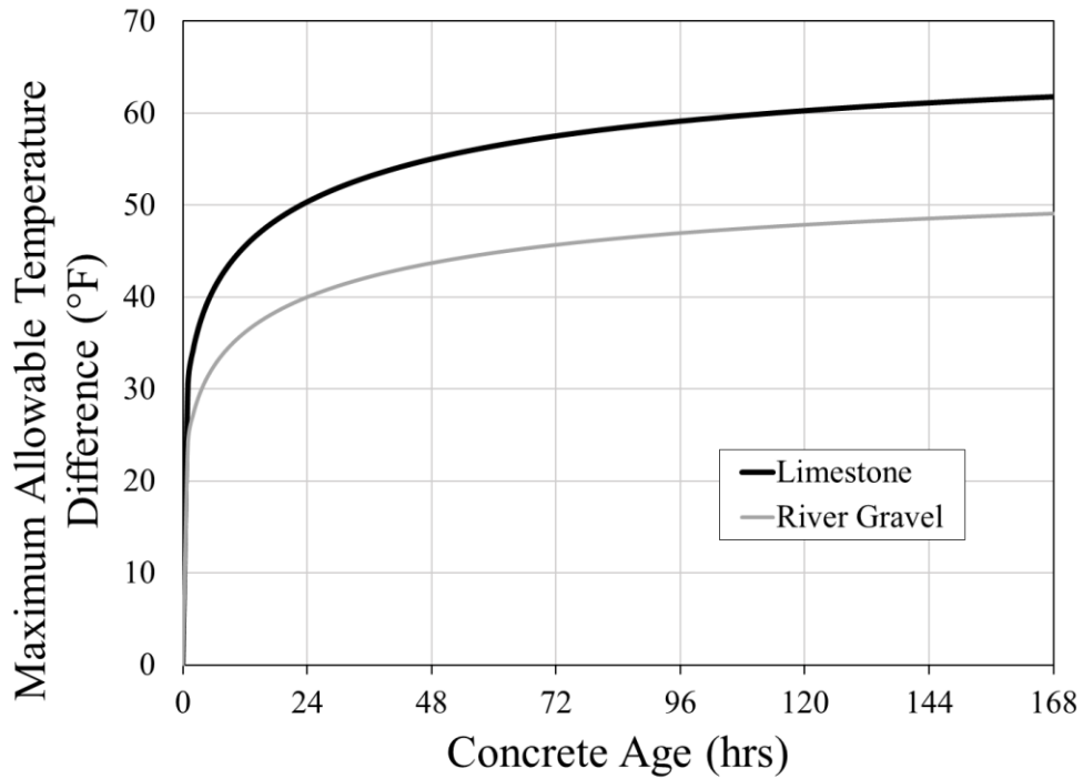
Figure 7-6: Maximum allowable temperature difference limits - Bamforth
