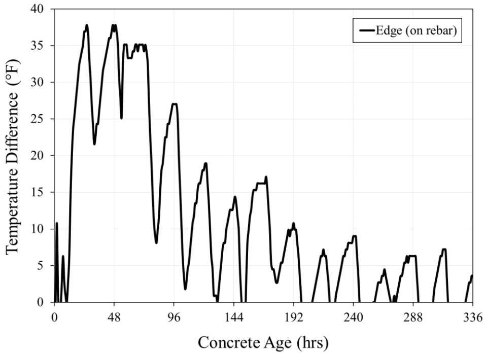
Figure 5-42: Brewton bent cap 14-day temperature difference data
