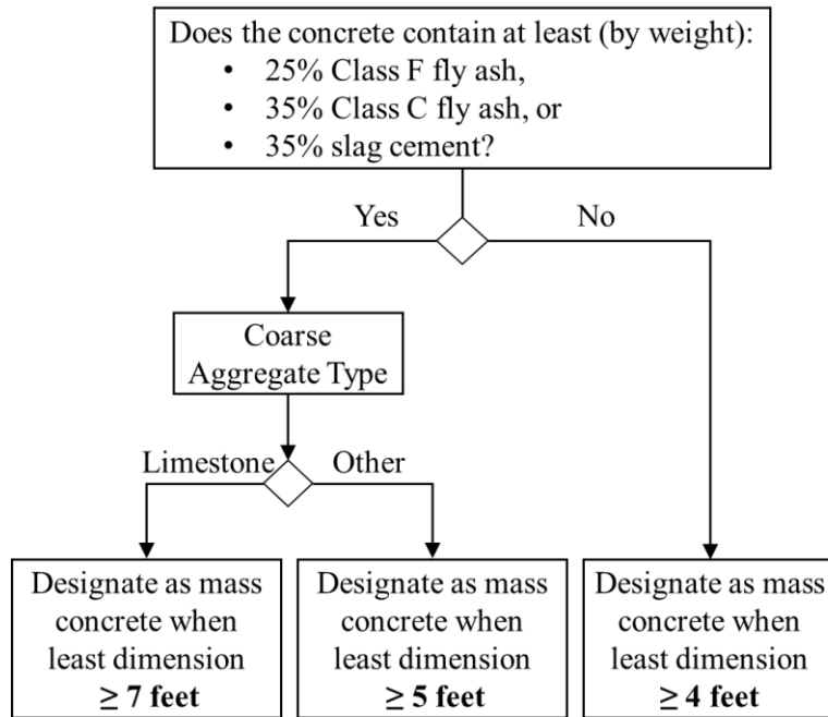
Figure 1: Mass Concrete Size Designation Based on Cementing Materials and Coarse Aggregate Type
