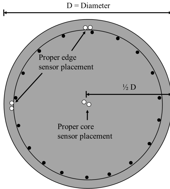
Figure 7-18: Proper sensor placement on circular cross section
