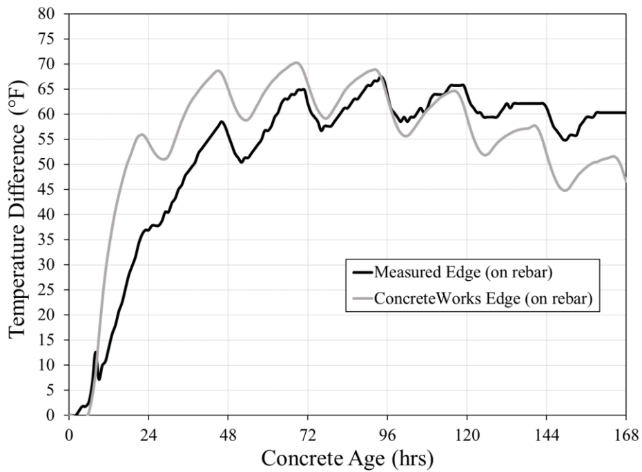
Figure 6-6: Scottsboro pedestal measured temperature difference data versus ConcreteWorks predictions (Eiland 2015)
