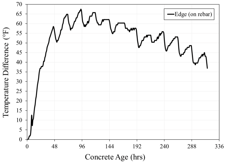
Figure 5-16: Scottsboro pedestal 14-day temperature difference data
