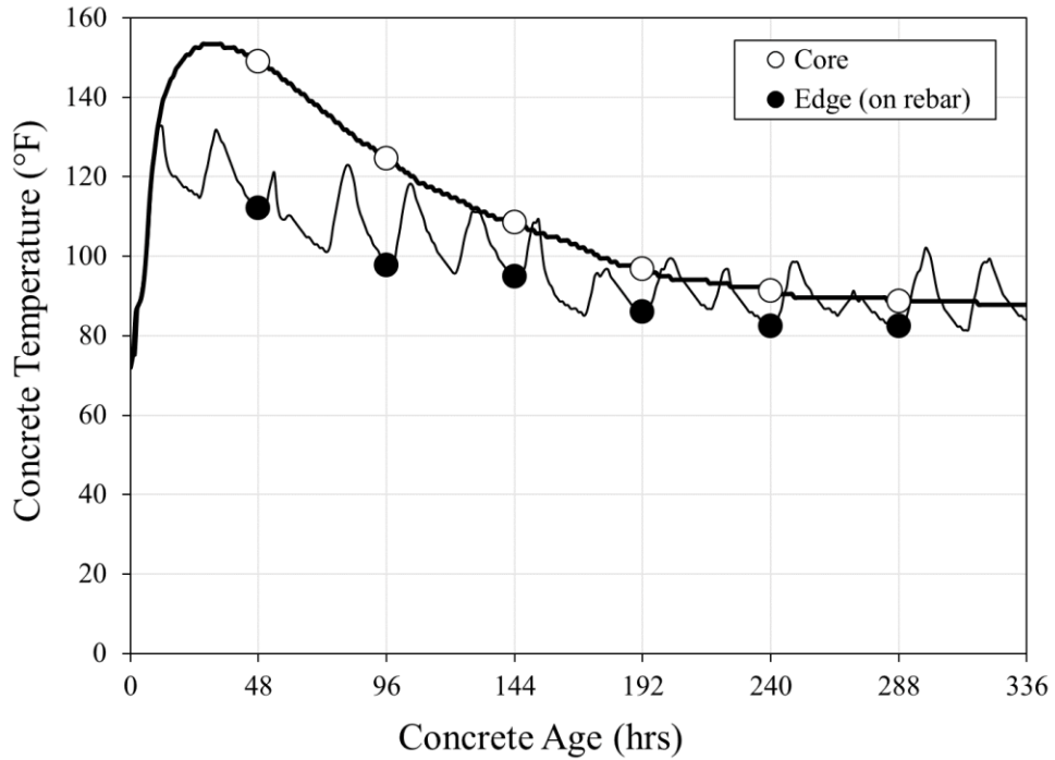
Figure 5-41: Brewton bent cap 14-day temperature data
