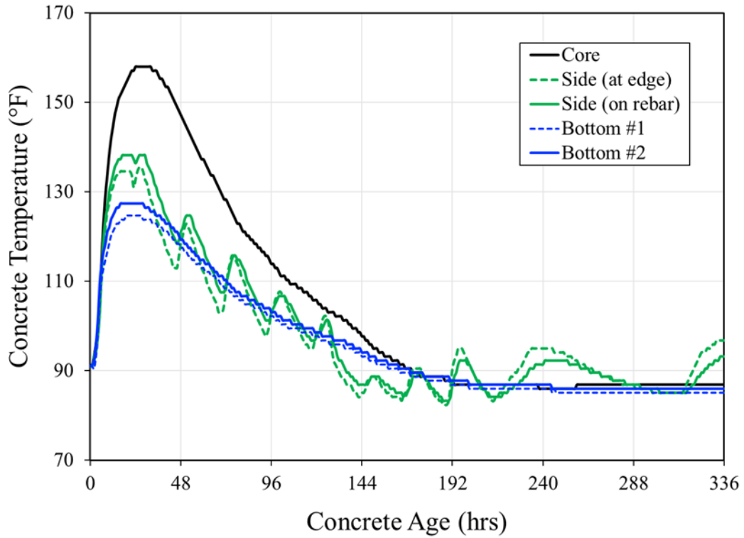
Appendix Figure C-1: Cross-section #1 temperature data – Harpersville crashwall
