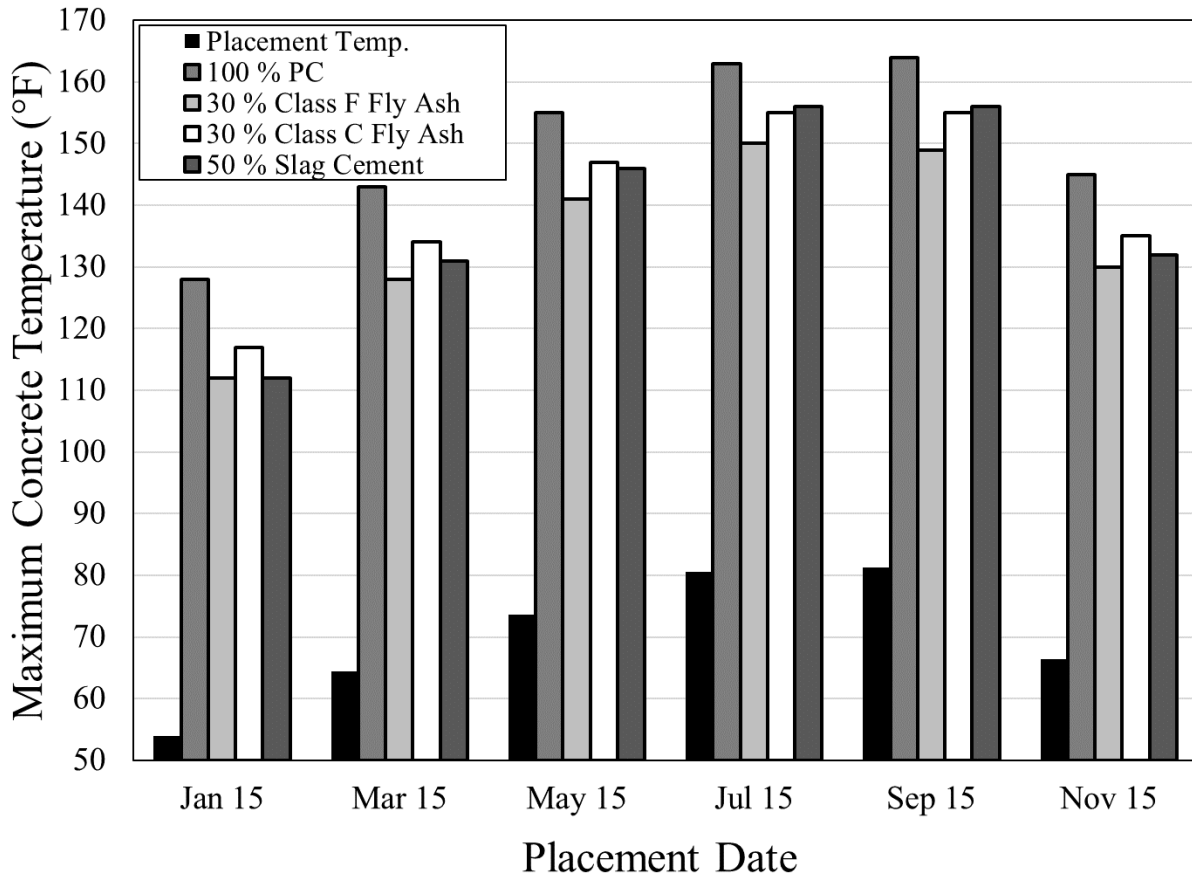
Figure 6-15: Effect of placement date and SCM type on maximum concrete temperature (Mobile, AL; Limestone; 6 ft x 6 ft) (adapted from Eiland 2015)
