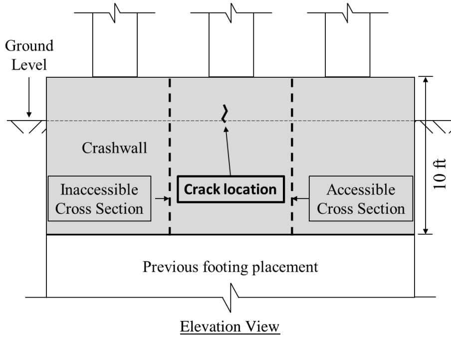
Figure 5-11: Harpersville crashwall approximate crack location
