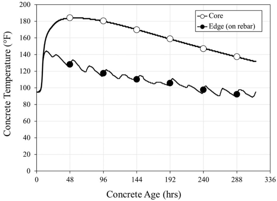
Figure 5-15: Scottsboro pedestal 14-day temperature data
