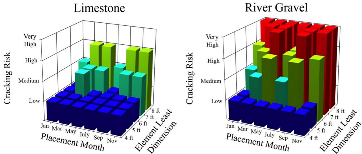
Figure 6-18: Effect of least dimension, coarse aggregate type, and placement date on maximum concrete cracking risk (Mobile, AL; 100% PCC) (Eiland 2015)
