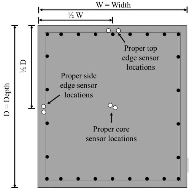
Figure 7: Proper temperature sensor placement on a rectangular bent cap cross section (example of vertically oriented cross section)
