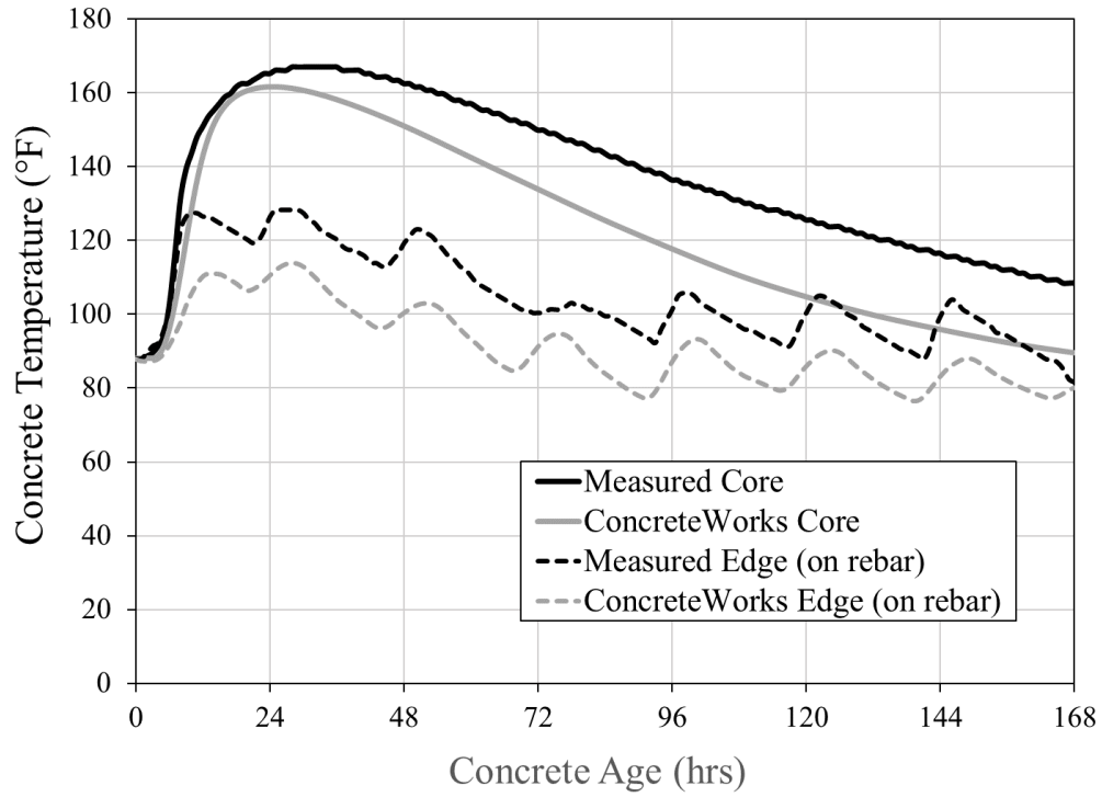
Figure 6-7: Scottsboro bent cap measured temperature data versus ConcreteWorks predictions (Eiland 2015)
