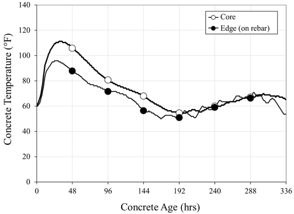
Figure 5-36: Birmingham column 14-day temperature data
