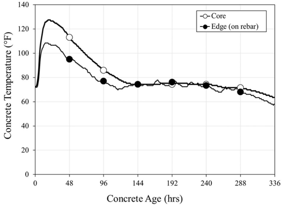
Figure 5-31: Elba bent cap 14-day temperature data
