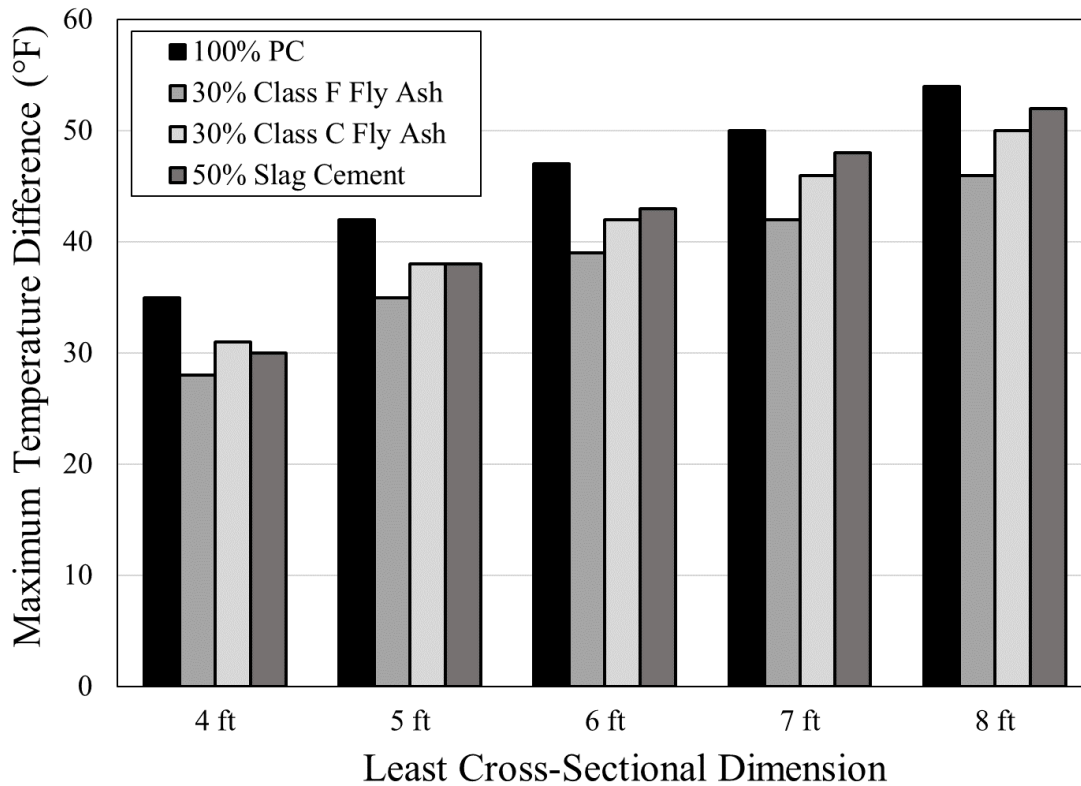
Figure 6-17: Effect of least dimension and SCM use on maximum concrete temperature difference (Mobile, AL; July 15; Limestone) (Eiland 2015)
