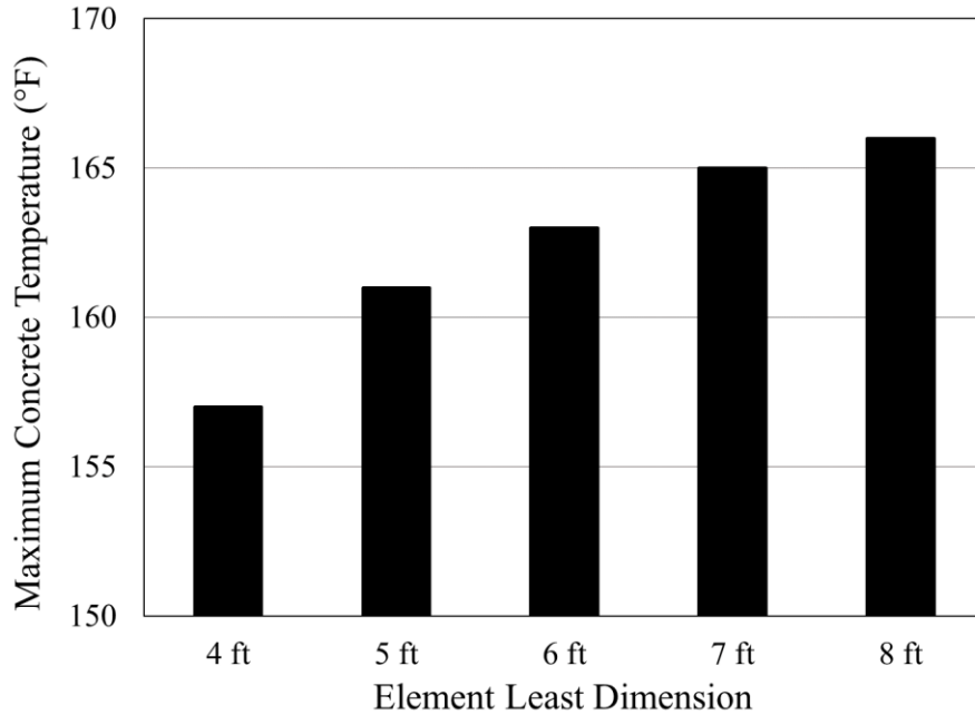
Figure 6-16: Effect of element least dimension on maximum concrete temperature (Mobile, AL; July 15; Limestone; 100% PC) (Eiland 2015)
