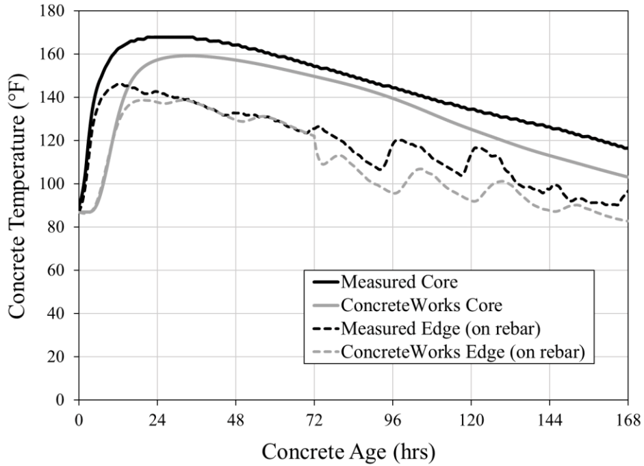
Figure 6-1: Albertville bent cap measured temperature data versus ConcreteWorks predictions (Eiland 2015)
