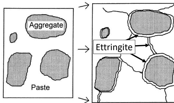
Figure 2-7: Proposed DEF expansion mechanism (Taylor et al. 2001)
