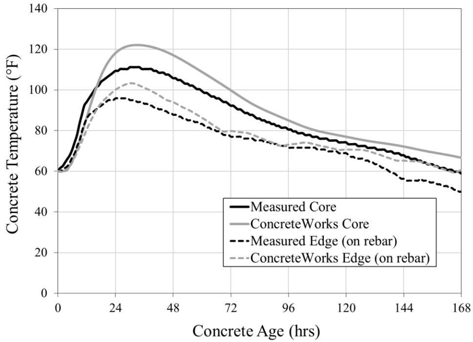
Figure 6-11: Birmingham column measured temperature data versus ConcreteWorks predictions (Eiland 2015)
