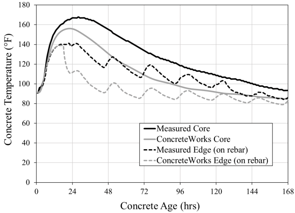
Figure 6-3: Harpersville crashwall measured temperature data versus ConcreteWorks predictions (Eiland 2015)
