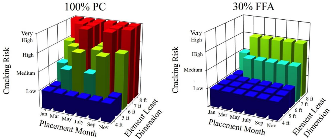
Figure 6-19: Effect of least dimension, SCM, and placement date on maximum concrete cracking risk (Mobile, AL; River Gravel) (Eiland 2015)
