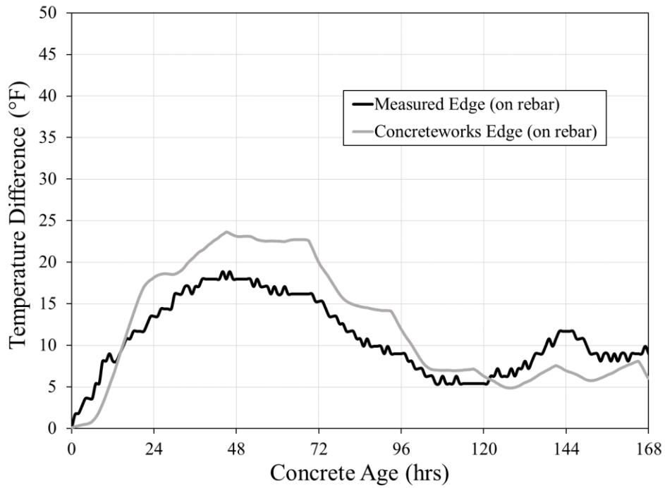
Figure 6-12: Birmingham column measured temperature difference data versus ConcreteWorks predictions (Eiland 2015)
