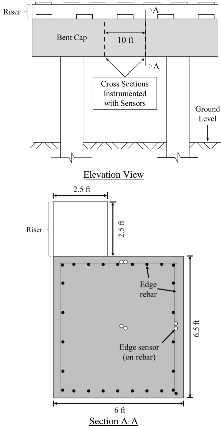
Figure 5-40: Brewton bent cap instrumented cross-section locations (top) and temperature sensor locations on these cross sections (bottom)
