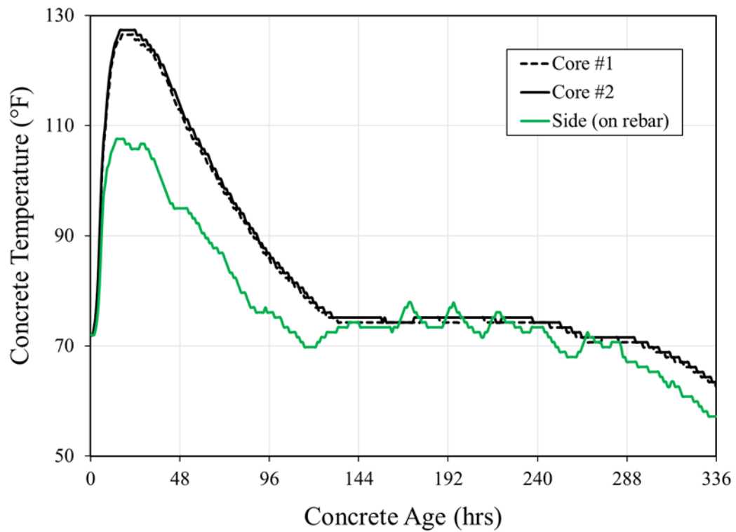
Appendix Figure F-2: Cross-section #2 temperature data – Elba bent cap
