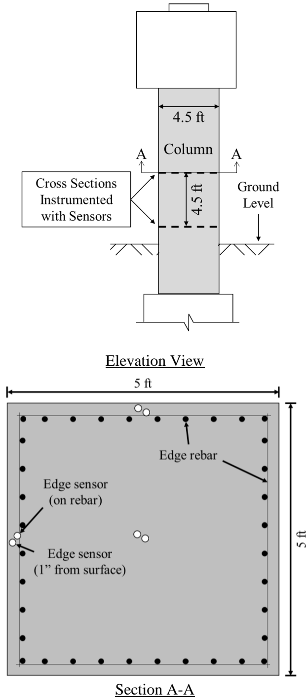
Figure 5-35: Birmingham column instrumented cross section locations (top) and temperature sensor locations on these cross sections (bottom)
