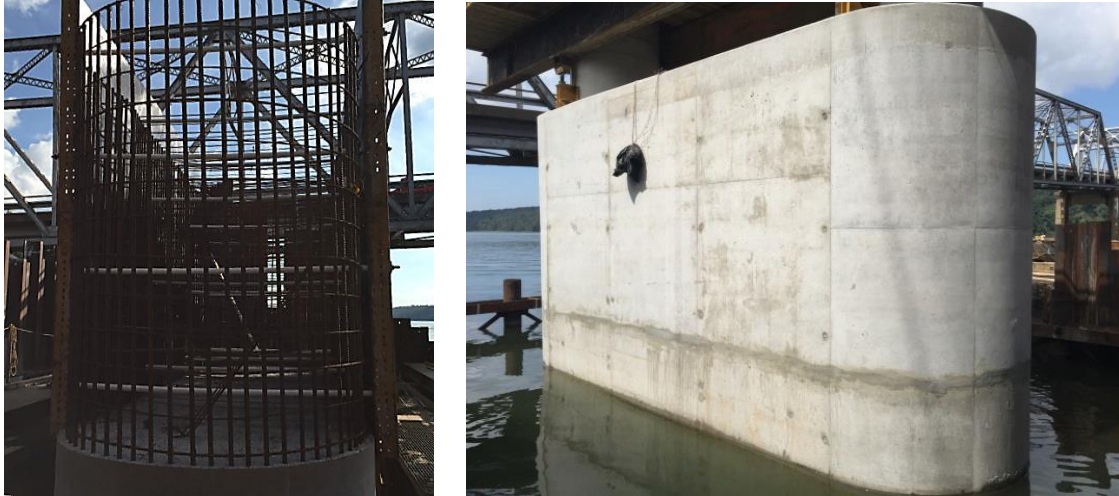
Figure 5-13: Scottsboro pedestal prior to placement (left) and post construction (right)
