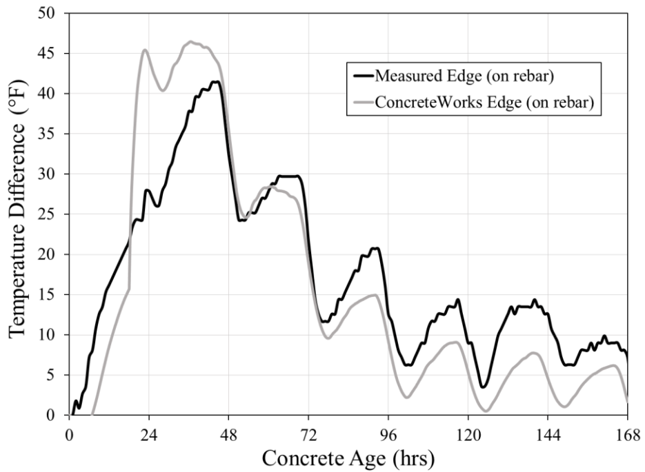
Figure 6-4: Harpersville crashwall measured temperature difference data versus ConcreteWorks predictions (Eiland 2015)
