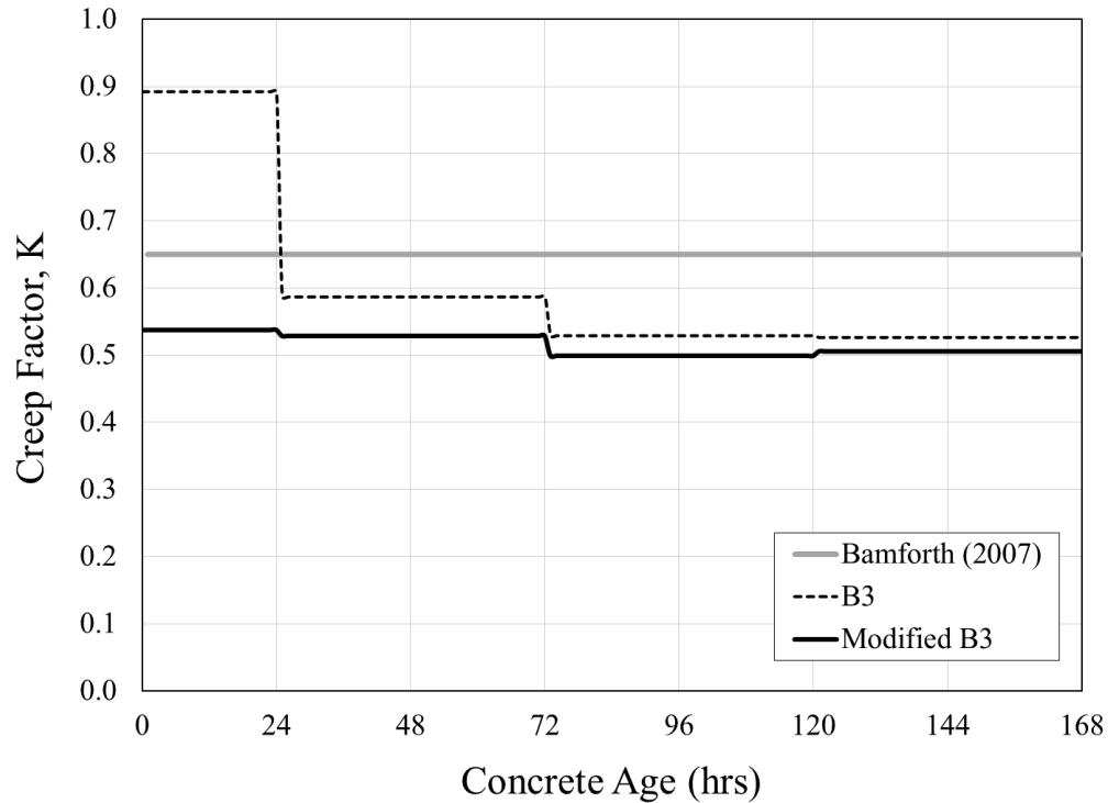
Figure 7-3: Creep factors: Bamforth versus B3 versus Modified B3 (Eiland 2015)
