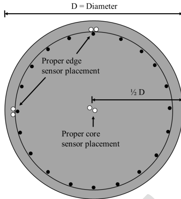
Figure 9: Correct temperature sensor placement on a circular column cross section (example of a horizontally oriented cross section)
