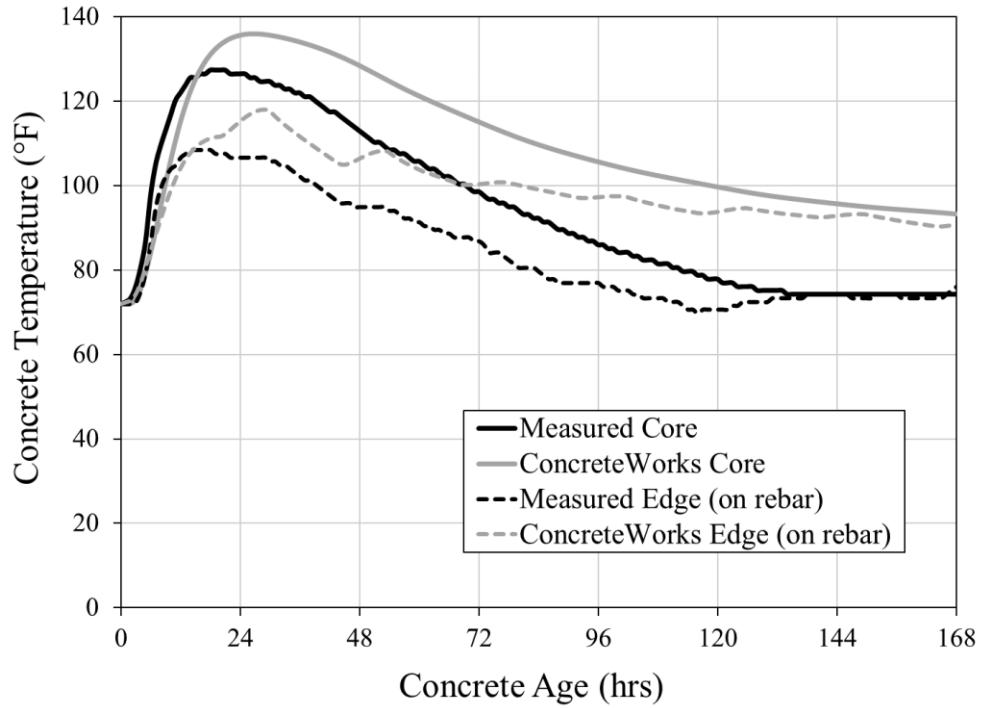
Figure 6-9: Elba bent cap measured temperature data versus ConcreteWorks predictions (Eiland 2015)
