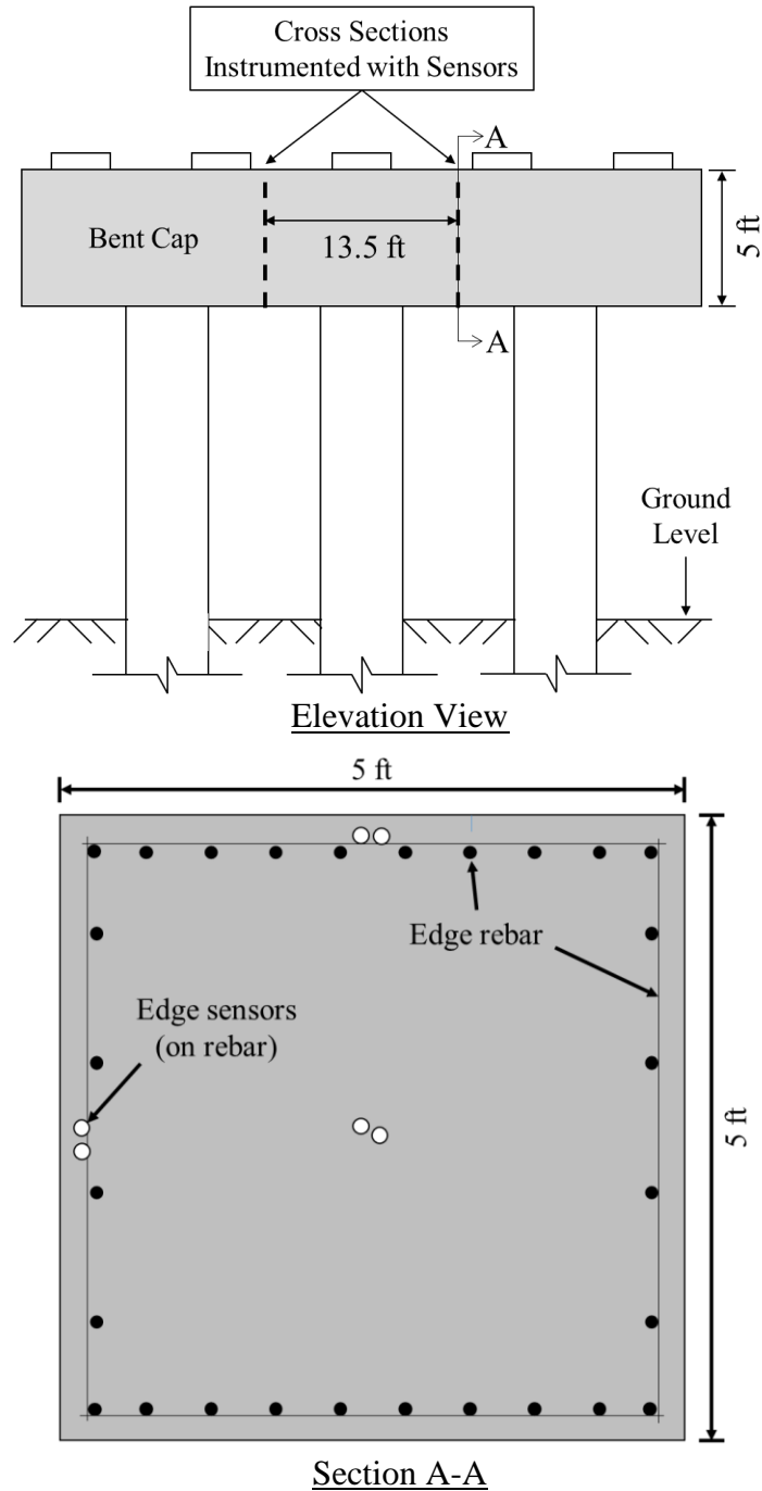
Figure 5-30: Elba bent cap instrumented cross section locations (top) and temperature sensor locations on these cross sections (bottom)
