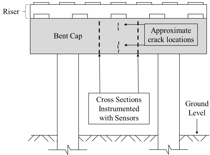
Figure 5-44: Brewton bent cap approximate crack locations
