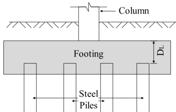
Figure 2: Footing with steel piles least dimension (DL)
