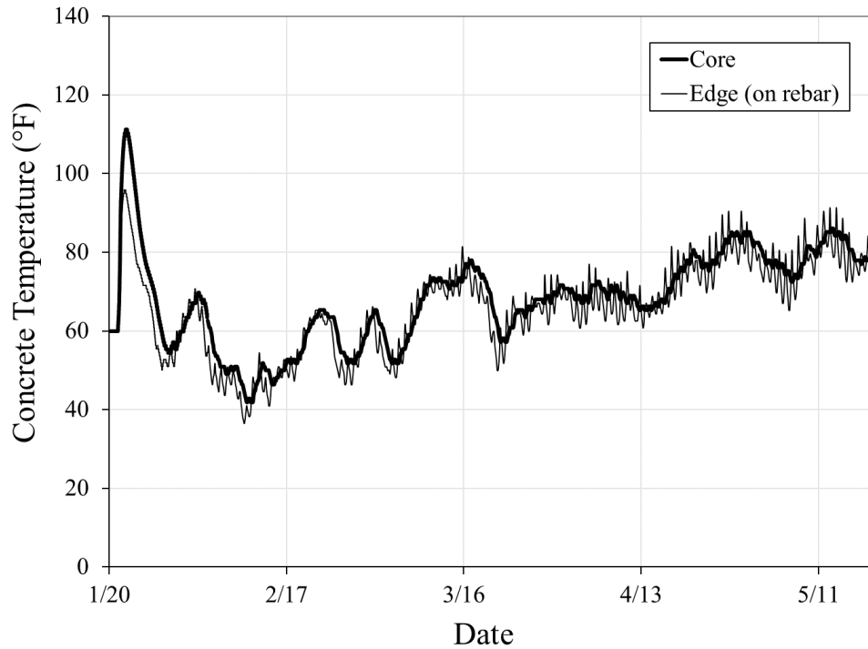
Figure 5-38: Birmingham column long-term temperature data
