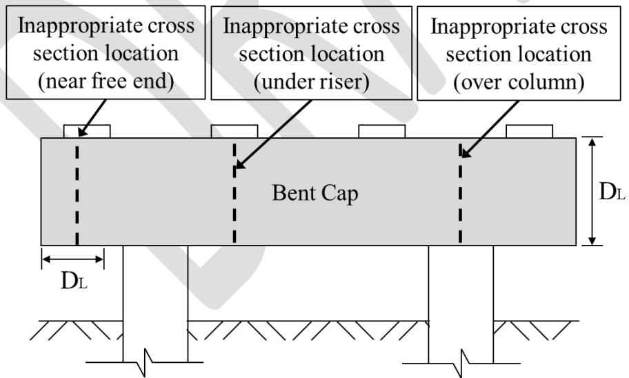
Figure 6: Inappropriate temperature sensor cross section locations within a bent cap ( D_L = least dimension) (example of vertically oriented cross section)
