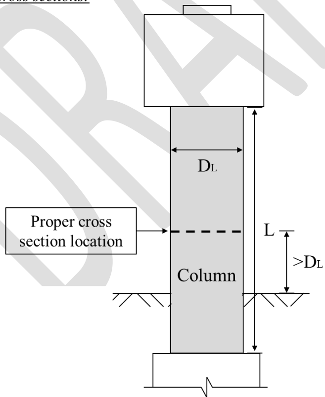
Figure 8: Proper temperature sensor cross section locations within a column ( D_L = least dimension) (example of a horizontally oriented cross section)
