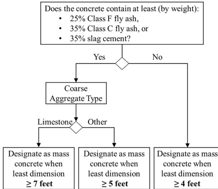
Figure 7-1: Mass concrete least dimension selection flow chart
