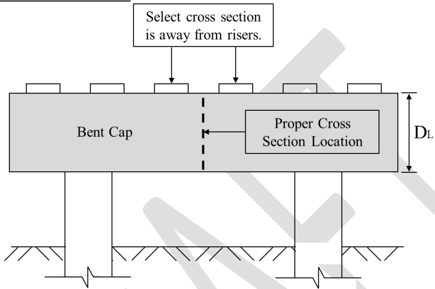
Figure 5: Proper temperature sensor cross-section location within a bent cap (example of vertically oriented cross section)
