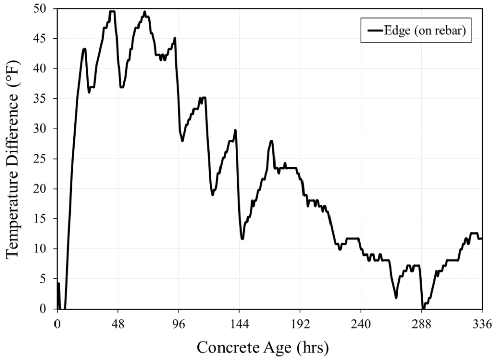
Figure 5-28: Scottsboro bent cap 14-day temperature difference data
