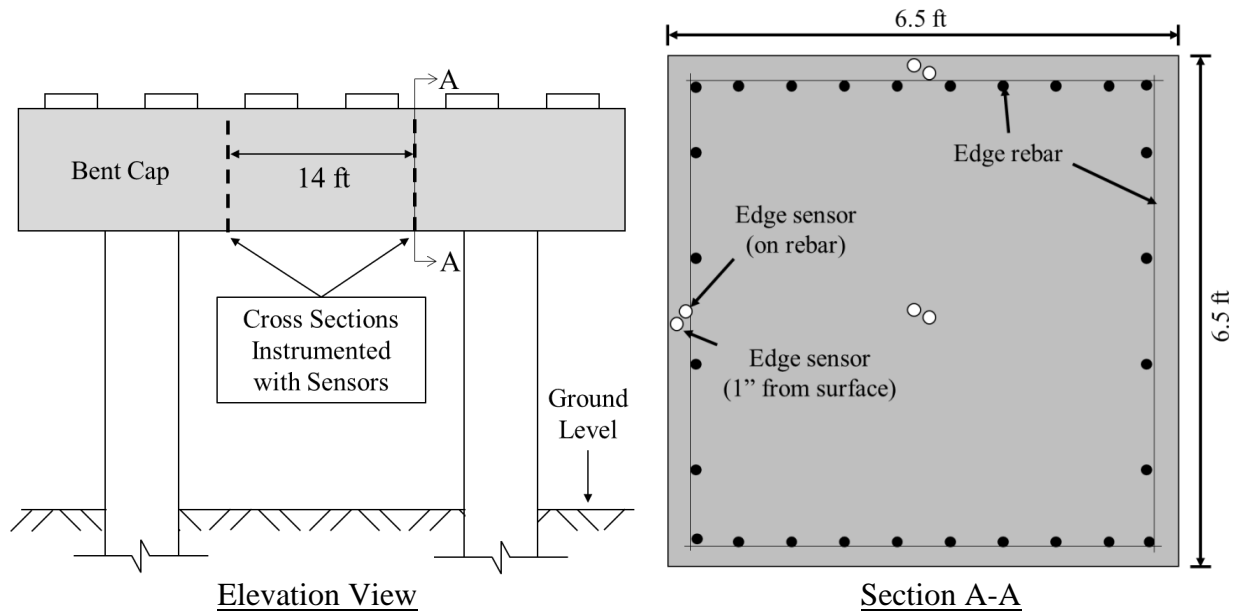
Figure 4-4: Example layout of temperature sensor cross sections in a bent cap (left) and temperature sensors within each cross section (right) (n.t.s.)
