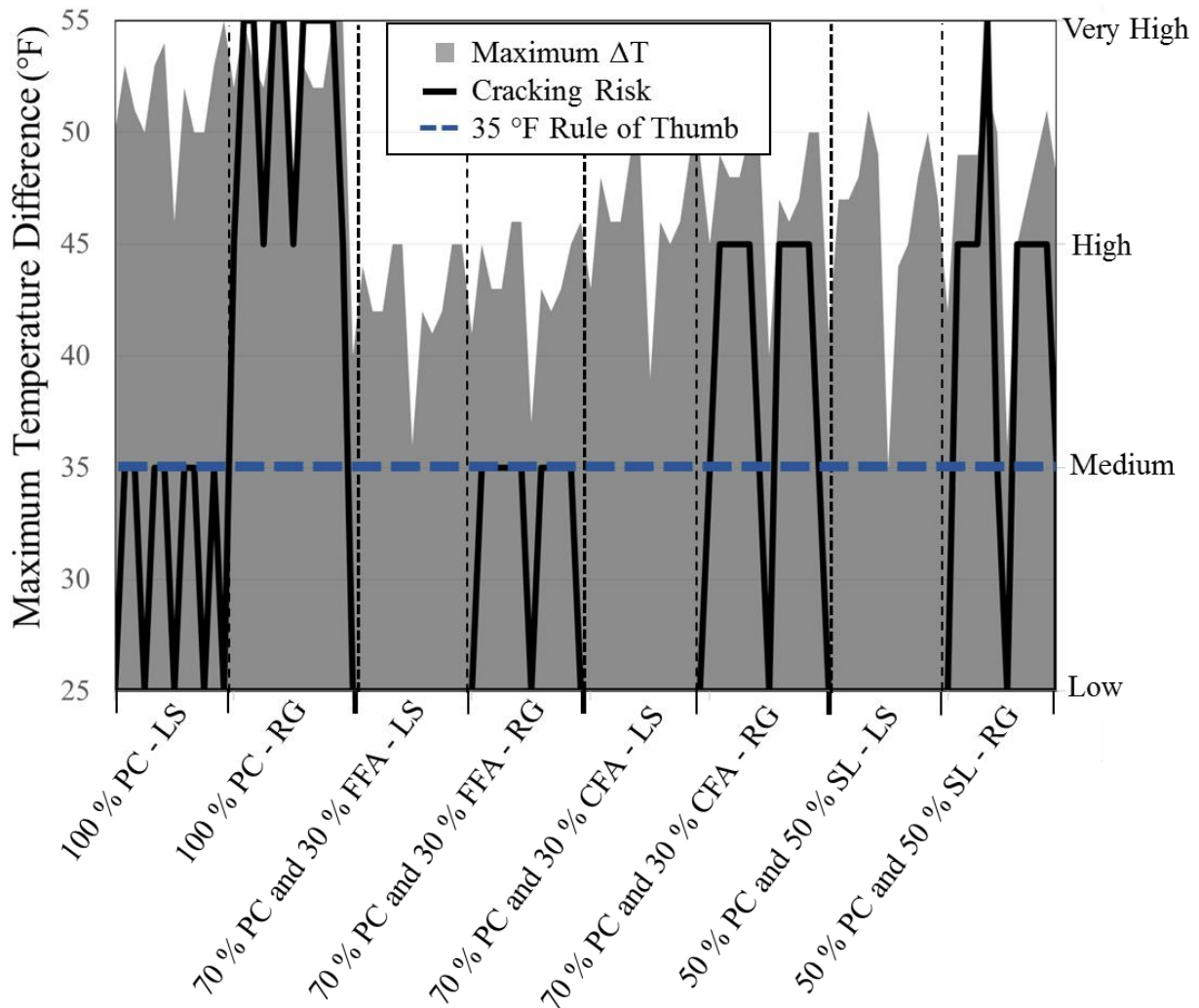
Figure 6-20: Comparing maximum temperature differences and their corresponding cracking risks on a 7 ft cross section (Eiland 2015)
