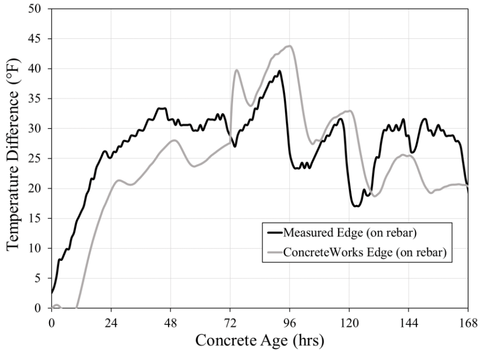
Figure 6-2: Albertville bent cap measured temperature difference data versus ConcreteWorks predictions (Eiland 2015)
