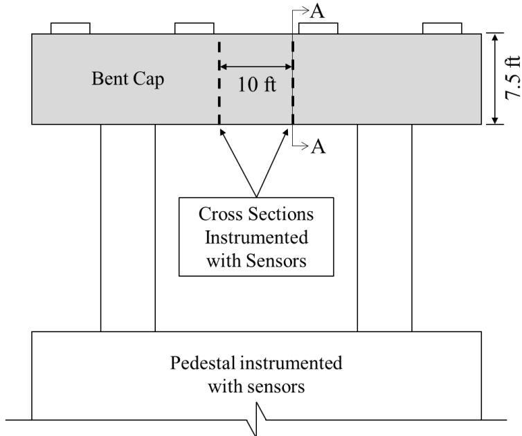
Elevation View
