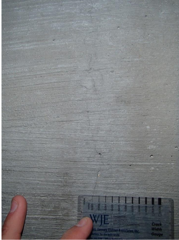
Figure 5-48: Brewton bent cap cracks (south face)
