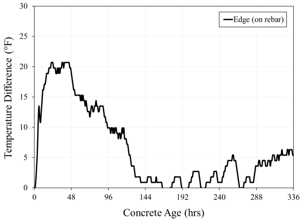
Figure 5-32: Elba bent cap 14-day temperature difference data
