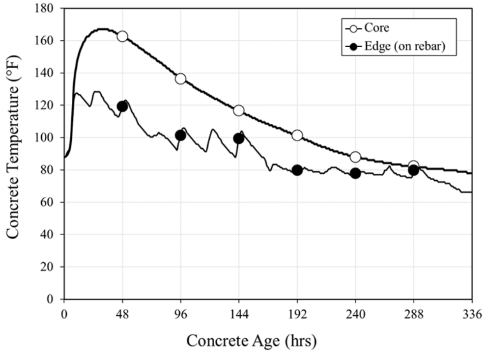
Figure 5-27: Scottsboro bent cap 14-day temperature data
