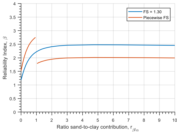
Figure 7-3: Comparison of reliability indices obtained from different factors of safety alternatives for layered soils
