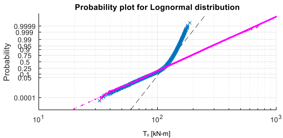
Figure B-7: Medium sand. \gamma=18.8 kN/m 3 N_{spt}=20 . Lognormal \lambda=1.21 COV=0.42
