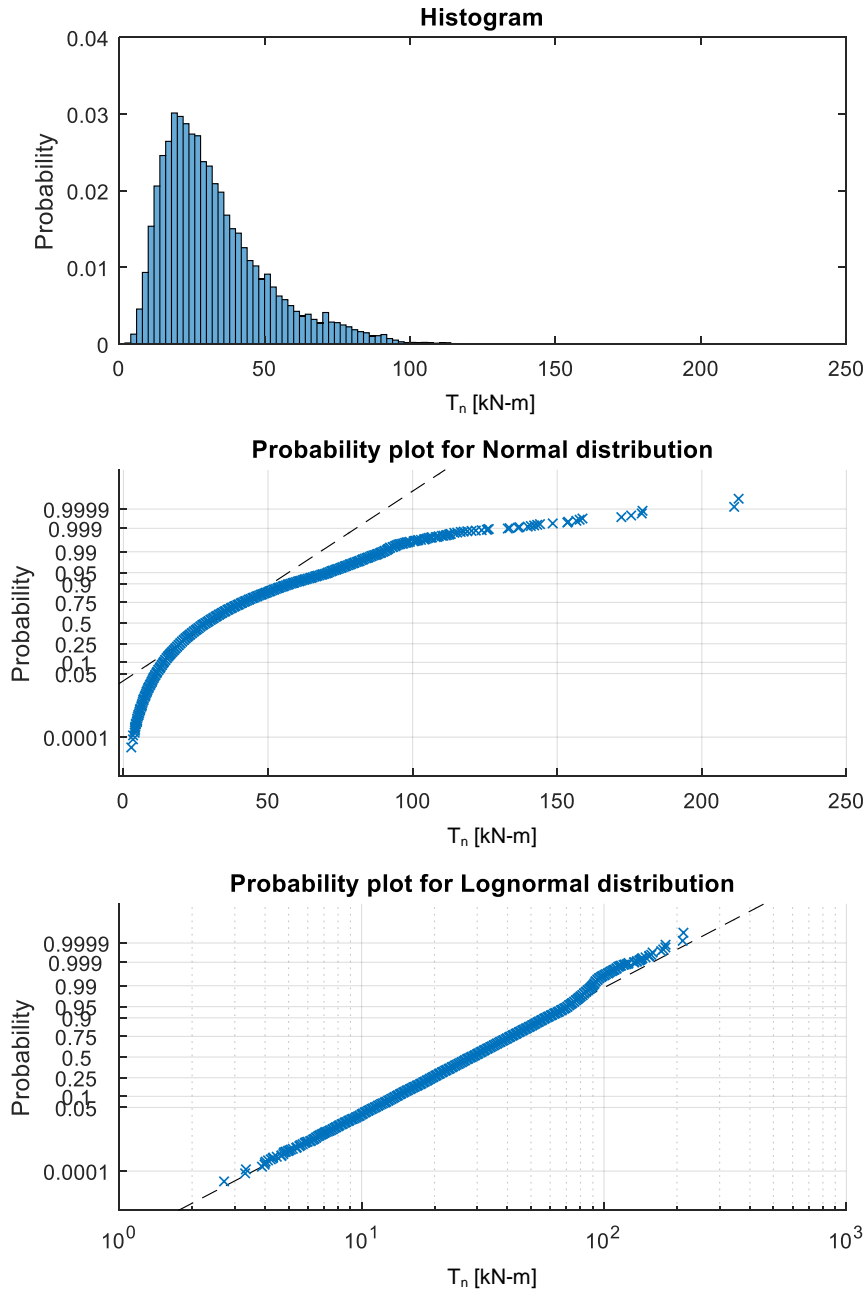
Figure B-3: Stiff weathered clay. \gamma=18.8 \text{ kN/m}^3 s_u=72 \text{ kPa} . Lognormal \lambda=1.00 COV=0.56
