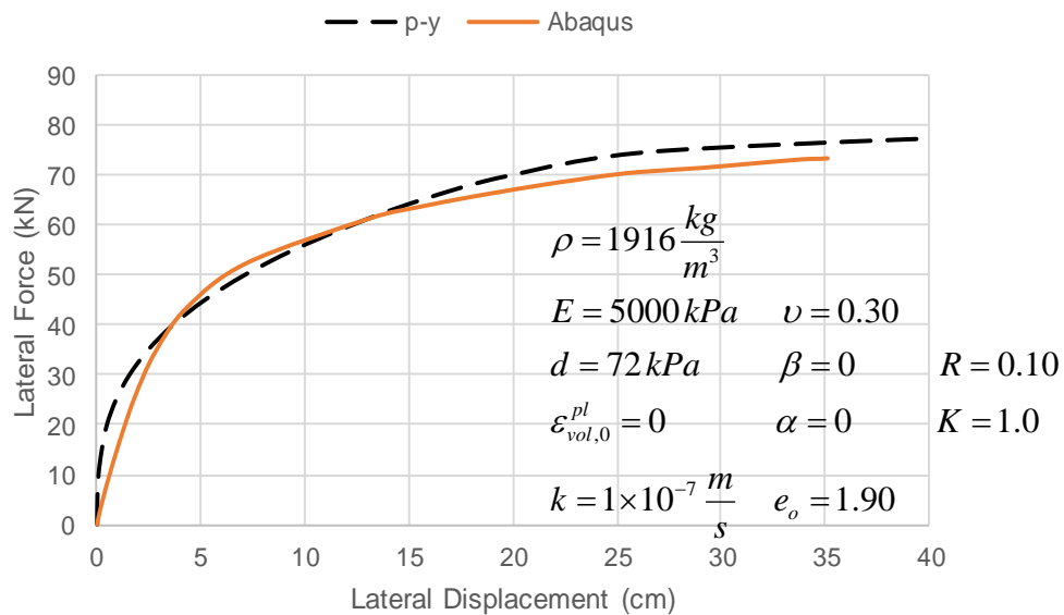
Figure 5-8: Calibration and calibrated properties for clay
