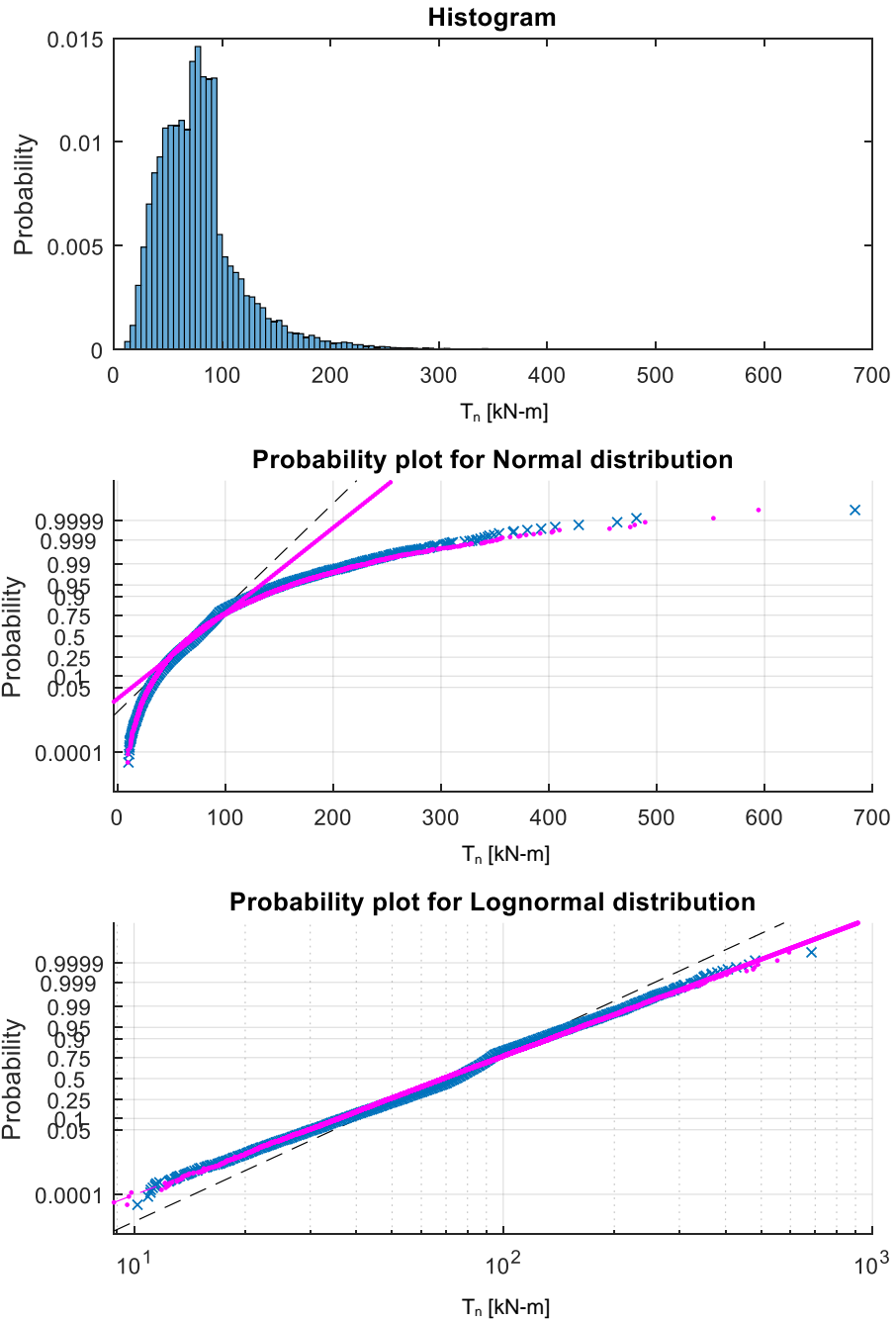
Figure B-5: Moderately hard to hard and hard clay. \gamma=20.4 \text{ kN/m}^3 s_u=192 \text{ kPa} . Lognormal \lambda=0.97 COV=0.54
