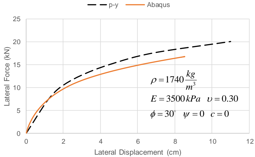
Figure 5-7: Calibration and calibrated properties for sand
