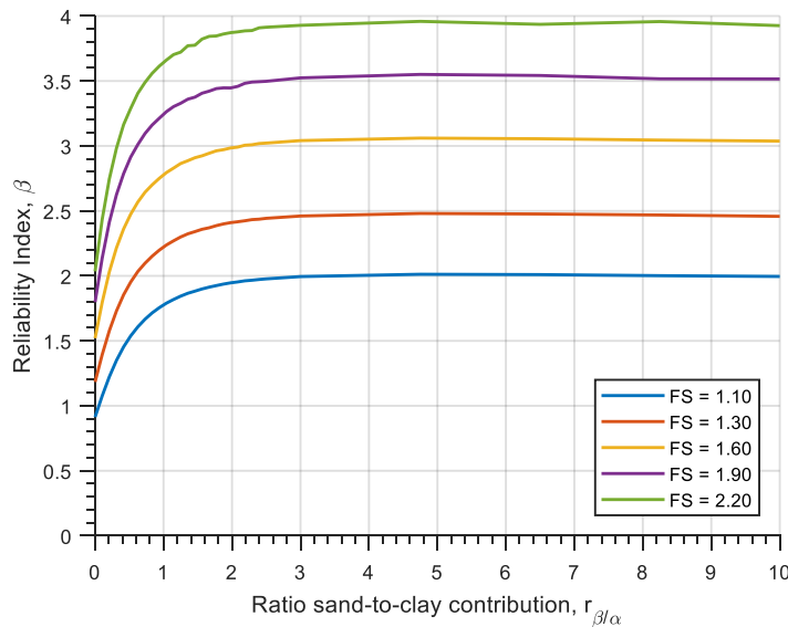
Figure 7-2: Reliability index vs. contribution ratio for various factors of safety
