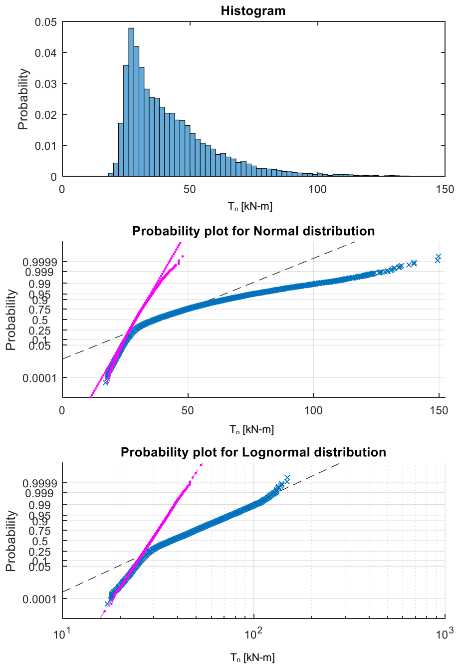
Figure B-6: Loose and very loose sand. \gamma=17.3 kN/m 3 N_{spt}=5 . Lognormal \lambda=0.72 COV=0.12
