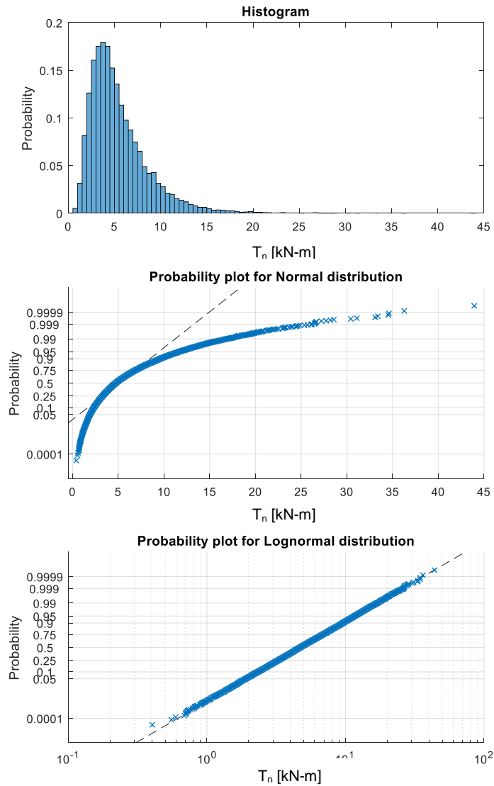
Figure B-1: Soft and extremely soft clay. \gamma=16.5 kN/m 3 s_u=12 kPa. Lognormal \lambda=1.00 COV=0.59
