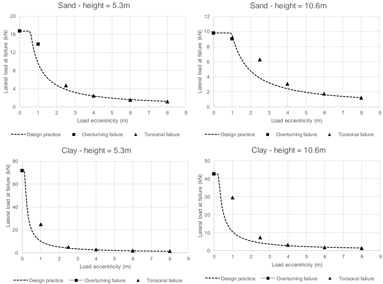
Figure 5-17: FEM results vs. typical design practice
