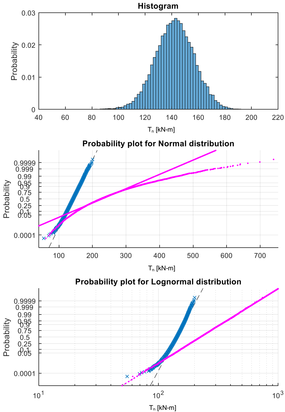
Figure B-8: Dense to very dense sand. \gamma=20.4 \text{ kN/m}^3 N_{\text{spt}}=40 . Lognormal \lambda=1.65 \text{COV}=0.31
