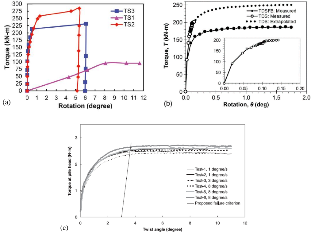
Figure 2-4: Typical torque-rotation angle response, (a) Thiyyakkandi et al. 2016; (b) Li et al., 2017; and (c) Zhang and Kong (2006)
