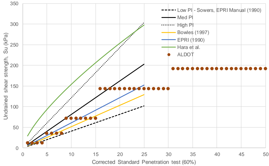
Figure 2-3: Undrained shear strength vs. standard penetration test from several sources
