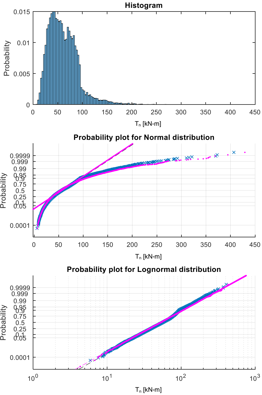
Figure B-4: Medium hard to hard and very stiff clay. \gamma=19.6 \text{ kN/m}^3 s_u=144 \text{ kPa} . Lognormal \lambda=0.93 COV=0.57
