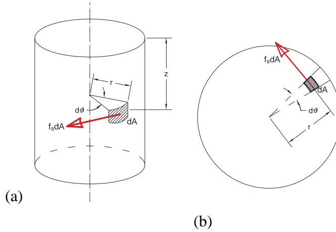
Figure 2-6: Differential element location: (a) at the side of the shaft; and (b) at the toe of the shaft
