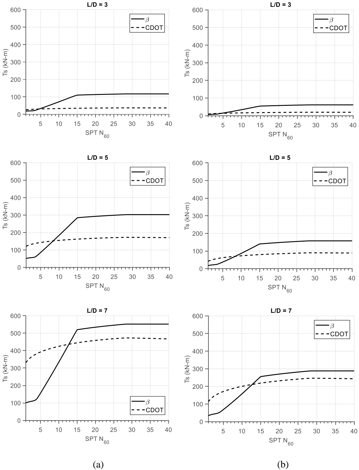
Figure 4-5: Torsional resistance from \beta and CDOT methods in uniform layers of sand, (a) dry condition, and (b) saturated condition
