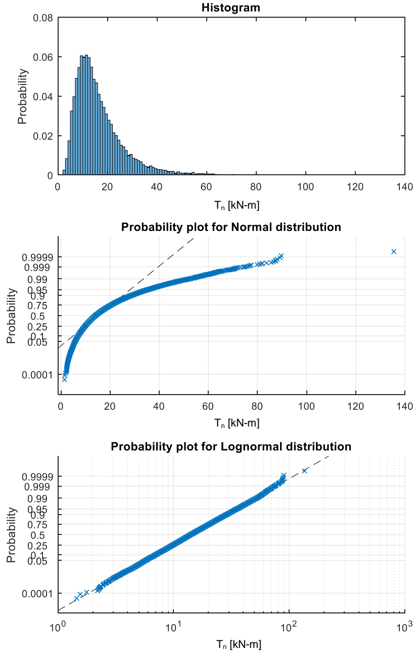
Figure B-2: Medium to moderately hard clay. \gamma=18.1 \text{ kN/m}^3 s_u=36 \text{ kPa} . Lognormal \lambda=1.00 COV=0.60
