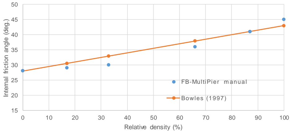
Figure 2-2: Internal friction angle vs. relative density from several sources
