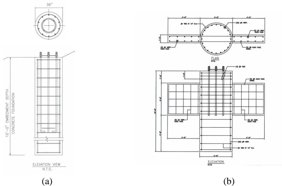
Figure 1-2: Drilled shaft foundation for a signal mast-arm pole, (a) standard foundation, (b) special foundation with wings for torsional resistance (Courtesy of ALDOT)
