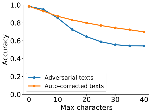
Figure 4.6: Defense against character-level adversarials. (Image credit: [Gon+18])
