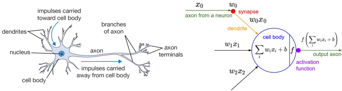
Figure 2.1: The artificial neuron (right) is inspired by the biological neurons (left). For the artificial neuron on the right, The x 's are signals from other neurons, weights w 's controls the signal strength. The cell is essentially a function f that aggregates and transforms the inputs to produce the signal. (image credit: cs231n)
