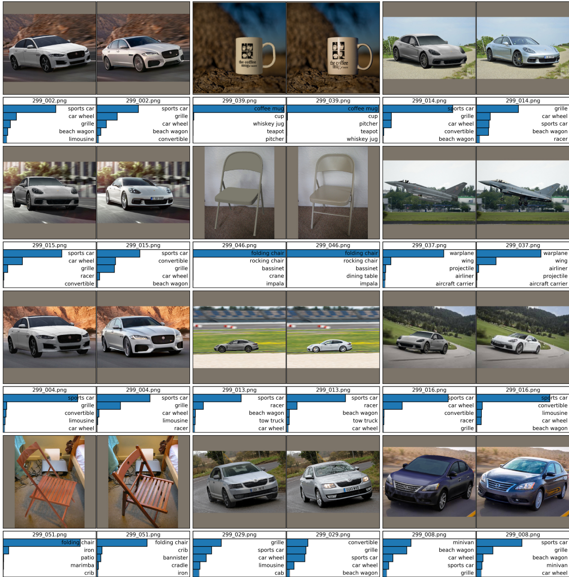
Figure 5.8: 12 random pairs of renders (left) and real photos (right) among 56 pairs produced in total for our 3D object rendering evaluation (Section 1). The renders are produced by the differentiable renderer by [KUH18]. More images are available at https://goo.gl/8z42zL . While discrepancies can be spotted in our side-by-side comparisons, we found that most of the renders passed our human visual Turing test if presented alone. (Image credit: [Alc+18])
