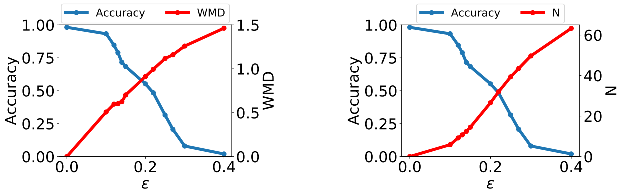
Figure 4.3: Word-level model’s accuracy with varying FGSM noise level. The WMD and N (number of words changed) empirically show the quality of the adversarial texts. (Image credit: [Gon+18])
