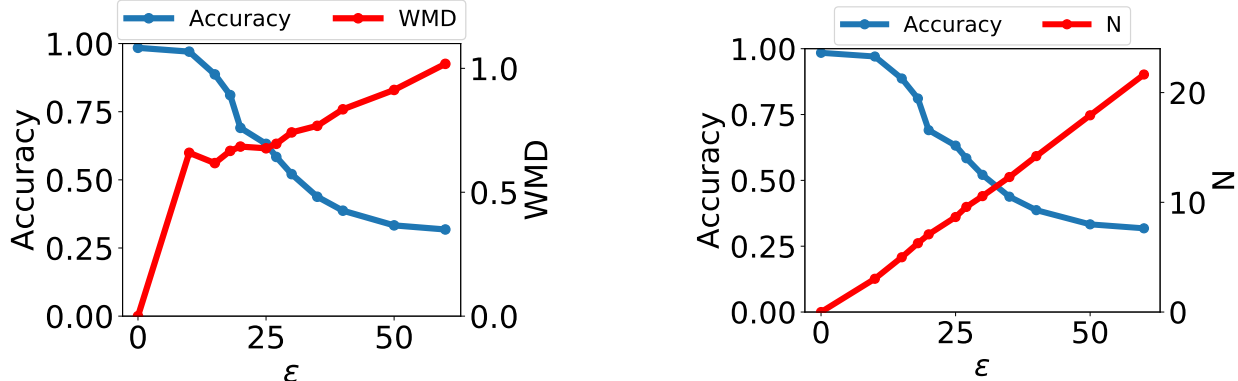
Figure 4.4: Word-level model’s accuracy with varying DeepFool overshoot value. The WMD and N (number of words changed) empirically show the quality of the adversarial texts. (Image credit: [Gon+18])
