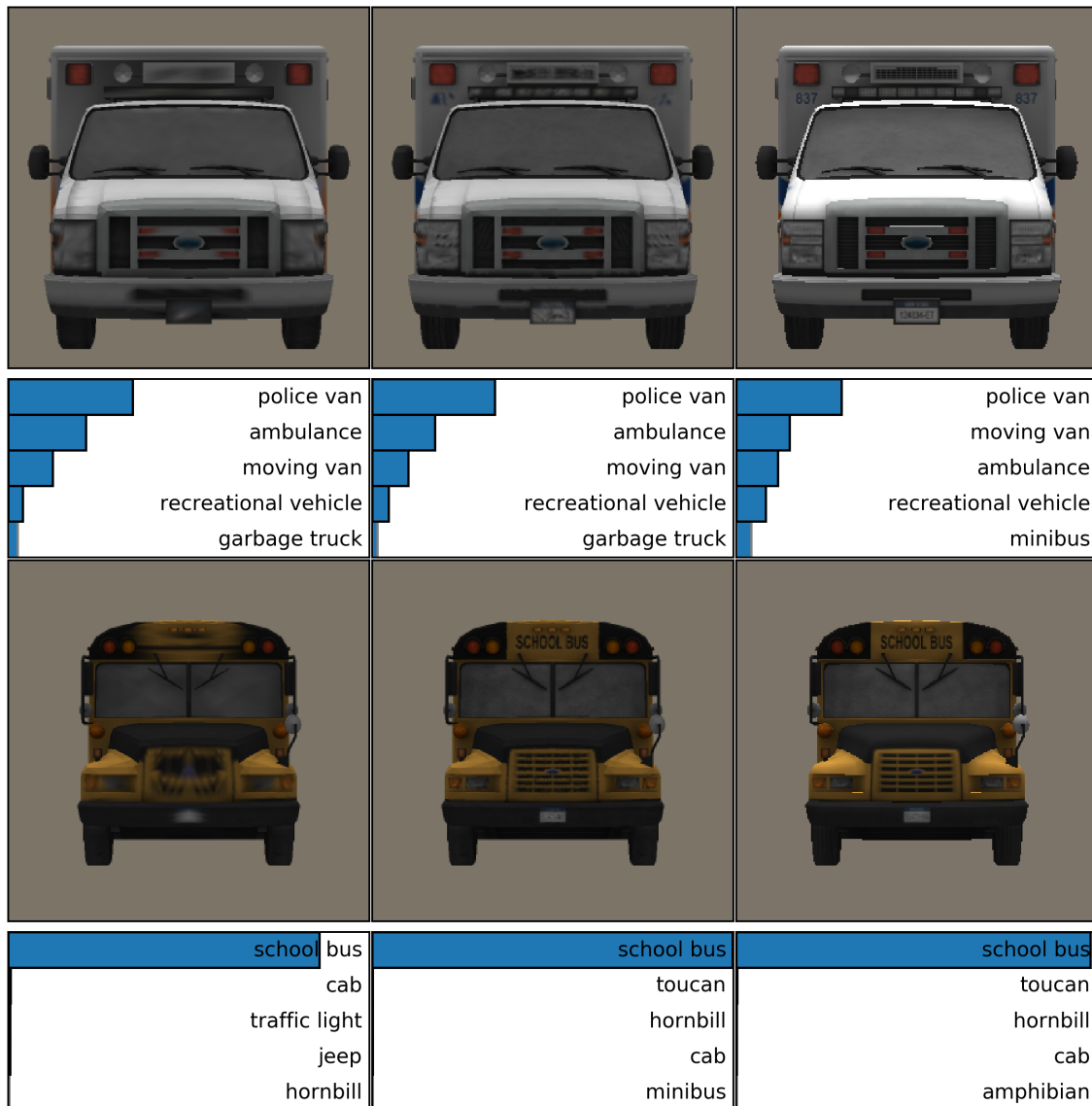
Figure 5.6: A comparison of 3D object renders (here, ambulance and school bus) before and after tessellation. (a) Original 3D models rendered by the differentiable renderer (DR) [KUH18] without tessellation. (b) DR renderings of the same objects after manual tessellation. (c) The non-differentiable renderer (NR), i.e., ModernGL [Dom19], renderings of the original objects. After manual tessellation, the render quality of the DR appears to be sharper ((a) vs. (b)) and closely matches that of the NR, which also internally tessellates objects ((b) vs. (c)). (Image credit: [Alc+18])
