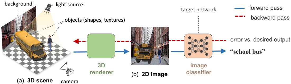
Figure 5.2: To test a target DNN, we build a 3D scene (a) that consists of 3D objects (here, a school bus and a pedestrian), lighting, a background scene, and camera parameters. Our 3D renderer renders the scene into a 2D image, which the image classifier labels school bus . We can estimate the pose changes of the school bus that cause the classifier to misclassify by (1) approximating gradients via finite differences; or (2) back-propagating (red dashed line dashed line) through a differentiable renderer. (Image credit: [Alc+18])
