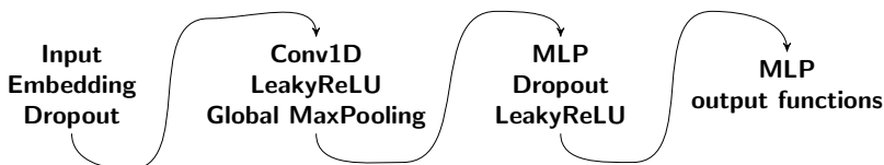
Figure 4.1: Word-level CNN model for text classification. (Image credit: [Gon+18])
