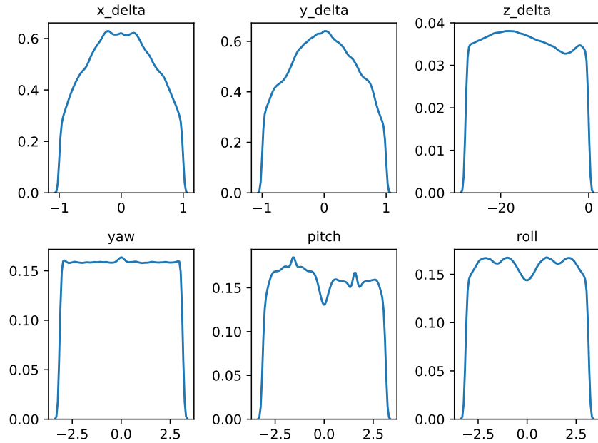
Figure 5.3: The distributions of individual pose parameters for high-confidence ( p \geq 0.7 ) incorrect classifications. x_{\delta} and y_{\delta} have been normalized w.r.t. their corresponding s from Equation (5.3). (Image credit: [Alc+18])
