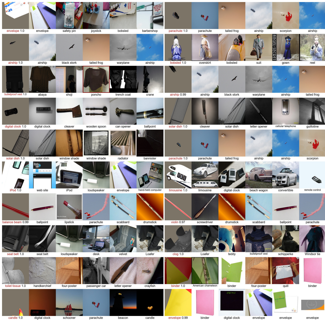
Figure 5.24: For each adversarial example (leftmost), we retrieved the five nearest neighbors (five rightmost photos) from the 50,000-image ImageNet validation set. The Euclidean distance between a pair of images was computed in the fc7 feature space of a pre-trained AlexNet [KSH12]. Below each adversarial example (AX) is its Inception-v3 [Sze+16] top-1 prediction label and confidence score. The associated ground-truth ImageNet label is beneath each retrieved photo. Here, we show an interesting, cherry-picked collection of cases where the nearest photos (in the fc7 feature space) are also qualitatively similar to the reference AX and sometimes come from the exact same class as the AX’s predicted label. More examples are available at https://goo.gl/8ib2PR . (Image credit: [Alc+18])
