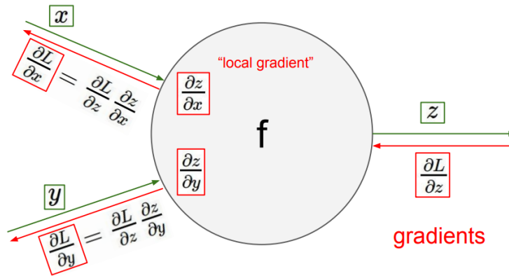
Figure 2.3: The error backpropagation in a single neuron. The green lines are forward pass, while the red lines are backward pass, i.e., the back-propagation. The error L is passed back through the system following the chain rule to calculate each weight’s contribution to the error term, e.g., \frac{\partial L}{\partial x} , \frac{\partial L}{\partial y} . (Image credit cs231n)
