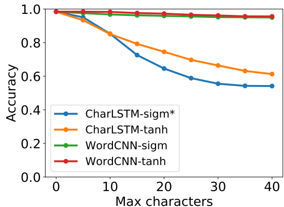
(b) Transferability of adversarial texts generated via Hotflip on character-level. The CharLSTM-sigm is the model used to generate the adversarial texts. (Image credit: [Gon+18])
