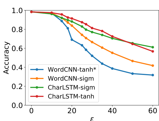
(a) Transferability of adversarial texts generated via DeepFool on word-level. The WordCNN-tanh is the model used to generate the adversarial texts.
