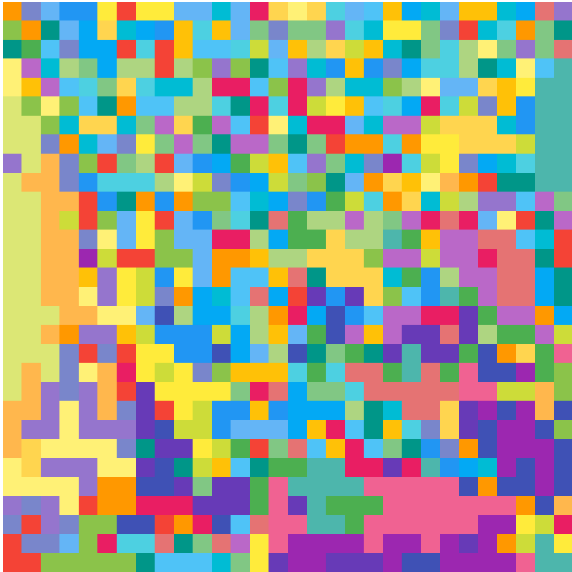
Figure 5.12: The same t-SNE as that in Figure 5.11 but using a unique color to denote the 3D object used to render the adversarial image (i.e., Inception-v3’s misclassification labels are not shown here). The original, high-resolution figure is available at https://goo.gl/TGgPgB . Compare and contrast this plot with the t-SNE of correctly classified poses (Figure 5.10). (Image credit: [Alc+18])
