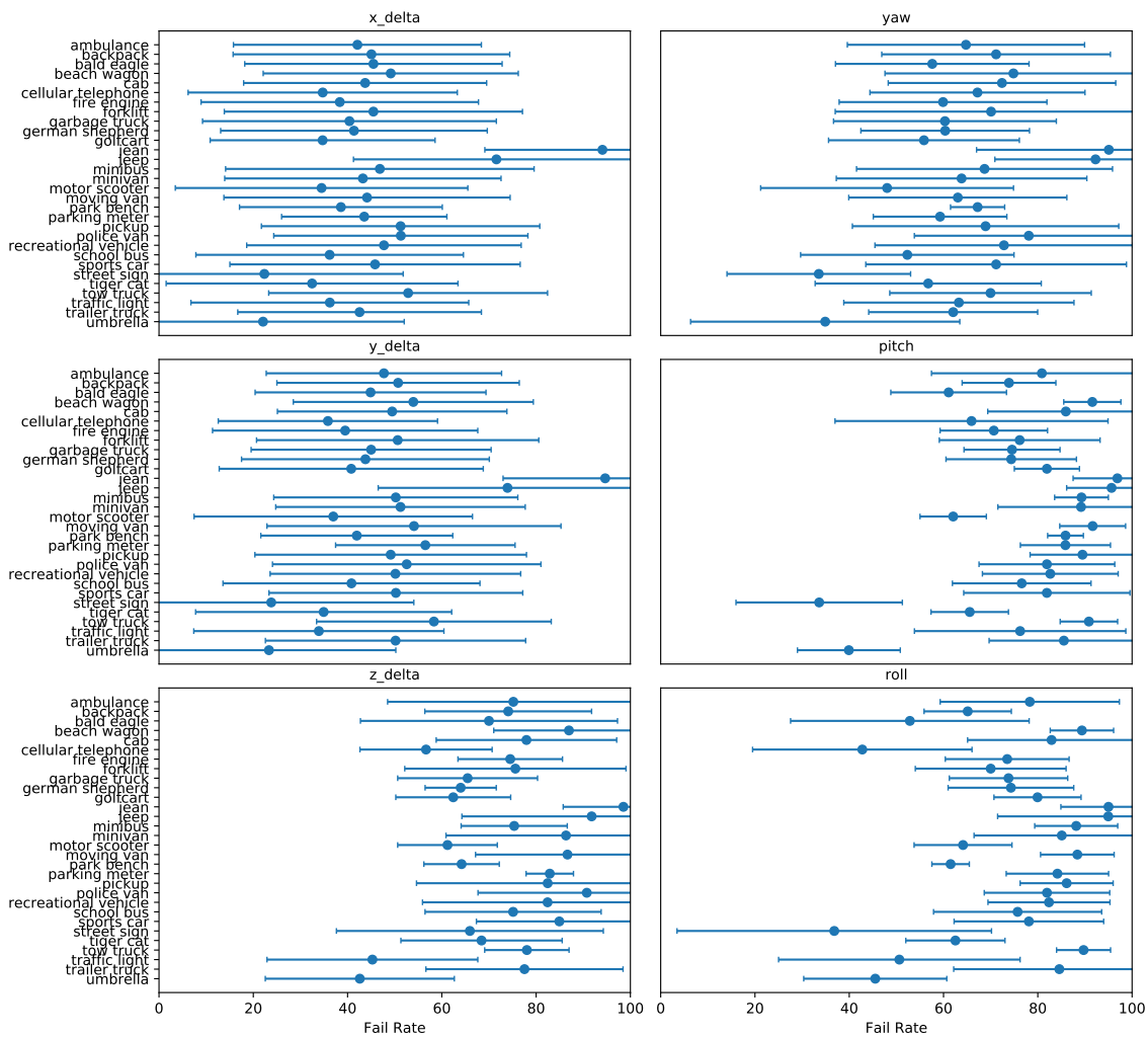
Figure 5.23: Inception-v3 [Sze+16] is sensitive to single parameter disturbances of object poses that had originally been correctly classified. For each object, we found 100 correctly classified 6D poses via a random sampling procedure (Section 5.3.3). Given each such pose, we re-sampled one parameter (shown on top of each panel, e.g., yaw) 100 times, yielding 100 classifications, while holding the other five pose parameters constant. In each panel, for each object (e.g., ambulance), we show an error plot for all resultant 100 \times 100 = 10,000 classifications. Each circle denotes the mean misclassification rate (Fail Rate) for each object, while the bars enclose one standard deviation. Across all objects, Inception-v3 is more sensitive to changes in yaw, pitch, roll, and depth ( z_{\text{delta}} ) than spatial changes ( x_{\text{delta}} and y_{\text{delta}} ). (Image credit: [Alc+18])
