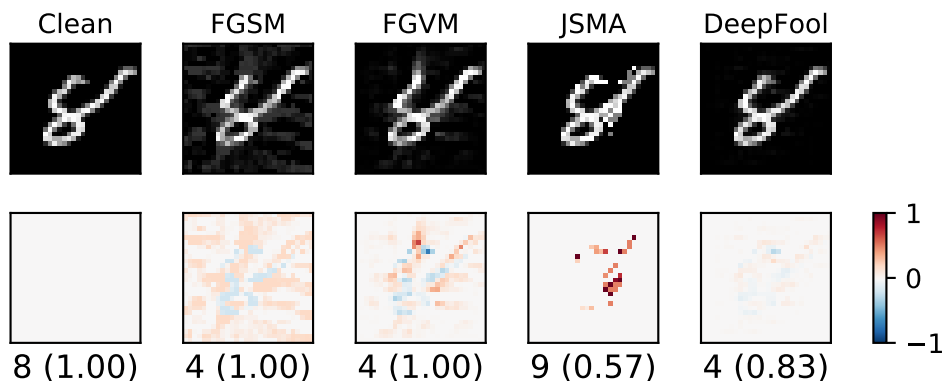
Figure 1.1: Adversarial images from a clean data sample in MNIST dataset [LC10]. The leftmost column is the clean image. The rest columns show 1) on the top, the adversarial images (top) and 2) on the bottom, the pixel difference between the adversarial image and the clean one. The labels on top of each column are the methods used to generate the adversarial samples. The labels below are the predictions by a well-trained neural network model (with test accuracy over 99% on clean test data) with probabilities (interpreted as confidence) in parenthesis. Note that the pixel values are normalized to (0, 1) before being fed into the classification model. As a result, the noise value range is (-1, 1) .
