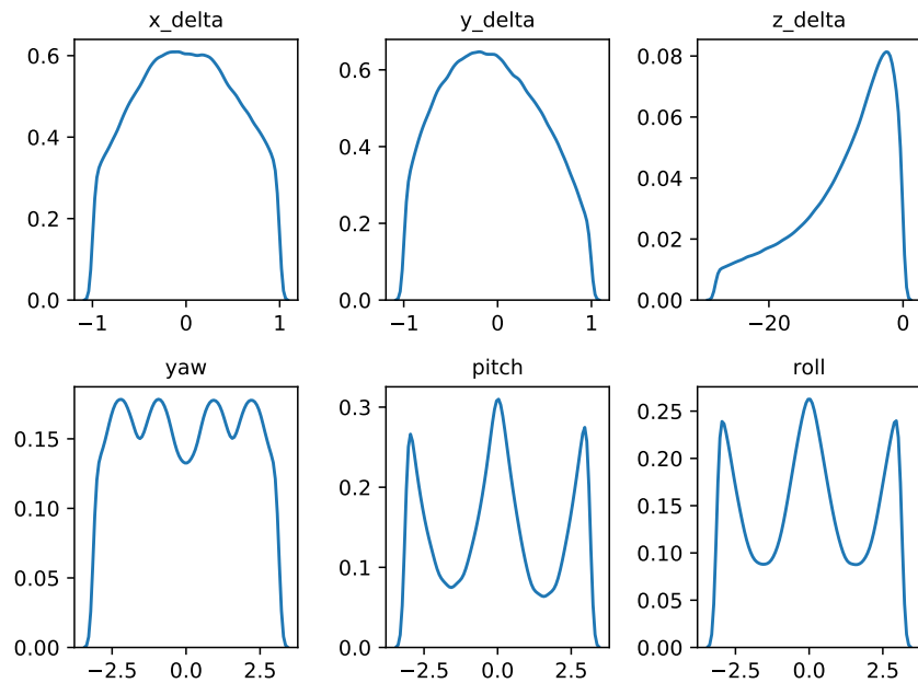
Figure 5.4: The distributions of individual pose parameters for high-confidence ( p \geq 0.7 ) correct classifications obtained from the random sampling procedure described in Section 5.2.5. x_{\delta} and y_{\delta} are also normalized as well. (Image credit: [Alc+18])
