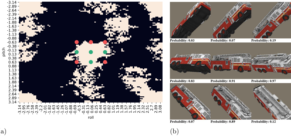
Figure 5.5: Inception-v3’s ability to correctly classify images is highly localized in the rotation and translation parameter space. (a) shows the classification landscape for a fire truck object when altering \theta_r and \theta_p and holding (x_\delta, y_\delta, z_\delta, \theta_y) at (0, 0, -3, \frac{\pi}{4}) , where light regions correspond to correct classifications while dark regions correspond to incorrect classifications. Green and red dots indicate correct and incorrect classifications, respectively, corresponding to the fire truck object poses in (b). (Image credit: [Alc+18])
