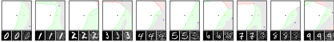
Figure 3.1: Adversarial training [Hua+15; KGB16b] does not work. This is a church window plot [WG16]. Each pixel (i, j) (row index and column index pair) represents a data point \tilde{x} in the input space and \tilde{x} = x + \mathbf{h}\epsilon_j + \mathbf{v}\epsilon_i , where \mathbf{h} is the direction computed by FGSM and \mathbf{v} is a random direction orthogonal to \mathbf{h} . The \epsilon ranges from [-0.5, 0.5] and \epsilon_{(\cdot)} is the interpolated value in between. The central black dot \bullet represents the original data point x , the orange dot (on the right of the center dot) \bullet represents the last adversarial sample created from x via FGSM that is used in the adversarial training and the blue dot \bullet represents a random adversarial sample created from x that cannot be recognized with adversarial training. The three digits below each image, from left to right, are the data samples that correspond to the black dot, orange dot and blue dot, respectively. \square ( \square ) represents the data samples that are always correctly (incorrectly) recognized by the model. \square represents the adversarial samples that can be correctly recognized without adversarial training only. And \square represents the data points that were correctly recognized with adversarial training only, i.e., the side effect of adversarial training. (Image credit: [GWK17])
