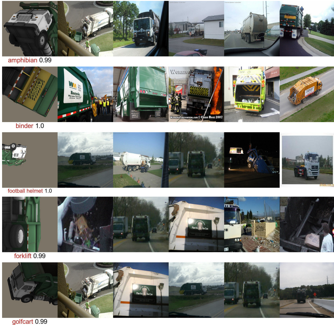
Figure 5.18: For each adversarial example (leftmost), we retrieved the five nearest neighbors (five rightmost photos) from all \sim 1,300 images in the garbage truck class. The Euclidean distance between a pair of images was computed in the fc7 feature space of a pre-trained AlexNet [KSH12]. The nearest photos from the class are mostly different from the adversarial poses. This result supports the hypothesis that the generated adversarial poses are out-of-distribution. The original high-resolution image is available at https://goo.gl/X31VXh . (Image credit: [Alc+18])
