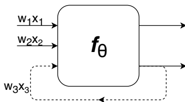
Figure 2.2: A general illustration of a neuron, which is a function. Some neurons may have internal parameters, e.g., filters in the convolution network. Others may have feedback loop, i.e., dotted lines in the figure, e.g., LSTM cells.
