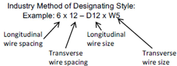
Figure 2-1 Welded Wire Reinforcement designation (Wire Reinforcement Institute 2016)
