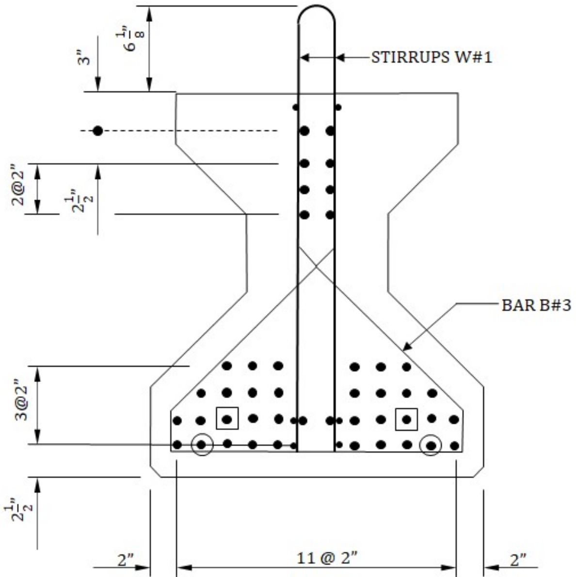
Figure 5-14 End cross section of modified AASHTO Type I girder
