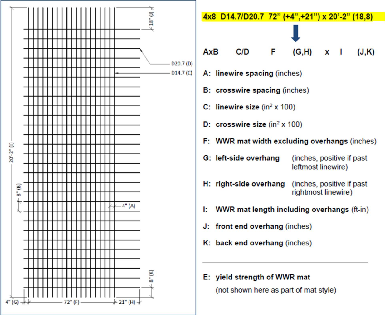
Figure 2-2 Welded Wire Reinforcement Layout (Wire Reinforcement Institute 2021)
