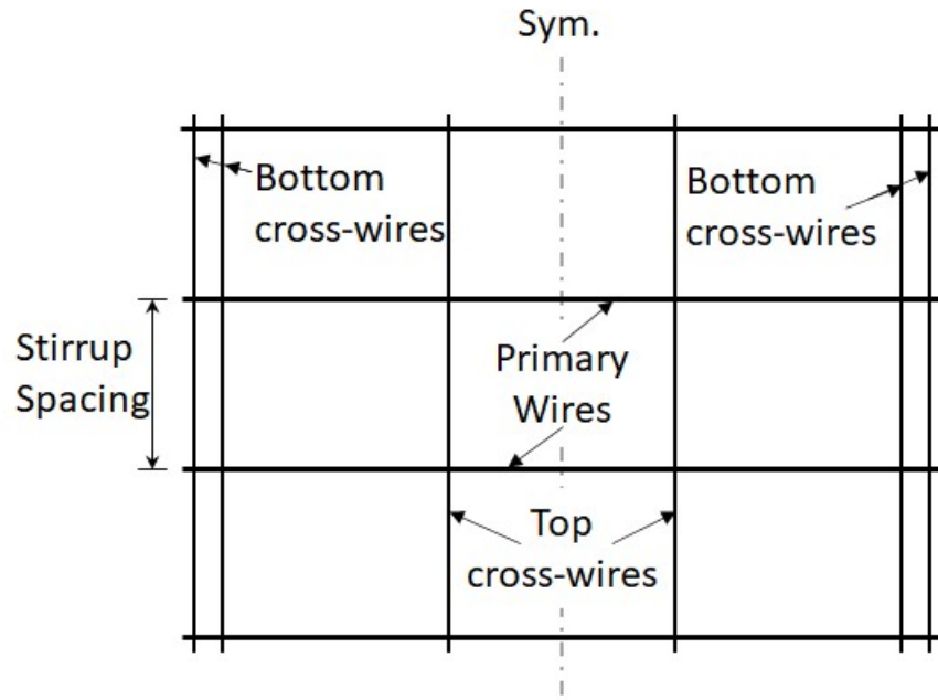
Figure 4-1 Typical WWR U-stirrup sheet prior to bending
