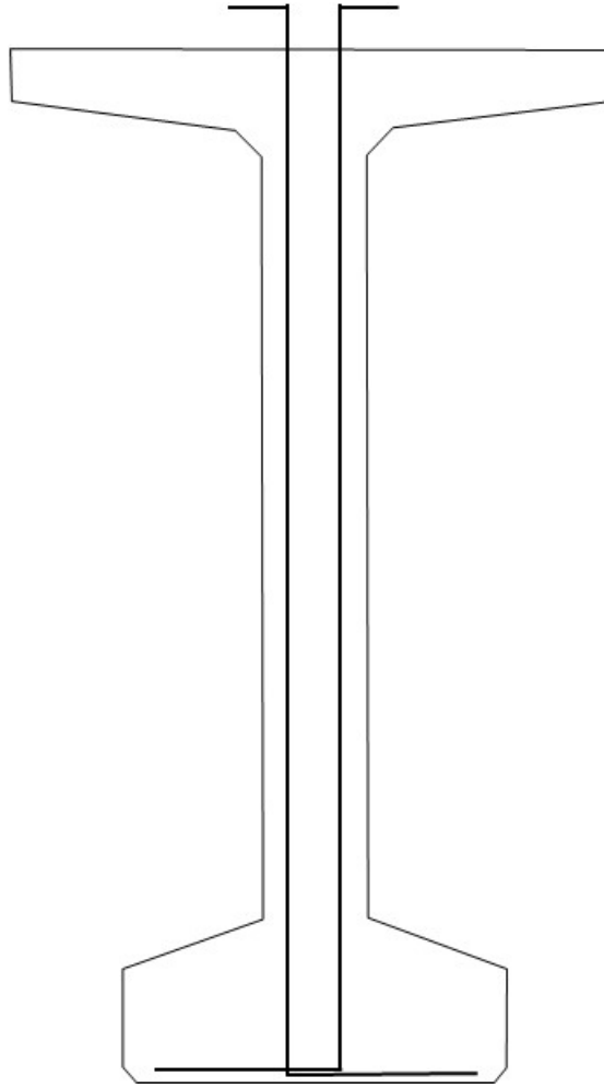
Figure 4-7 Typical reinforcing bar stirrup configuration.
