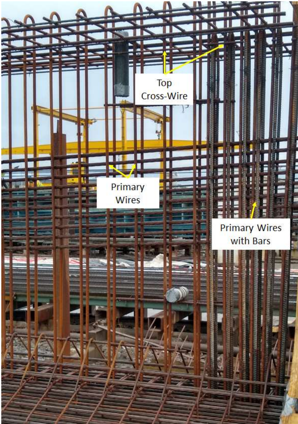
Figure 4-3 WWR stirrups placed in girder.
