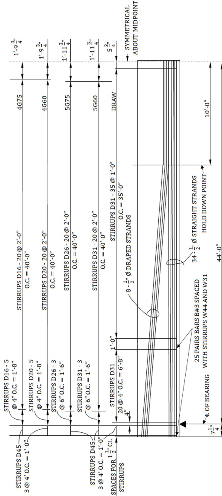
Figure 5-9 AASHTO Type III girder potential stirrup spacing configurations that meet AASHTO requirements
