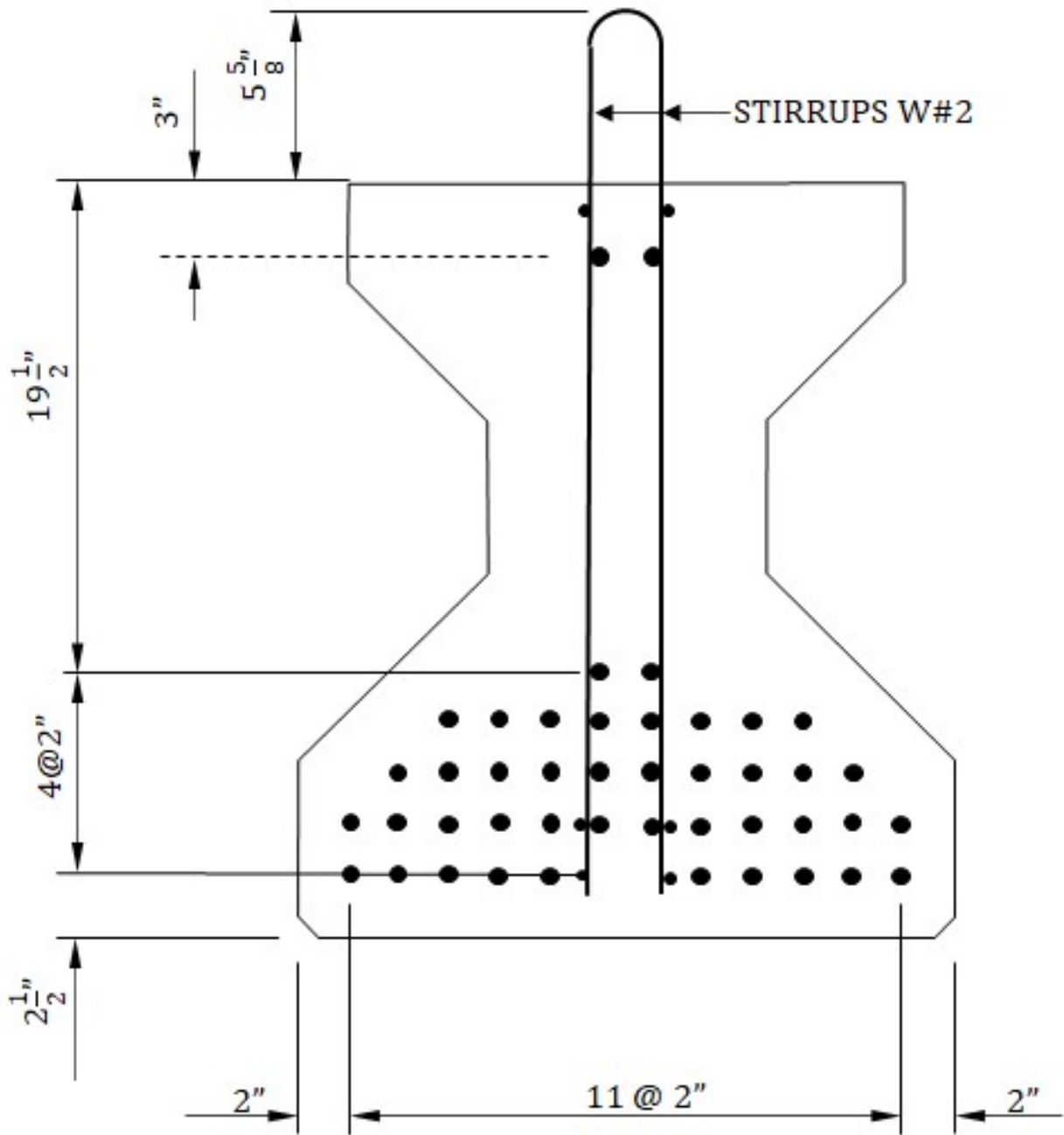
Figure 5-15 Cross section at the hold down point of the modified AASHTO Type I girder
