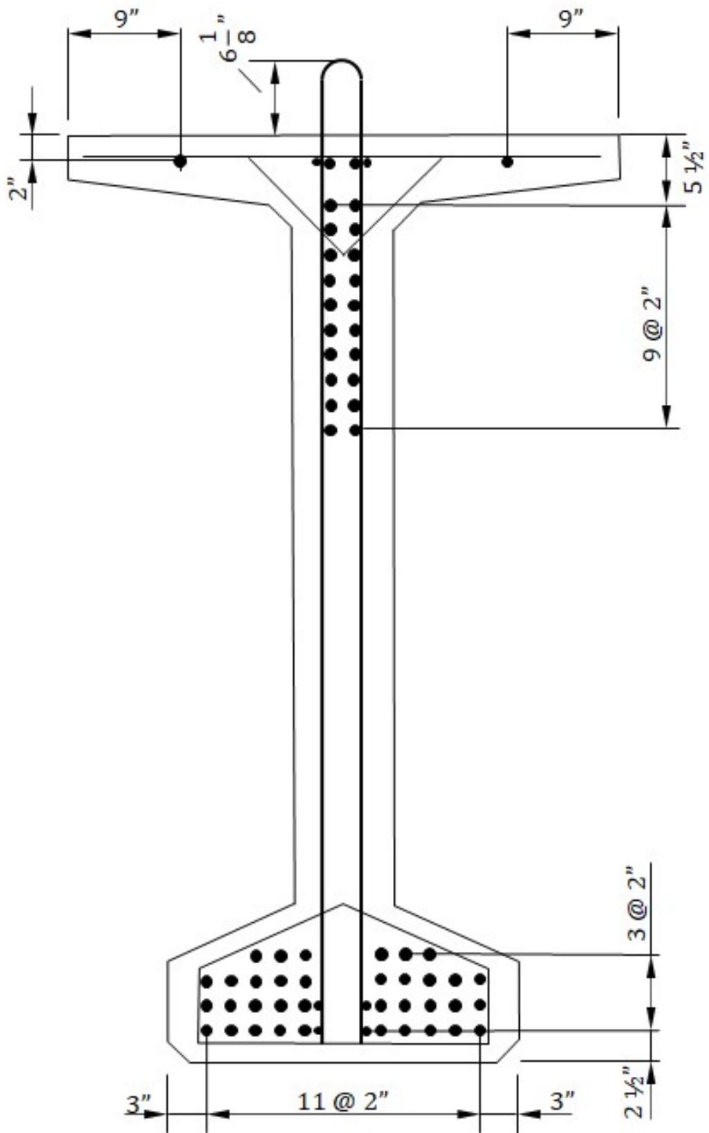
Figure 5-1 End cross section of BT-74 modified section
