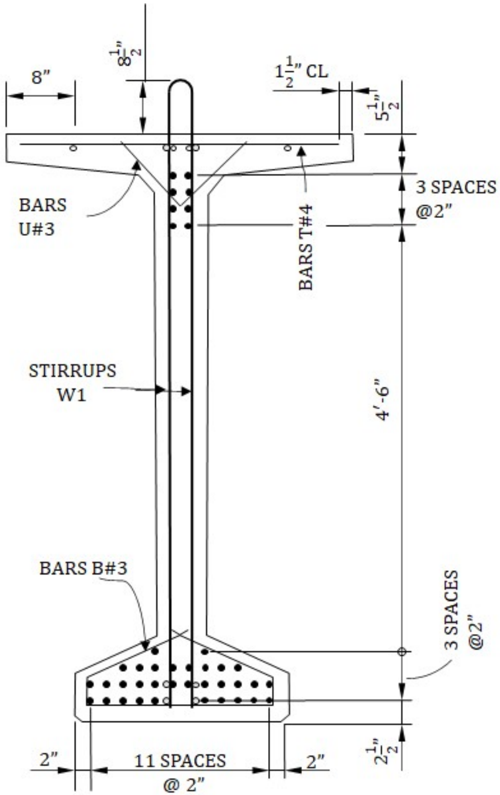
Figure 5-10 End cross section of BT-72 girder
